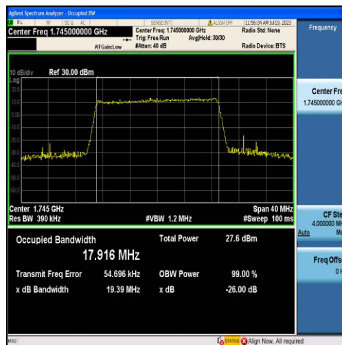
Band4-20MHz-16QAM-20300-100RB#0-17.916
