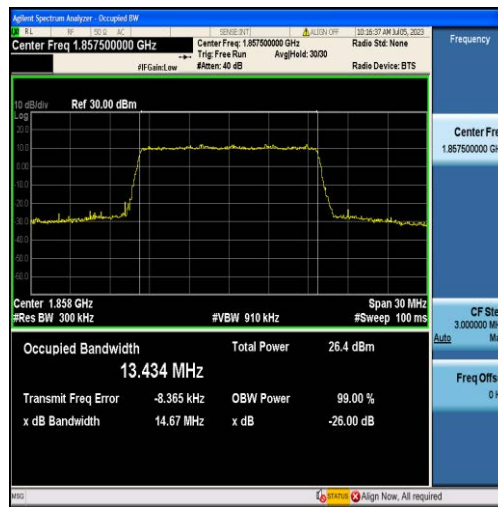
Band2-15MHz-QPSK-18675-75RB#0-13.434
