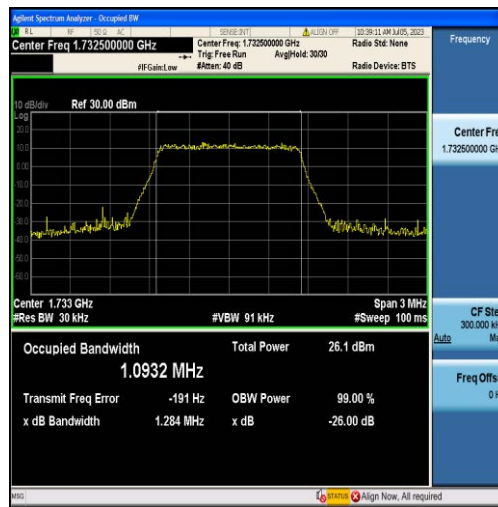
Band4-1.4MHz-16QAM-20175-6RB#0-1.0932
