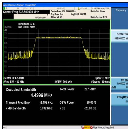
Band5-5MHz-QPSK-20525-25RB#0-4.4996
