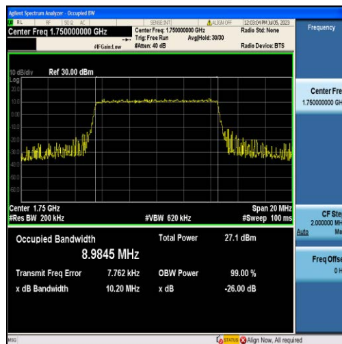
Band4-10MHz-16QAM-20350-50RB#0-8.9845
