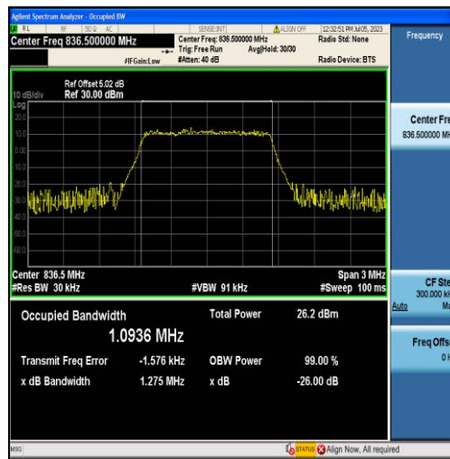
Band5-1.4MHz-16QAM-20525-6RB#0-1.0936
