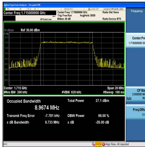
Band4-10MHz-16QAM-20000-50RB#0-8.9674
