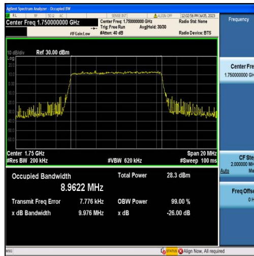
Band4-10MHz-QPSK-20350-50RB#0-8.9622
