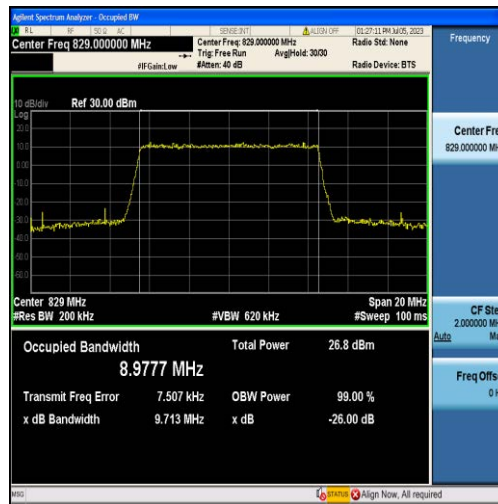
Band5-10MHz-16QAM-20450-50RB#0-8.9777
