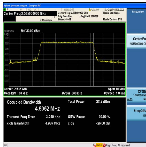
Band7-5MHz-QPSK-21100-25RB#0-4.5052
