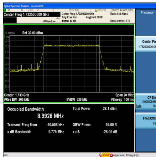
Band4-10MHz-QPSK-20175-50RB#0-8.9928
