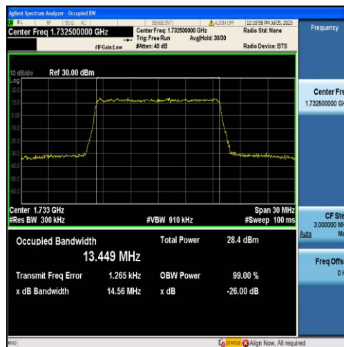
Band4-15MHz-QPSK-20175-75RB#0-13.449
