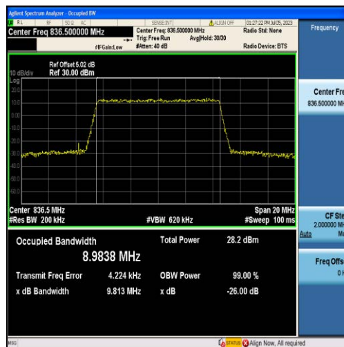
Band5-10MHz-QPSK-20525-50RB#0-8.9838
