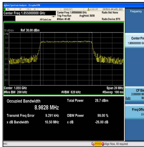
Band2-10MHz-QPSK-18650-50RB#0-8.9828
