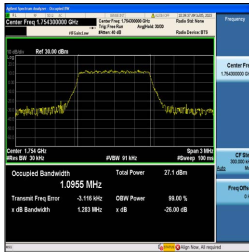
Band4-1.4MHz-QPSK-20393-6RB#0-1.0955
