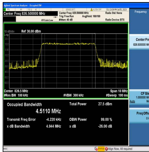
Band5-5MHz-QPSK-20425-25RB#0-4.5110
