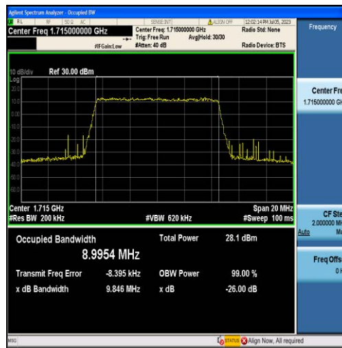
Band4-10MHz-QPSK-20000-50RB#0-8.9954
