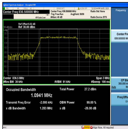
Band5-1.4MHz-QPSK-20525-6RB#0-1.0941
