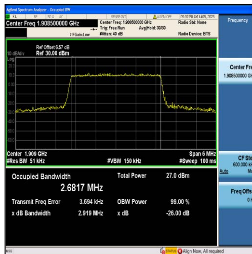
Band2-3MHz-16QAM-19185-15RB#0-2.6817
