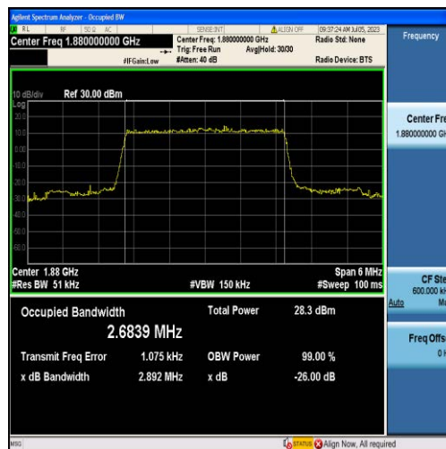
Band2-3MHz-QPSK-18900-15RB#0-2.6839
