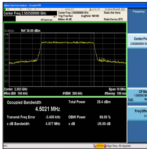
Band7-5MHz-QPSK-20775-25RB#0-4.5021
