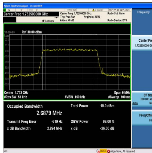
Band4-3MHz-QPSK-20175-15RB#0-2.6879
