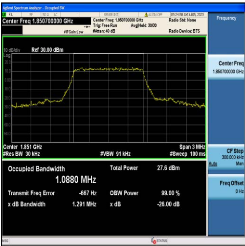
Band2-1.4MHz-QPSK-18607-6RB#0-1.0880
