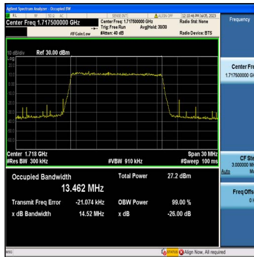
Band4-15MHz-16QAM-20025-75RB#0-13.462
