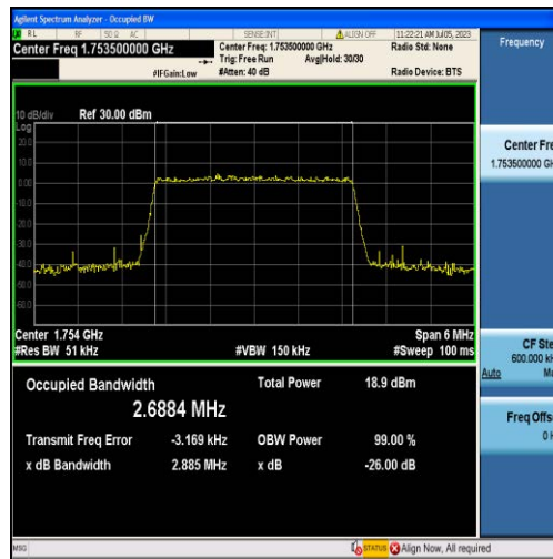
Band4-3MHz-QPSK-20385-15RB#0-2.6884
