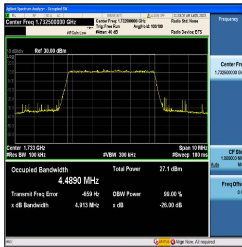
Band4-5MHz-16QAM-20175-25RB#0-4.4890
