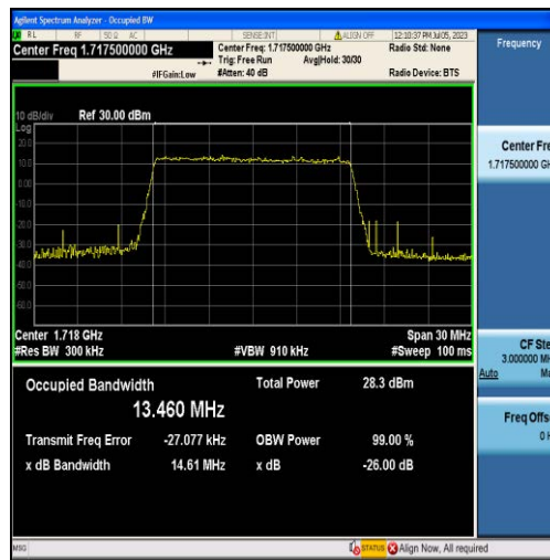
Band4-15MHz-QPSK-20025-75RB#0-13.460
