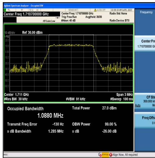
Band4-1.4MHz-QPSK-19957-6RB#0-1.0880
