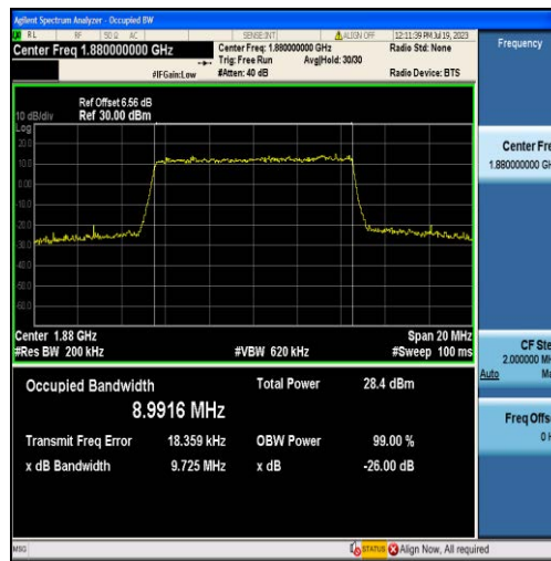
Band2-10MHz-16QAM-18900-50RB#0-8.9916
