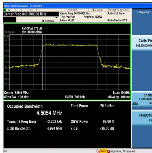
Band5-5MHz-16QAM-20625-25RB#0-4.5054
