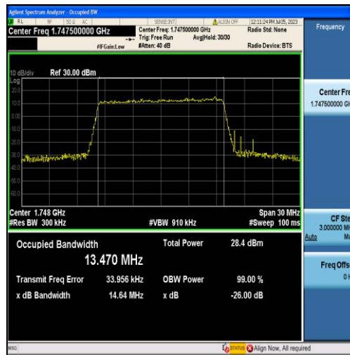
Band4-15MHz-QPSK-20325-75RB#0-13.470
