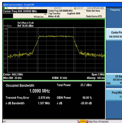
Band5-1.4MHz-16QAM-20643-6RB#0-1.0990
