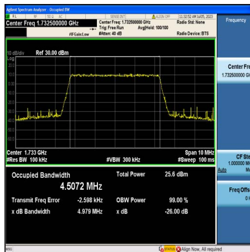
Band4-5MHz-QPSK-20175-25RB#0-4.5072
