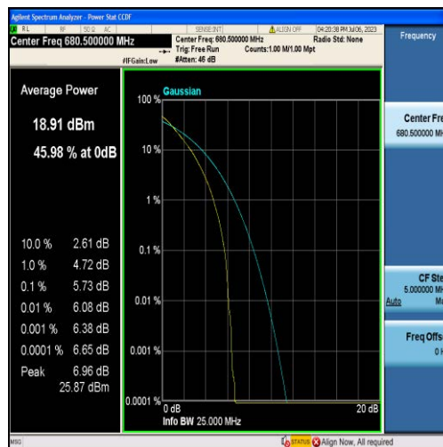
Band71-15MHz-QPSK-133297-75RB#0
