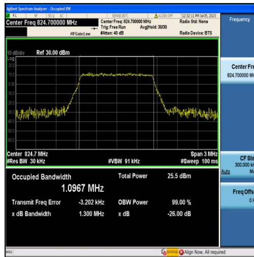
Band5-1.4MHz-16QAM-20407-6RB#0-1.0967
