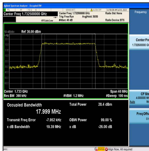
Band4-20MHz-QPSK-20175-100RB#0-17.999
