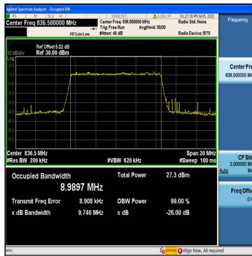
Band5-10MHz-16QAM-20525-50RB#0-8.9897
