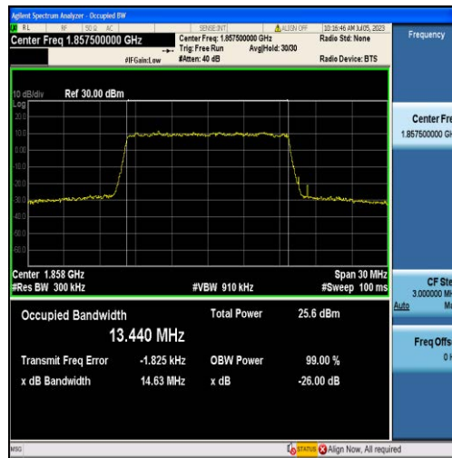
Band2-15MHz-16QAM-18675-75RB#0-13.440
