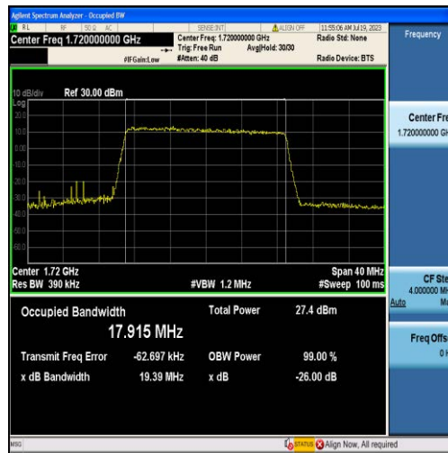
Band4-20MHz-16QAM-20050-100RB#0-17.915
