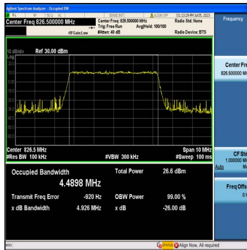
Band5-5MHz-16QAM-20425-25RB#0-4.4898
