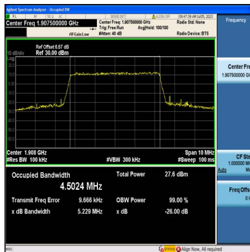
Band2-5MHz-16QAM-19175-25RB#0-4.5024
