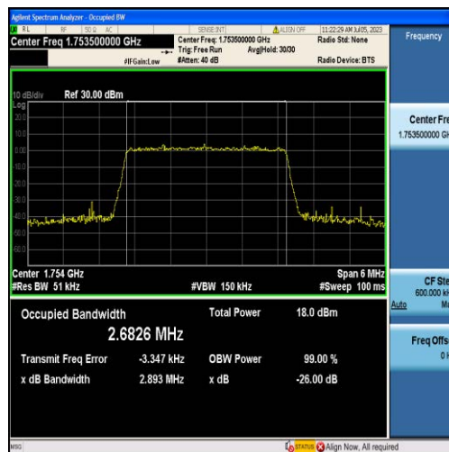
Band4-3MHz-16QAM-20385-15RB#0-2.6826
