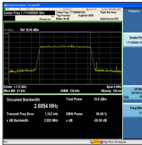
Band4-3MHz-QPSK-19965-15RB#0-2.6854
