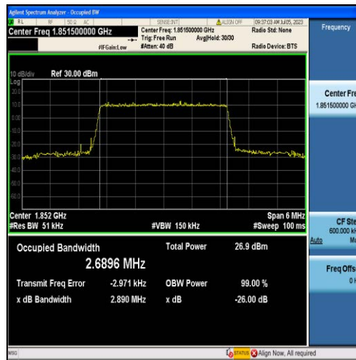
Band2-3MHz-16QAM-18615-15RB#0-2.6896
