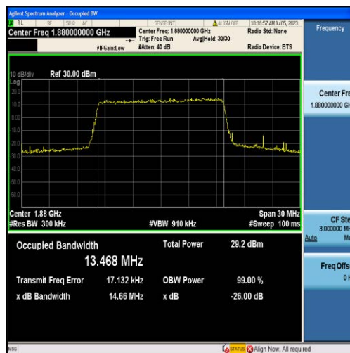
Band2-15MHz-QPSK-18900-75RB#0-13.468
