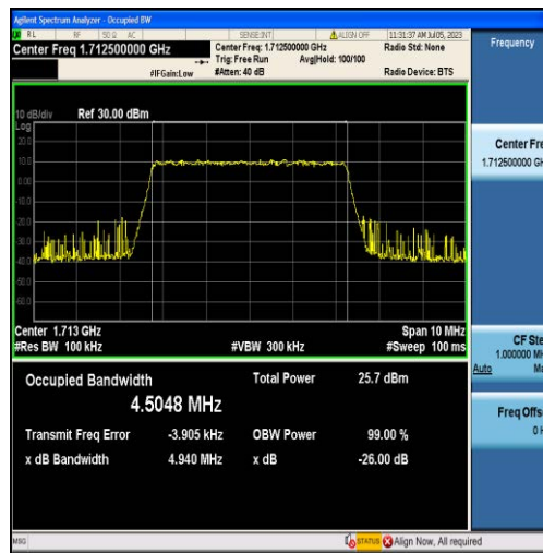
Band4-5MHz-QPSK-19975-25RB#0-4.5048
