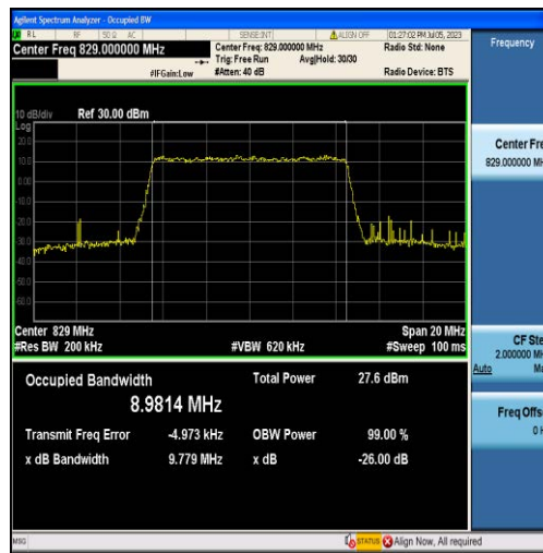
Band5-10MHz-QPSK-20450-50RB#0-8.9814
