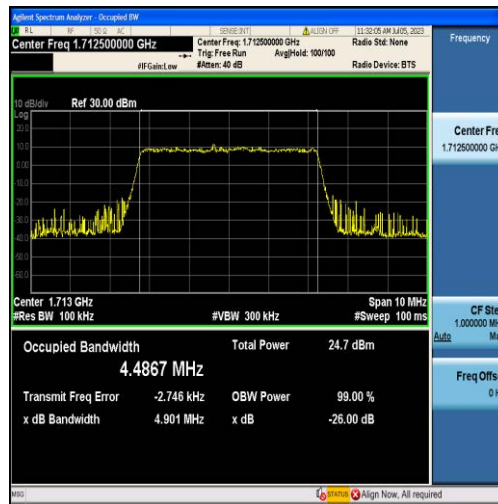
Band4-5MHz-16QAM-19975-25RB#0-4.4867
