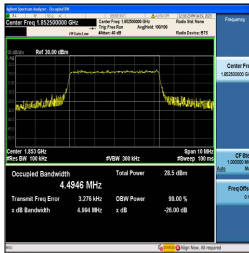
Band2-5MHz-QPSK-18625-25RB#0-4.4946
