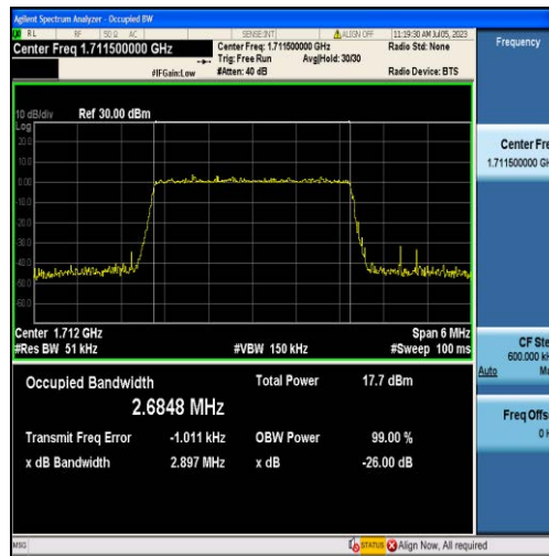
Band4-3MHz-16QAM-19965-15RB#0-2.6848
