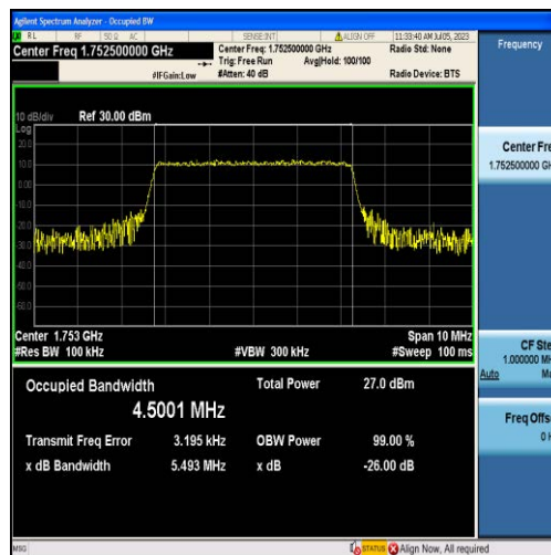
Band4-5MHz-16QAM-20375-25RB#0-4.5001
