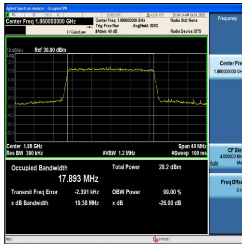
Band2-20MHz-16QAM-18700-100RB#0-17.893
