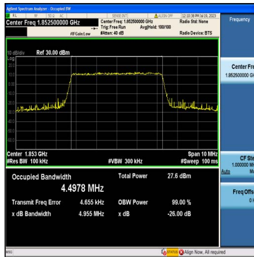
Band2-5MHz-16QAM-18625-25RB#0-4.4978
