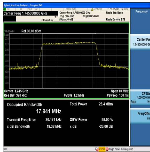
Band4-20MHz-QPSK-20300-100RB#0-17.941
