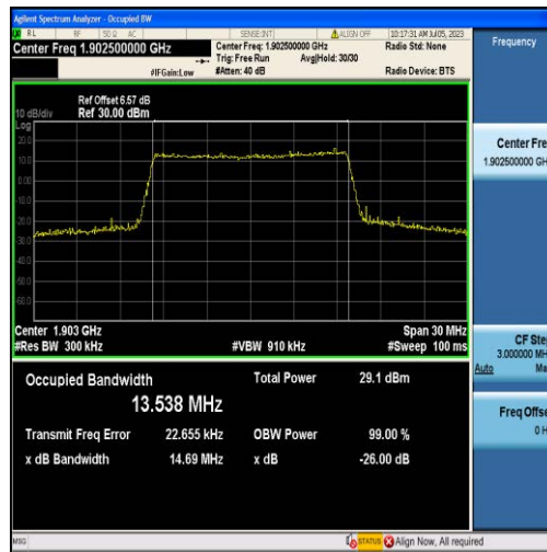
Band2-15MHz-QPSK-19125-75RB#0-13.538
