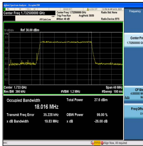
Band4-20MHz-16QAM-20175-100RB#0-18.016
