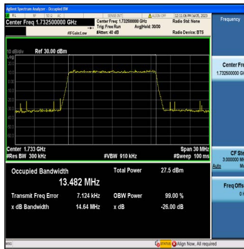
Band4-15MHz-16QAM-20175-75RB#0-13.482
