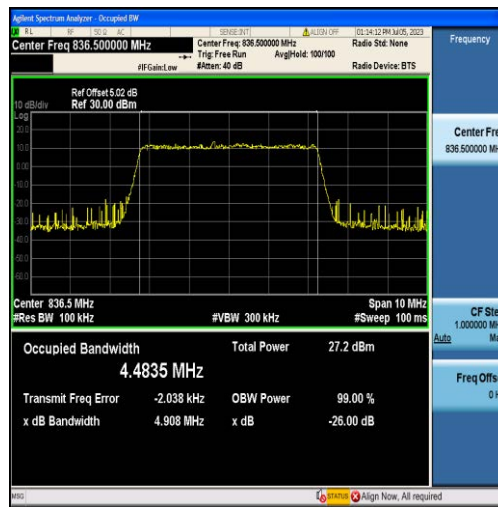
Band5-5MHz-16QAM-20525-25RB#0-4.4835
