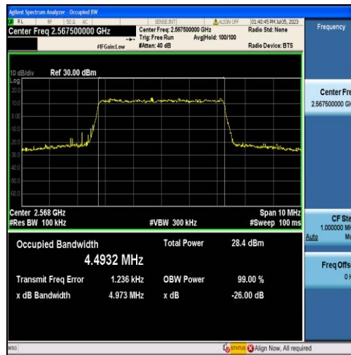
Band7-5MHz-QPSK-21425-25RB#0-4.4932
