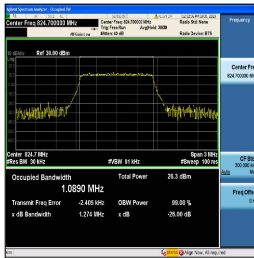
Band5-1.4MHz-QPSK-20407-6RB#0-1.0890
