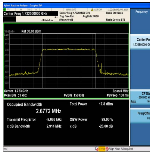
Band4-3MHz-16QAM-20175-15RB#0-2.6772
