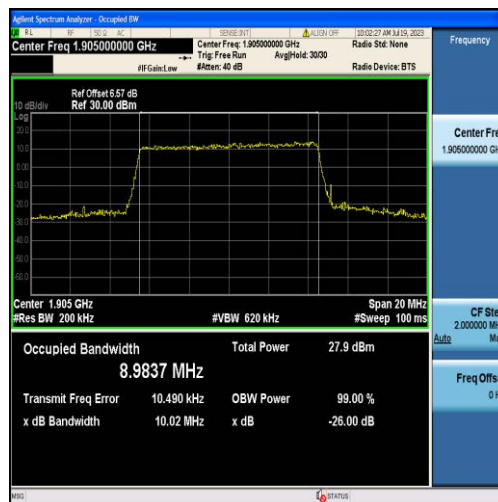
Band2-10MHz-16QAM-19150-50RB#0-8.9837
