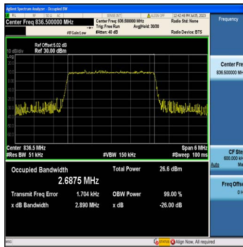
Band5-3MHz-16QAM-20525-15RB#0-2.6875
