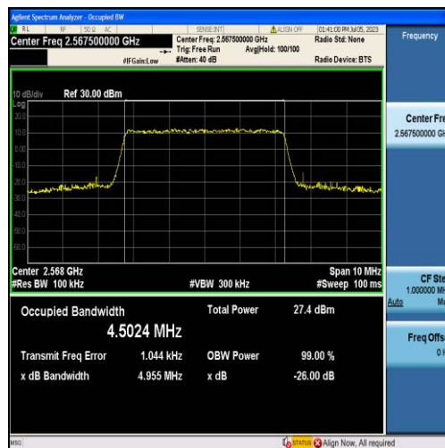
Band7-5MHz-16QAM-21425-25RB#0-4.5024
