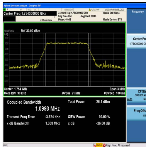
Band4-1.4MHz-16QAM-20393-6RB#0-1.0993
