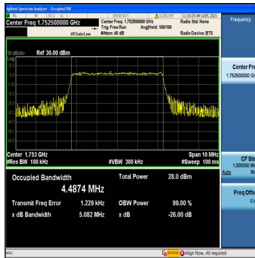
Band4-5MHz-QPSK-20375-25RB#0-4.4874
