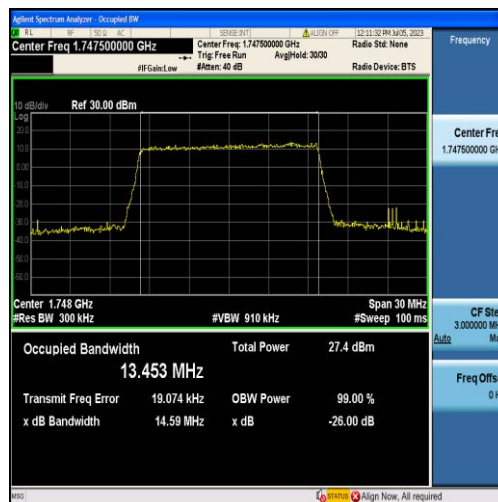
Band4-15MHz-16QAM-20325-75RB#0-13.453
