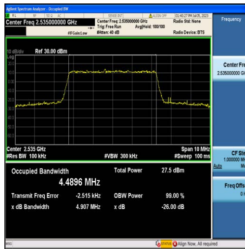
Band7-5MHz-16QAM-21100-25RB#0-4.4896
