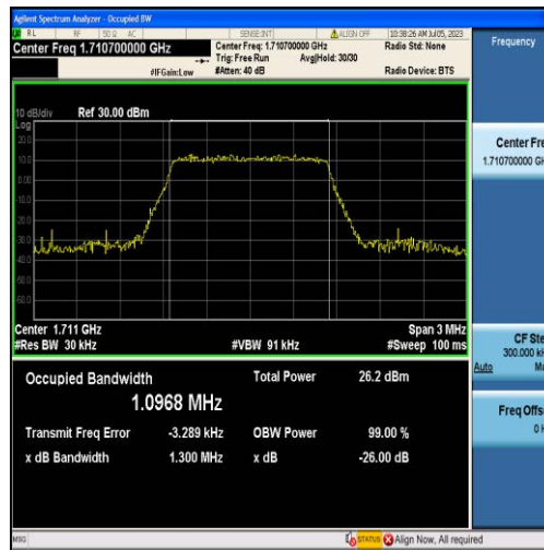
Band4-1.4MHz-16QAM-19957-6RB#0-1.0968
