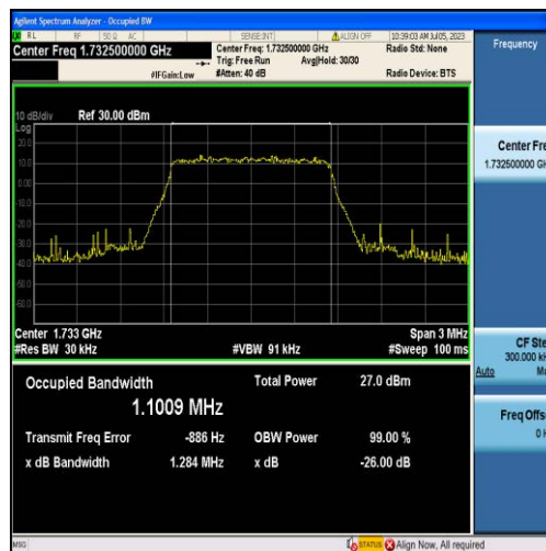
Band4-1.4MHz-QPSK-20175-6RB#0-1.1009
