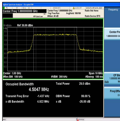
Band2-5MHz-QPSK-18900-25RB#0-4.5047
