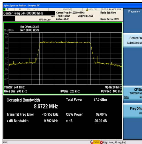
Band5-10MHz-16QAM-20600-50RB#0-8.9722
