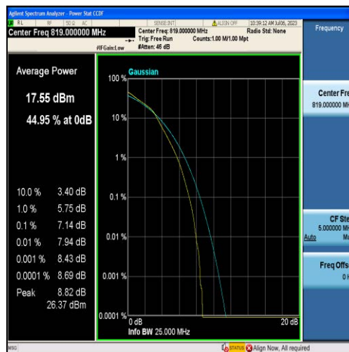
Band26-3MHz-16QAM-26740-15RB#0
