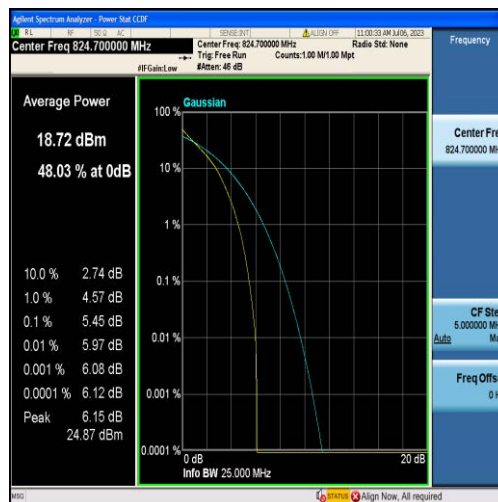
Band26-1.4MHz-QPSK-26797-6RB#0
