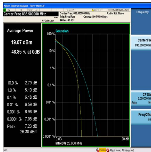
Band26-15MHz-QPSK-26915-75RB#0
