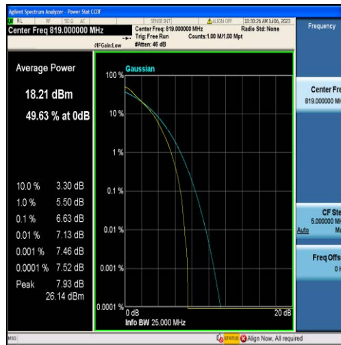
Band26-1.4MHz-QPSK-26740-6RB#0
