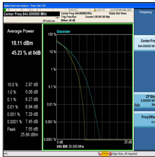
Band26-10MHz-16QAM-26990-50RB#0
