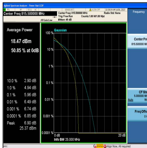
Band26-3MHz-QPSK-26705-15RB#0
