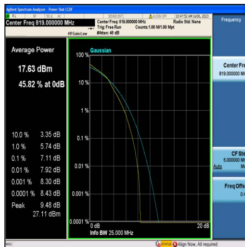
Band26-5MHz-16QAM-26740-25RB#0
