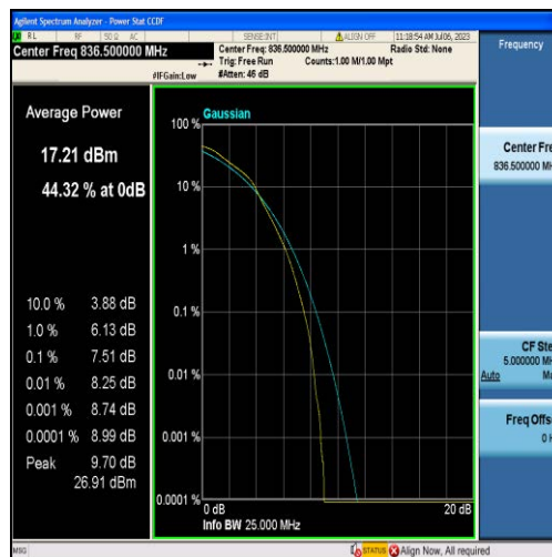
Band26-3MHz-16QAM-26915-15RB#0
