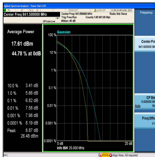
Band26-15MHz-16QAM-26965-75RB#0
