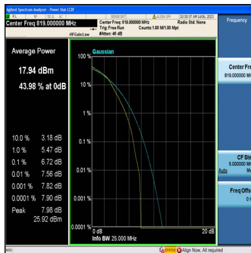
Band26-1.4MHz-16QAM-26740-6RB#0
