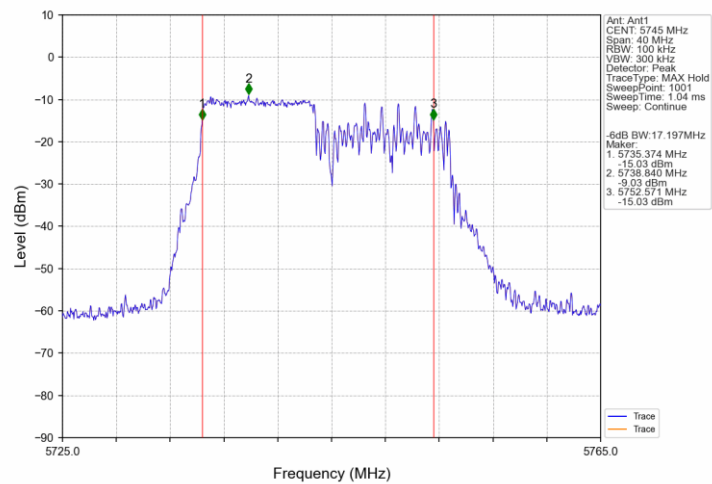
802.11ax(HEW20)_LCH_5745MHz_RU106_Left_Ant1_NTNV
