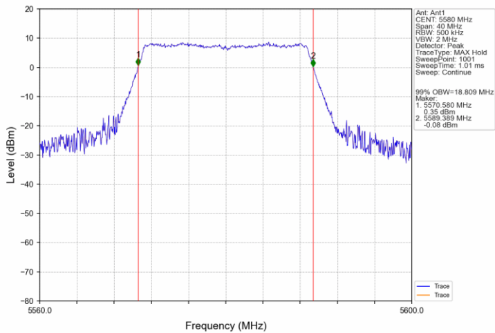
802.11ac(VHT20)_MCH_5580MHz_Ant1_NTNV
