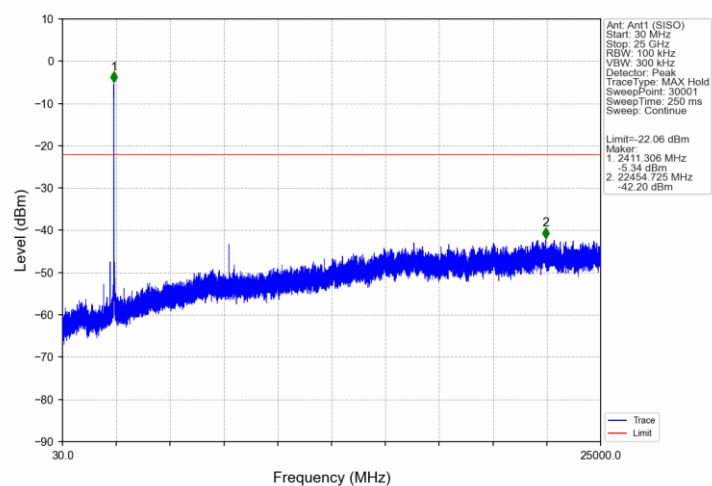
802.11ax(HEW40)_LCH_2422MHz_RU484_65_Ant1 (SISO)_NTNV
