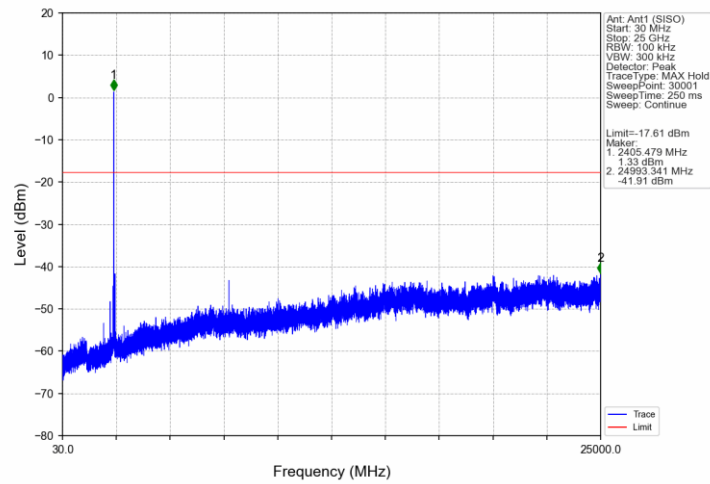
802.11ax(HEW40)_LCH_2422MHz_RU52_40_Ant1 (SISO)_NTNV
