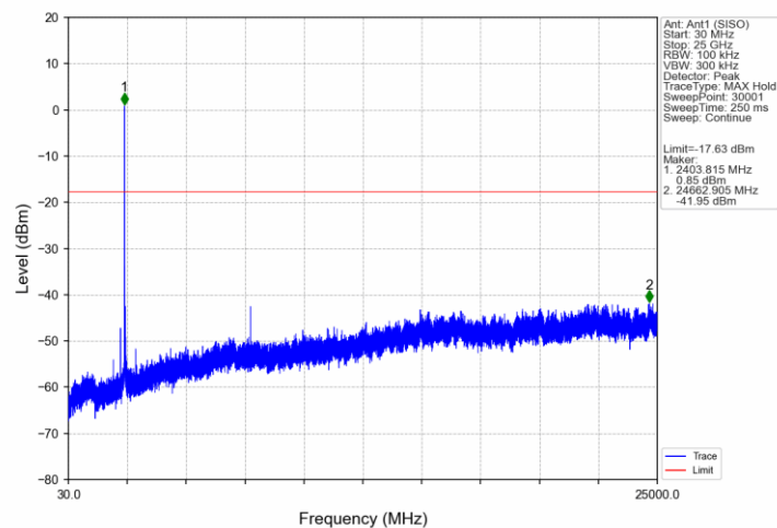
802.11ax(HEW40)_LCH_2422MHz_RU52_44_Ant1 (SISO)_NTNV
