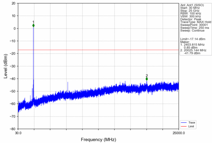
802.11ax(HEW40)_LCH_2422MHz_RU106_53_Ant1 (SISO)_NTNV
