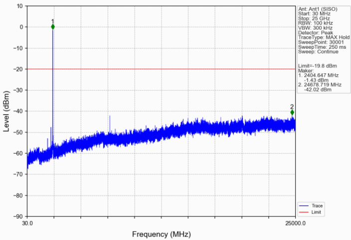
802.11ax(HEW20)_LCH_2412MHz_RU242_61_Ant1 (SISO)_NTNV
