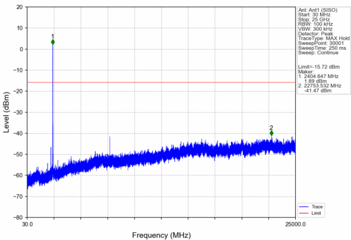
802.11ax(HEW20)_LCH_2412MHz_RU106_53_Ant1 (SISO)_NTNV
