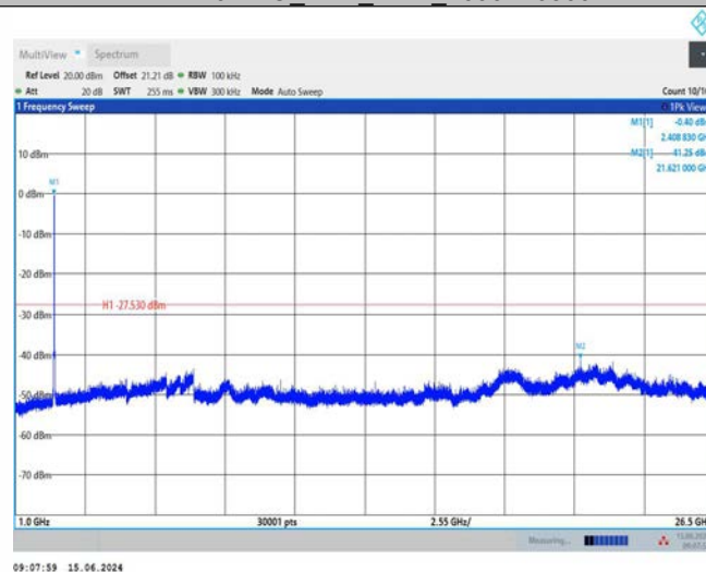
11AX20SISO_Ant1_2437_0~Reference
