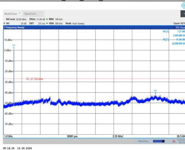
11G_Ant1_2462_0~Reference
