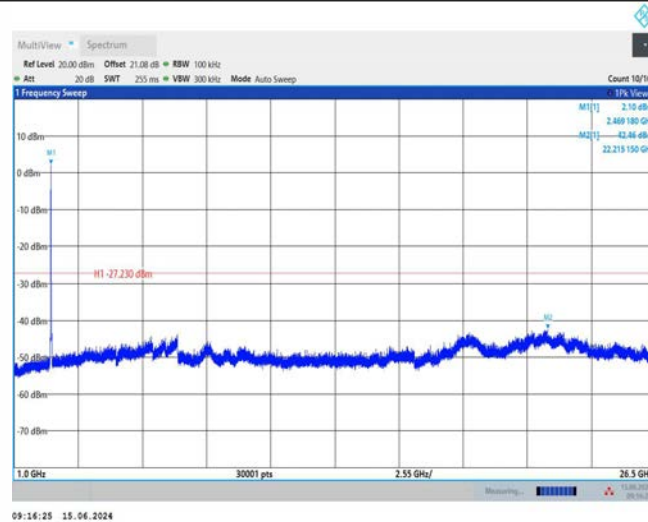
11AX20SISO_Ant1_2462_1000~26500
