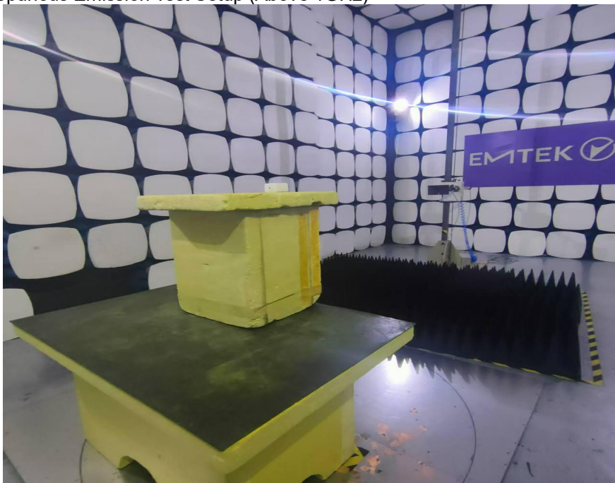
Spurious Emission Test Setup (Above 1GHz)
