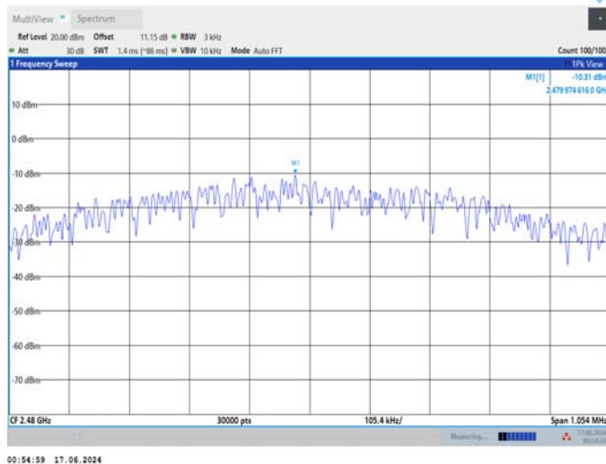
BLE_1M_Ant1_2480
