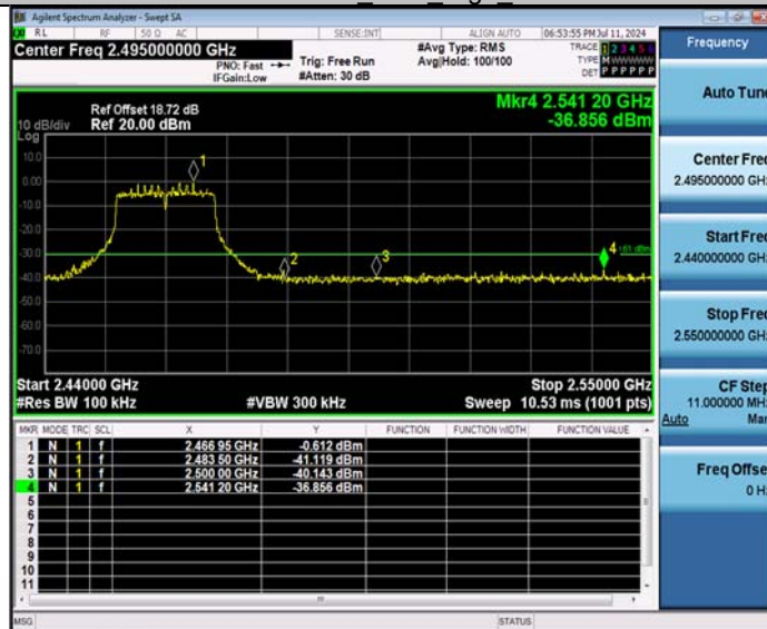
11N20SISO_Ant1_High_2462
