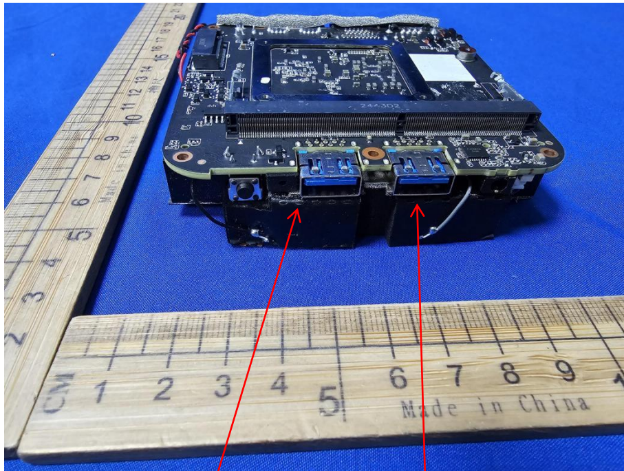
Location of 2.4G Antenna
