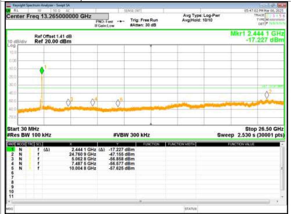
Tx. Spurious NVNT n40 2452MHz Ant2 Emission
