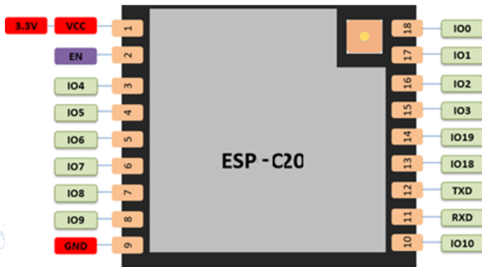
Fig.2.1 ESP-C20 Pins Definition
