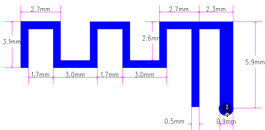
Antenna Dimension for ANT-6651
