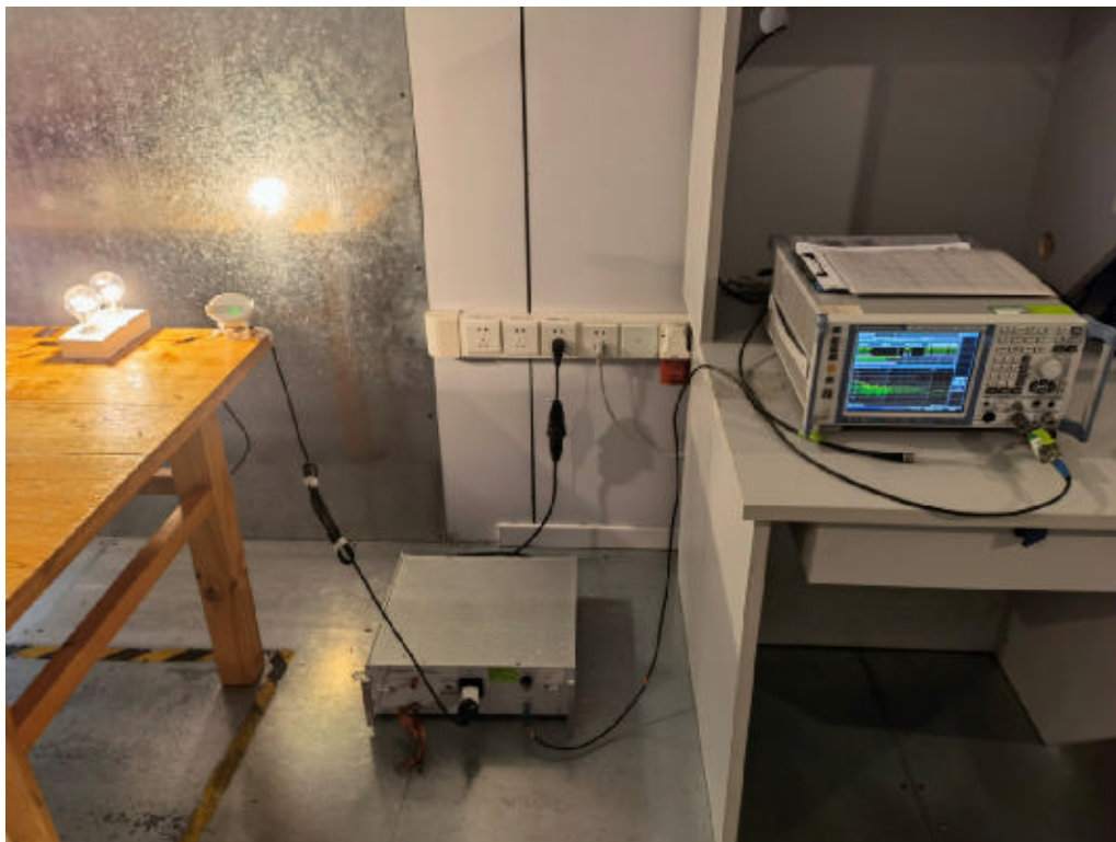
Setup Photo FCC ID: 2BB6O-ISE101-5
