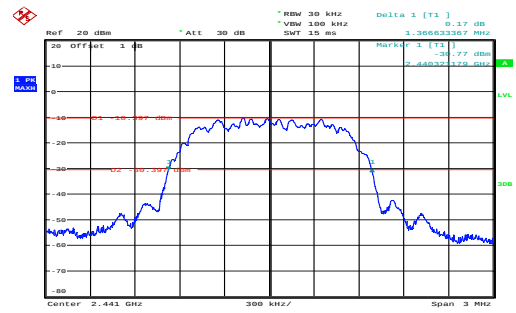
PI/4-DQPSK_Mid_2DH1
