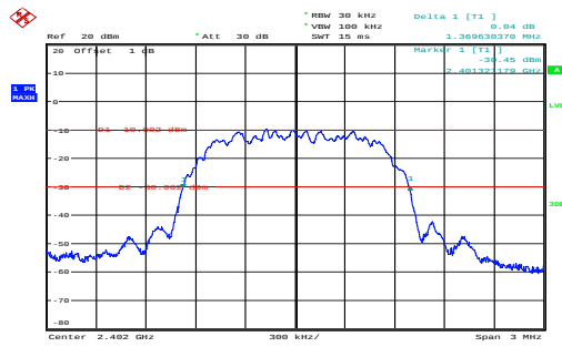
PI/4-DQPSK_Low_2DH1
