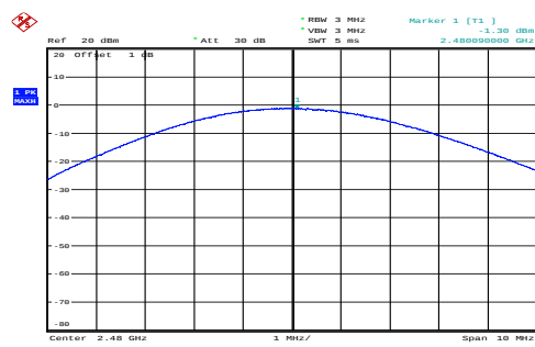
PI/4-DQPSK_High_2DH1
