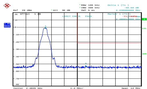
GFSK_High_DH1
