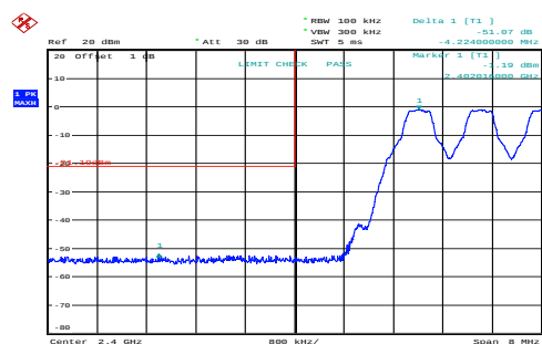
GFSK_Hopping_Lower_DH1
