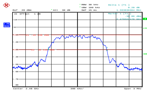
PI/4-DQPSK_High_2DH1
