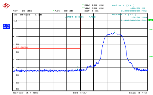
PI/4-DQPSK_Low_2DH1
