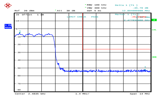
PI/4-DQPSK_Hopping_Upper_2DH1
