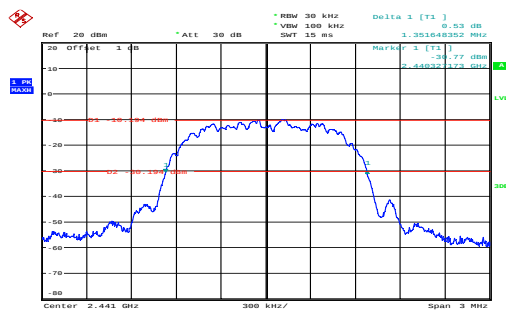
8DPSK_Mid_3DH1
