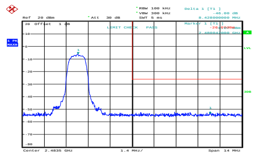
PI/4-DQPSK_High_2DH1
