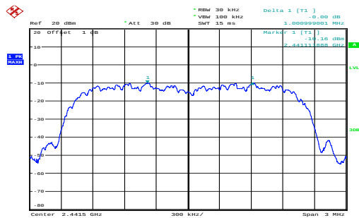
8DPSK_Mid_3DH1
