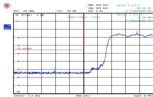
PI/4-DQPSK_Hopping_Lower_2DH1
