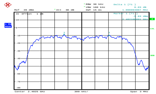
8DPSK_Low_3DH1
