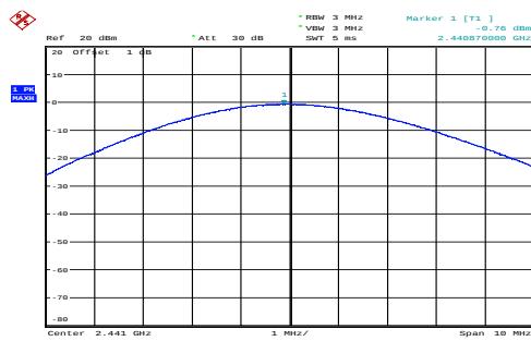
8DPSK_Mid_3DH1
