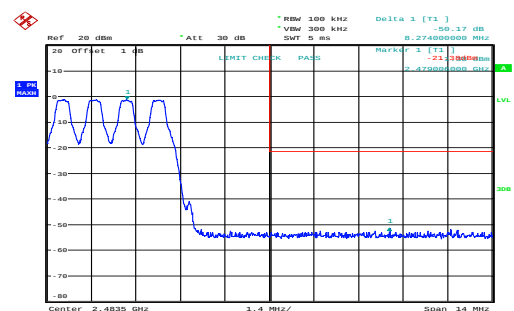
GFSK_Hopping_Upper_DH1
