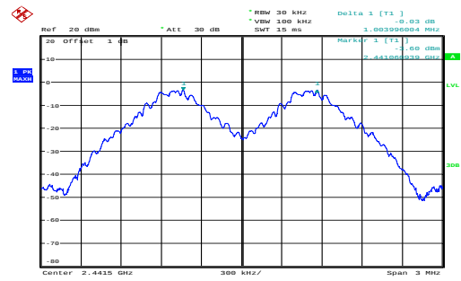
GFSK_Mid_DH1
