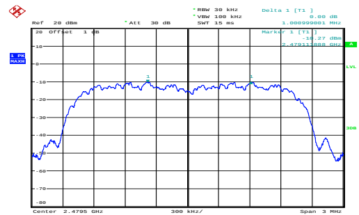
8DPSK_High_3DH1
