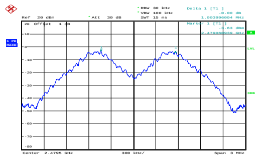
GFSK_High_DH1
