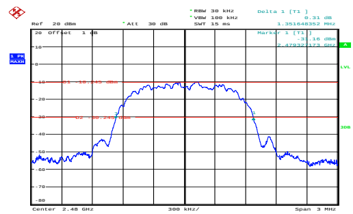
8DPSK_High_3DH1
