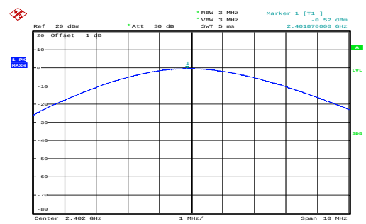
8DPSK_Low_3DH1
