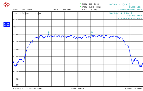
PI/4-DQPSK_High_2DH1
