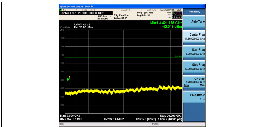
Band66_10MHz_QPSK_131022_1RB#0_3000~131022_3000~131022
