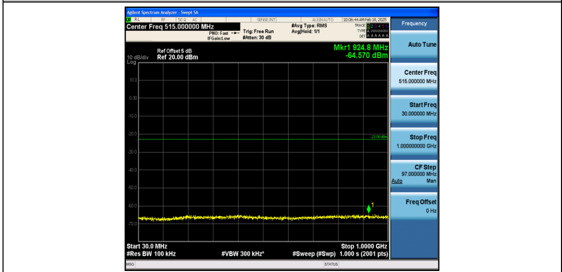
Band66_15MHz_QPSK_132322_1RB#0_30~1000_30~1000
