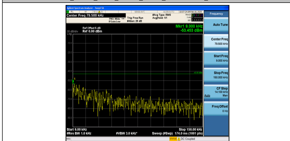
Band66_15MHz_16QAM_132322_1RB#0_0.009~0.15_0.009~0.15
