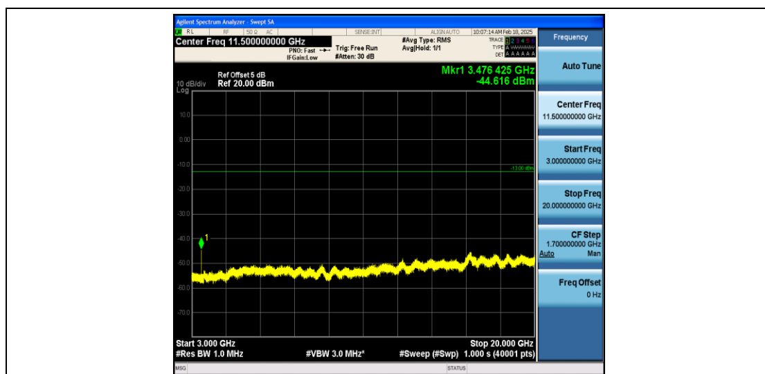
Band66_15MHz_QPSK_132322_1RB#0_3000~131022_3000~131022
