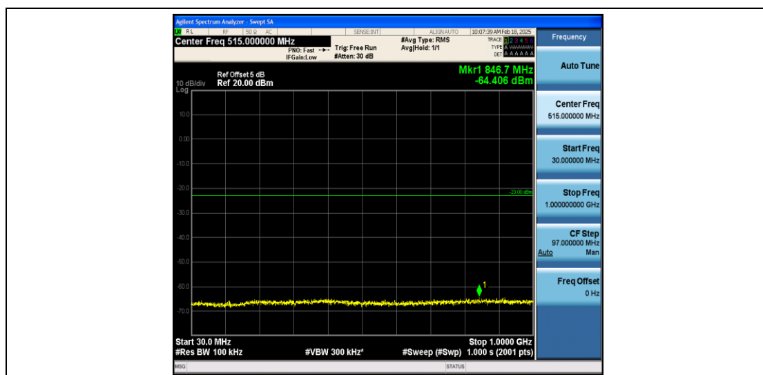
Band66_15MHz_16QAM_132322_1RB#0_30~1000_30~1000
