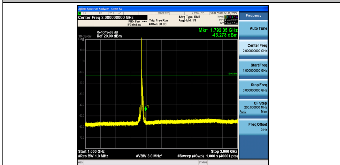
Band66_15MHz_16QAM_132322_1RB#0_1000~3000_1000~3000
