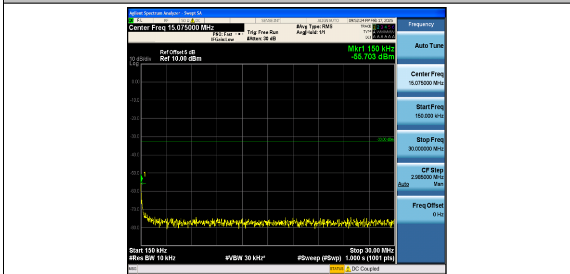
Band66_10MHz_16QAM_131022_1RB#0_0.15~30_0.15~30
