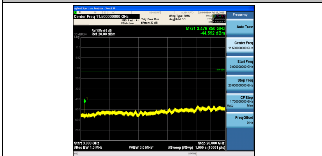
Band66_15MHz_16QAM_132322_1RB#0_3000~131022_3000~131022
