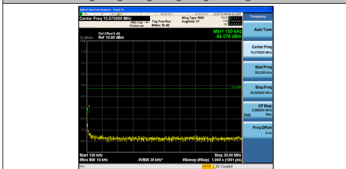
Band66_15MHz_16QAM_132322_1RB#0_0.15~30_0.15~30
