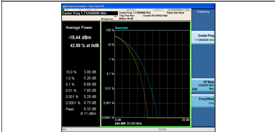
Band66-5MHz-16QAM-131997-1RB#0-PASS
