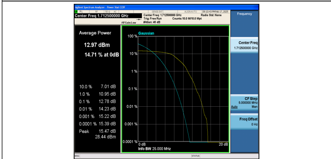
Band66-5MHz-QPSK-131997-1RB#0-PASS
