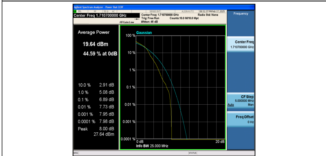
Band66-1.4MHz-16QAM-131979-1RB#0-PASS
