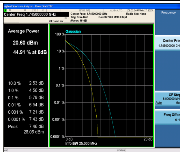
Band66-3MHz-QPSK-132322-15RB#0-PASS
