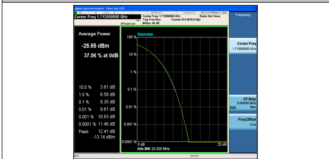
Band66-5MHz-16QAM-131997-25RB#0-PASS
