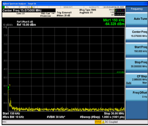
Band41_5MHz_16QAM_39675_1RB#0_0.15~30_0.15~30
