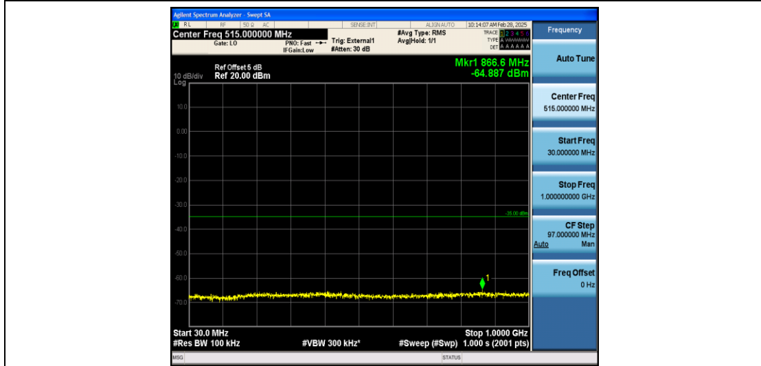
Band41_5MHz_QPSK_39675_1RB#0_30~1000_30~1000
