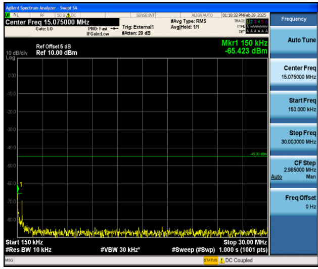
Band41_10MHz_16QAM_39700_1RB#0_0.15~30_0.15~30
