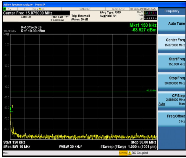
Band41_5MHz_QPSK_41565_1RB#0_0.15~30_0.15~30
