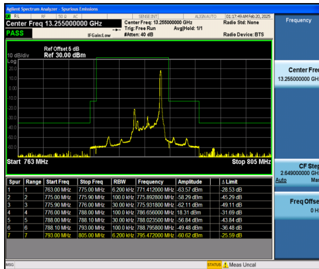
Band13_5MHz_QPSK_23255_1RB#24
