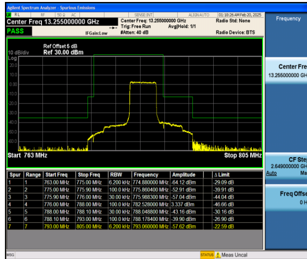
Band13_5MHz_QPSK_23255_25RB#0
