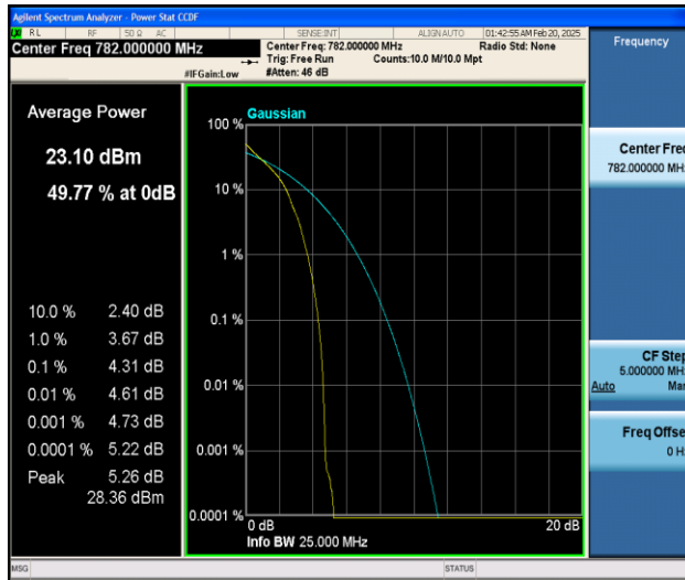
Band13-10MHz-QPSK-23230-1RB#0-PASS
