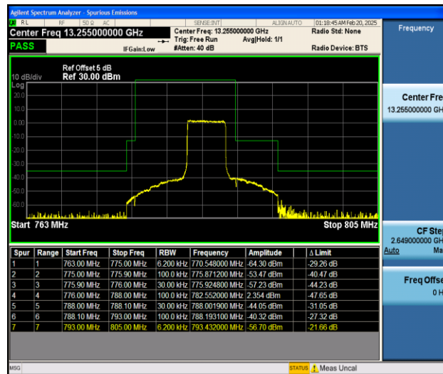
Band13_5MHz_16QAM_23255_25RB#0
