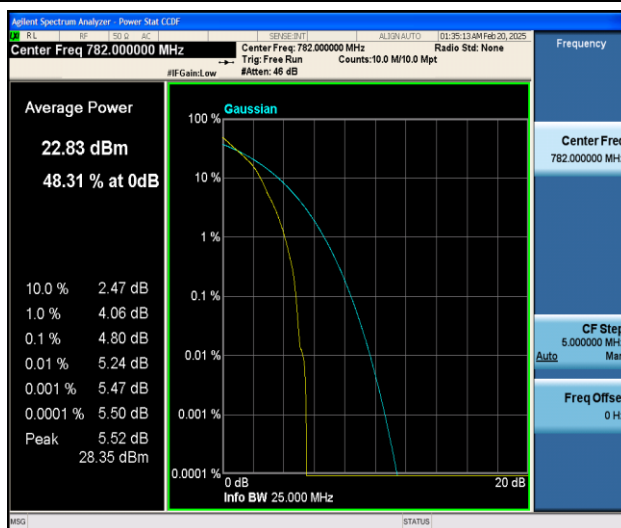
Band13-5MHz-QPSK-23230-1RB#0-PASS
