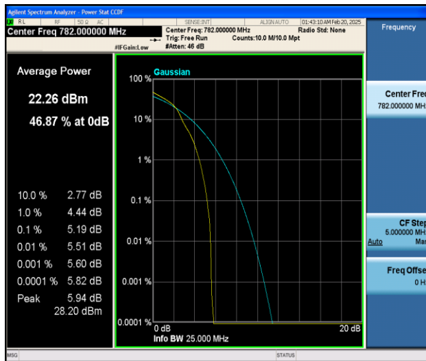
Band13-10MHz-16QAM-23230-1RB#0-PASS
