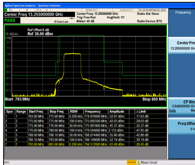
Band13_5MHz_16QAM_23205_25RB#0
