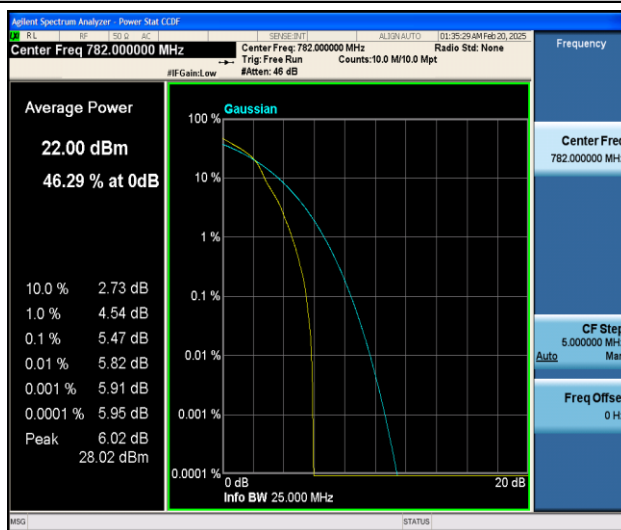
Band13-5MHz-16QAM-23230-1RB#0-PASS
