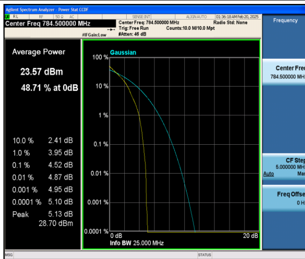
Band13-5MHz-QPSK-23255-1RB#0-PASS
