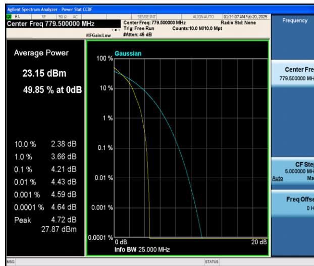
Band13-5MHz-QPSK-23205-1RB#0-PASS
