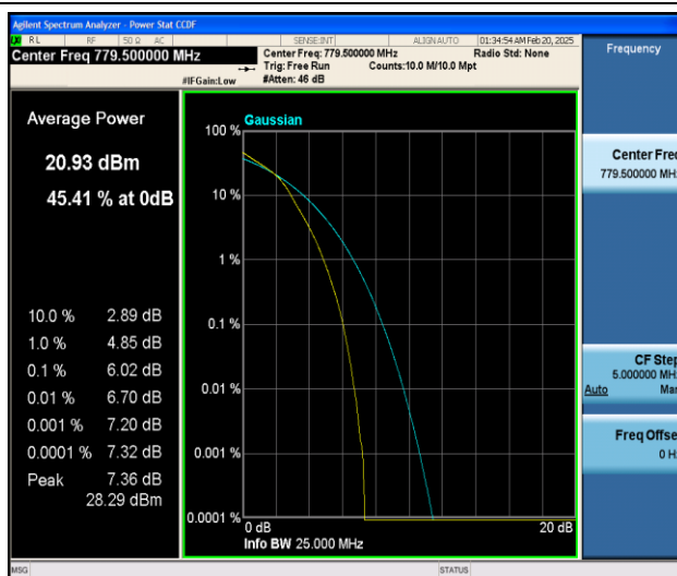
Band13-5MHz-16QAM-23205-25RB#0-PASS
