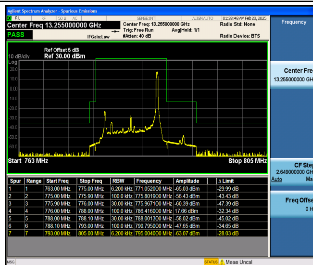
Band13_10MHz_16QAM_23230_1RB#49
