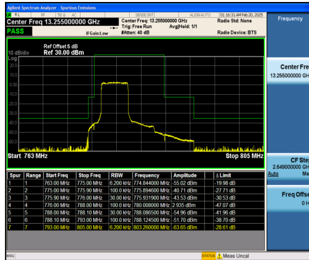
Band13_5MHz_QPSK_23205_25RB#0
