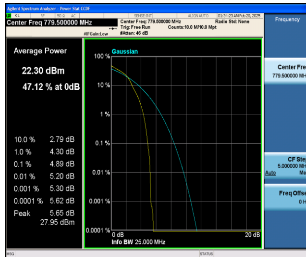
Band13-5MHz-16QAM-23205-1RB#0-PASS
