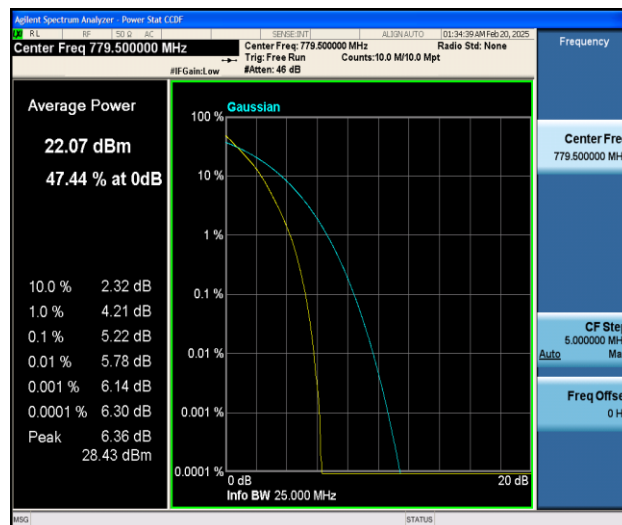
Band13-5MHz-QPSK-23205-25RB#0-PASS
