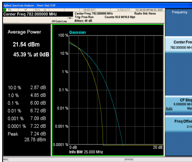
Band13-5MHz-16QAM-23230-25RB#0-PASS
