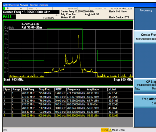
Band13_5MHz_16QAM_23255_1RB#24
