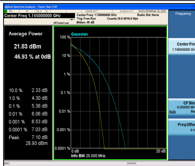
Band4-20MHz-QPSK-20300-100RB#0-PASS
