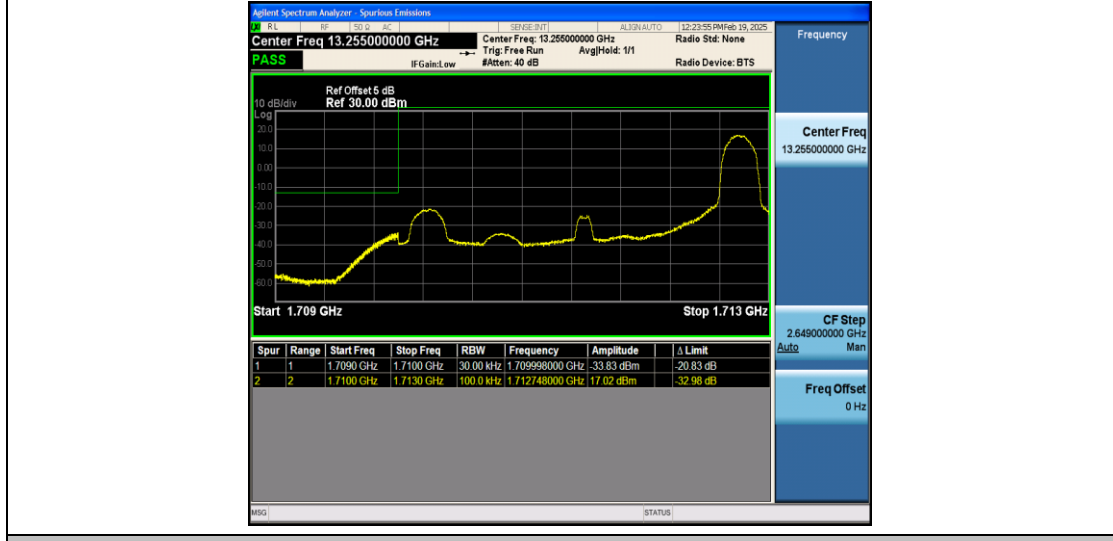
Band4_3MHz_QPSK_19965_1RB#14
