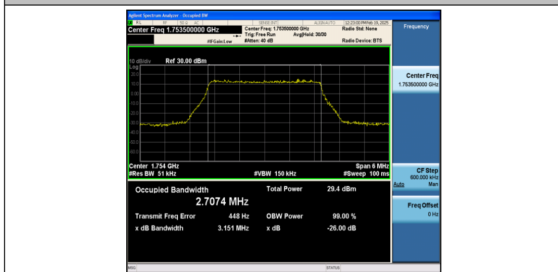
Band4-3MHz-QPSK-20385-15RB#0-PASS
