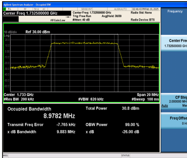
Band4-10MHz-QPSK-20175-50RB#0-PASS
