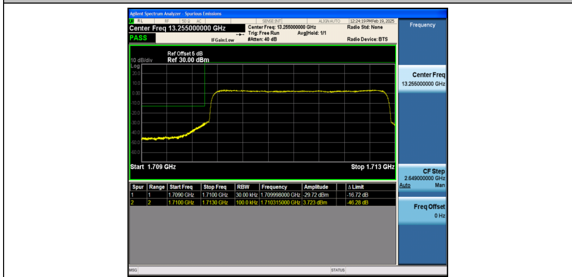
Band4_3MHz_QPSK_19965_15RB#0
