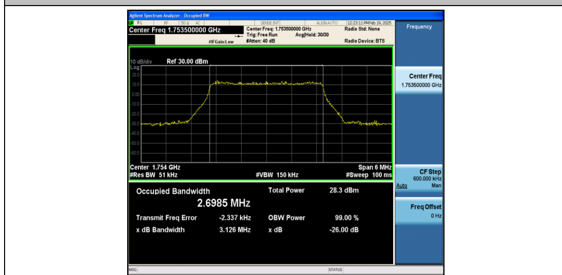
Band4-3MHz-16QAM-20385-15RB#0-PASS
