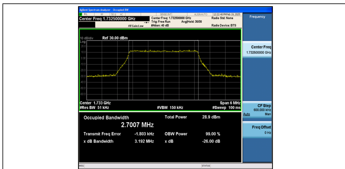
Band4-3MHz-16QAM-20175-15RB#0-PASS
