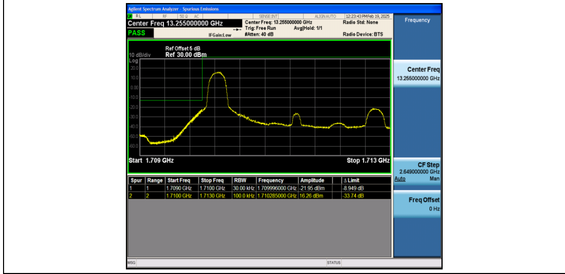
Band4_3MHz_16QAM_19965_1RB#0
