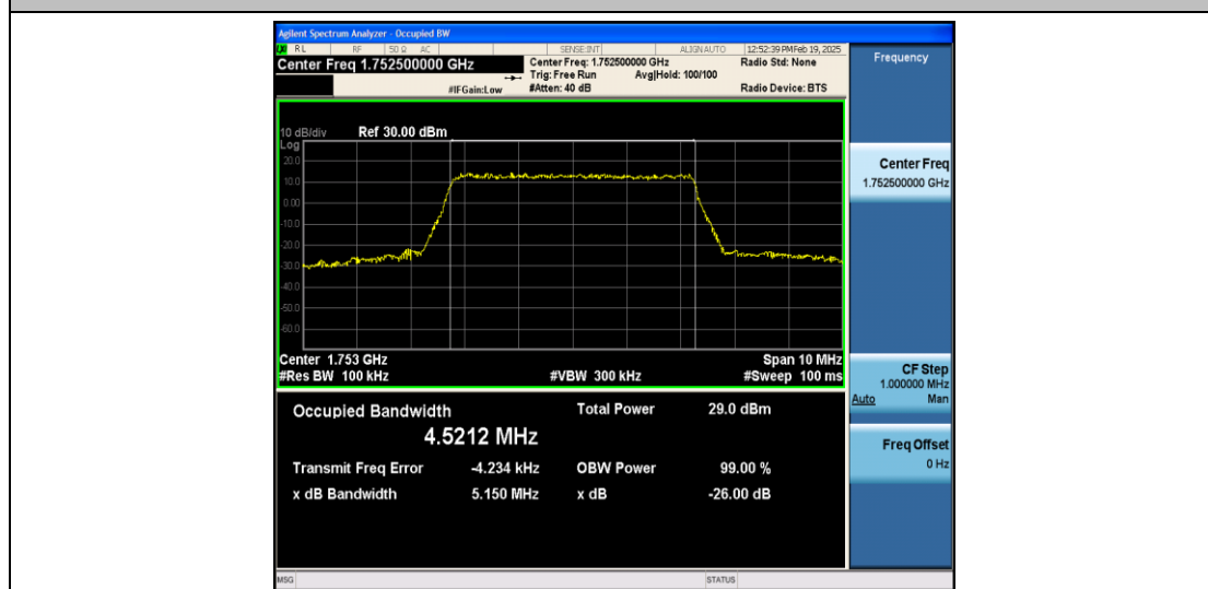
Band4-5MHz-16QAM-20375-25RB#0-PASS
