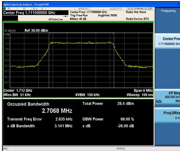
Band4-3MHz-QPSK-19965-15RB#0-PASS
