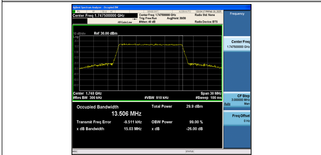
Band4-15MHz-QPSK-20325-75RB#0-PASS
