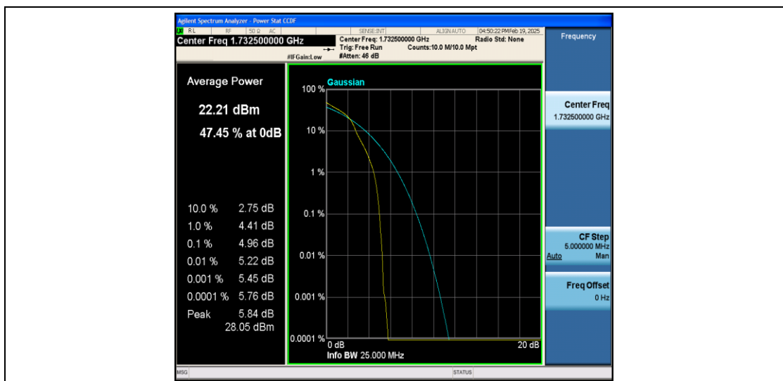
Band4-20MHz-16QAM-20175-1RB#0-PASS
