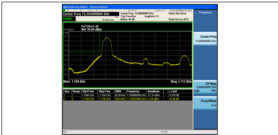
Band4_3MHz_QPSK_19965_1RB#0
