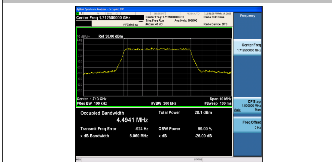
Band4-5MHz-16QAM-19975-25RB#0-PASS
