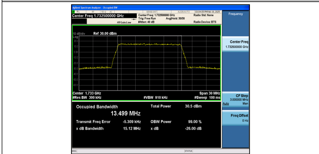
Band4-15MHz-QPSK-20175-75RB#0-PASS
