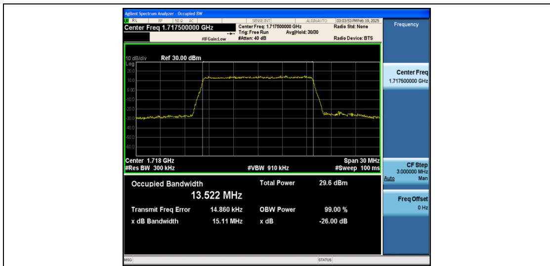
Band4-15MHz-QPSK-20025-75RB#0-PASS
