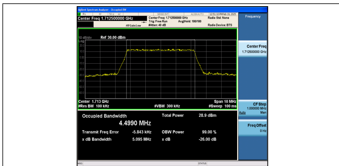
Band4-5MHz-QPSK-19975-25RB#0-PASS
