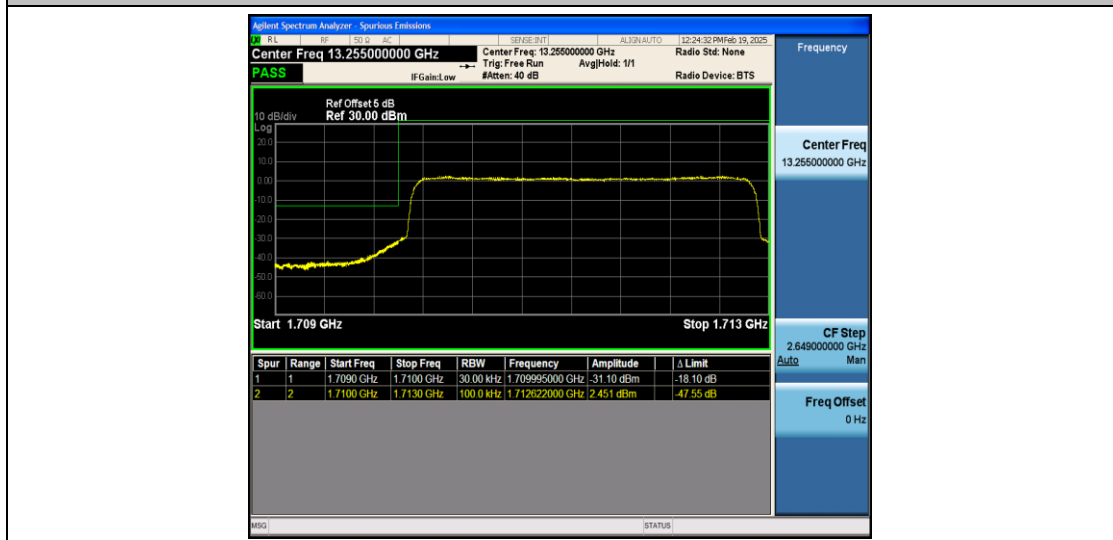
Band4_3MHz_16QAM_19965_15RB#0
