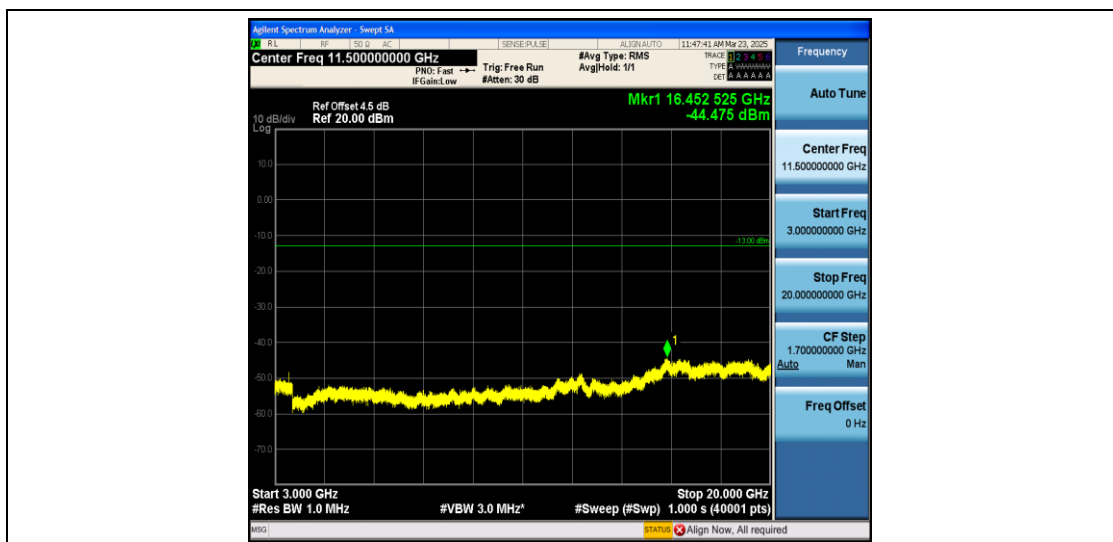
Band66_10MHz_QPSK_132322_1RB#0_3000~131022_3000~131022
