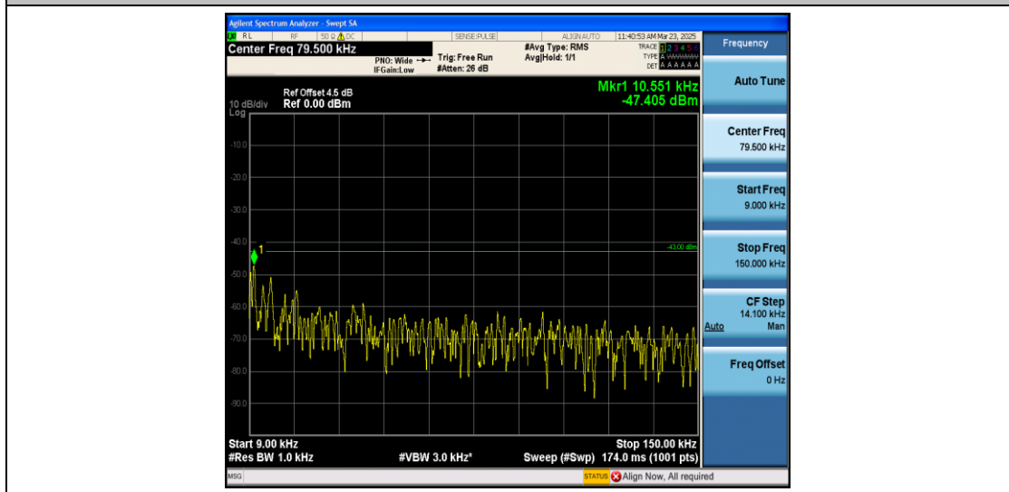
Band66_5MHz_16QAM_132322_1RB#0_0.009~0.15_0.009~0.15
