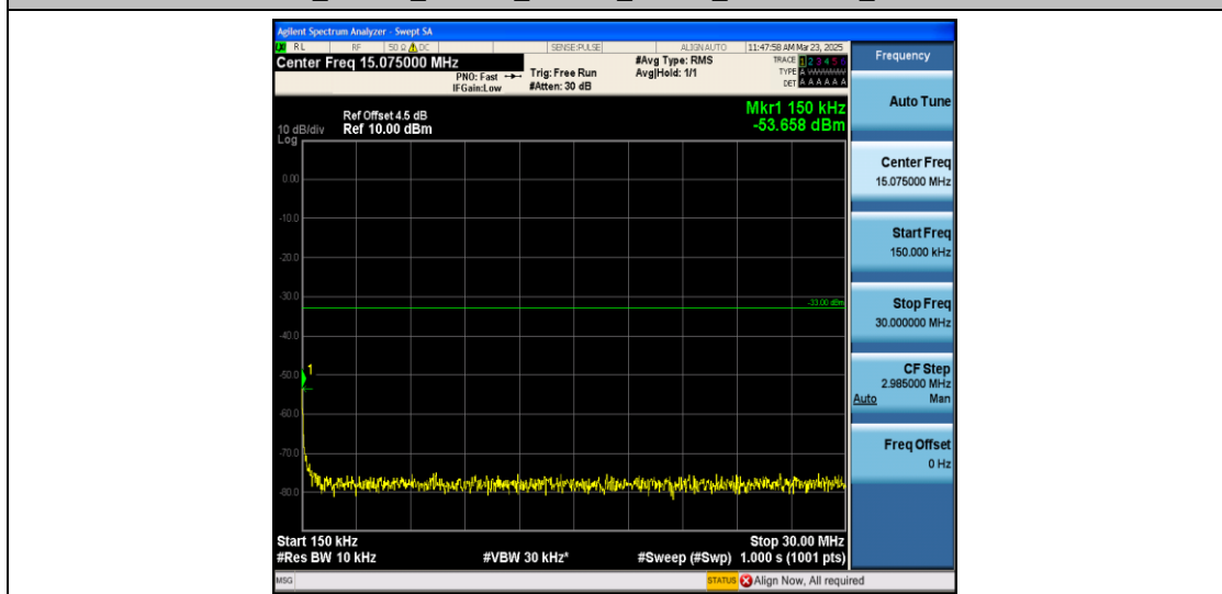
Band66_10MHz_16QAM_132322_1RB#0_0.15~30_0.15~30
