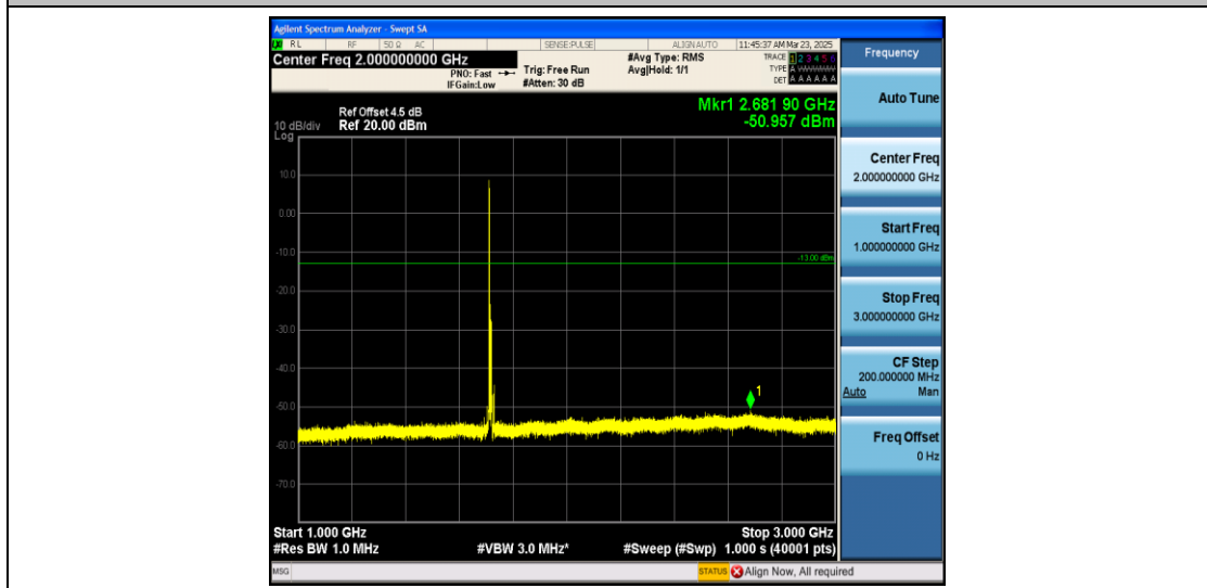
Band66_10MHz_QPSK_131022_1RB#0_1000~3000_1000~3000
