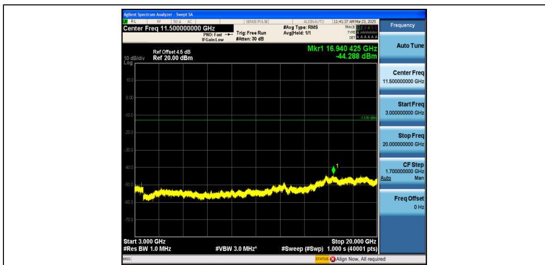
Band66_5MHz_16QAM_132322_1RB#0_3000~131022_3000~131022
