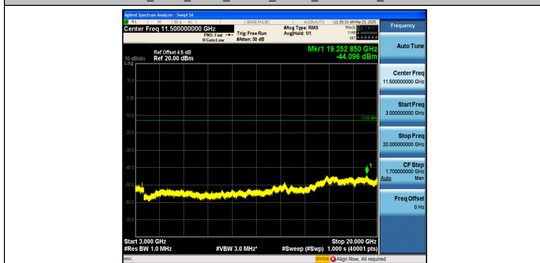
Band66_3MHz_QPSK_132322_1RB#0_3000~131022_3000~131022
