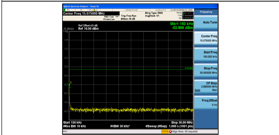
Band66_10MHz_QPSK_131022_1RB#0_0.15~30_0.15~30
