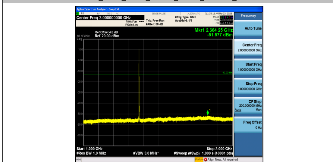
Band66_3MHz_QPSK_132322_1RB#0_1000~3000_1000~3000
