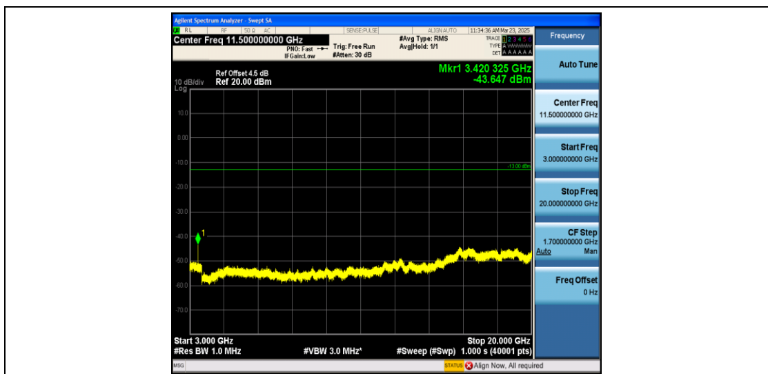
Band66_3MHz_16QAM_131987_1RB#0_3000~131022_3000~131022
