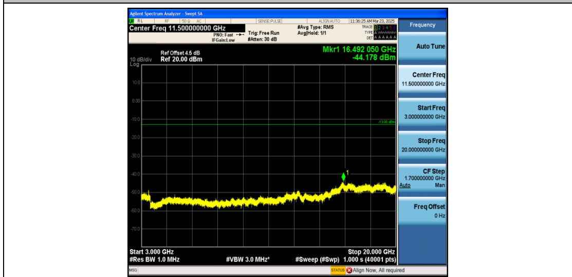
Band66_3MHz_16QAM_132322_1RB#0_3000~131022_3000~131022
