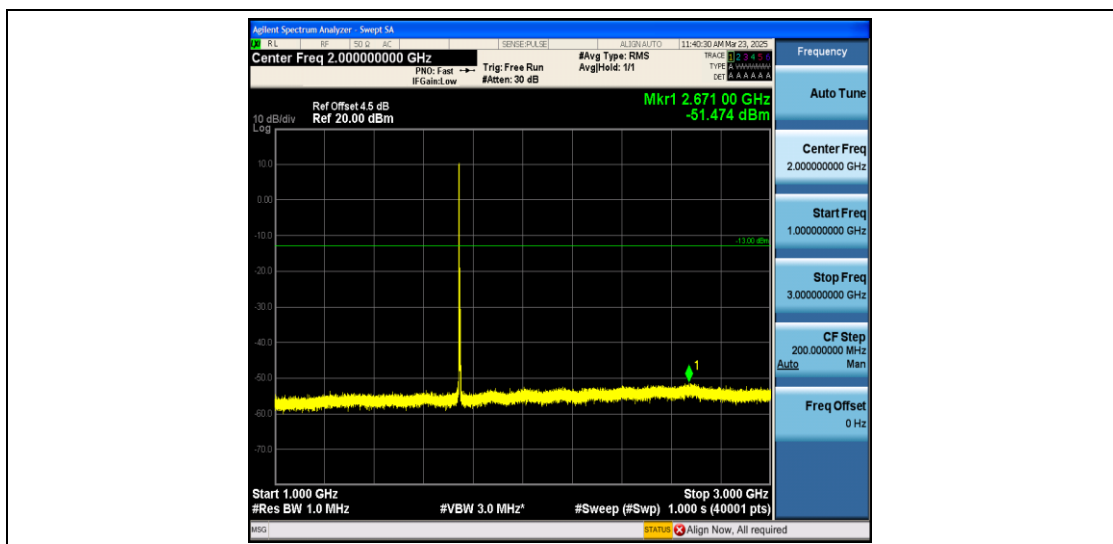
Band66_5MHz_QPSK_132322_1RB#0_1000~3000_1000~3000
