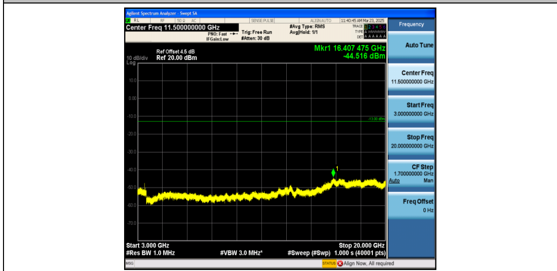
Band66_5MHz_QPSK_132322_1RB#0_3000~131022_3000~131022
