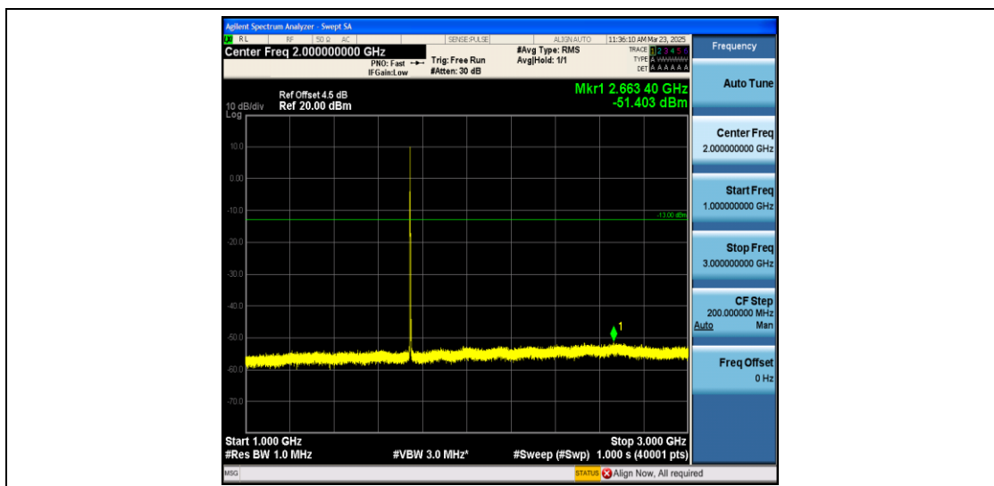
Band66_3MHz_16QAM_132322_1RB#0_1000~3000_1000~3000
