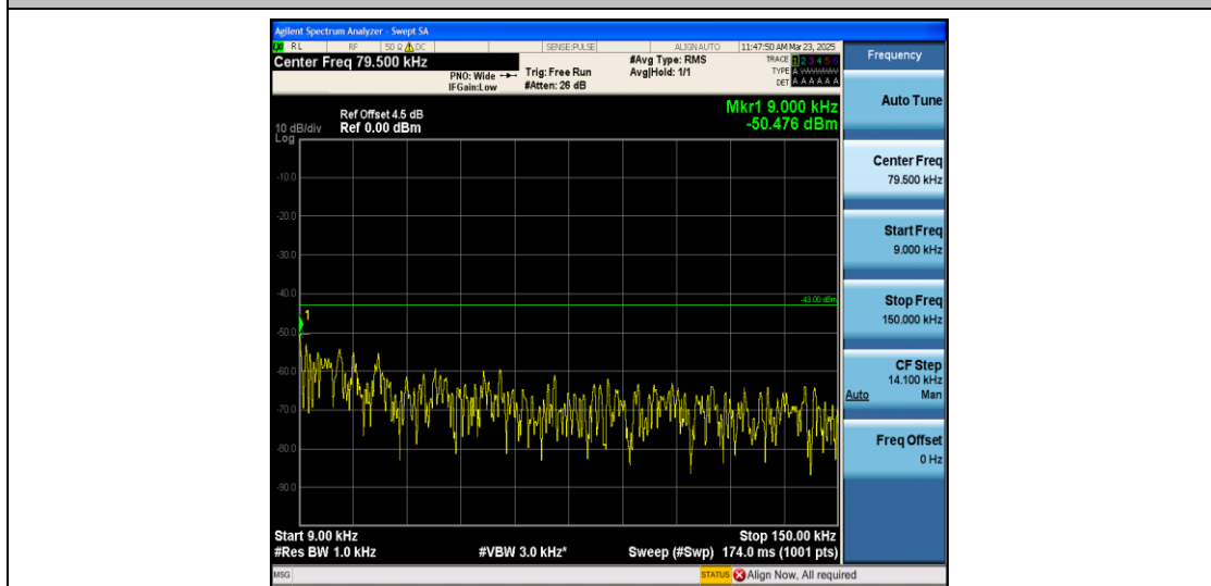
Band66_10MHz_16QAM_132322_1RB#0_0.009~0.15_0.009~0.15
