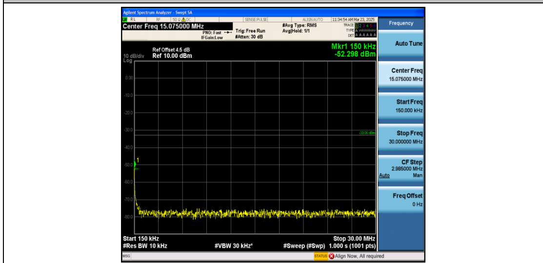
Band66_3MHz_QPSK_132322_1RB#0_0.15~30_0.15~30
