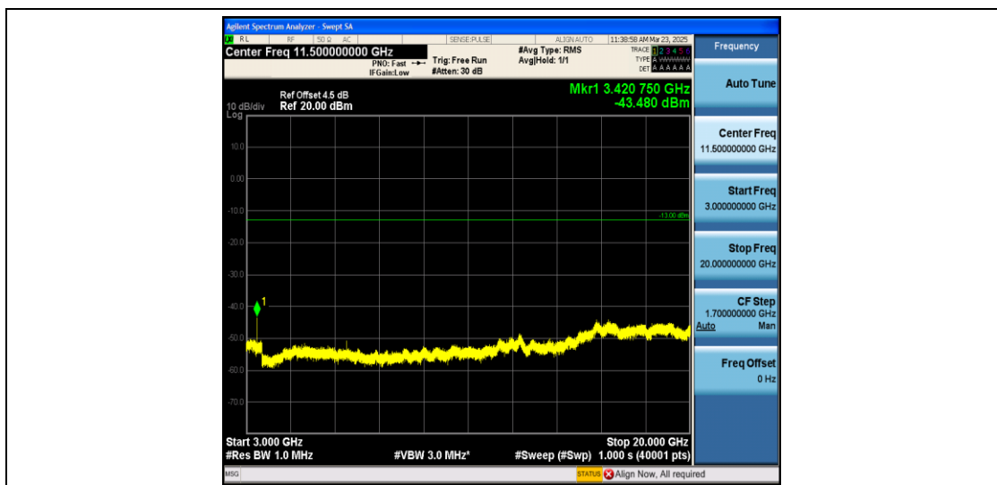
Band66_5MHz_QPSK_131997_1RB#0_3000~131022_3000~131022
