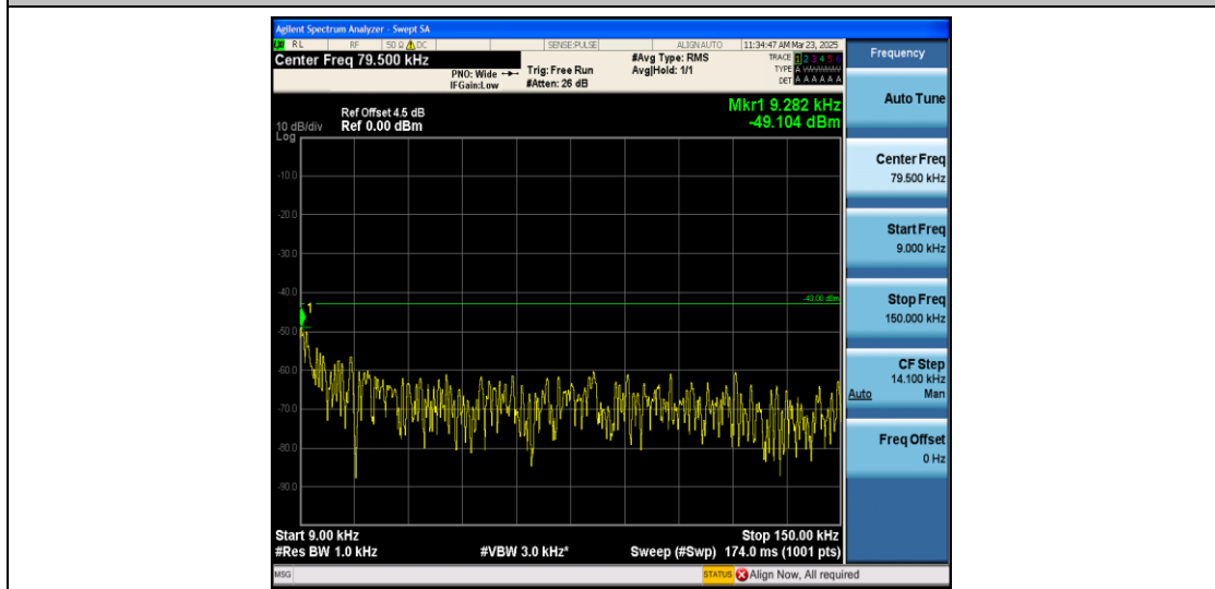
Band66_3MHz_QPSK_132322_1RB#0_0.009~0.15_0.009~0.15
