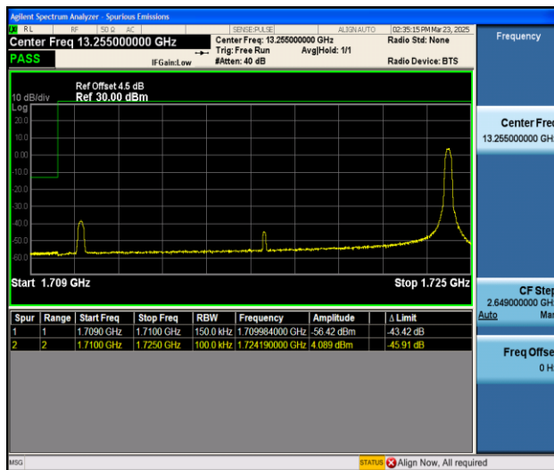
Band66_15MHz_16QAM_131047_1RB#74
