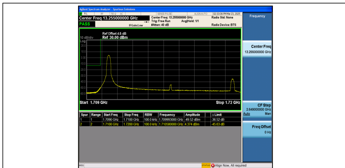
Band66_10MHz_QPSK_131022_1RB#0
