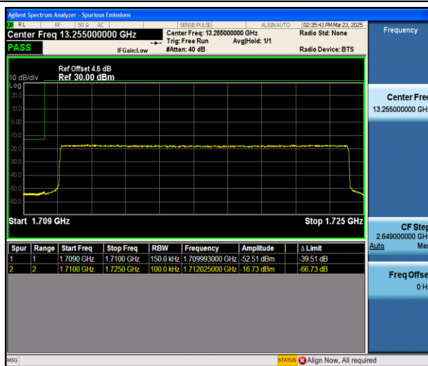
Band66_15MHz_16QAM_131047_75RB#0
