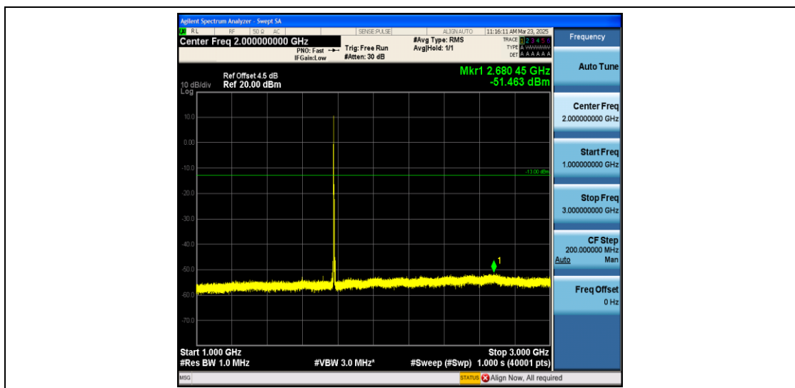
Band66_5MHz_QPSK_132647_1RB#0_1000~3000_1000~3000
