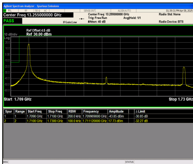
Band66_20MHz_16QAM_132072_1RB#0
