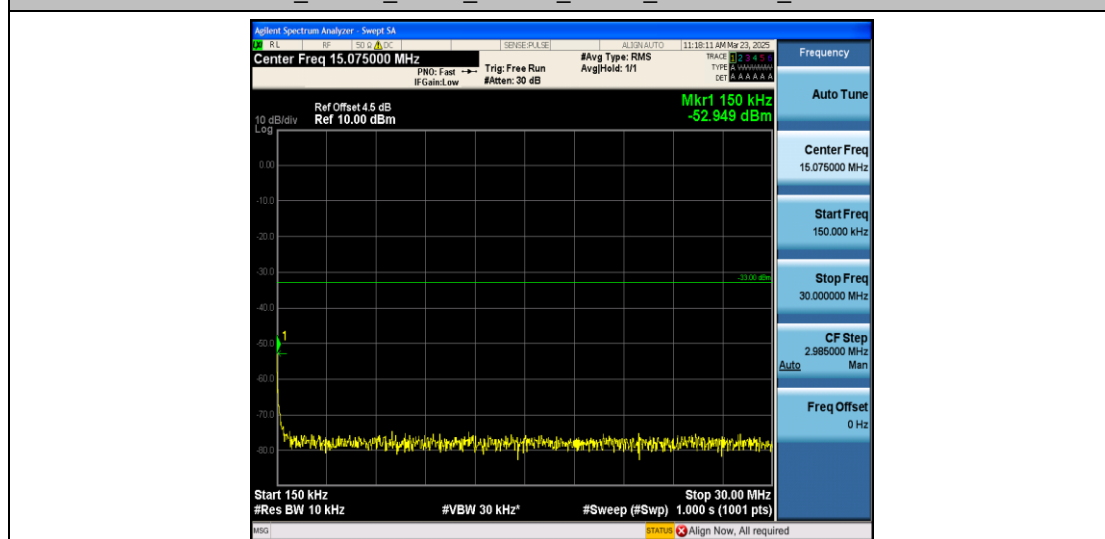
Band66_10MHz_QPSK_132622_1RB#0_0.15~30_0.15~30
