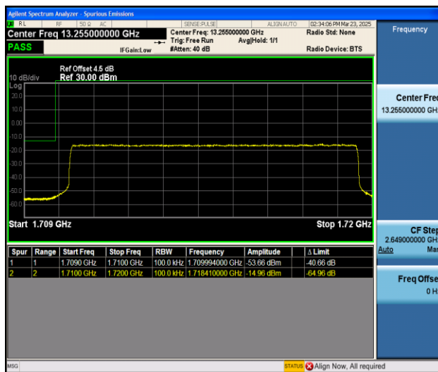
Band66_10MHz_16QAM_131022_50RB#0
