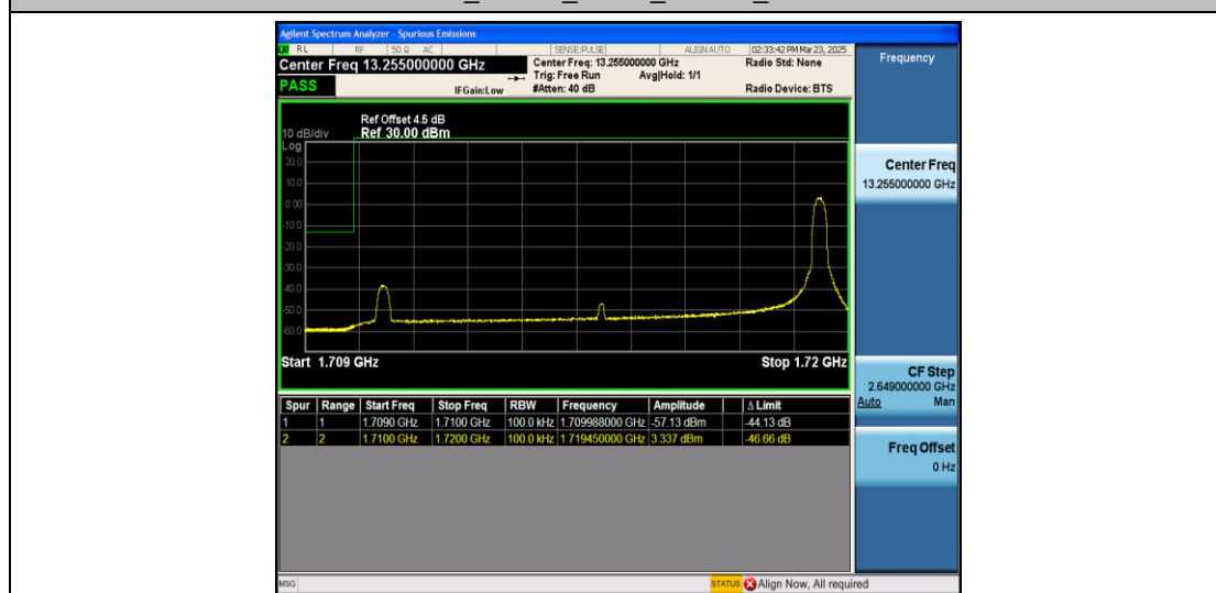
Band66_10MHz_16QAM_131022_1RB#49
