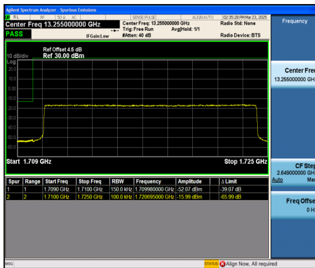
Band66_15MHz_QPSK_131047_75RB#0
