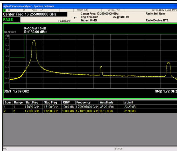
Band66_10MHz_16QAM_131022_1RB#0
