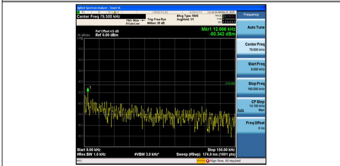
Band66_5MHz_16QAM_132647_1RB#0_0.009~0.15_0.009~0.15
