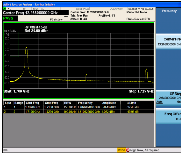
Band66_15MHz_QPSK_131047_1RB#0
