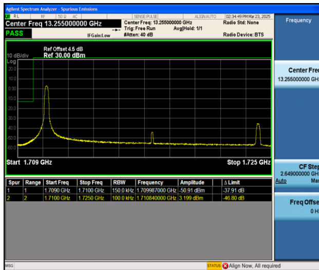
Band66_15MHz_16QAM_131047_1RB#0
