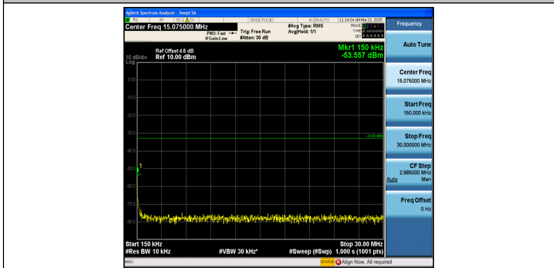
Band66_3MHz_16QAM_132657_1RB#0_0.15~30_0.15~30
