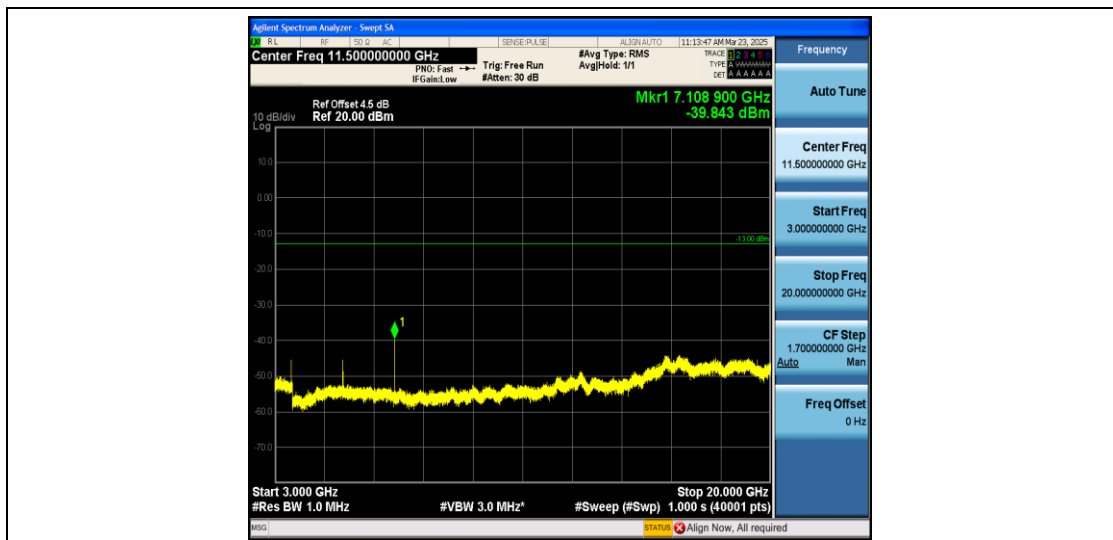
Band66_3MHz_QPSK_132657_1RB#0_3000~131022_3000~131022
