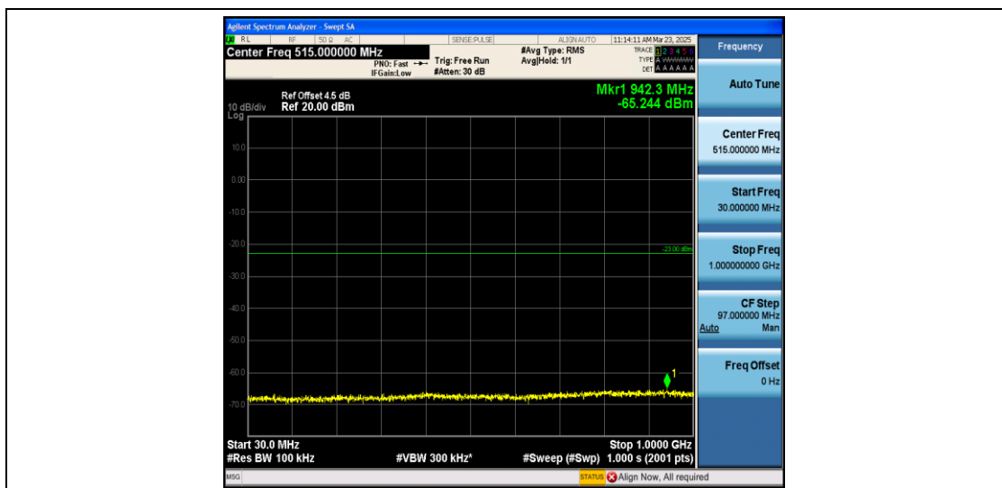
Band66_3MHz_16QAM_132657_1RB#0_30~1000_30~1000
