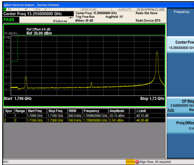
Band66_20MHz_16QAM_132072_1RB#99
