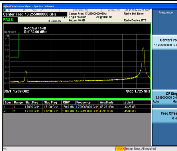
Band66_15MHz_QPSK_131047_1RB#74
