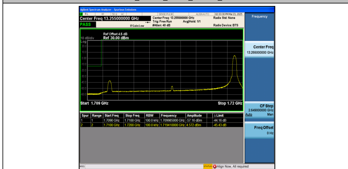
Band66_10MHz_QPSK_131022_1RB#49
