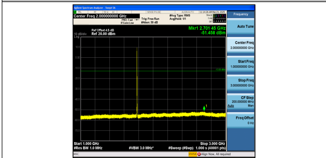
Band66_3MHz_16QAM_132657_1RB#0_1000~3000_1000~3000
