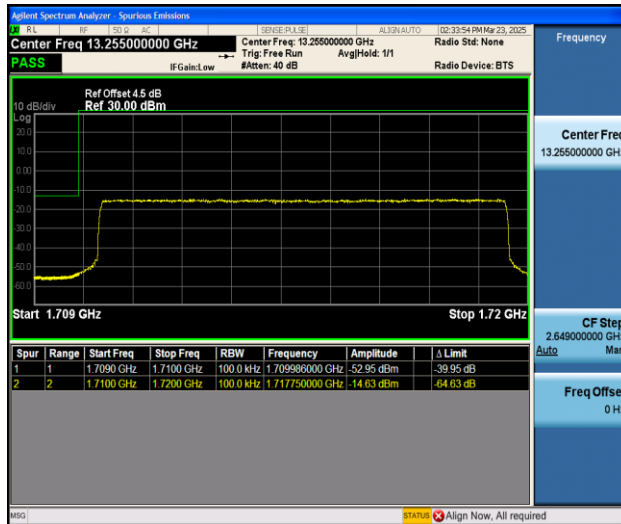
Band66_10MHz_QPSK_131022_50RB#0
