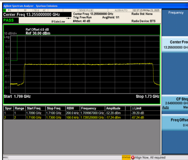
Band66_20MHz_16QAM_132072_100RB#0
