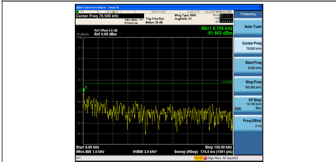
Band66_3MHz_16QAM_132657_1RB#0_0.009~0.15_0.009~0.15
