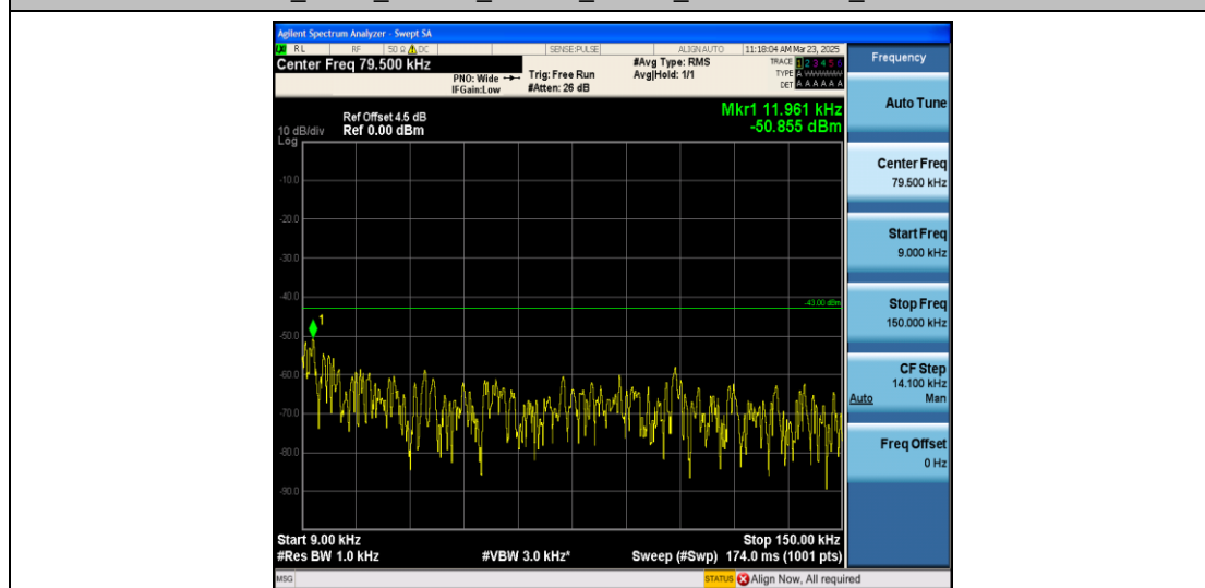
Band66_10MHz_QPSK_132622_1RB#0_0.009~0.15_0.009~0.15
