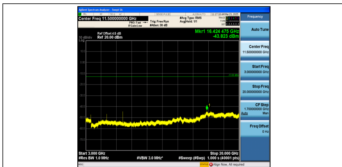
Band66_5MHz_16QAM_132647_1RB#0_3000~131022_3000~131022
