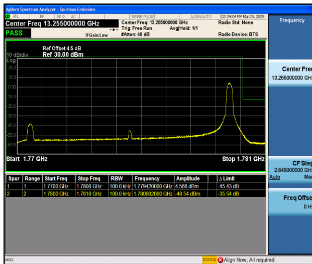
Band66_10MHz_16QAM_132622_1RB#49
