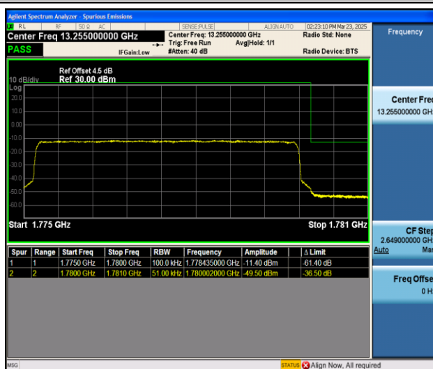
Band66_5MHz_16QAM_132647_25RB#0
