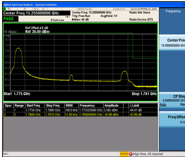
Band66_5MHz_QPSK_132647_1RB#0
