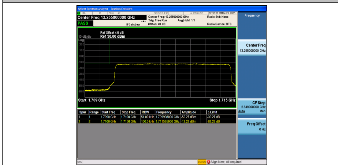
Band66_5MHz_16QAM_131997_25RB#0
