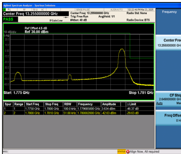
Band66_5MHz_16QAM_132647_1RB#24
