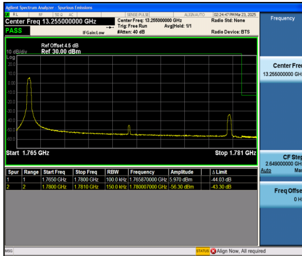
Band66_15MHz_QPSK_132597_1RB#0
