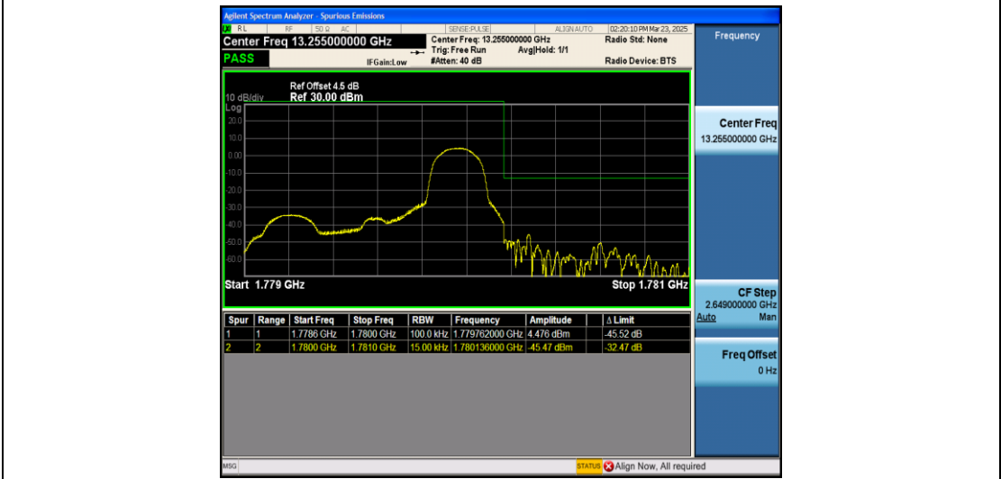
Band66_1.4MHz_16QAM_132665_1RB#5
