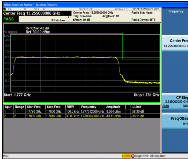
Band66_3MHz_QPSK_132657_15RB#0
