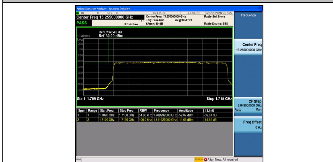
Band66_5MHz_QPSK_131997_25RB#0
