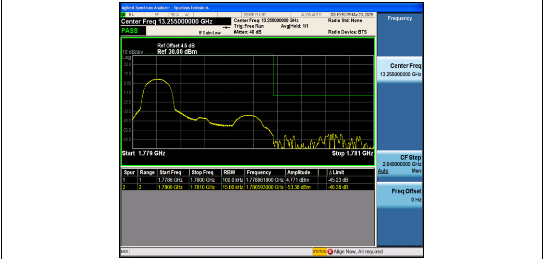
Band66_1.4MHz_16QAM_132665_1RB#0
