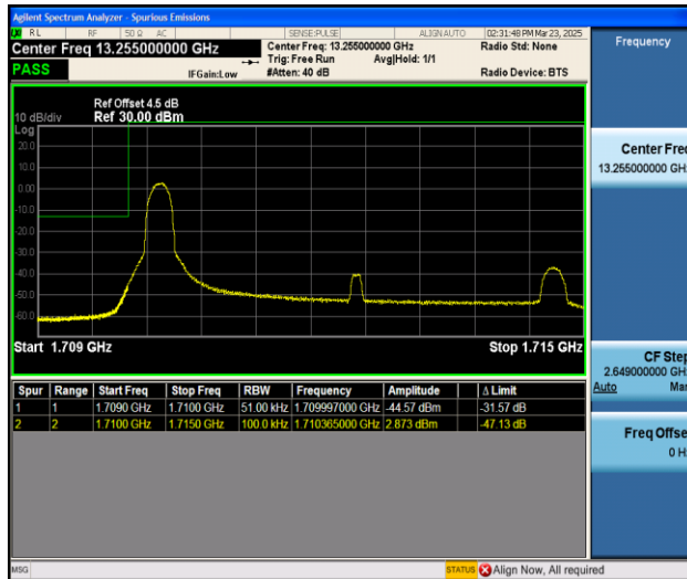
Band66_5MHz_16QAM_131997_1RB#0
