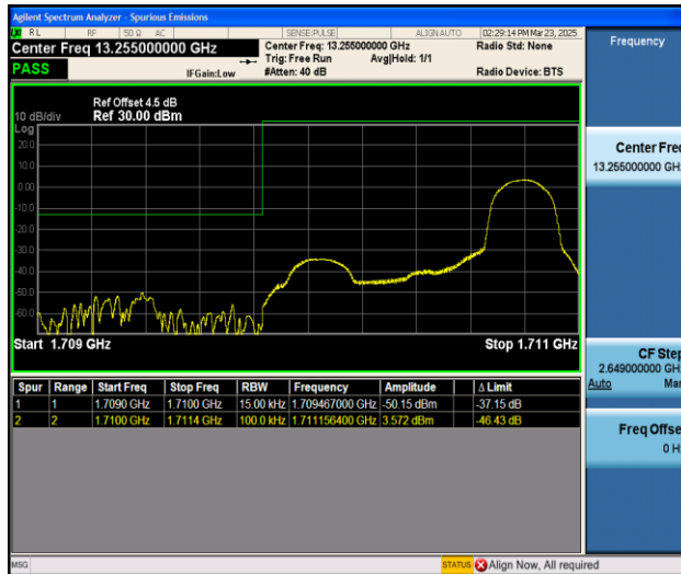
Band66_1.4MHz_16QAM_131979_1RB#5
