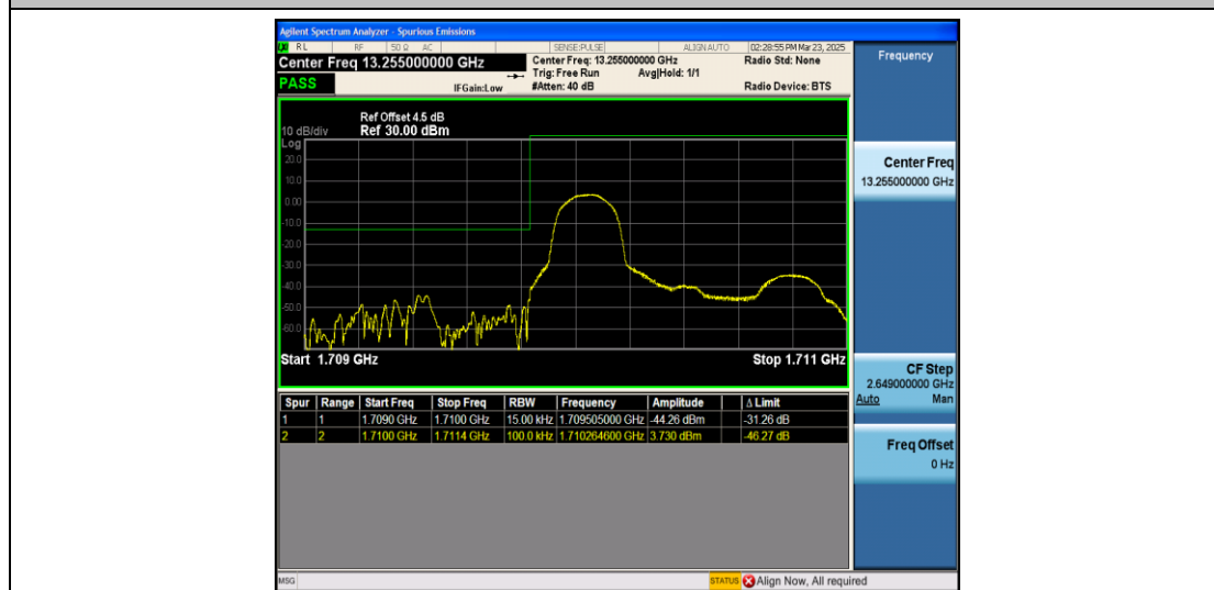
Band66_1.4MHz_16QAM_131979_1RB#0
