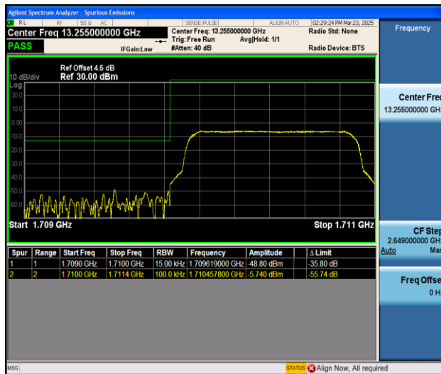
Band66_1.4MHz_QPSK_131979_6RB#0
