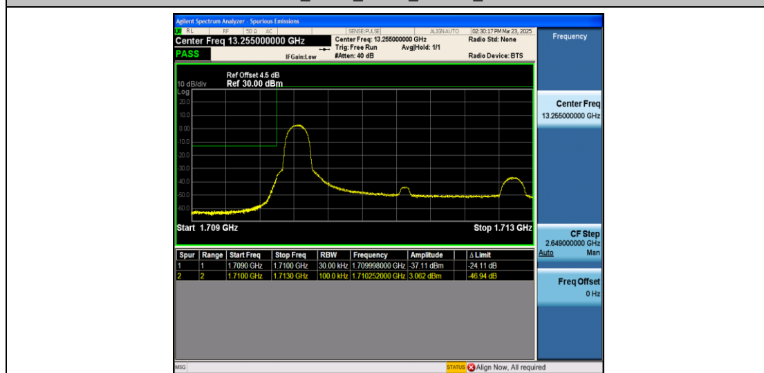
Band66_3MHz_16QAM_131987_1RB#0
