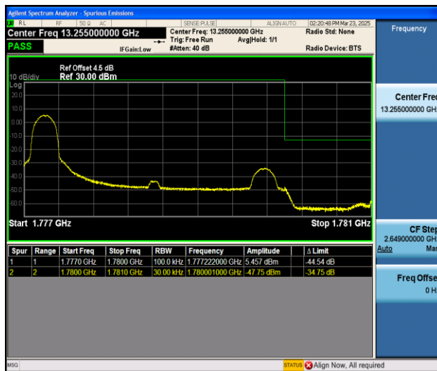
Band66_3MHz_QPSK_132657_1RB#0
