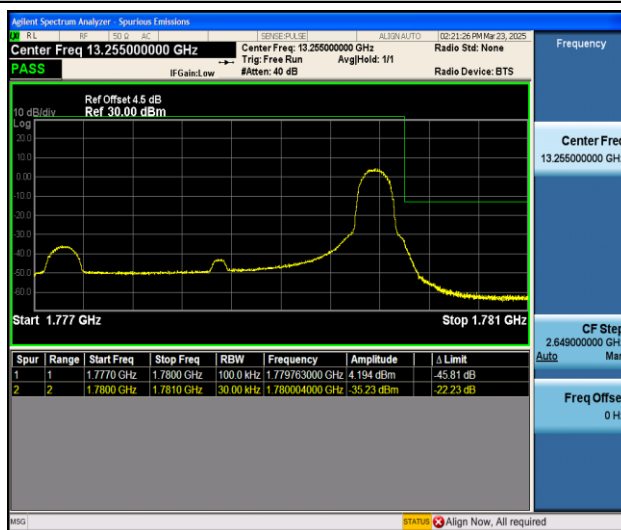
Band66_3MHz_16QAM_132657_1RB#14
