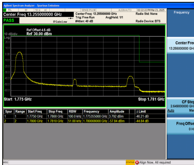
Band66_5MHz_16QAM_132647_1RB#0
