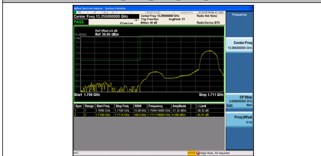
Band66_1.4MHz_QPSK_131979_1RB#5
