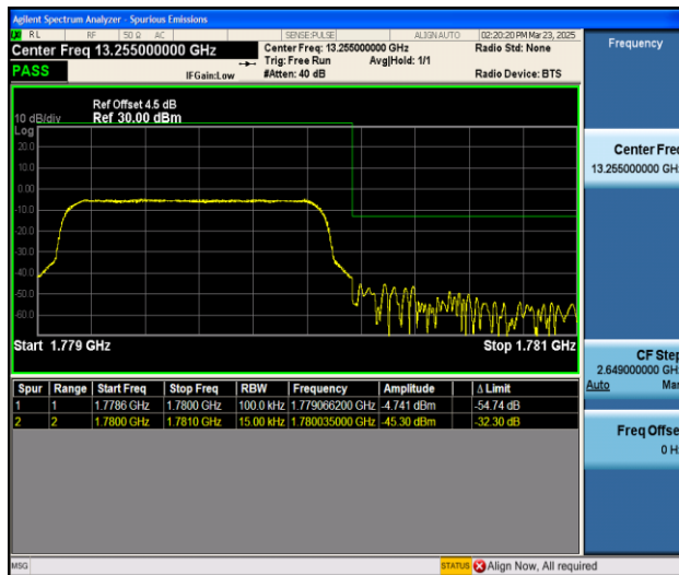
Band66_1.4MHz_QPSK_132665_6RB#0
