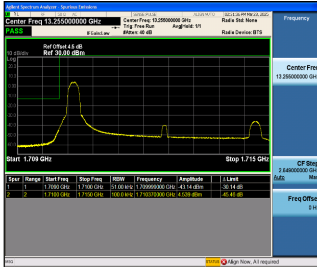
Band66_5MHz_QPSK_131997_1RB#0
