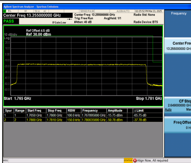
Band66_15MHz_16QAM_132597_75RB#0
