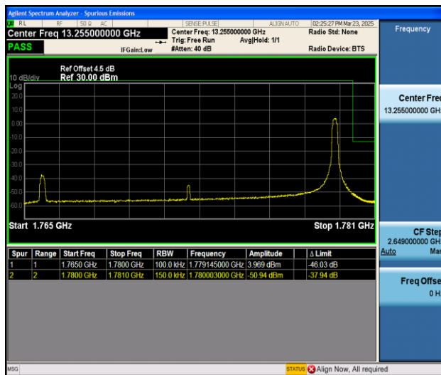
Band66_15MHz_16QAM_132597_1RB#74
