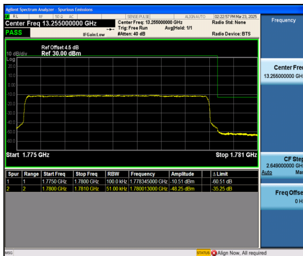
Band66_5MHz_QPSK_132647_25RB#0
