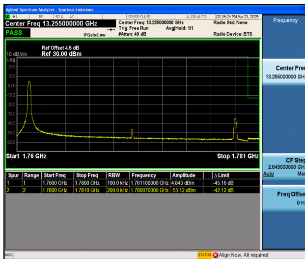
Band66_20MHz_16QAM_132572_1RB#0
