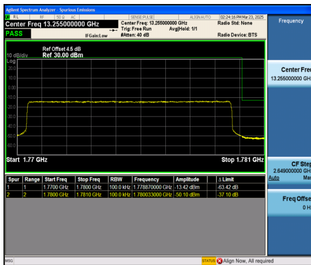
Band66_10MHz_QPSK_132622_50RB#0
