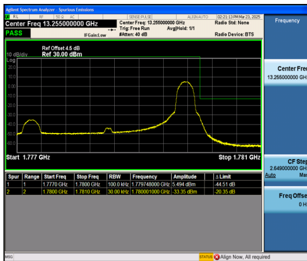
Band66_3MHz_QPSK_132657_1RB#14
