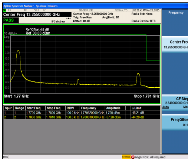
Band66_10MHz_16QAM_132622_1RB#0
