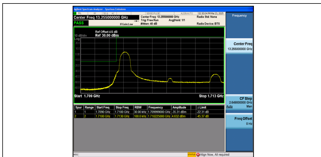
Band66_3MHz_QPSK_131987_1RB#0
