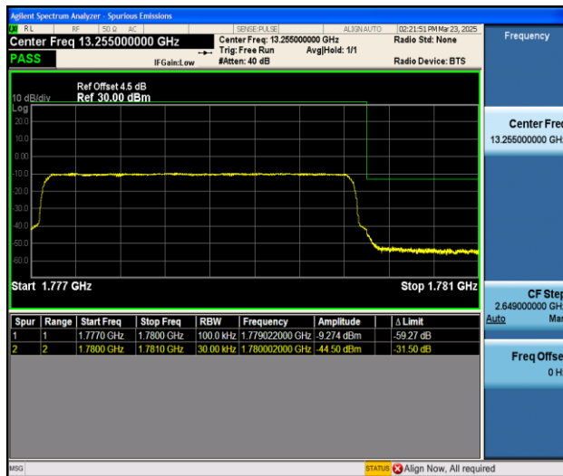
Band66_3MHz_16QAM_132657_15RB#0
