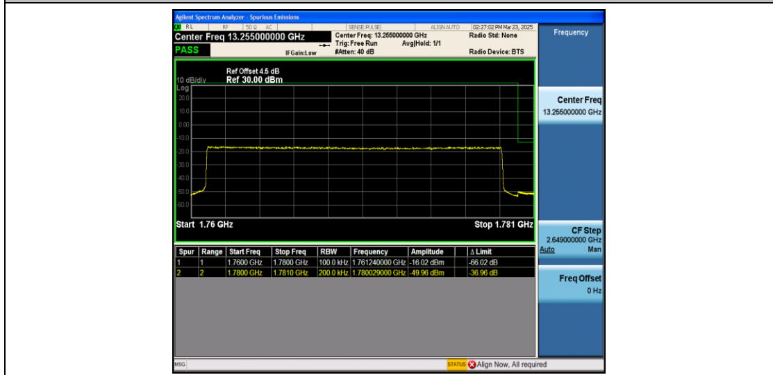
Band66_20MHz_QPSK_132572_100RB#0
