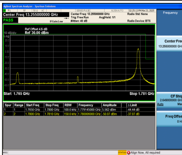
Band66_15MHz_QPSK_132597_1RB#74
