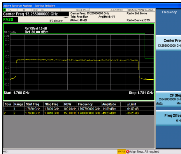
Band66_15MHz_QPSK_132597_75RB#0
