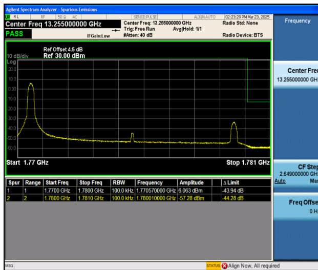
Band66_10MHz_QPSK_132622_1RB#0
