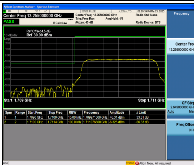
Band66_1.4MHz_16QAM_131979_6RB#0
