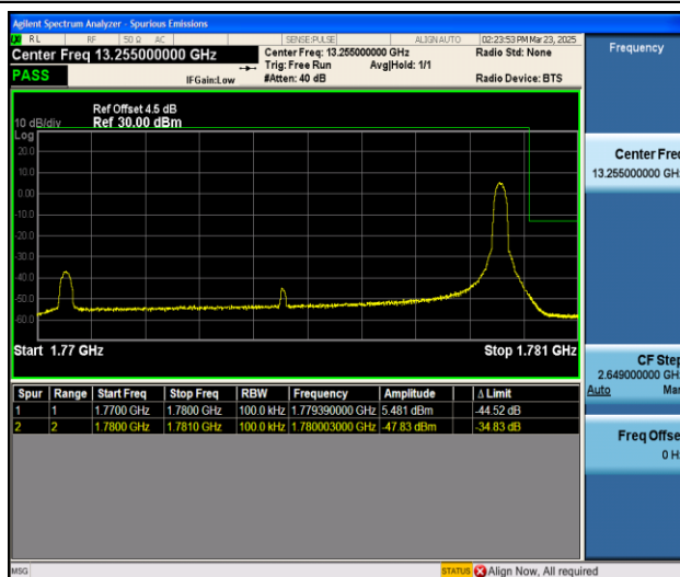
Band66_10MHz_QPSK_132622_1RB#49
