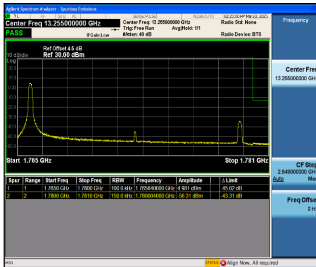
Band66_15MHz_16QAM_132597_1RB#0
