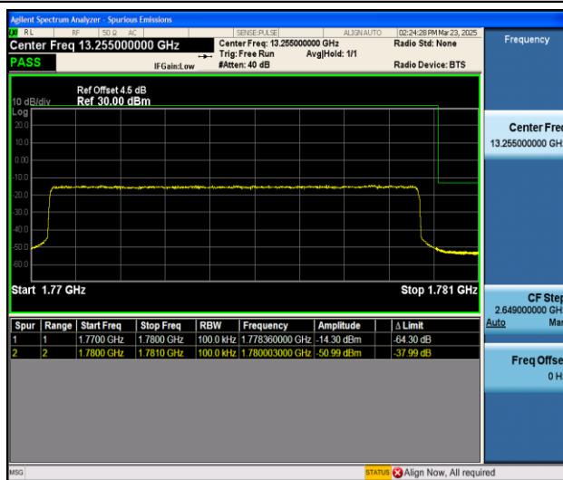
Band66_10MHz_16QAM_132622_50RB#0
