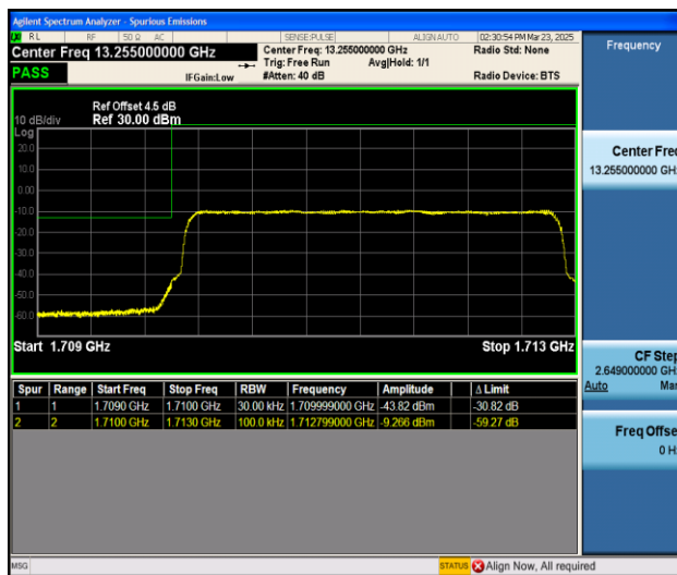
Band66_3MHz_QPSK_131987_15RB#0
