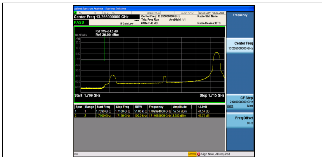
Band66_5MHz_16QAM_131997_1RB#24
