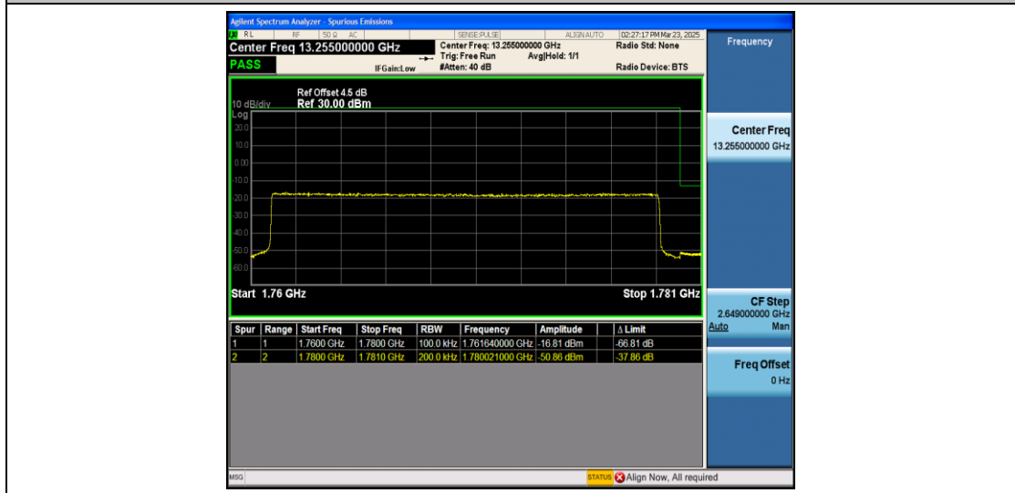
Band66_20MHz_16QAM_132572_100RB#0
