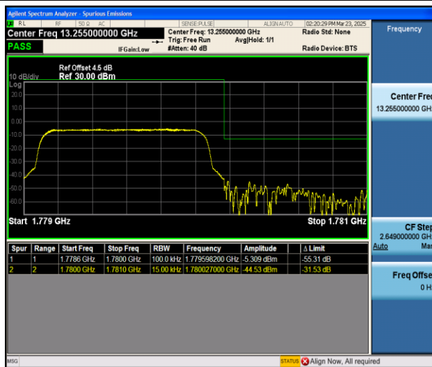
Band66_1.4MHz_16QAM_132665_6RB#0
