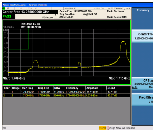
Band66_5MHz_QPSK_131997_1RB#24
