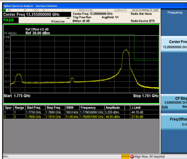
Band66_5MHz_QPSK_132647_1RB#24
