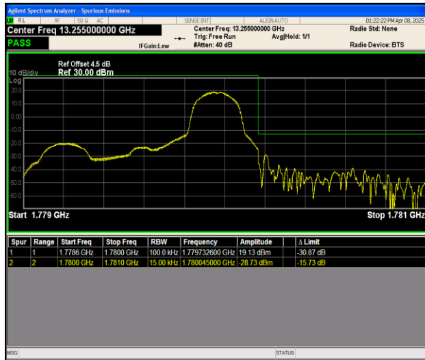
Band66_1.4MHz_QPSK_132665_1RB#5
