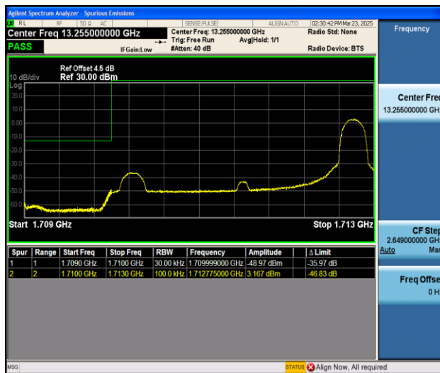
Band66_3MHz_16QAM_131987_1RB#14
