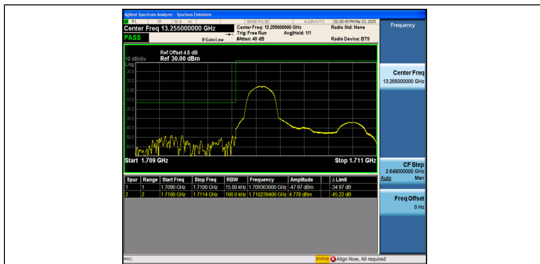
Band66_1.4MHz_QPSK_131979_1RB#0
