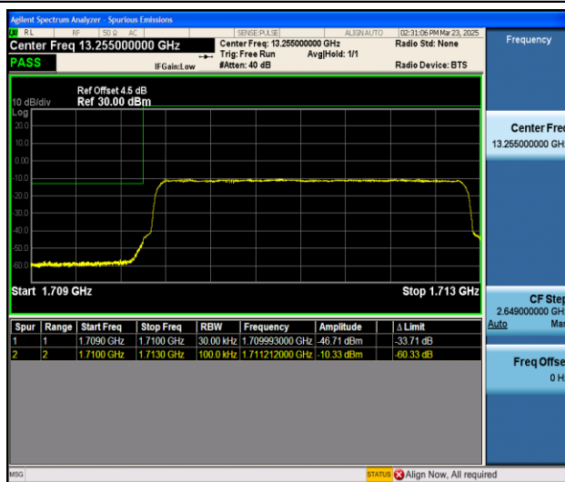
Band66_3MHz_16QAM_131987_15RB#0
