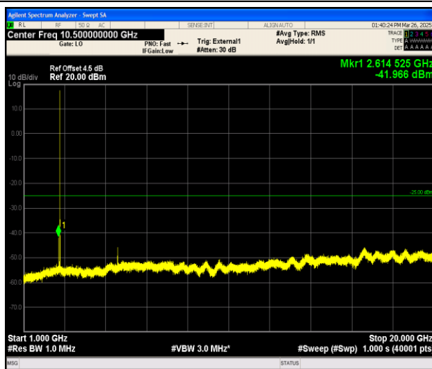
Band41_15MHz_QPSK_41515_1RB#0_1000~20000_1000~20000
