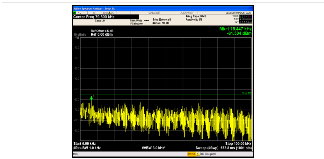
Band41_15MHz_16QAM_40620_1RB#0_0.009~0.15_0.009~0.15
