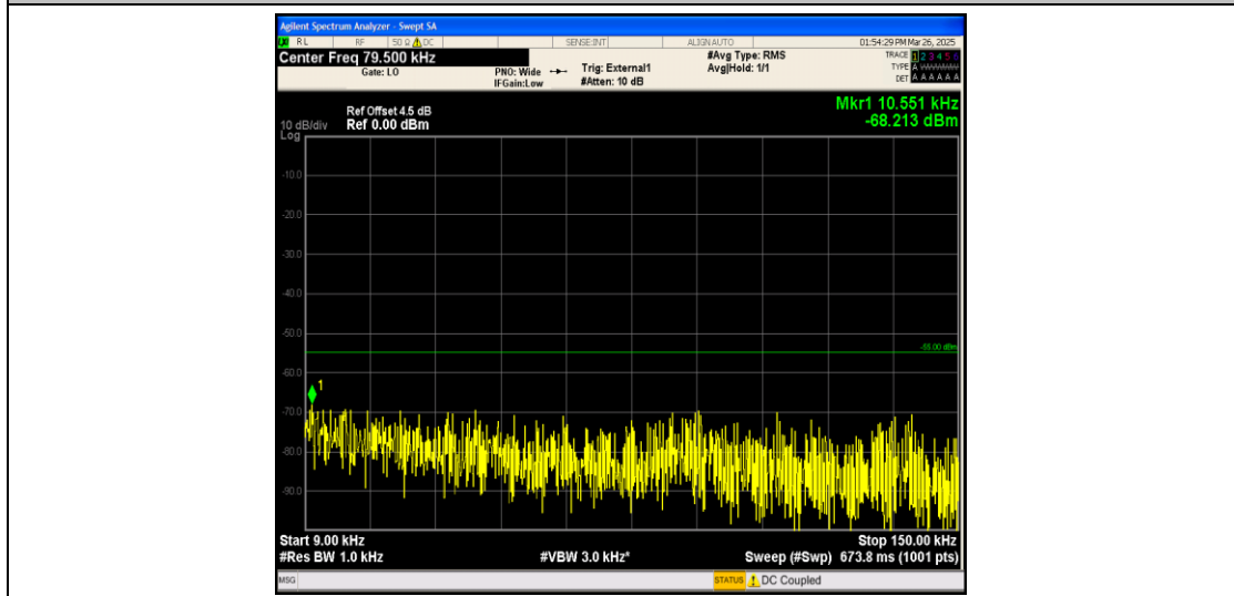
Band41_20MHz_16QAM_39750_1RB#0_0.009~0.15_0.009~0.15
