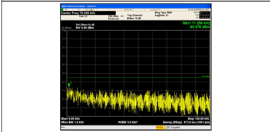
Band41_10MHz_16QAM_39700_1RB#0_0.009~0.15_0.009~0.15
