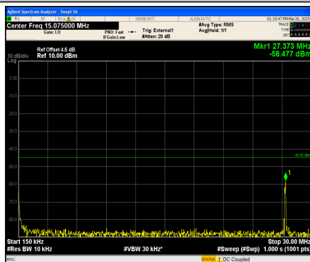
Band41_10MHz_QPSK_40620_1RB#0_0.15~30_0.15~30
