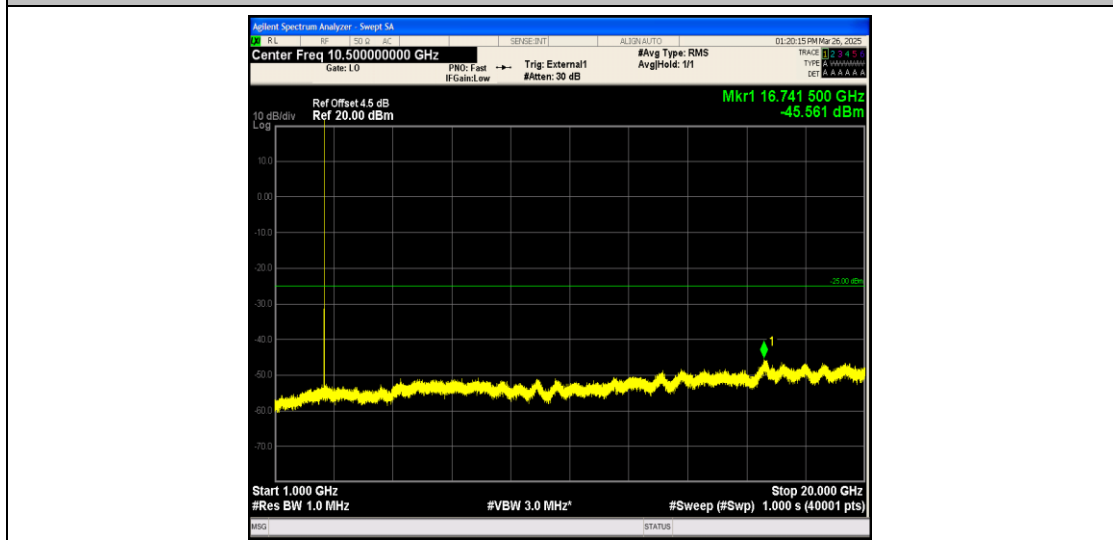
Band41_10MHz_QPSK_40620_1RB#0_1000~20000_1000~20000
