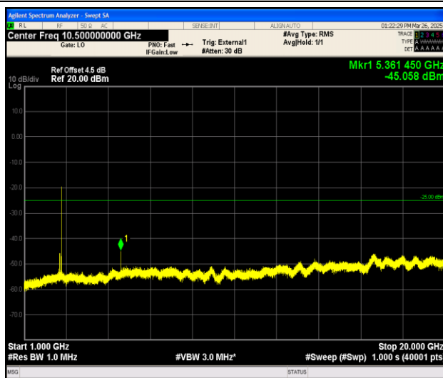
Band41_10MHz_QPSK_41540_1RB#0_1000~20000_1000~20000
