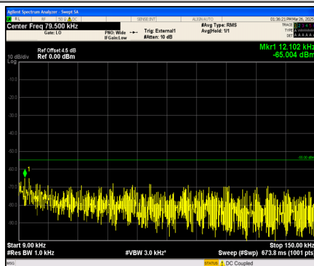
Band41_15MHz_16QAM_39725_1RB#0_0.009~0.15_0.009~0.15
