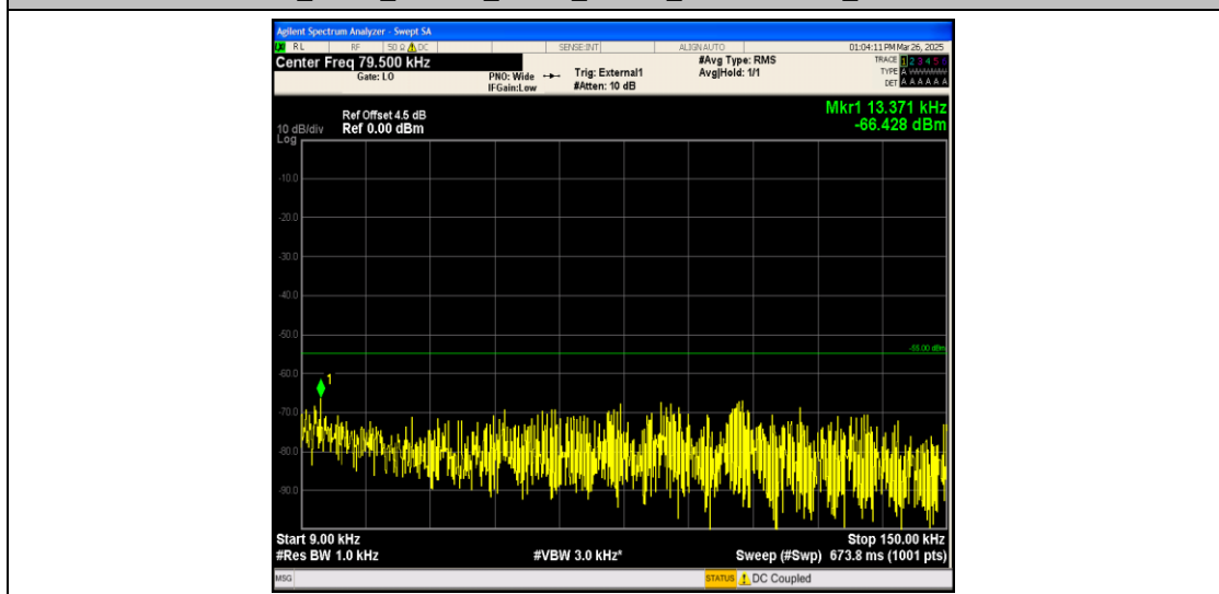
Band41_5MHz_QPSK_41565_1RB#0_0.009~0.15_0.009~0.15
