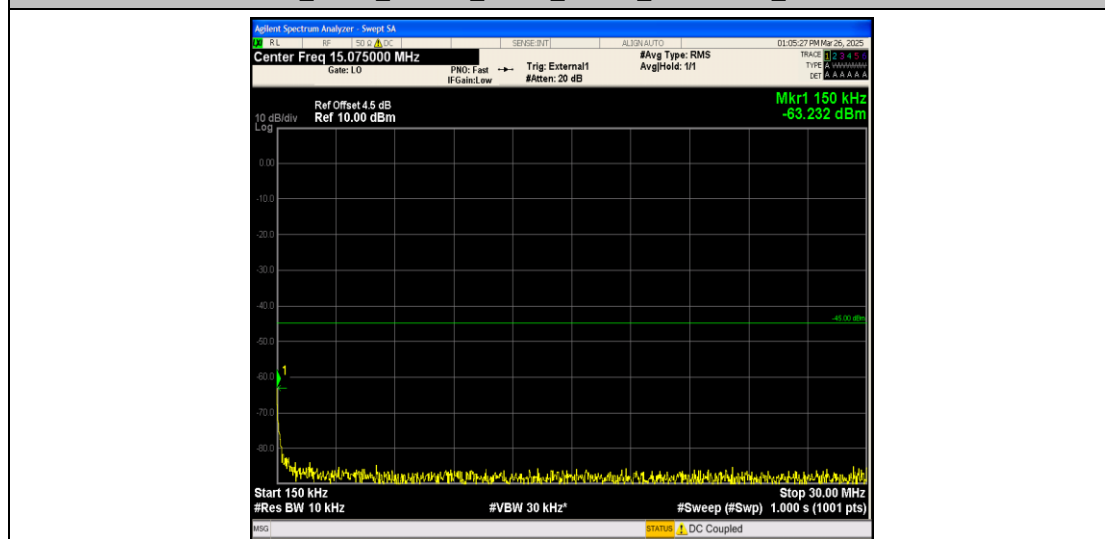
Band41_5MHz_16QAM_41565_1RB#0_0.15~30_0.15~30
