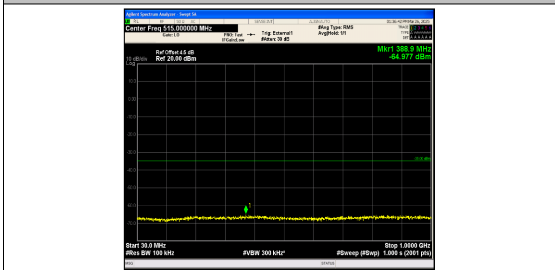
Band41_15MHz_16QAM_39725_1RB#0_30~1000_30~1000
