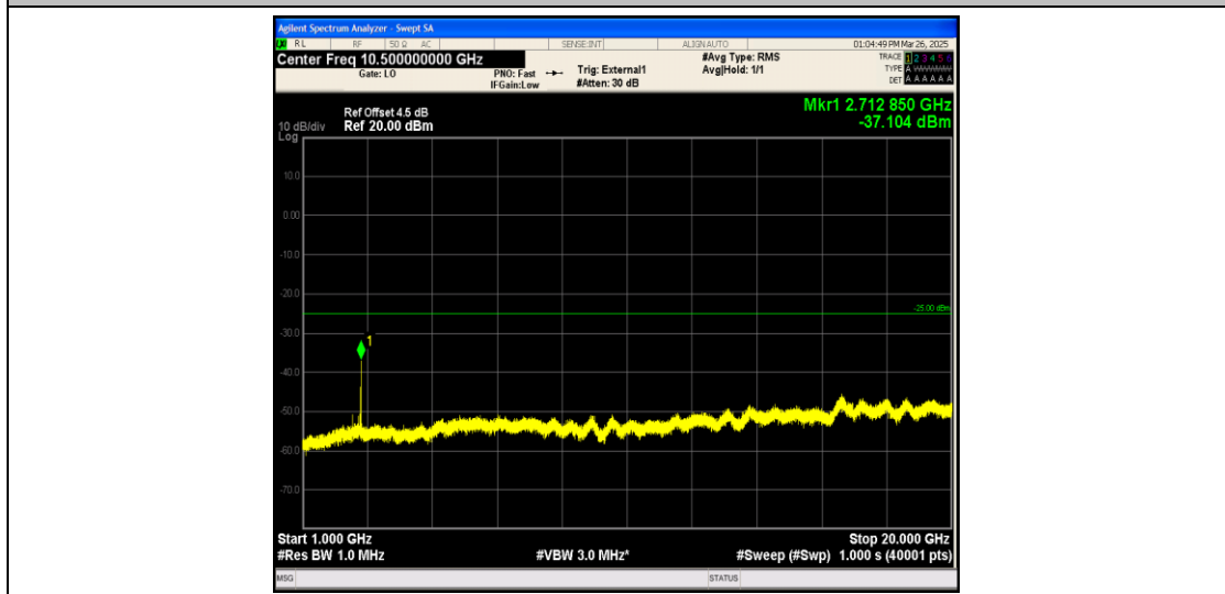
Band41_5MHz_QPSK_41565_1RB#0_1000~20000_1000~20000
