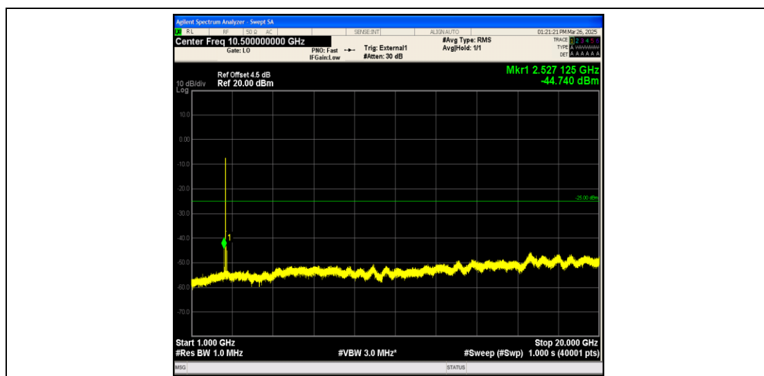
Band41_10MHz_16QAM_40620_1RB#0_1000~20000_1000~20000
