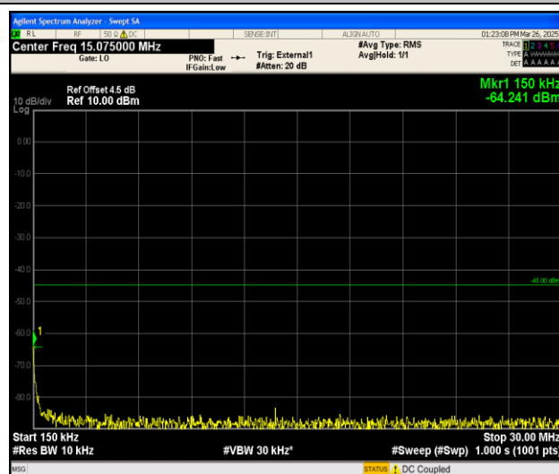
Band41_10MHz_16QAM_41540_1RB#0_0.15~30_0.15~30
