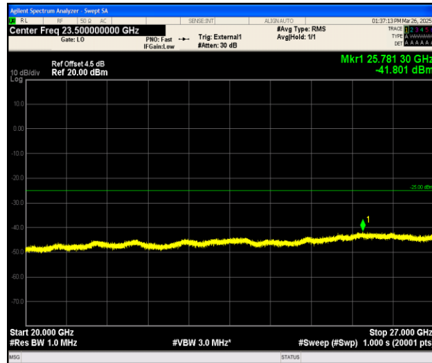
Band41_15MHz_16QAM_39725_1RB#0_20000~27000_20000~27000
