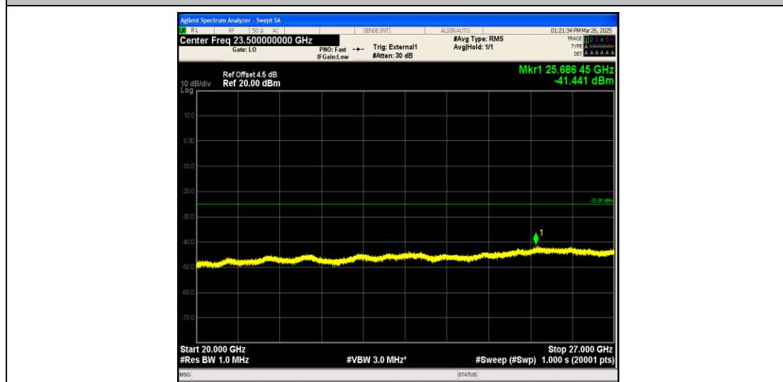
Band41_10MHz_16QAM_40620_1RB#0_20000~27000_20000~27000
