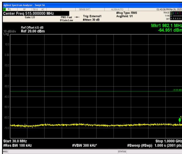
Band41_15MHz_QPSK_41515_1RB#0_30~1000_30~1000
