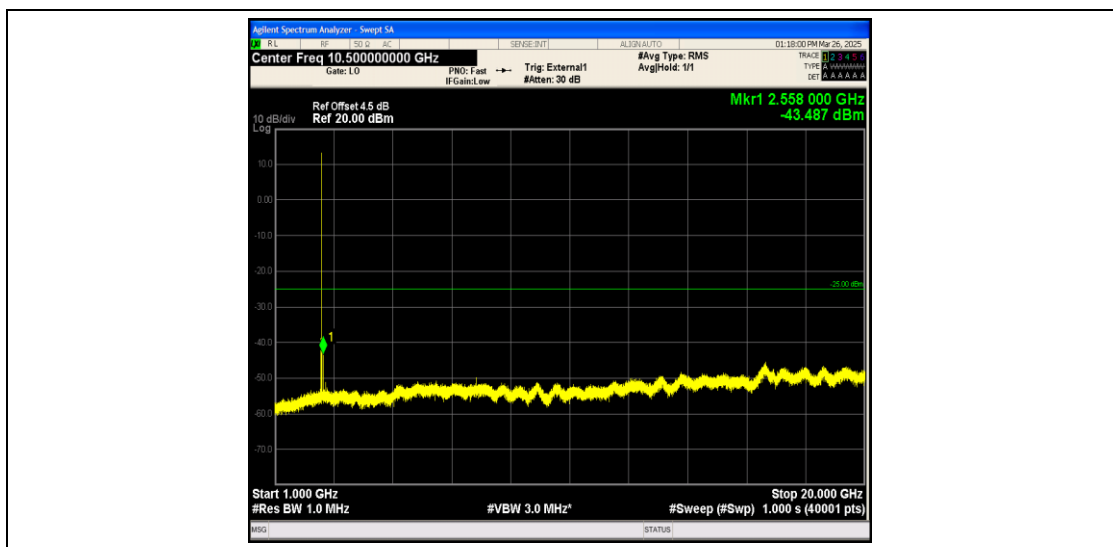
Band41_10MHz_QPSK_39700_1RB#0_1000~20000_1000~20000
