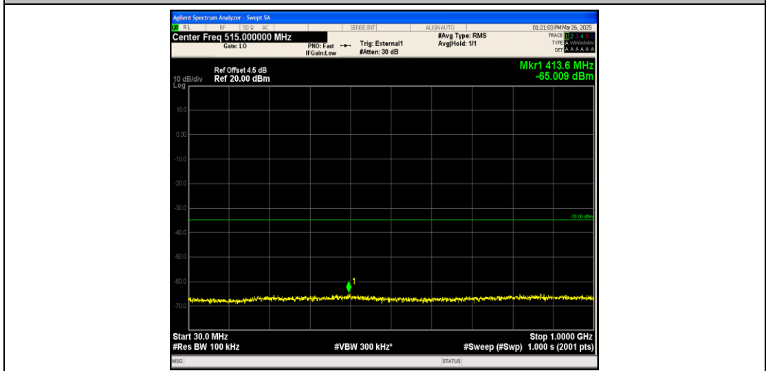
Band41_10MHz_16QAM_40620_1RB#0_30~1000_30~1000
