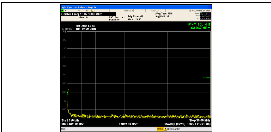
Band41_15MHz_16QAM_39725_1RB#0_0.15~30_0.15~30
