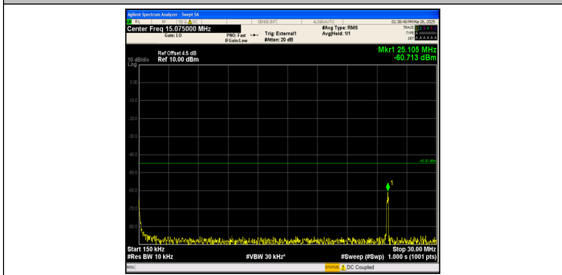
Band41_15MHz_16QAM_40620_1RB#0_0.15~30_0.15~30
