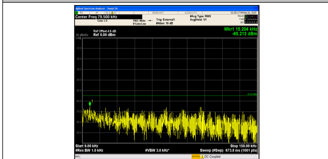
Band41_5MHz_16QAM_41565_1RB#0_0.009~0.15_0.009~0.15
