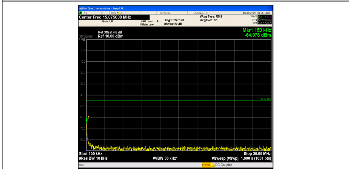
Band41_15MHz_QPSK_39725_1RB#0_0.15~30_0.15~30
