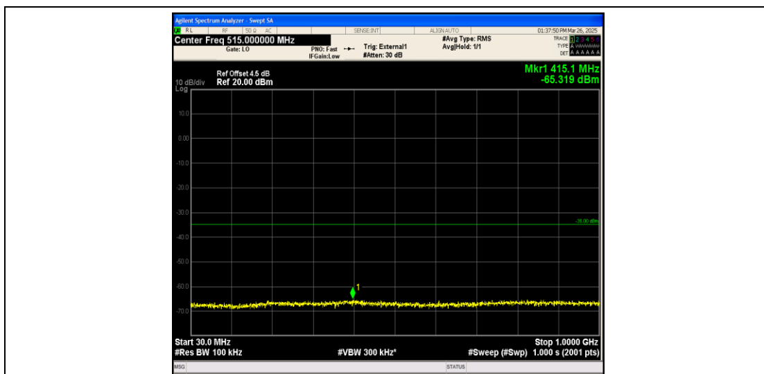
Band41_15MHz_QPSK_40620_1RB#0_30~1000_30~1000
