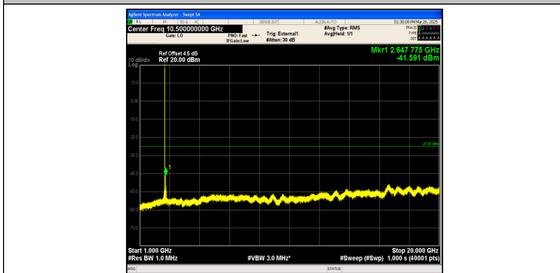
Band41_15MHz_QPSK_40620_1RB#0_1000~20000_1000~20000
