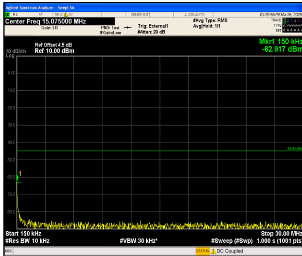
Band41_15MHz_QPSK_41515_1RB#0_0.15~30_0.15~30
