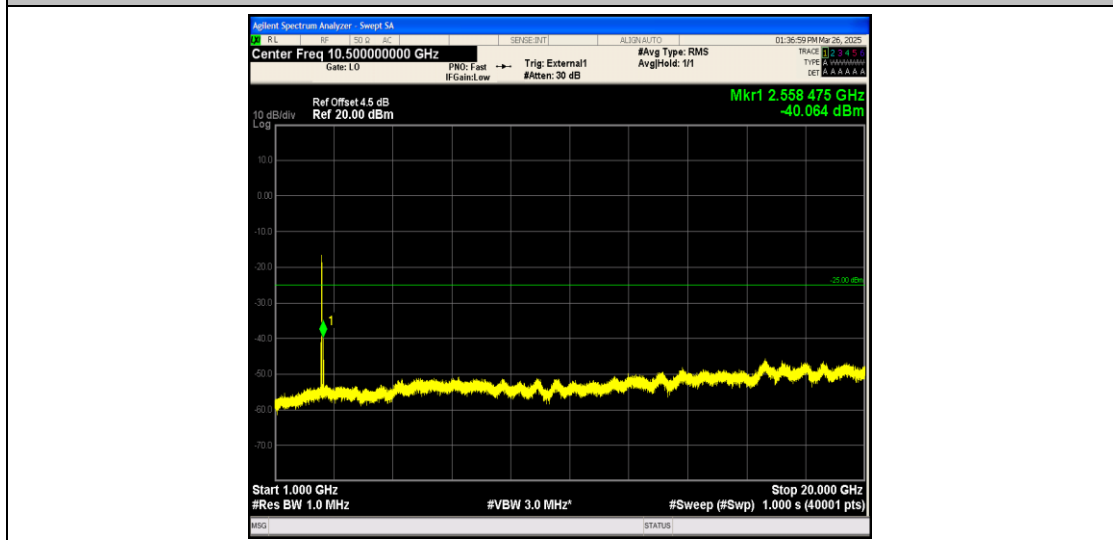
Band41_15MHz_16QAM_39725_1RB#0_1000~20000_1000~20000
