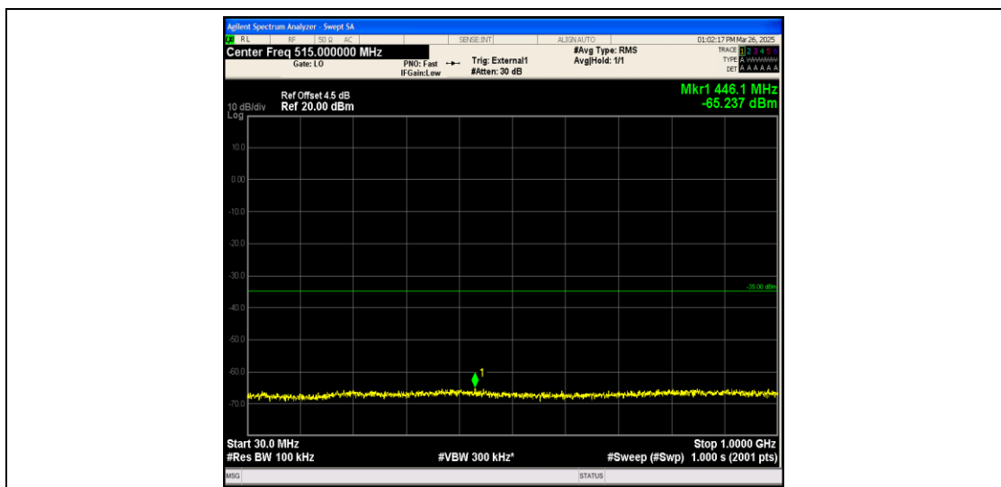
Band41_5MHz_QPSK_40620_1RB#0_30~1000_30~1000
