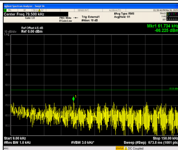
Band41_15MHz_QPSK_41515_1RB#0_0.009~0.15_0.009~0.15
