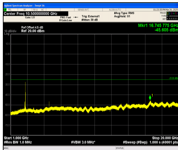
Band41_10MHz_16QAM_41540_1RB#0_1000~20000_1000~20000
