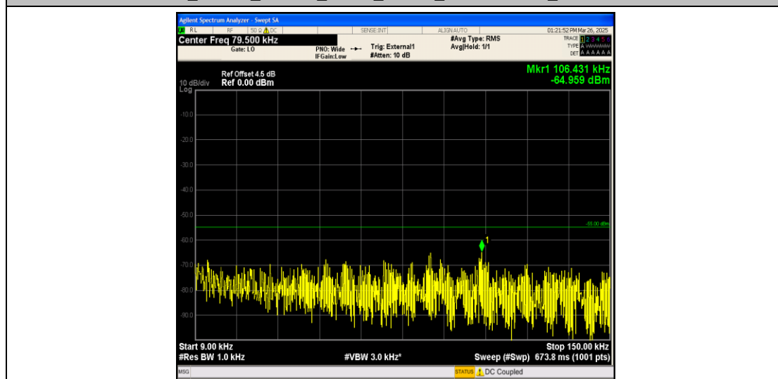
Band41_10MHz_QPSK_41540_1RB#0_0.009~0.15_0.009~0.15
