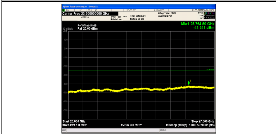
Band41_5MHz_16QAM_40620_1RB#0_20000~27000_20000~27000
