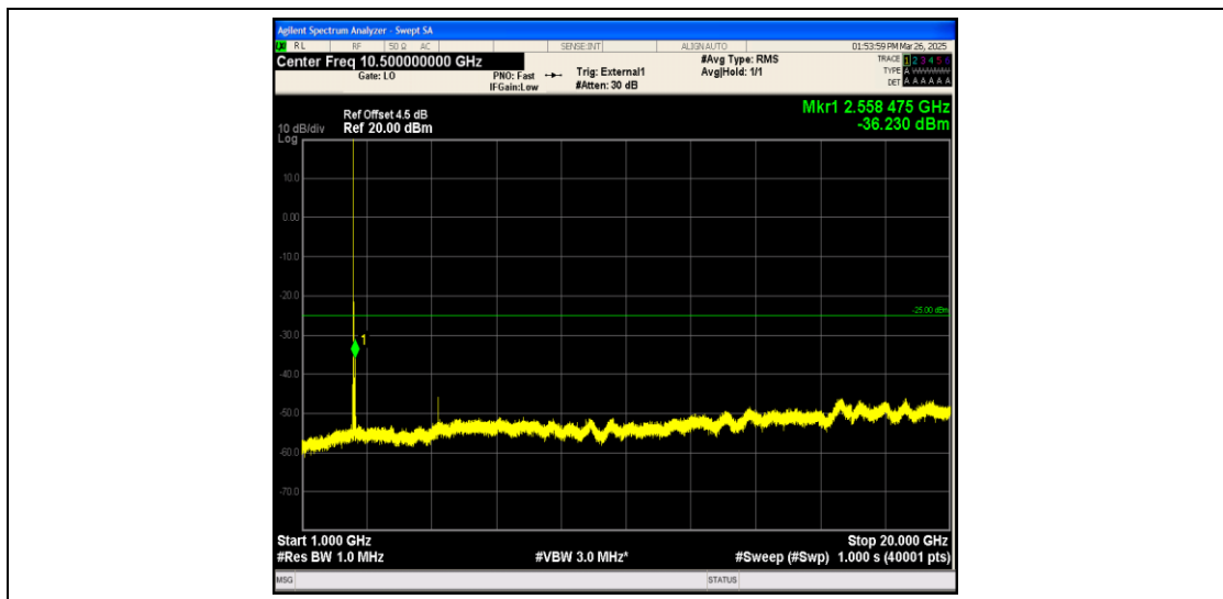
Band41_20MHz_QPSK_39750_1RB#0_1000~20000_1000~20000
