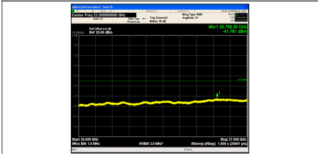
Band41_20MHz_QPSK_39750_1RB#0_20000~27000_20000~27000
