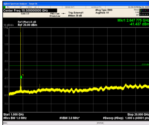
Band41_15MHz_16QAM_40620_1RB#0_1000~20000_1000~20000
