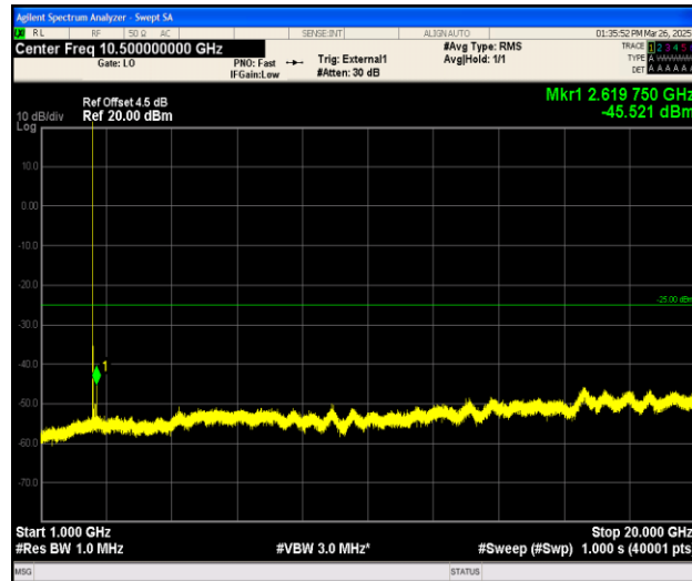
Band41_15MHz_QPSK_39725_1RB#0_1000~20000_1000~20000
