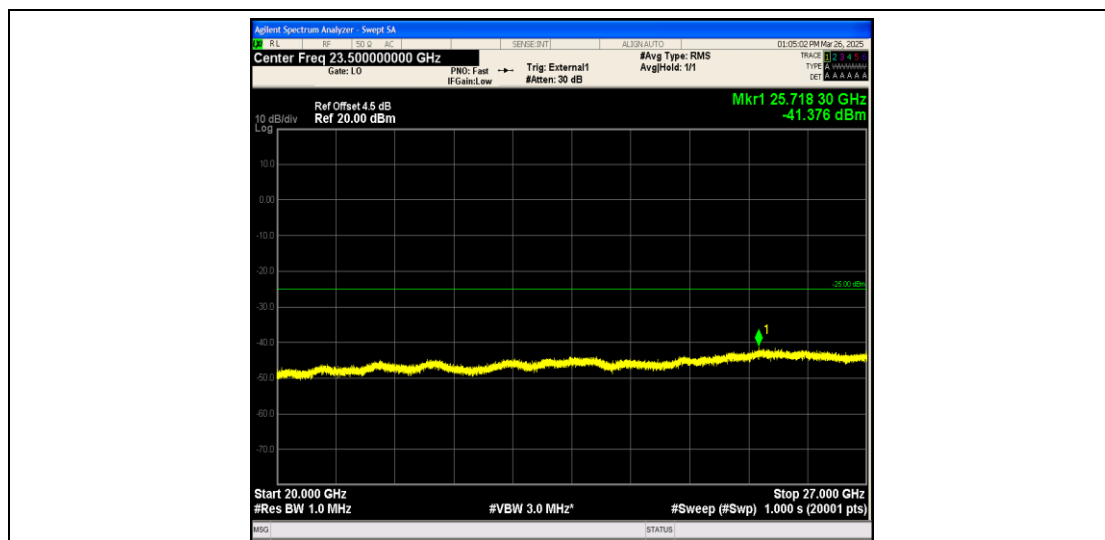
Band41_5MHz_QPSK_41565_1RB#0_20000~27000_20000~27000
