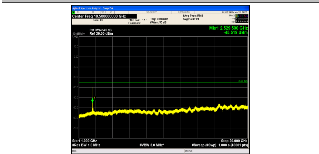
Band41_5MHz_QPSK_40620_1RB#0_1000~20000_1000~20000
