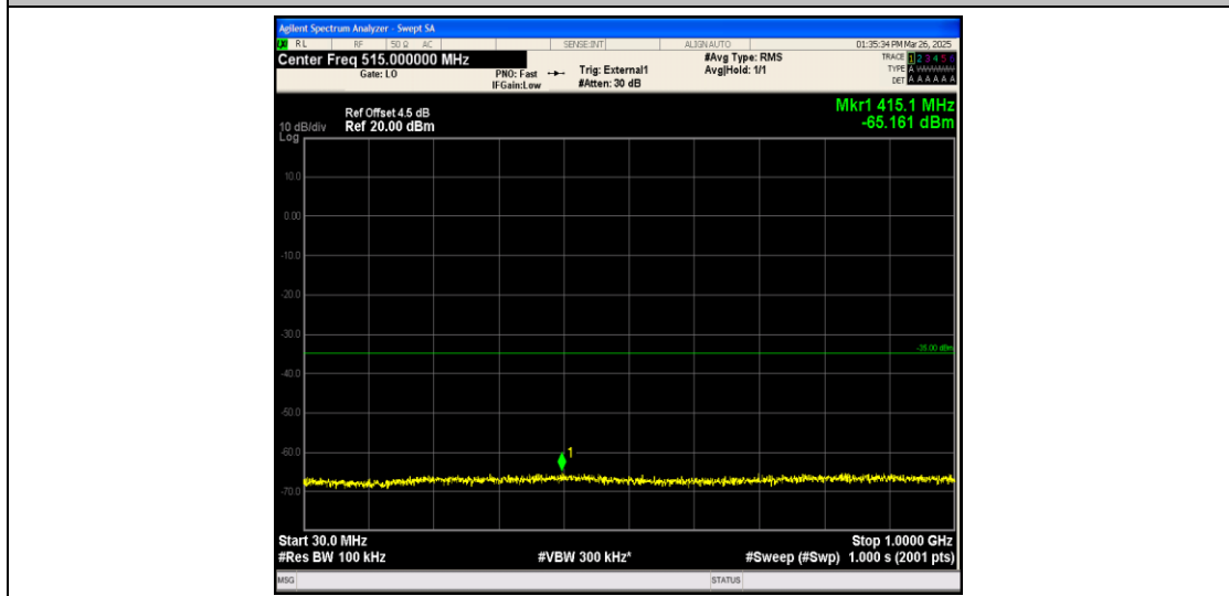
Band41_15MHz_QPSK_39725_1RB#0_30~1000_30~1000
