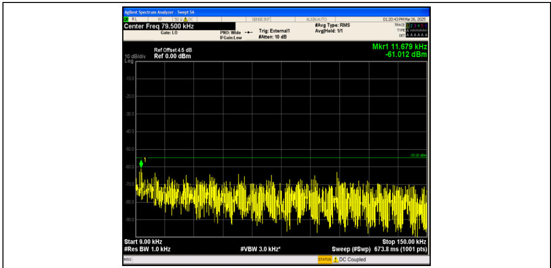
Band41_10MHz_16QAM_40620_1RB#0_0.009~0.15_0.009~0.15
