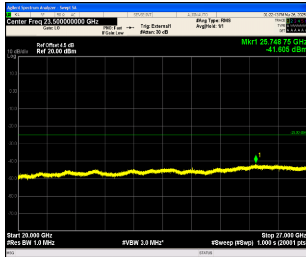
Band41_10MHz_QPSK_41540_1RB#0_20000~27000_20000~27000
