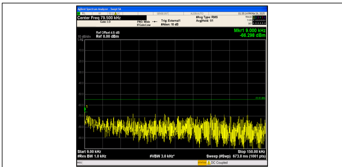
Band41_15MHz_QPSK_39725_1RB#0_0.009~0.15_0.009~0.15
