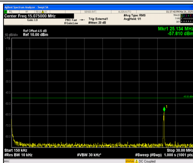
Band41_15MHz_QPSK_40620_1RB#0_0.15~30_0.15~30
