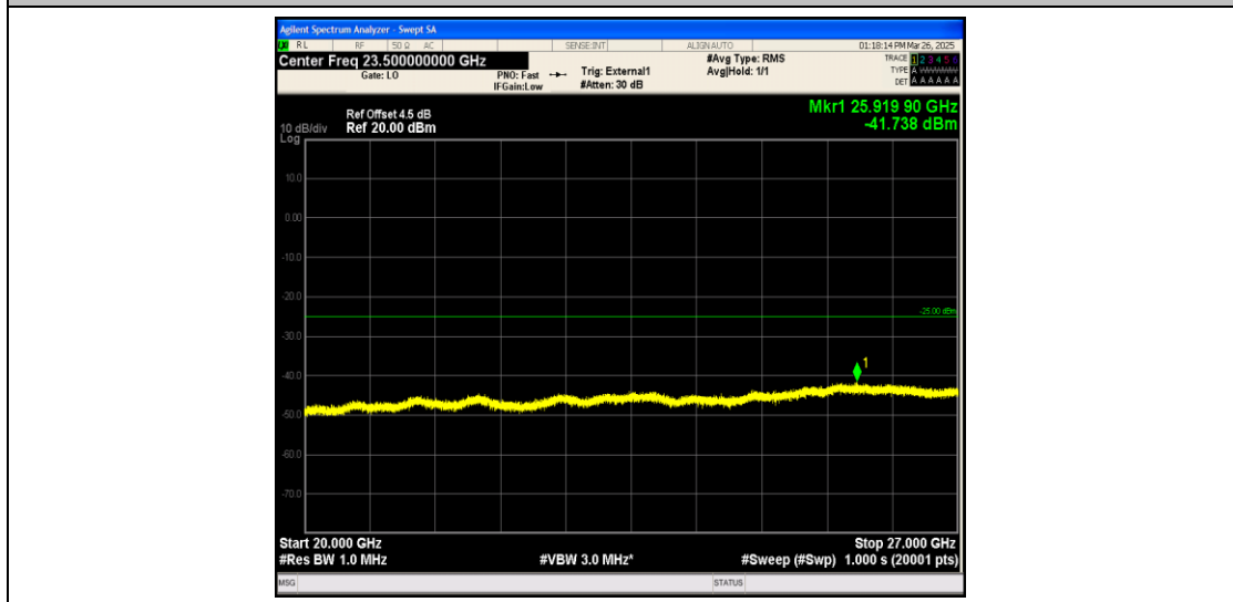
Band41_10MHz_QPSK_39700_1RB#0_20000~27000_20000~27000
