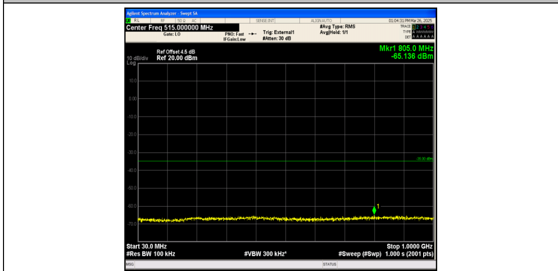
Band41_5MHz_QPSK_41565_1RB#0_30~1000_30~1000
