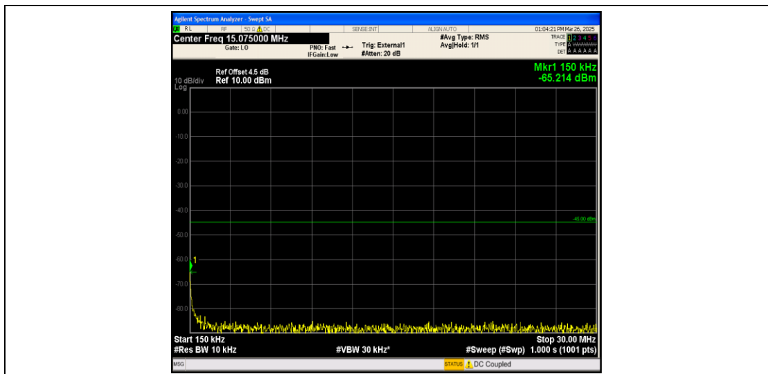
Band41_5MHz_QPSK_41565_1RB#0_0.15~30_0.15~30
