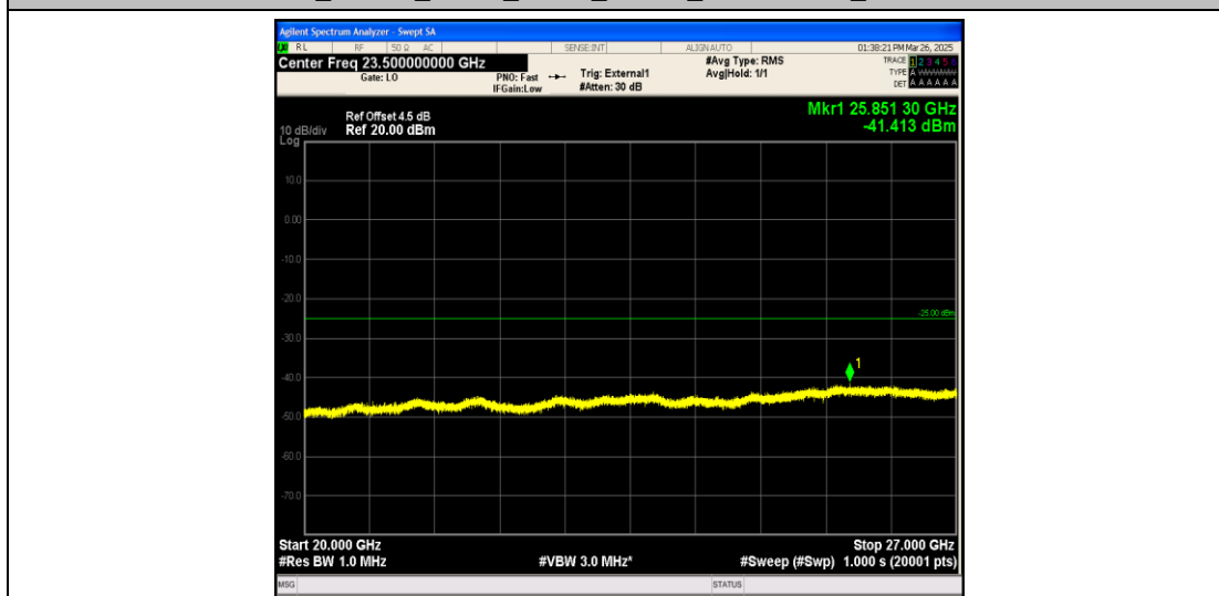
Band41_15MHz_QPSK_40620_1RB#0_20000~27000_20000~27000
