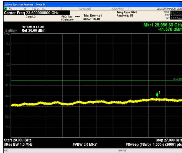
Band41_5MHz_16QAM_39675_1RB#0_20000~27000_20000~27000
