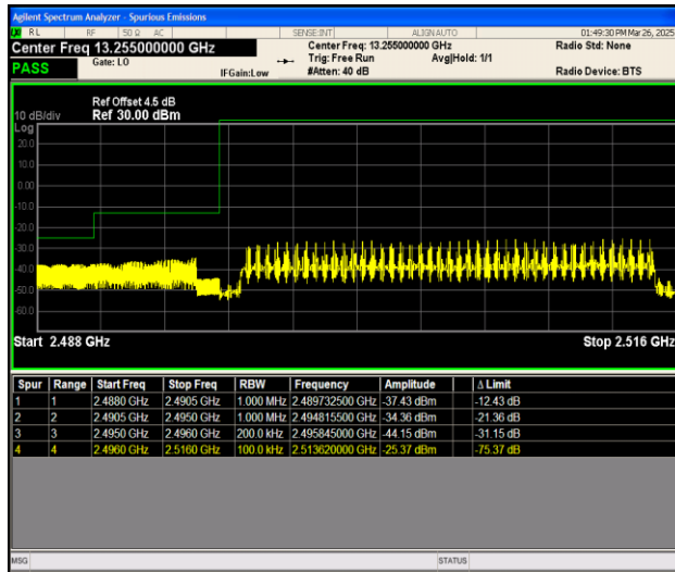
Band41_20MHz_16QAM_39750_100RB#0
