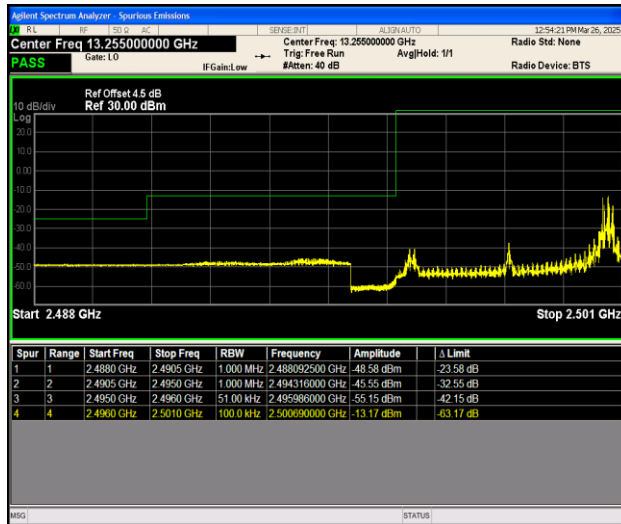
Band41_5MHz_QPSK_39675_1RB#24
