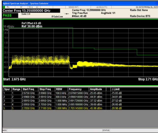
Band41_15MHz_16QAM_41515_75RB#0
