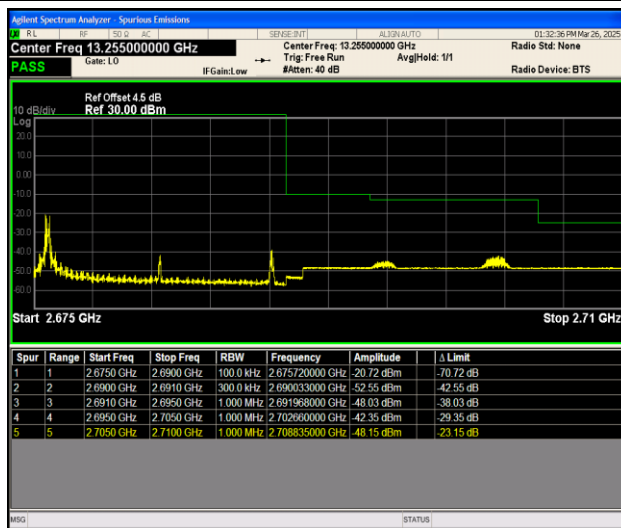
Band41_15MHz_16QAM_41515_1RB#0
