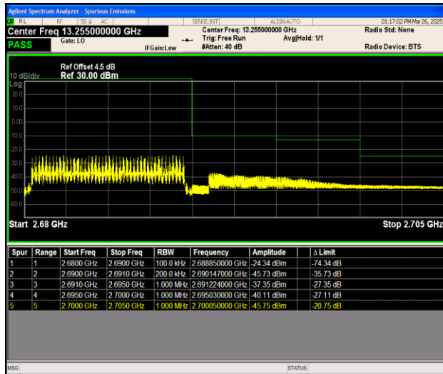
Band41_10MHz_16QAM_41540_50RB#0
