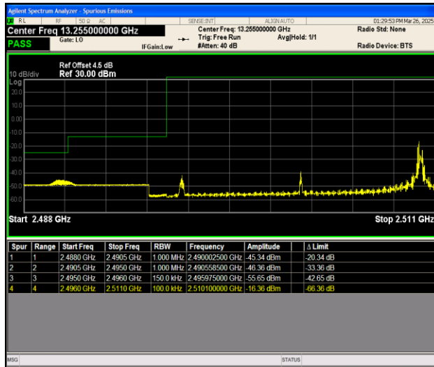
Band41_15MHz_QPSK_39725_1RB#74
