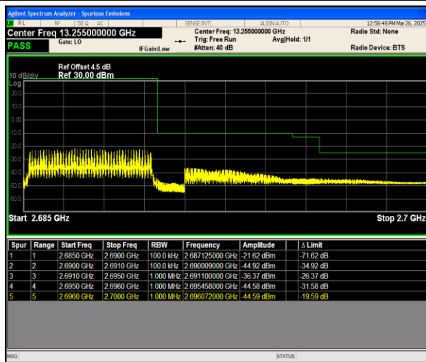
Band41_5MHz_QPSK_41565_25RB#0
