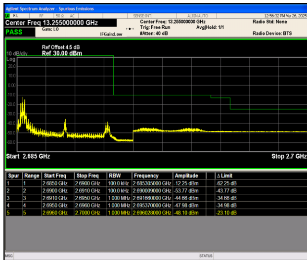
Band41_5MHz_QPSK_41565_1RB#0
