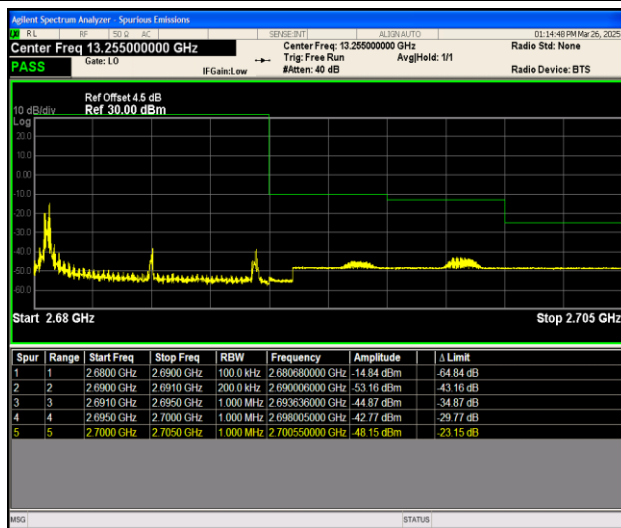
Band41_10MHz_16QAM_41540_1RB#0
