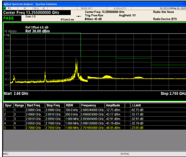
Band41_10MHz_QPSK_41540_1RB#49
