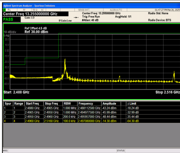
Band41_20MHz_16QAM_39750_1RB#0
