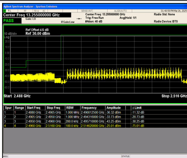
Band41_20MHz_QPSK_39750_100RB#0
