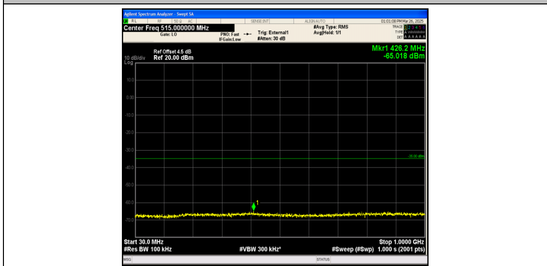
Band41_5MHz_16QAM_39675_1RB#0_30~1000_30~1000
