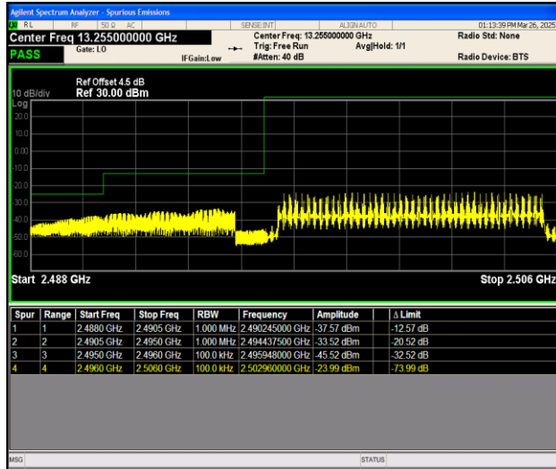
Band41_10MHz_16QAM_39700_50RB#0
