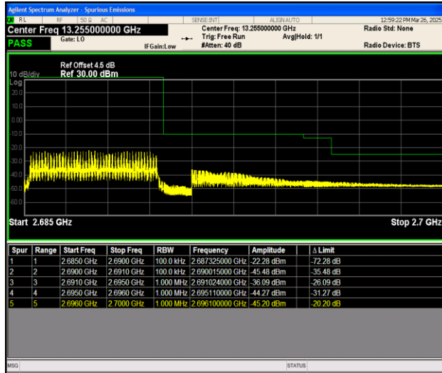
Band41_5MHz_16QAM_41565_25RB#0
