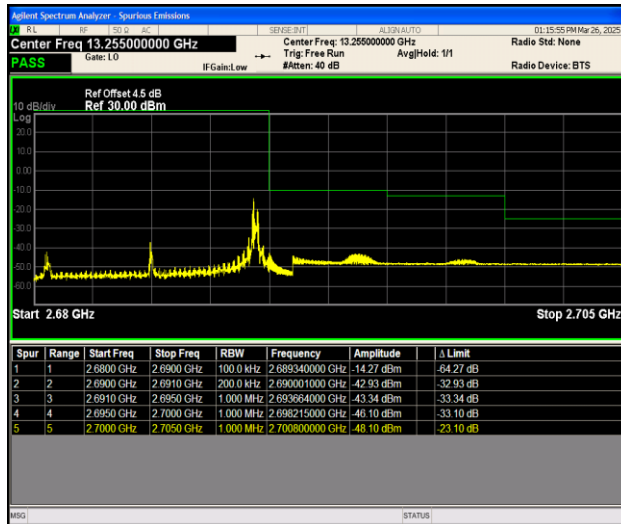
Band41_10MHz_16QAM_41540_1RB#49
