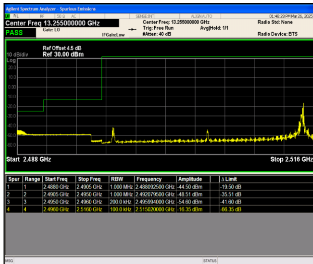
Band41_20MHz_16QAM_39750_1RB#99
