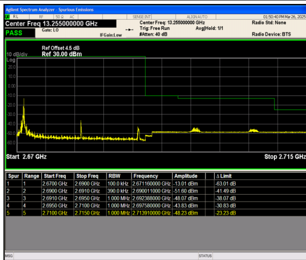
Band41_20MHz_16QAM_41490_1RB#0
