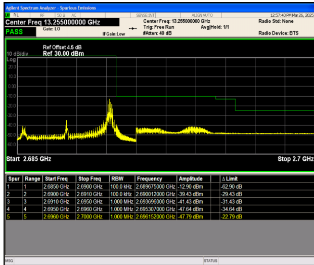
Band41_5MHz_QPSK_41565_1RB#24
