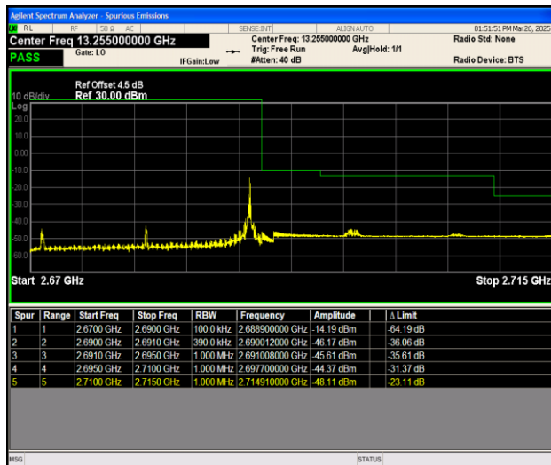
Band41_20MHz_16QAM_41490_1RB#99
