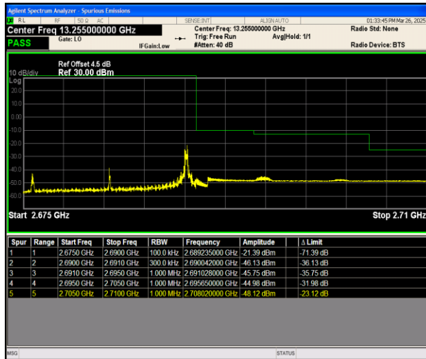
Band41_15MHz_16QAM_41515_1RB#74
