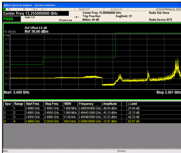
Band41_5MHz_16QAM_39675_1RB#24
