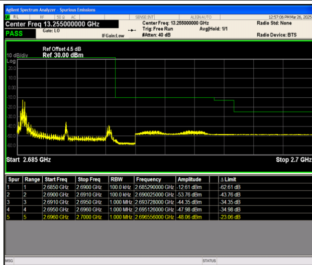
Band41_5MHz_16QAM_41565_1RB#0
