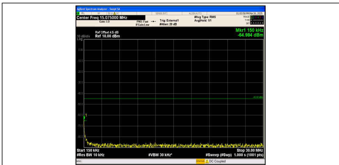
Band41_5MHz_16QAM_39675_1RB#0_0.15~30_0.15~30
