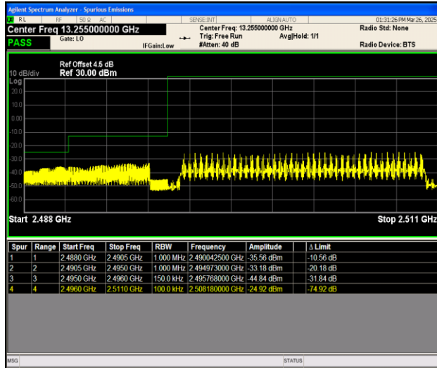
Band41_15MHz_16QAM_39725_75RB#0
