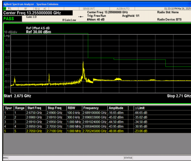
Band41_15MHz_QPSK_41515_1RB#74
