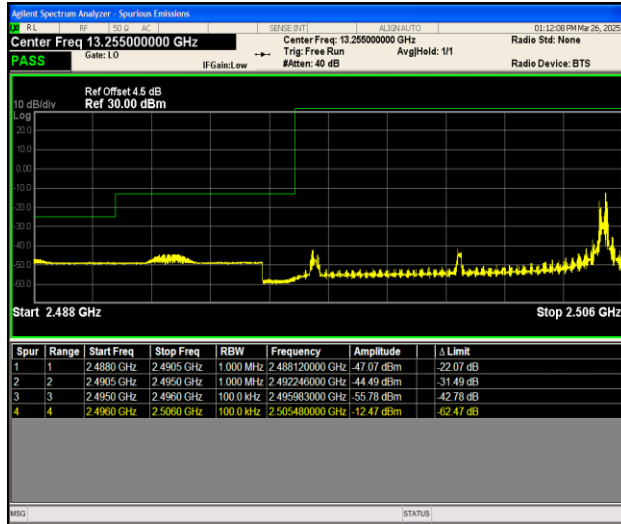
Band41_10MHz_QPSK_39700_1RB#49
