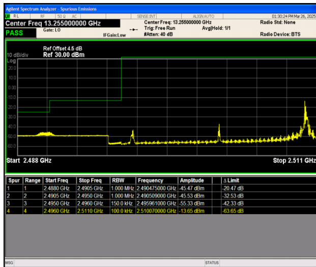
Band41_15MHz_16QAM_39725_1RB#74
