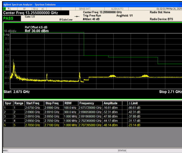
Band41_15MHz_QPSK_41515_1RB#0
