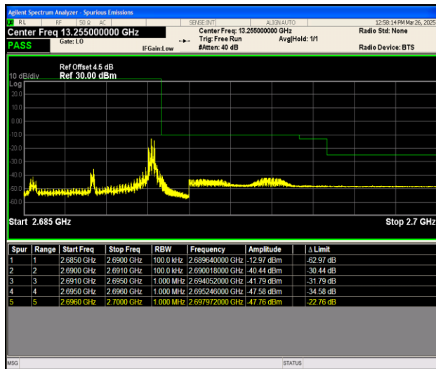
Band41_5MHz_16QAM_41565_1RB#24
