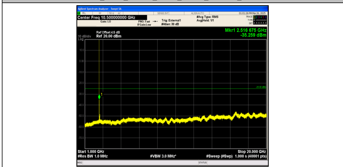
Band41_5MHz_16QAM_39675_1RB#0_1000~20000_1000~20000
