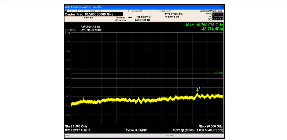
Band41_5MHz_QPSK_39675_1RB#0_1000~20000_1000~20000
