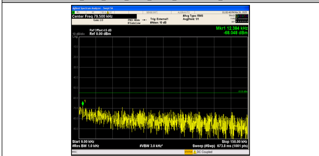
Band41_5MHz_16QAM_39675_1RB#0_0.009~0.15_0.009~0.15
