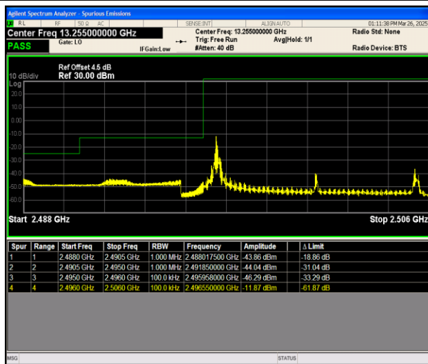
Band41_10MHz_16QAM_39700_1RB#0
