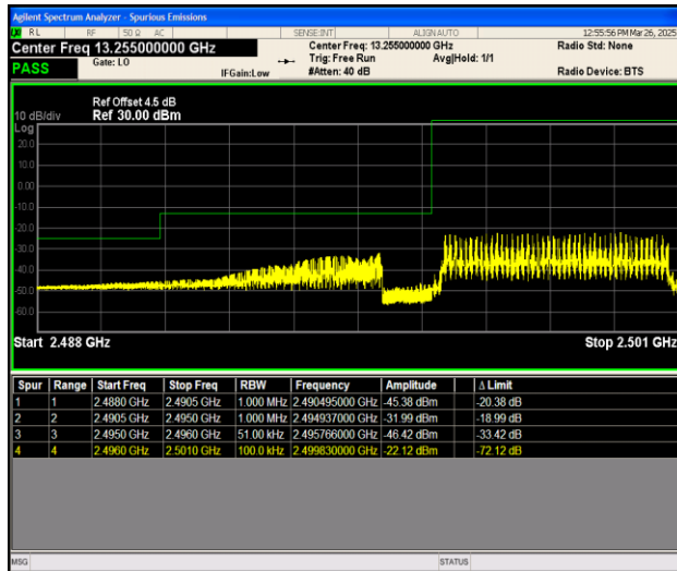
Band41_5MHz_16QAM_39675_25RB#0
