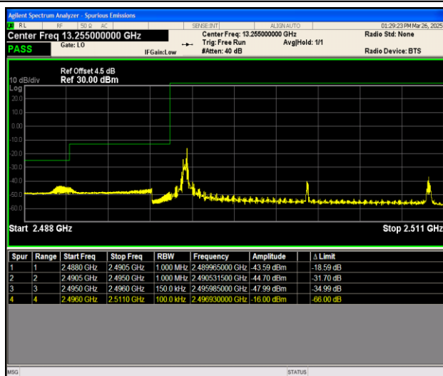
Band41_15MHz_16QAM_39725_1RB#0
