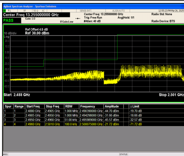
Band41_5MHz_QPSK_39675_25RB#0
