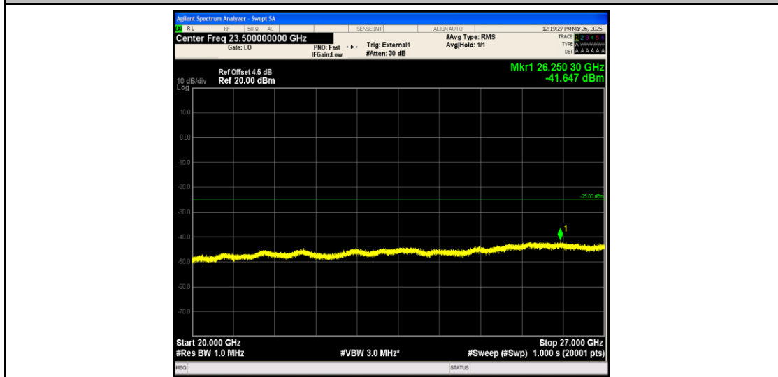
Band38_15MHz_16QAM_38000_1RB#0_20000~27000_20000~27000
