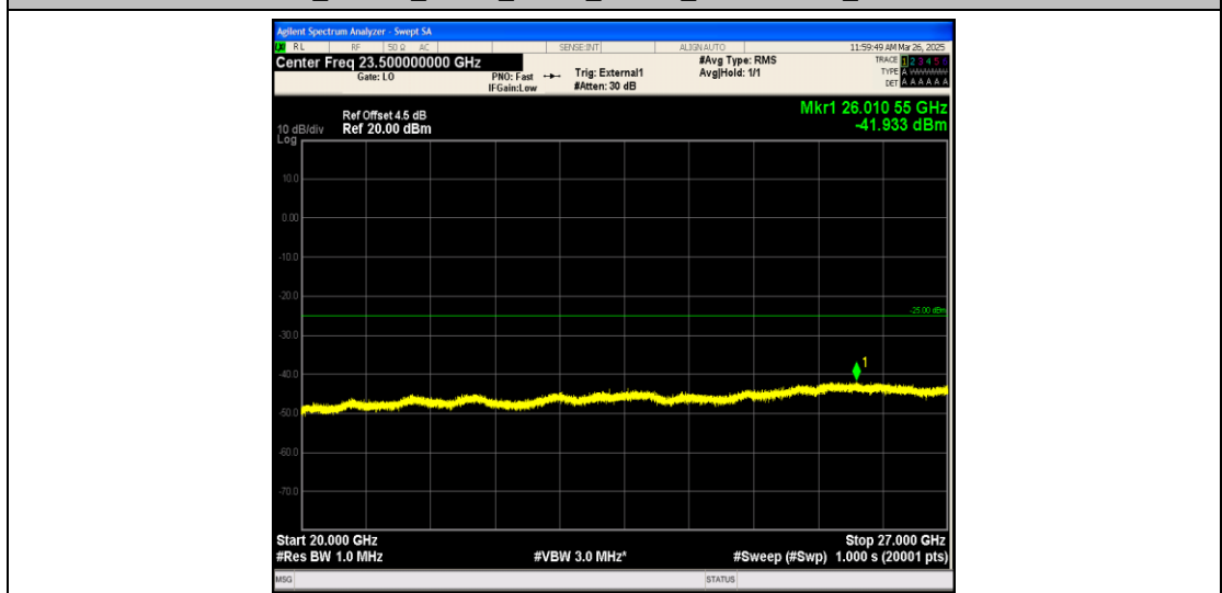
Band38_10MHz_QPSK_38000_1RB#0_20000~27000_20000~27000
