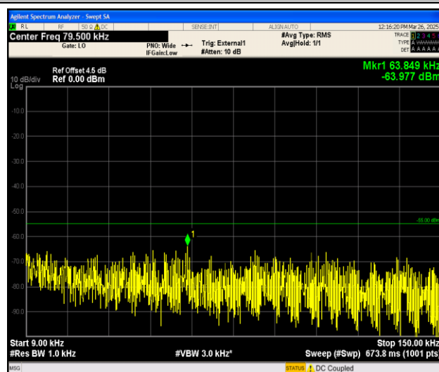
Band38_15MHz_16QAM_37825_1RB#0_0.009~0.15_0.009~0.15
