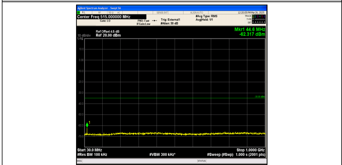
Band38_15MHz_QPSK_38175_1RB#0_30~1000_30~1000
