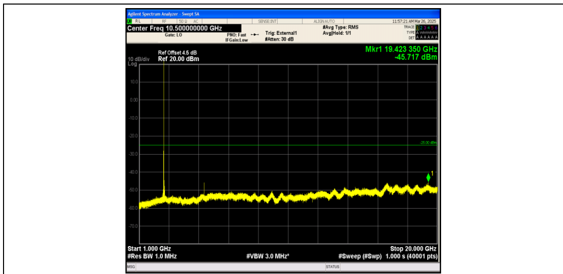
Band38_10MHz_QPSK_37800_1RB#0_1000~20000_1000~20000
