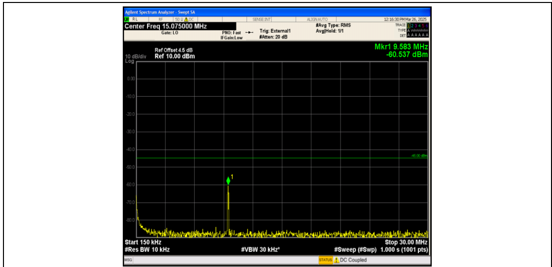
Band38_15MHz_16QAM_37825_1RB#0_0.15~30_0.15~30
