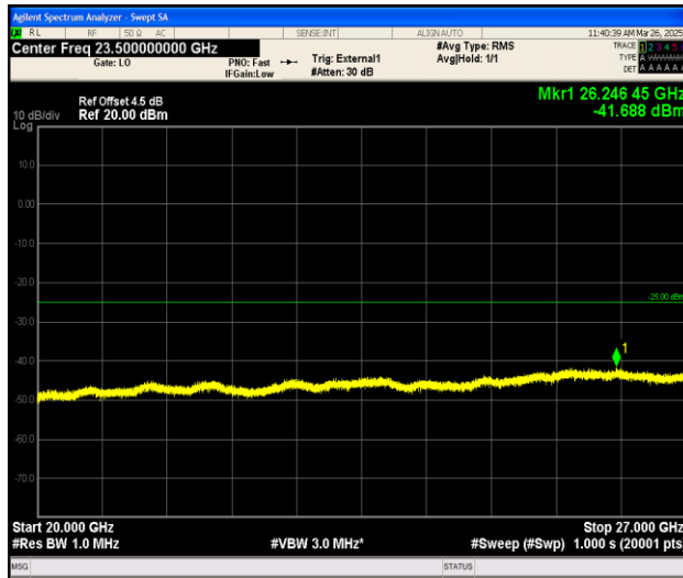
Band38_5MHz_16QAM_37775_1RB#0_20000~27000_20000~27000
