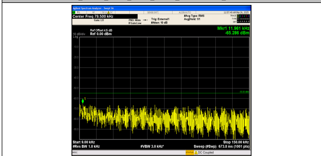
Band38_10MHz_16QAM_37800_1RB#0_0.009~0.15_0.009~0.15
