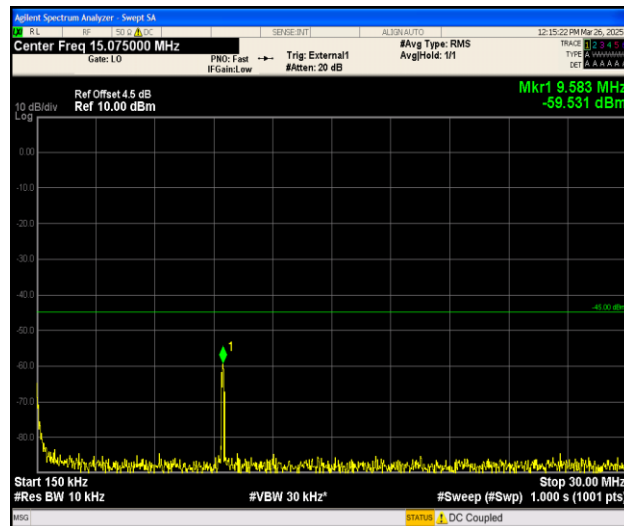
Band38_15MHz_QPSK_37825_1RB#0_0.15~30_0.15~30
