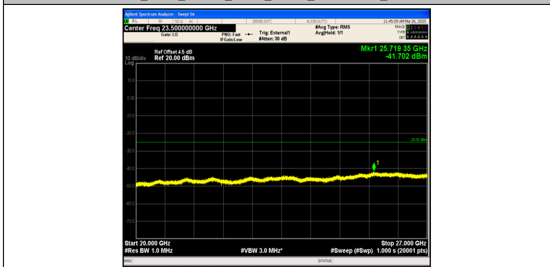
Band38_5MHz_16QAM_38225_1RB#0_20000~27000_20000~27000
