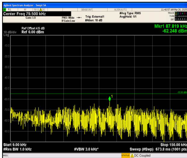
Band38_5MHz_QPSK_38000_1RB#0_0.009~0.15_0.009~0.15
