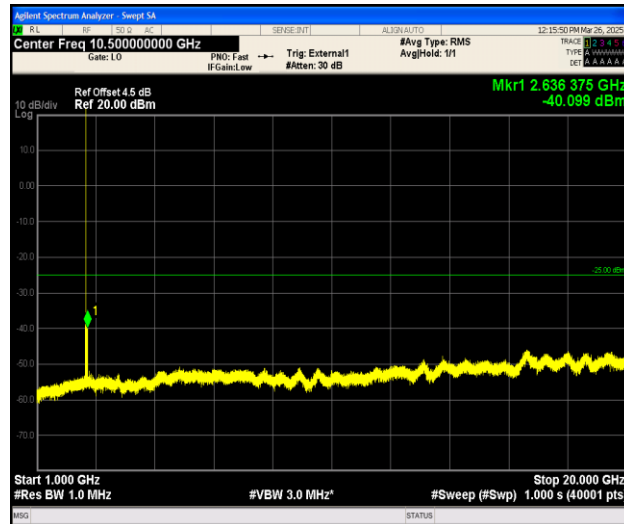
Band38_15MHz_QPSK_37825_1RB#0_1000~20000_1000~20000
