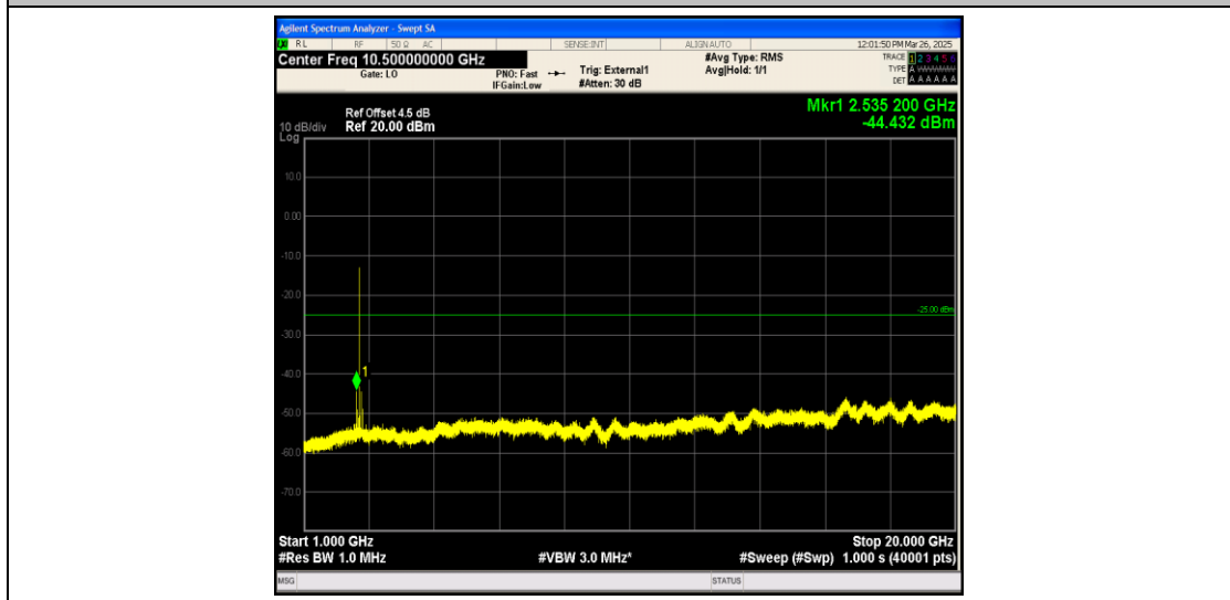
Band38_10MHz_QPSK_38200_1RB#0_1000~20000_1000~20000
