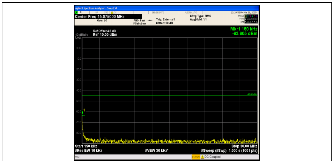
Band38_15MHz_QPSK_38175_1RB#0_0.15~30_0.15~30
