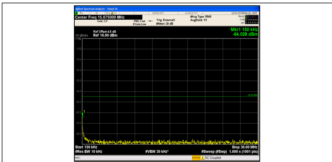
Band38_10MHz_QPSK_38200_1RB#0_0.15~30_0.15~30
