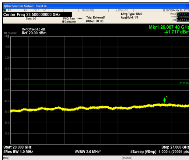
Band38_10MHz_16QAM_38000_1RB#0_20000~27000_20000~27000
