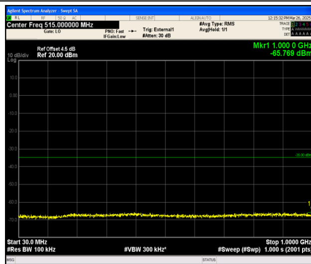
Band38_15MHz_QPSK_37825_1RB#0_30~1000_30~1000
