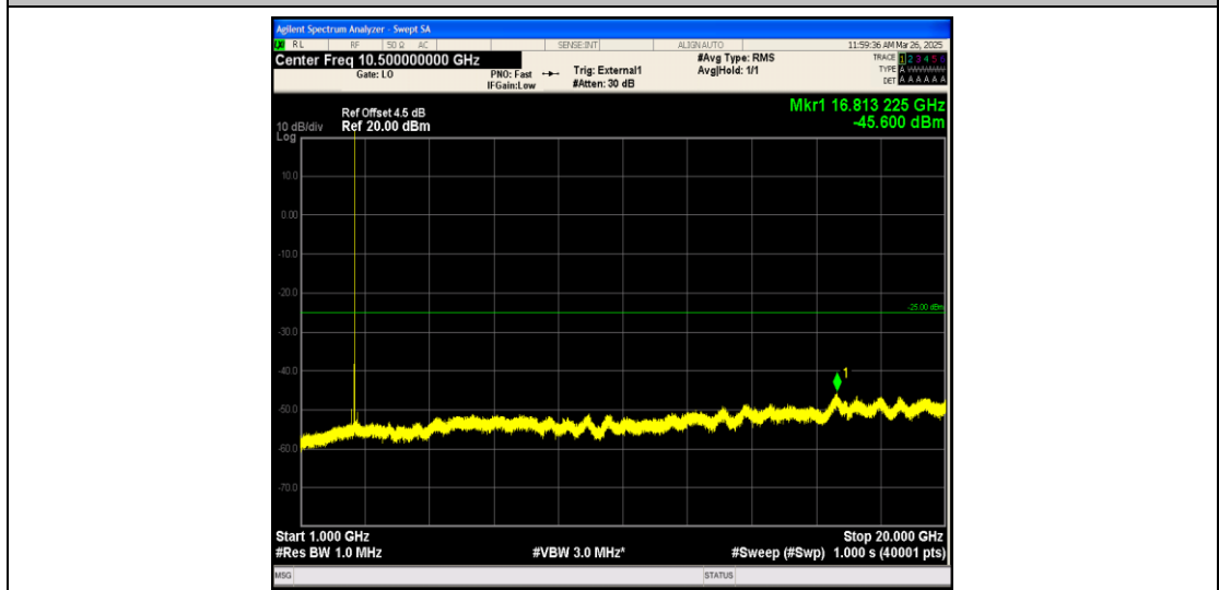
Band38_10MHz_QPSK_38000_1RB#0_1000~20000_1000~20000
