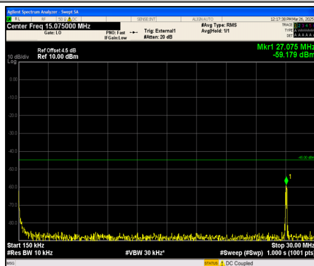
Band38_15MHz_QPSK_38000_1RB#0_0.15~30_0.15~30
