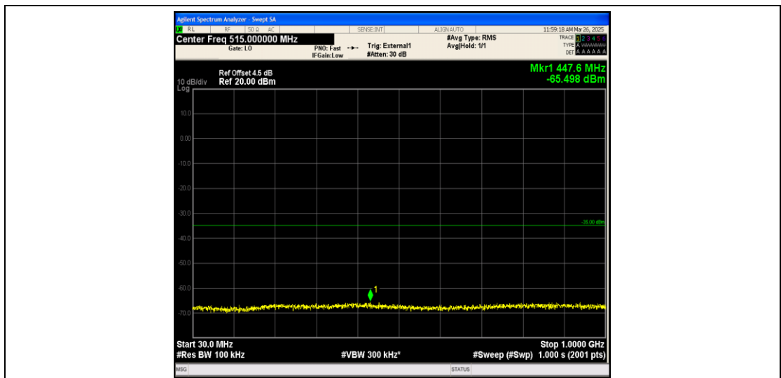
Band38_10MHz_QPSK_38000_1RB#0_30~1000_30~1000
