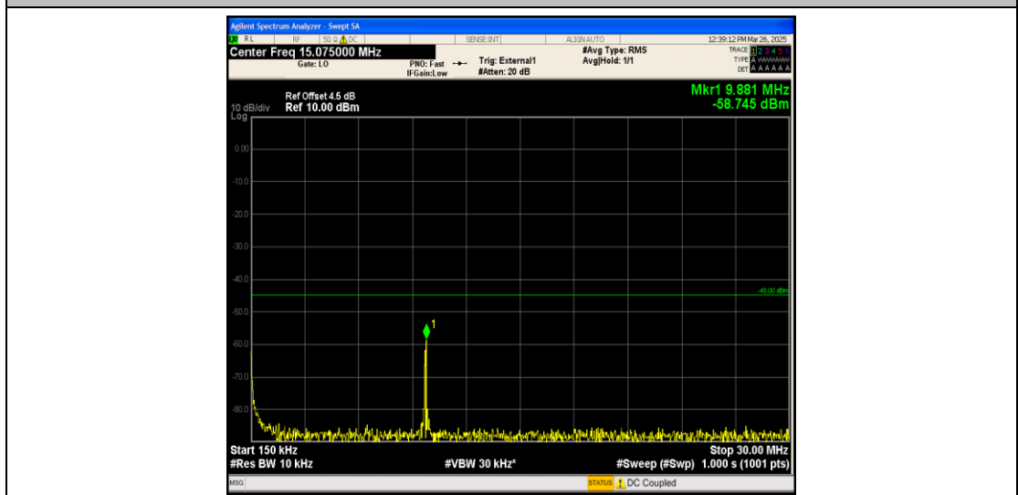
Band38_20MHz_QPSK_37850_1RB#0_0.15~30_0.15~30
