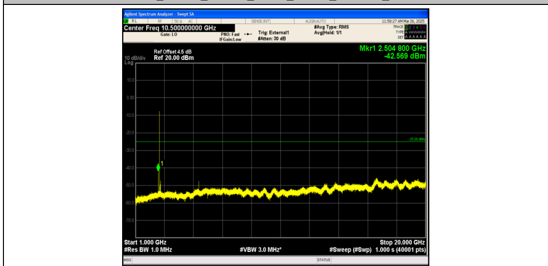
Band38_10MHz_16QAM_37800_1RB#0_1000~20000_1000~20000
