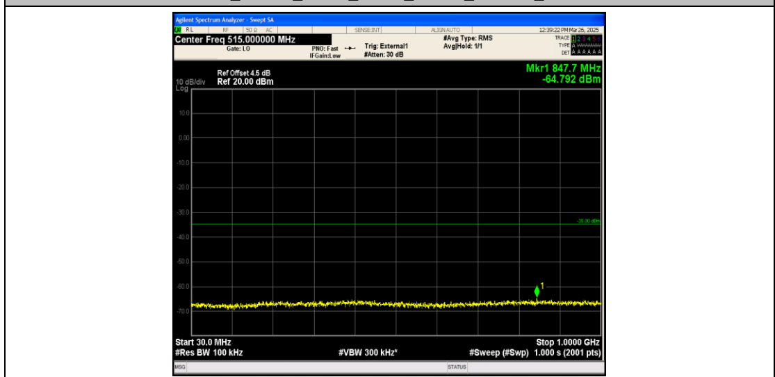
Band38_20MHz_QPSK_37850_1RB#0_30~1000_30~1000
