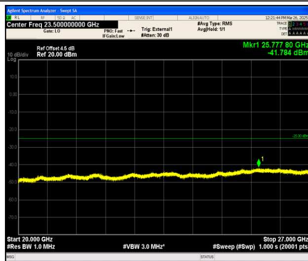
Band38_15MHz_16QAM_38175_1RB#0_20000~27000_20000~27000
