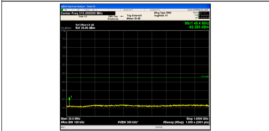
Band38_10MHz_QPSK_38200_1RB#0_30~1000_30~1000
