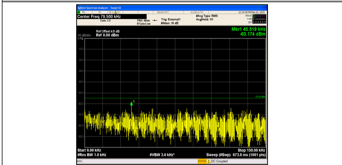
Band38_15MHz_QPSK_38175_1RB#0_0.009~0.15_0.009~0.15
