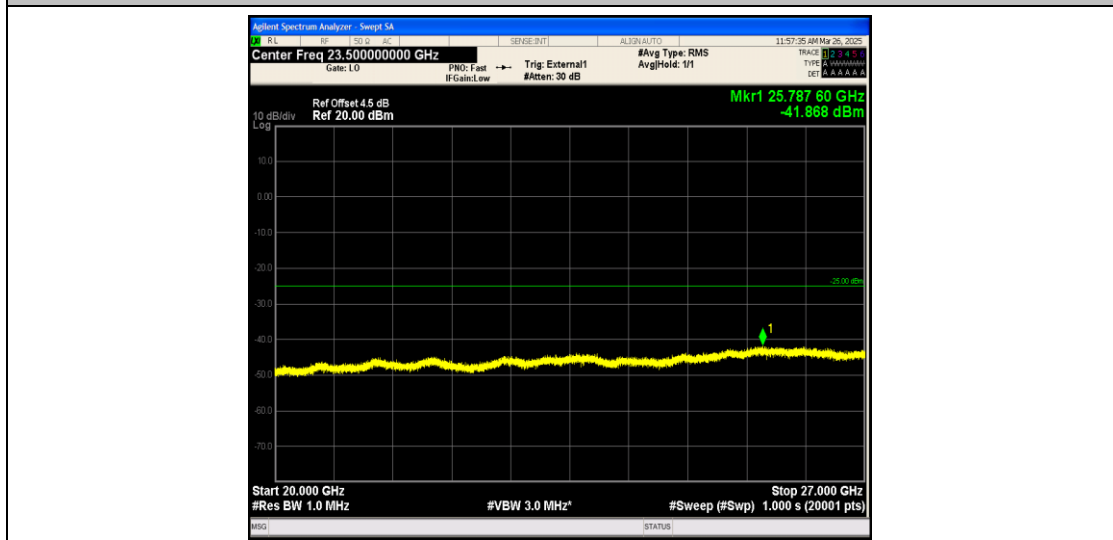
Band38_10MHz_QPSK_37800_1RB#0_20000~27000_20000~27000
