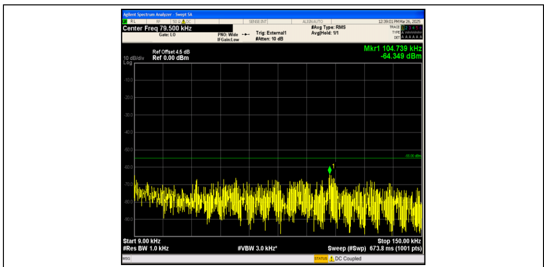
Band38_20MHz_QPSK_37850_1RB#0_0.009~0.15_0.009~0.15
