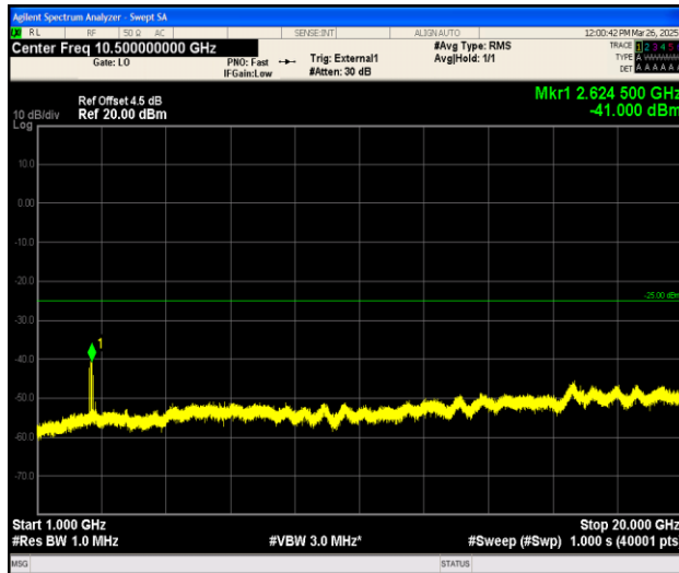
Band38_10MHz_16QAM_38000_1RB#0_1000~20000_1000~20000
