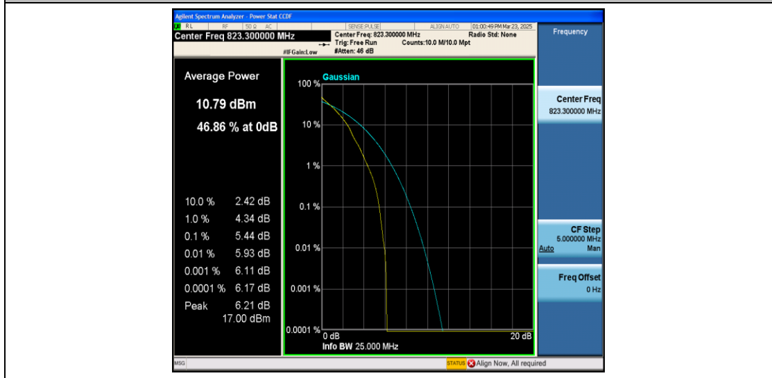
26(814-824)-1.4MHz-QPSK-26783-1RB#0-PASS
