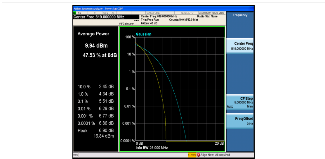
26(814-824)-1.4MHz-QPSK-26740-6RB#0-PASS
