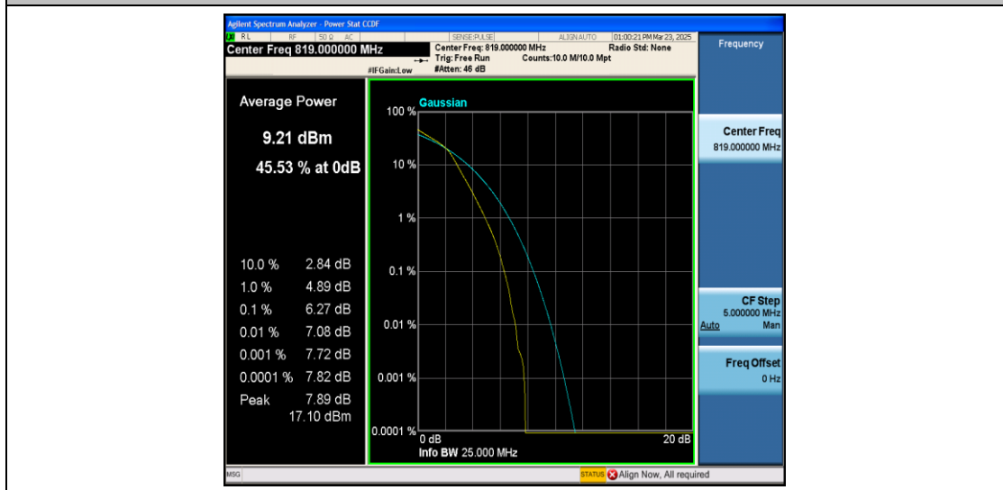
26(814-824)-1.4MHz-16QAM-26740-6RB#0-PASS
