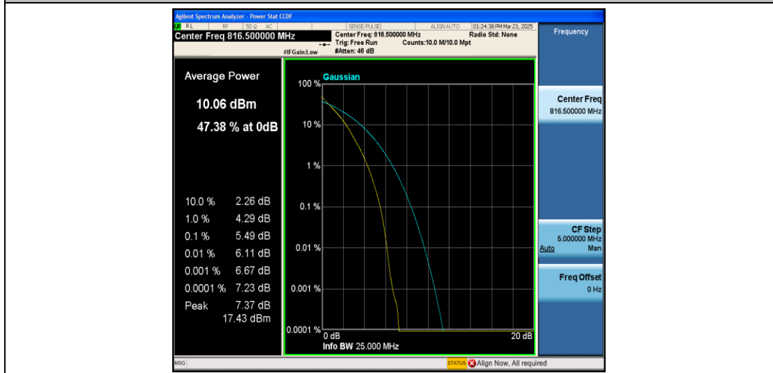
26(814-824)-5MHz-QPSK-26715-25RB#0-PASS
