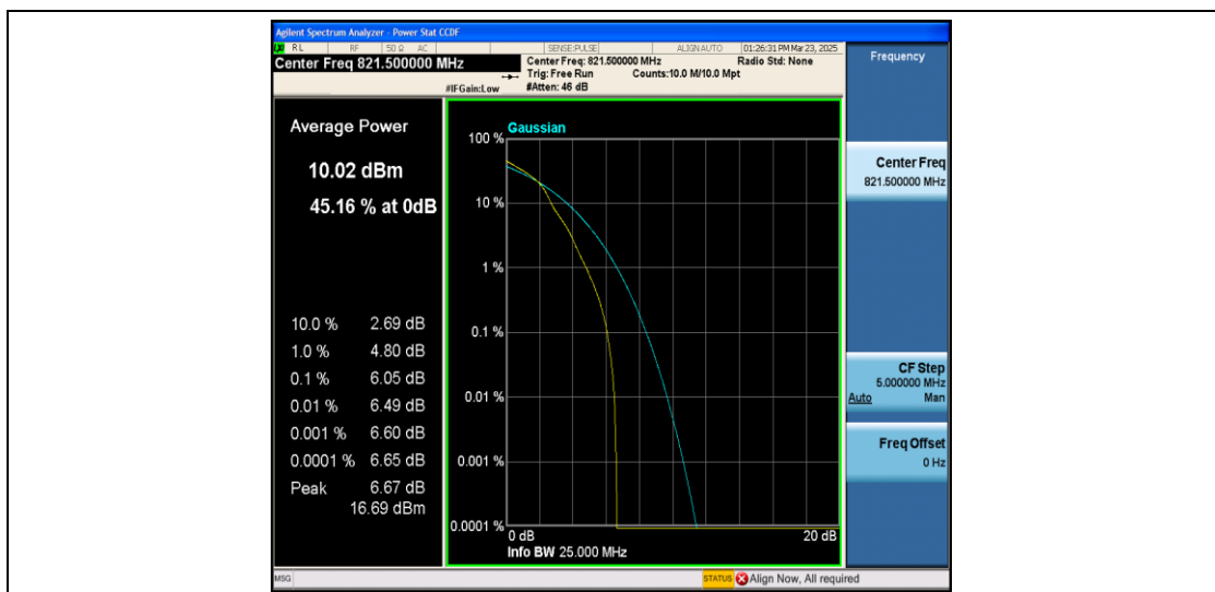
26(814-824)-5MHz-16QAM-26765-1RB#0-PASS
