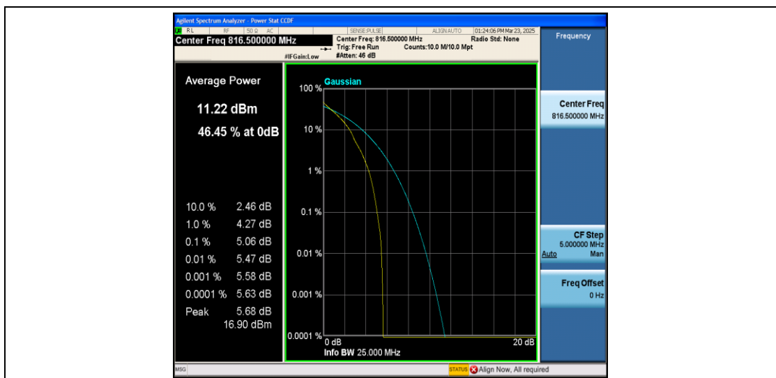
26(814-824)-5MHz-QPSK-26715-1RB#0-PASS
