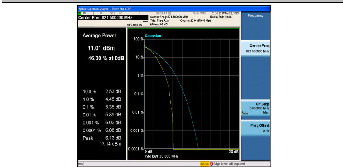
26(814-824)-5MHz-QPSK-26765-1RB#0-PASS
