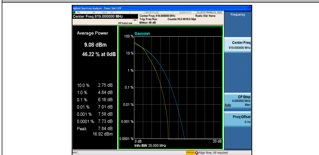
26(814-824)-5MHz-16QAM-26740-25RB#0-PASS
