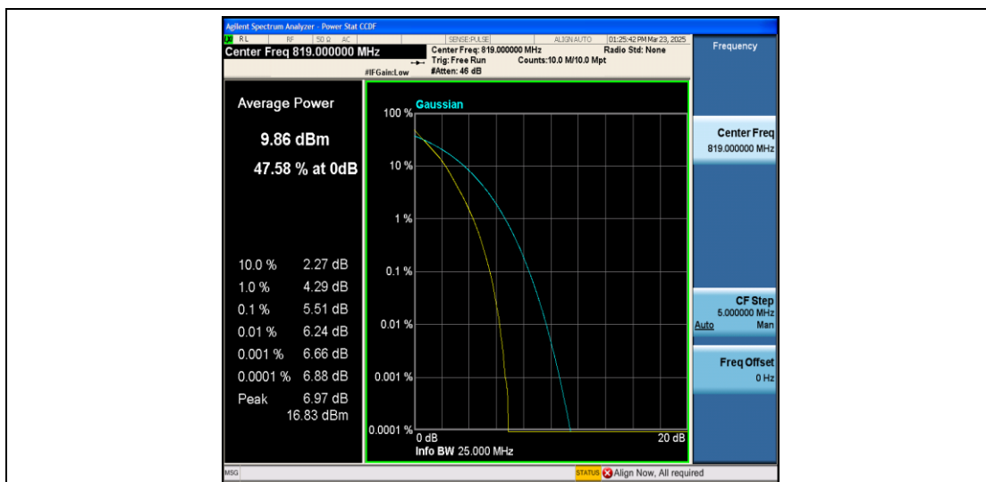
26(814-824)-5MHz-QPSK-26740-25RB#0-PASS
