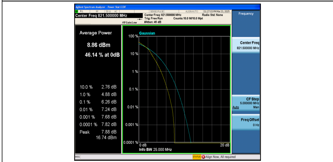
26(814-824)-5MHz-16QAM-26765-25RB#0-PASS
