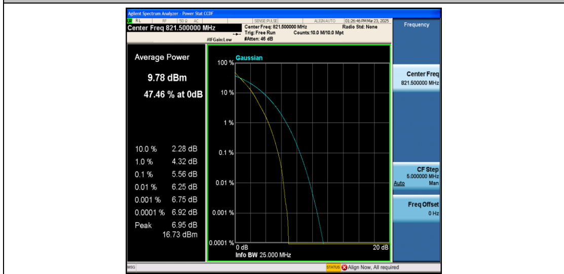
26(814-824)-5MHz-QPSK-26765-25RB#0-PASS
