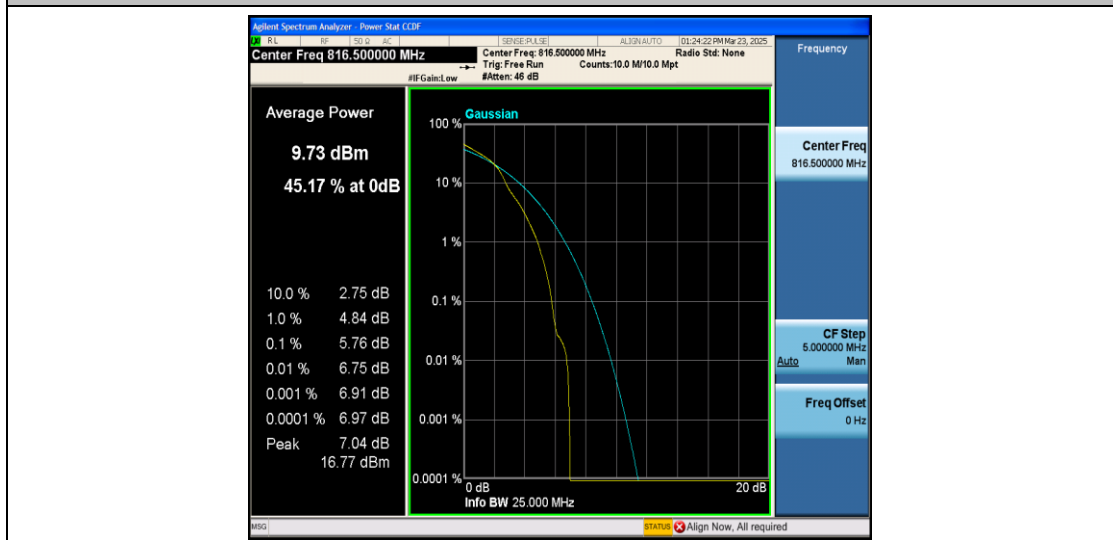
26(814-824)-5MHz-16QAM-26715-1RB#0-PASS
