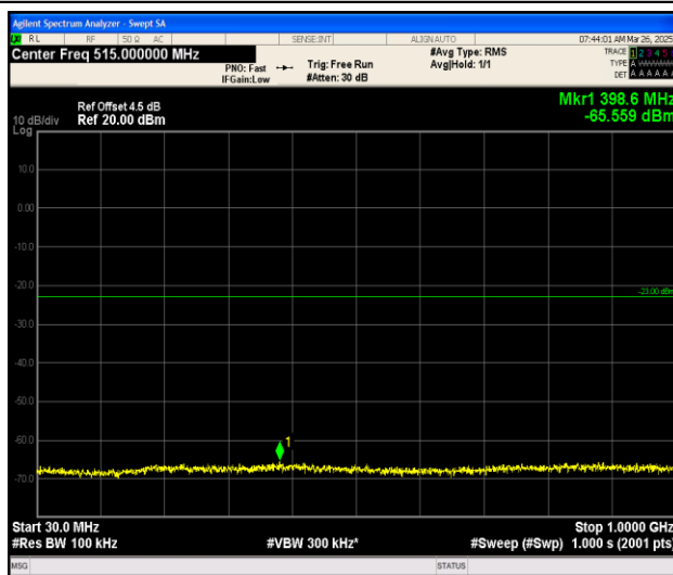
Band25_3MHz_QPSK_26675_1RB#0_30~1000_30~1000
