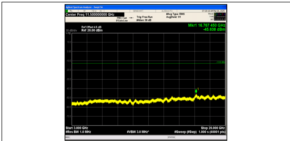
Band25_3MHz_QPSK_26365_1RB#0_3000~20000_3000~20000
