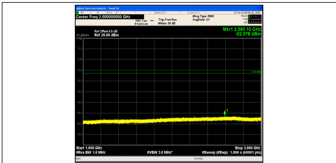
Band25_3MHz_QPSK_26675_1RB#0_1000~3000_1000~3000
