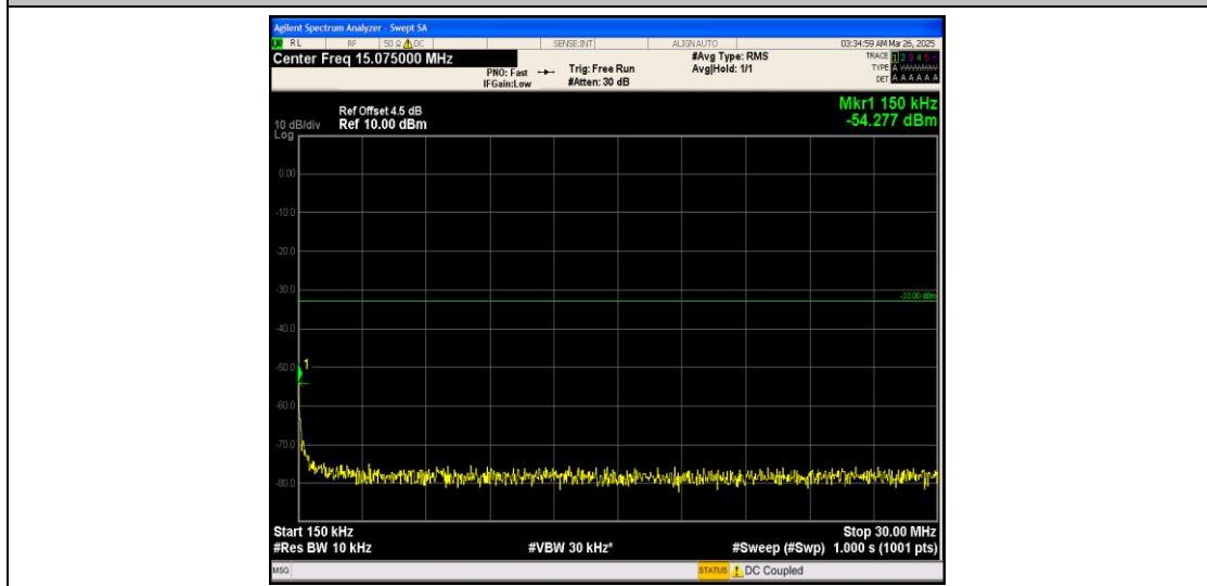
Band25_1.4MHz_16QAM_26365_1RB#0_0.15~30_0.15~30
