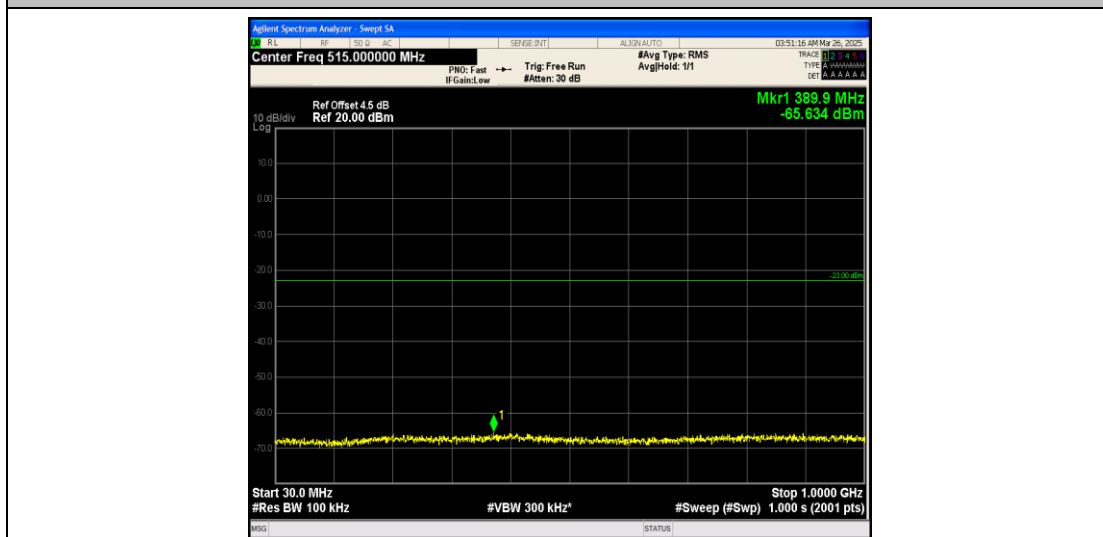
Band25_1.4MHz_16QAM_26683_1RB#0_30~1000_30~1000
