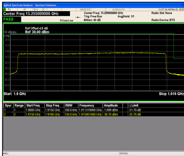
Band25_15MHz_16QAM_26615_75RB#0
