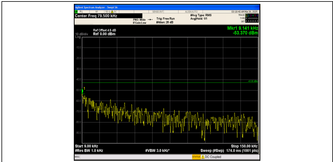
Band25_1.4MHz_16QAM_26047_1RB#0_0.009~0.15_0.009~0.15
