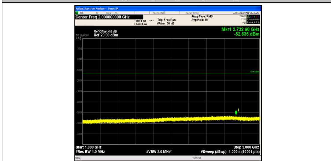
Band25_1.4MHz_16QAM_26683_1RB#0_1000~3000_1000~3000
