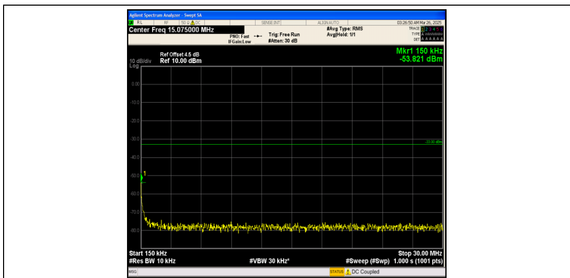
Band25_1.4MHz_QPSK_26365_1RB#0_0.15~30_0.15~30
