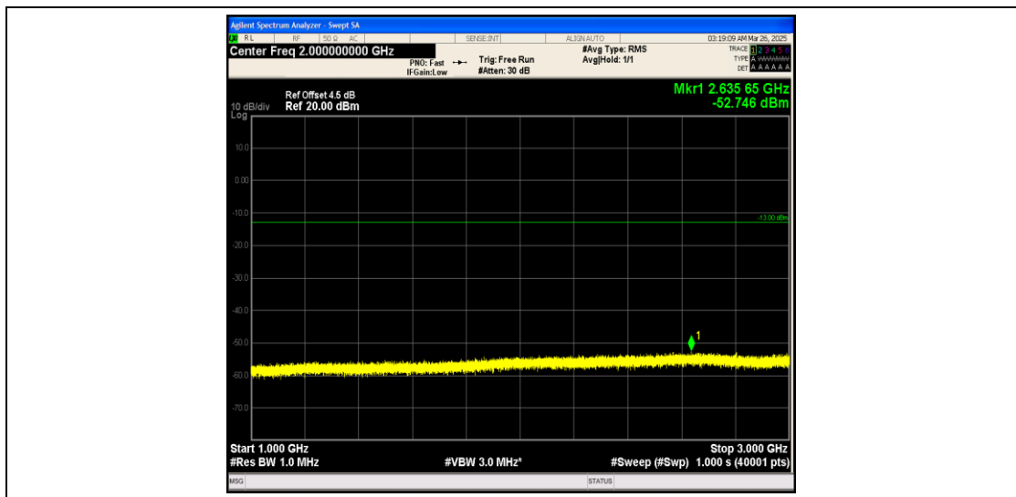
Band25_1.4MHz_16QAM_26047_1RB#0_1000~3000_1000~3000
