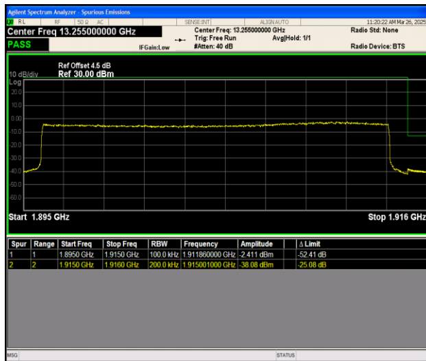
Band25_20MHz_16QAM_26590_100RB#0
