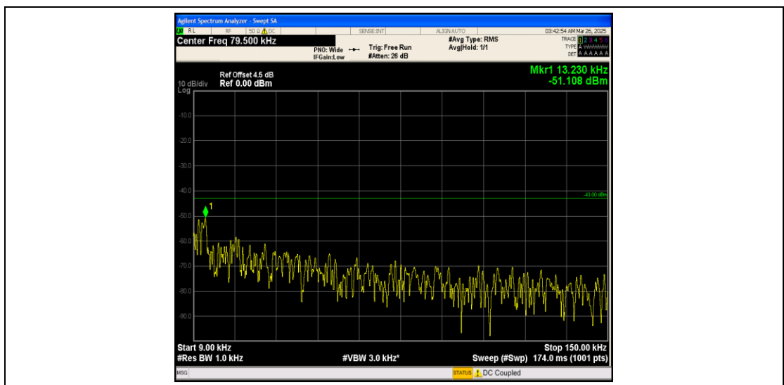
Band25_1.4MHz_QPSK_26683_1RB#0_0.009~0.15_0.009~0.15
