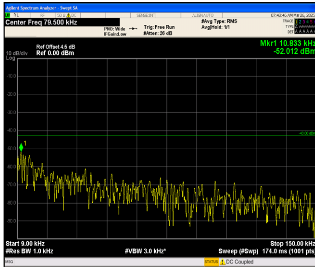
Band25_3MHz_QPSK_26675_1RB#0_0.009~0.15_0.009~0.15
