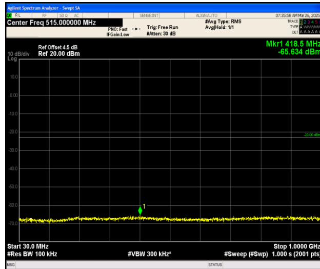
Band25_3MHz_16QAM_26365_1RB#0_30~1000_30~1000
