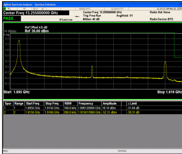
Band25_20MHz_16QAM_26590_1RB#0
