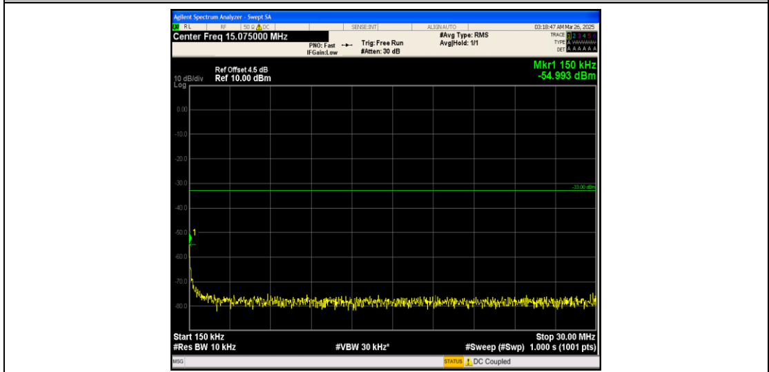
Band25_1.4MHz_16QAM_26047_1RB#0_0.15~30_0.15~30
