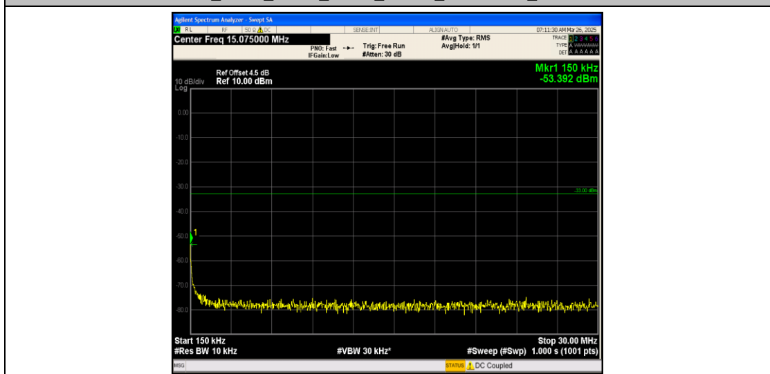
Band25_3MHz_QPSK_26055_1RB#0_0.15~30_0.15~30
