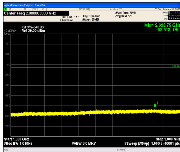
Band25_3MHz_16QAM_26365_1RB#0_1000~3000_1000~3000
