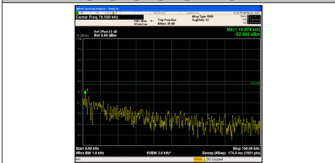
Band25_3MHz_16QAM_26675_1RB#0_0.009~0.15_0.009~0.15
