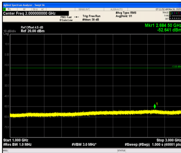
Band25_3MHz_QPSK_26055_1RB#0_1000~3000_1000~3000
