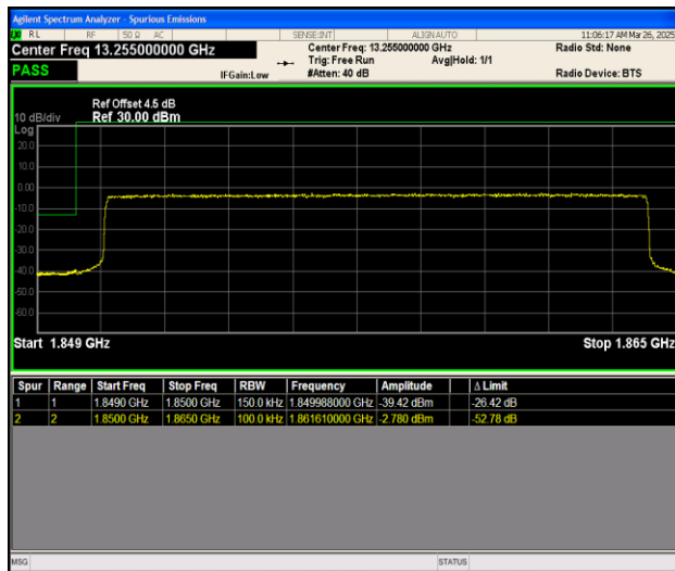
Band25_15MHz_16QAM_26115_75RB#0
