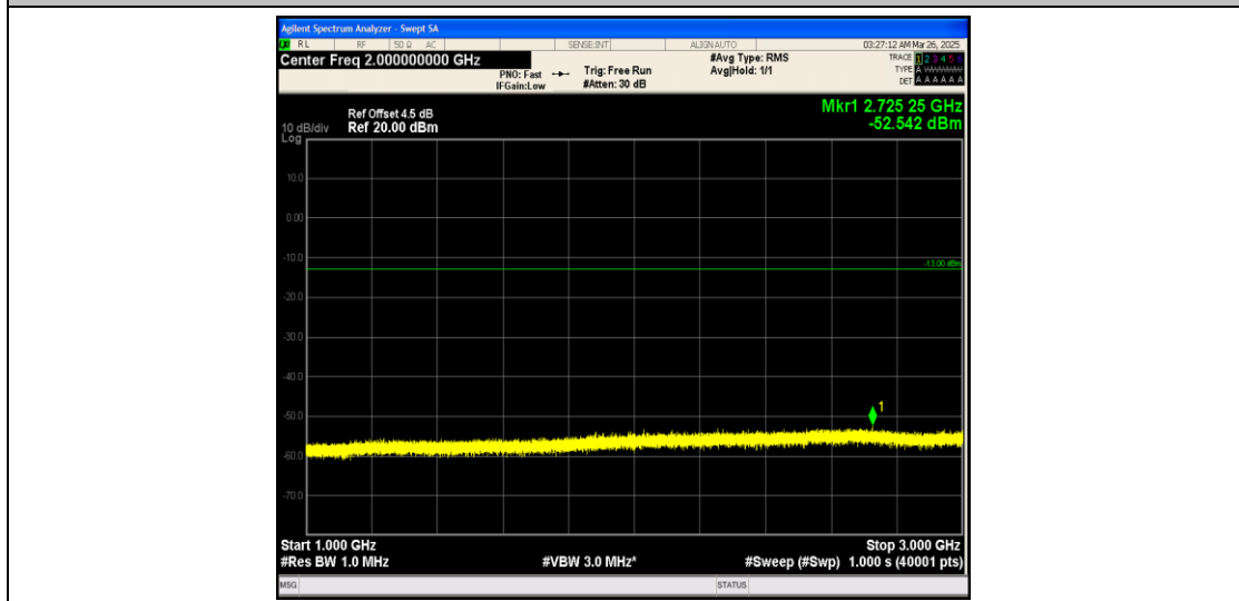
Band25_1.4MHz_QPSK_26365_1RB#0_1000~3000_1000~3000
