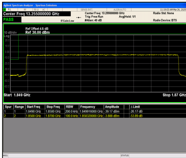
Band25_20MHz_16QAM_26140_100RB#0
