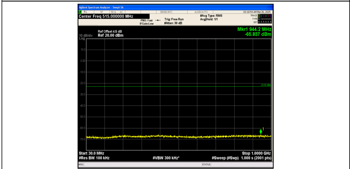
Band25_1.4MHz_16QAM_26047_1RB#0_30~1000_30~1000
