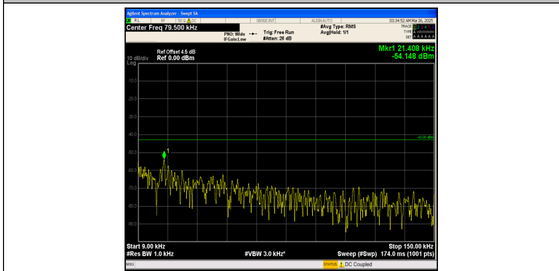
Band25_1.4MHz_16QAM_26365_1RB#0_0.009~0.15_0.009~0.15
