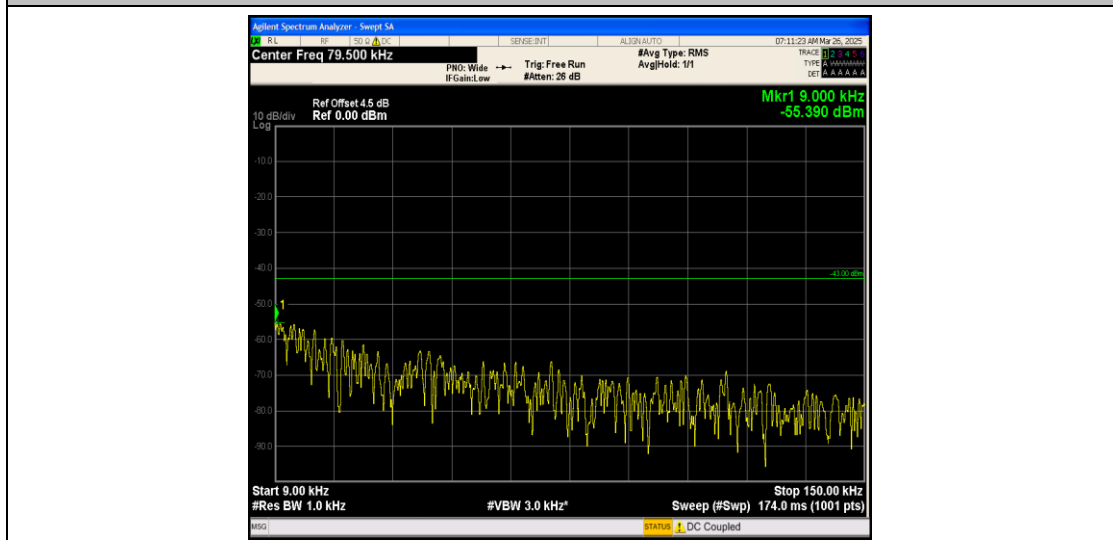
Band25_3MHz_QPSK_26055_1RB#0_0.009~0.15_0.009~0.15
