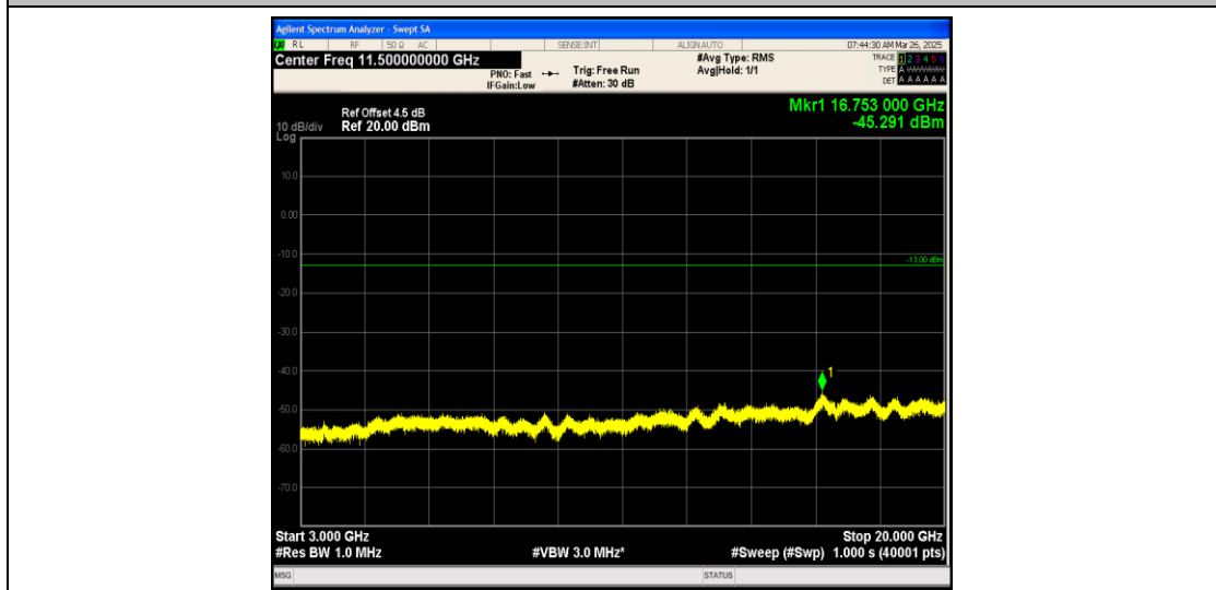
Band25_3MHz_QPSK_26675_1RB#0_3000~20000_3000~20000
