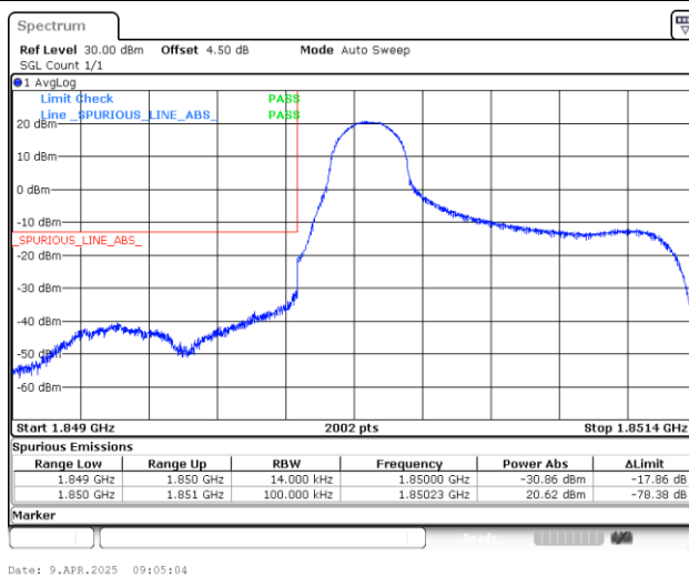
Band25_1.4MHz_QPSK_26047_1RB#0
