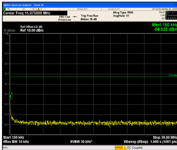
Band25_3MHz_QPSK_26675_1RB#0_0.15~30_0.15~30
