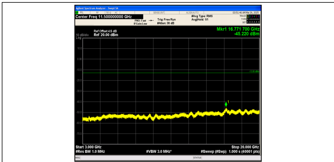
Band25_1.4MHz_16QAM_26683_1RB#0_3000~20000_3000~20000
