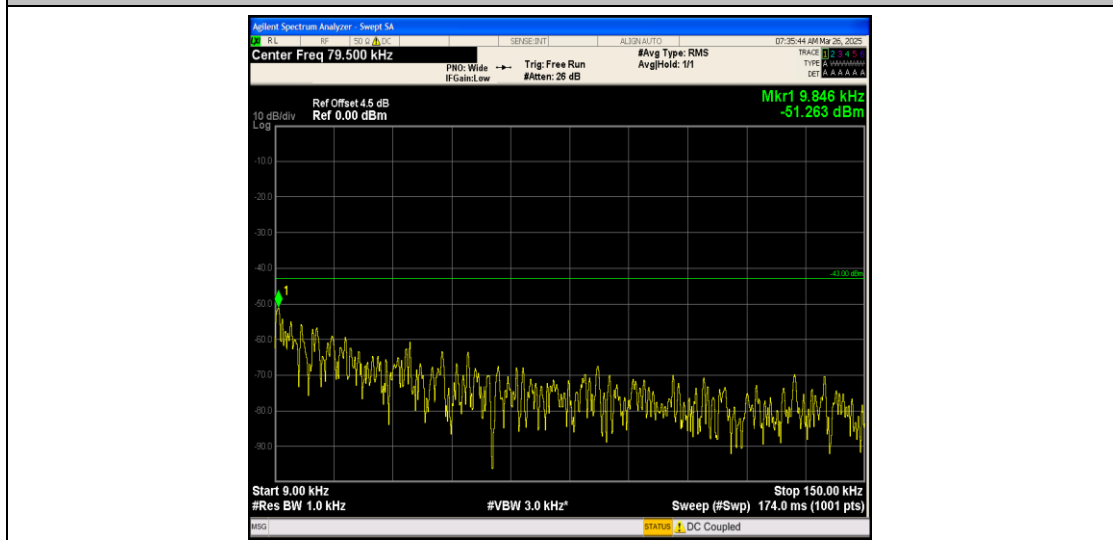
Band25_3MHz_16QAM_26365_1RB#0_0.009~0.15_0.009~0.15
