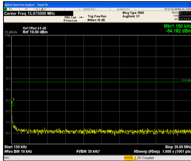
Band25_3MHz_QPSK_26365_1RB#0_0.15~30_0.15~30
