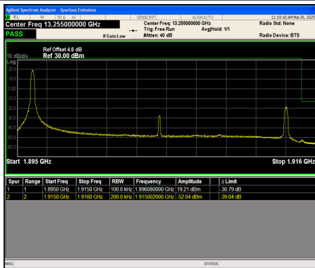
Band25_20MHz_QPSK_26590_1RB#0
