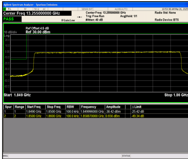
Band25_10MHz_QPSK_26090_50RB#0
