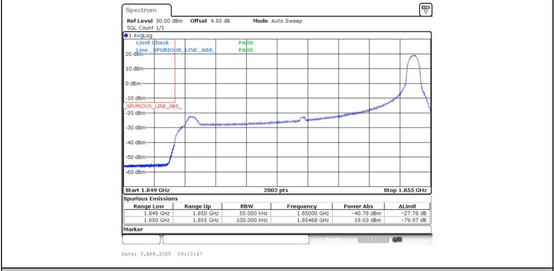
Band25_5MHz_16QAM_26065_1RB#24
