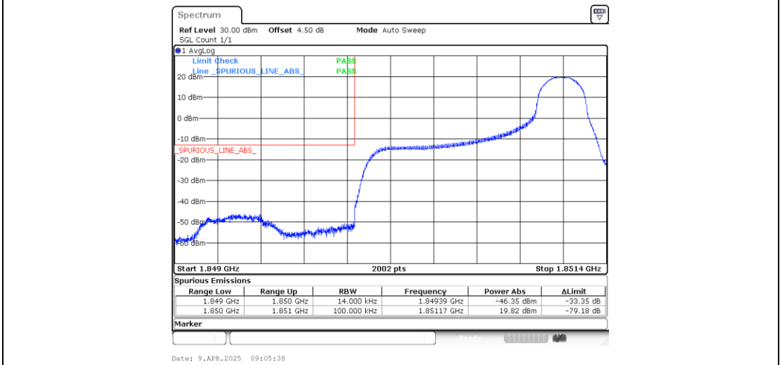
Band25_1.4MHz_16QAM_26047_1RB#5
