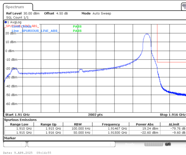
Band25_5MHz_16QAM_26665_1RB#24
