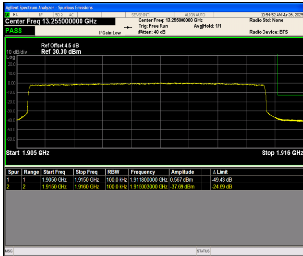
Band25_10MHz_QPSK_26640_50RB#0
