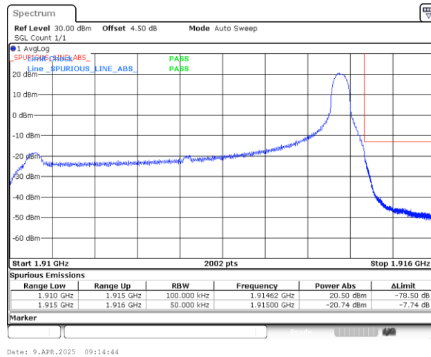
Band25_5MHz_QPSK_26665_1RB#24
