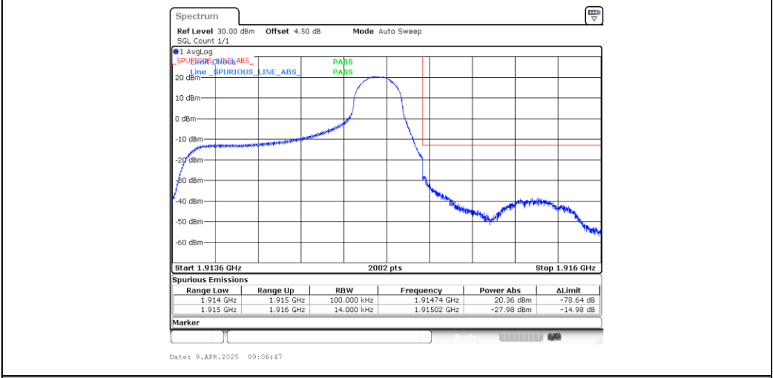
Band25_1.4MHz_QPSK_26683_1RB#5
