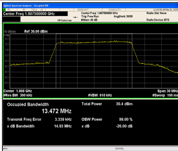
Band25-15MHz-16QAM-26615-75RB#0-PASS
