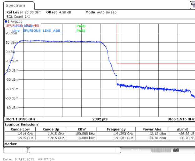
Band25_1.4MHz_QPSK_26683_6RB#0
