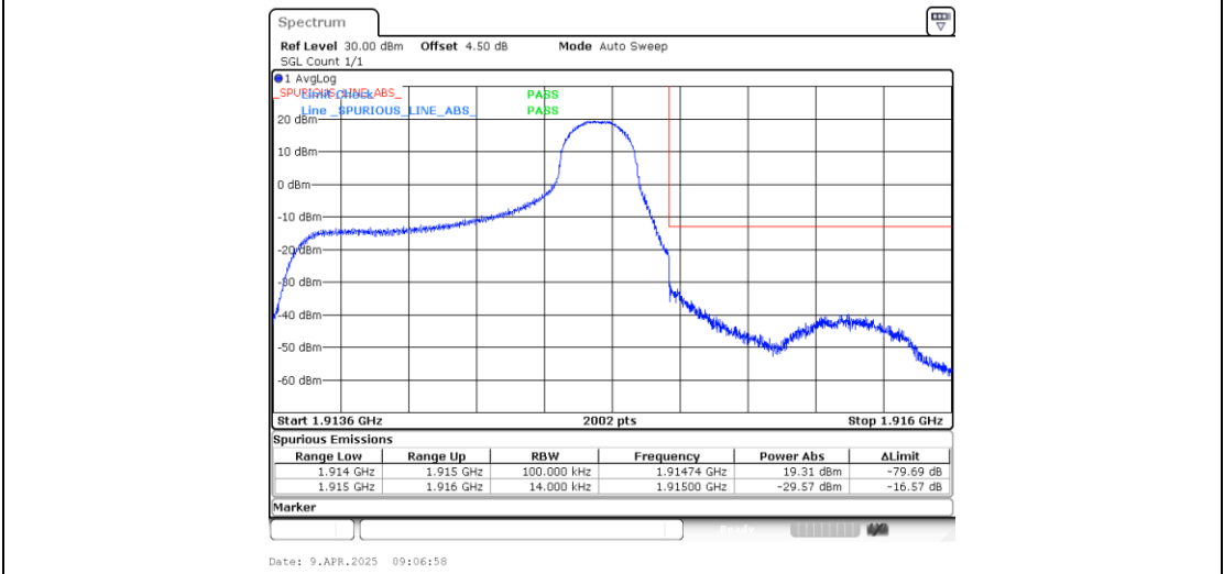
Band25_1.4MHz_16QAM_26683_1RB#5
