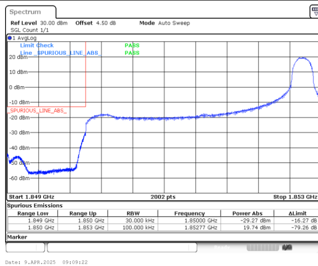
Band25_3MHz_16QAM_26055_1RB#14
