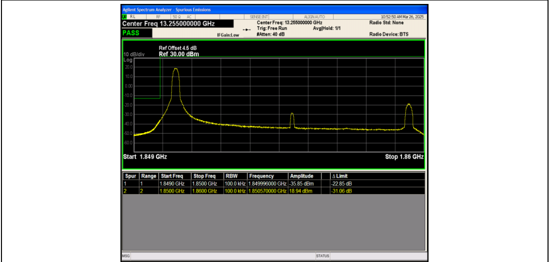
Band25_10MHz_QPSK_26090_1RB#0
