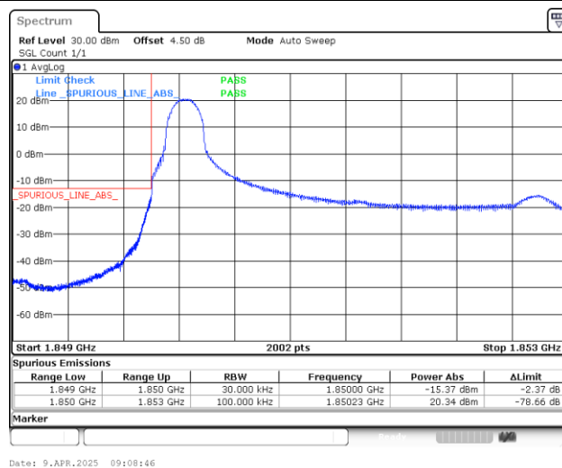
Band25_3MHz_QPSK_26055_1RB#0
