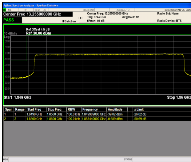
Band25_10MHz_16QAM_26090_50RB#0
