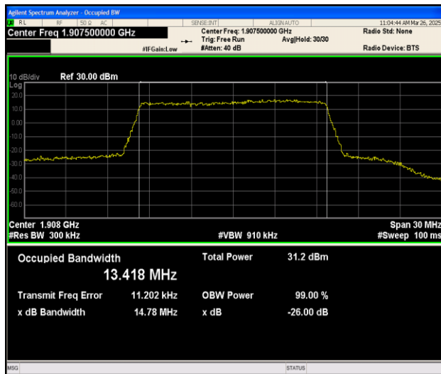
Band25-15MHz-QPSK-26615-75RB#0-PASS
