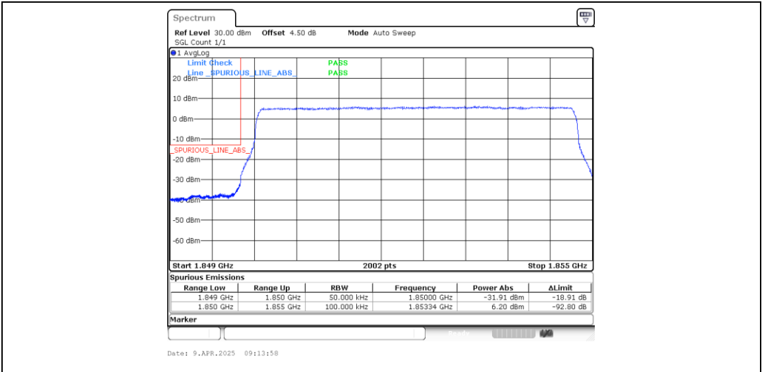
Band25_5MHz_QPSK_26065_25RB#0
