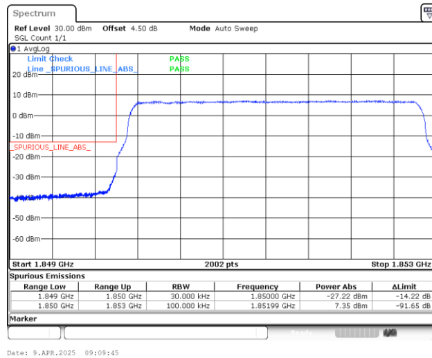
Band25_3MHz_16QAM_26055_15RB#0
