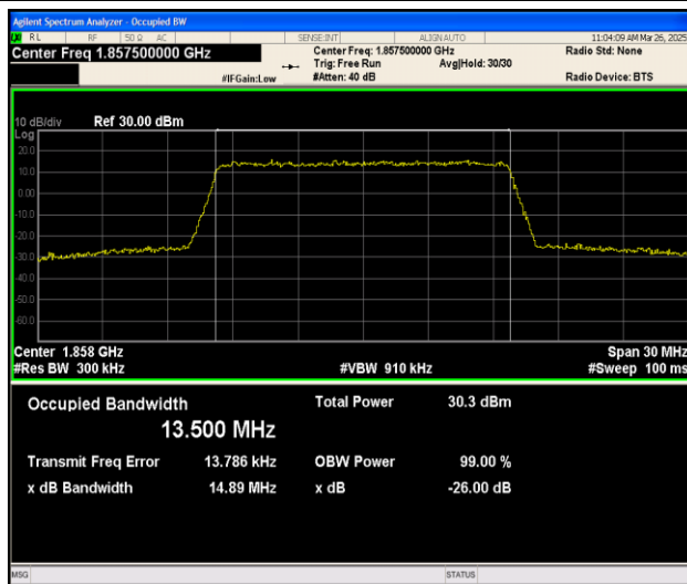
Band25-15MHz-16QAM-26115-75RB#0-PASS
