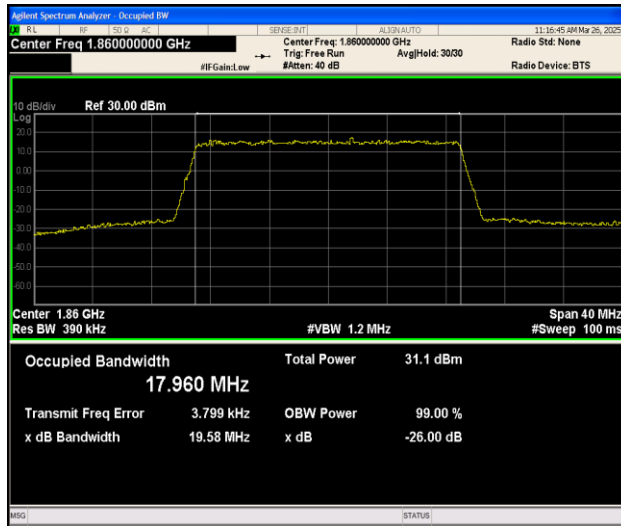
Band25-20MHz-QPSK-26140-100RB#0-PASS
