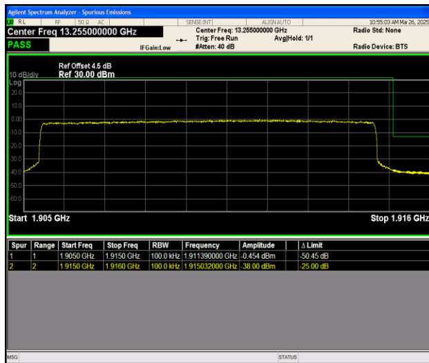
Band25_10MHz_16QAM_26640_50RB#0
