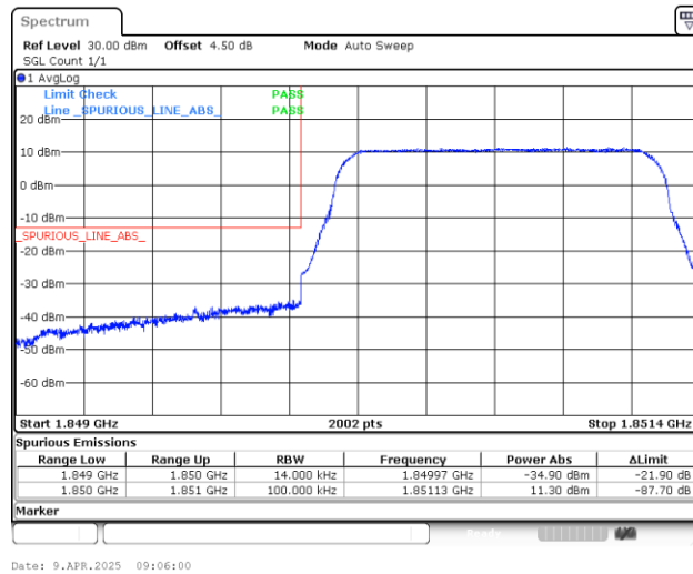
Band25_1.4MHz_16QAM_26047_6RB#0
