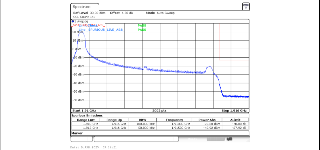
Band25_5MHz_QPSK_26665_1RB#0
