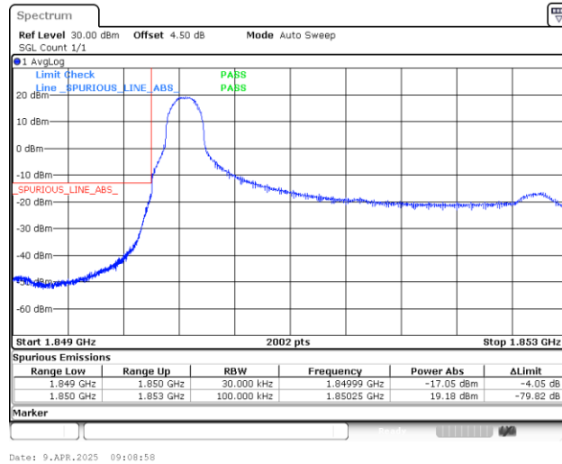
Band25_3MHz_16QAM_26055_1RB#0
