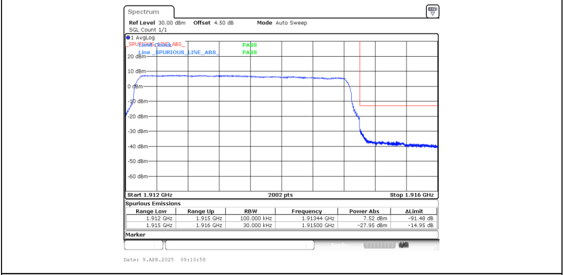
Band25_3MHz_16QAM_26675_15RB#0
