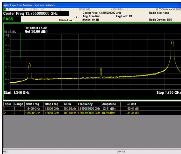
Band25_15MHz_QPSK_26115_1RB#74
