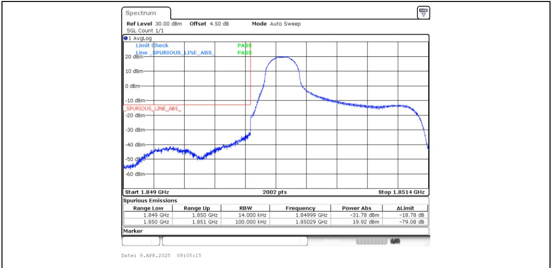
Band25_1.4MHz_16QAM_26047_1RB#0
