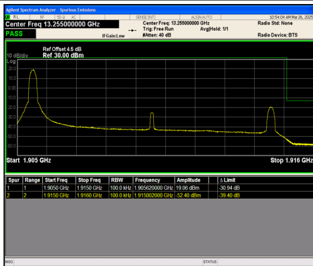
Band25_10MHz_QPSK_26640_1RB#0
