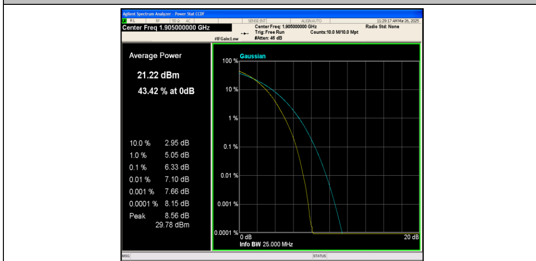
Band25-20MHz-16QAM-26590-100RB#0-PASS
