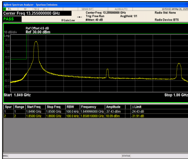
Band25_10MHz_16QAM_26090_1RB#0
