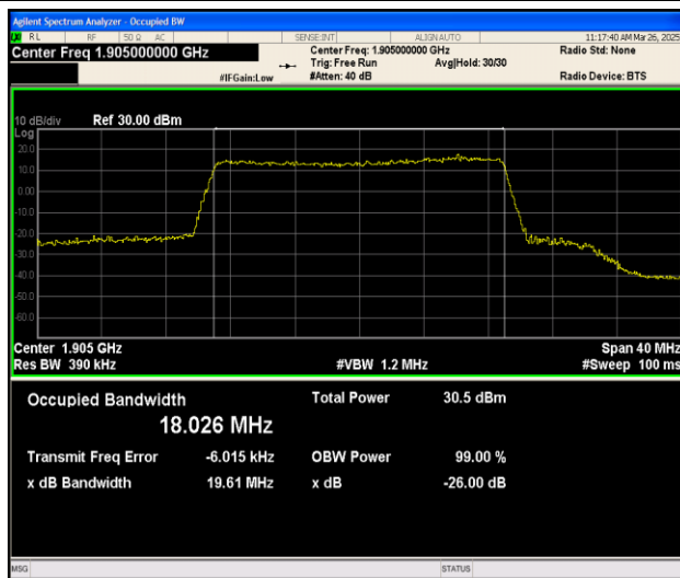
Band25-20MHz-16QAM-26590-100RB#0-PASS
