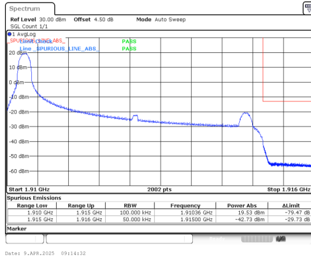
Band25_5MHz_16QAM_26665_1RB#0
