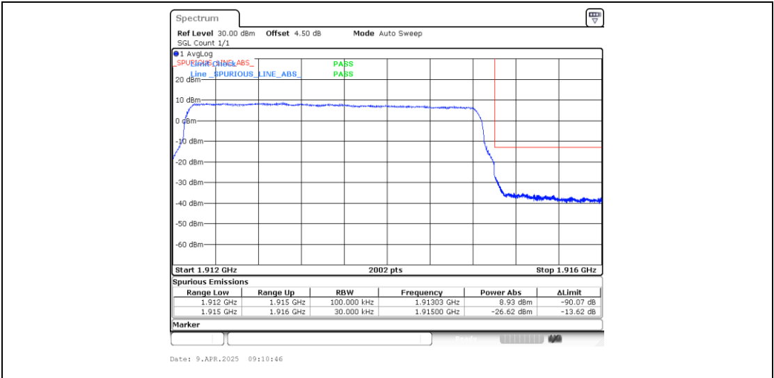
Band25_3MHz_QPSK_26675_15RB#0
