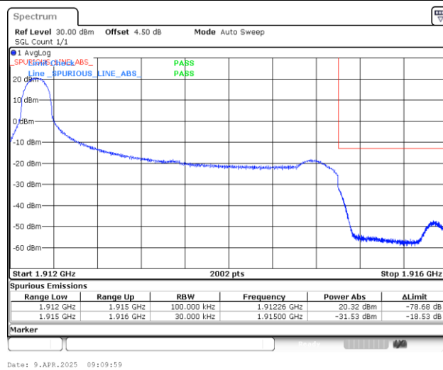
Band25_3MHz_QPSK_26675_1RB#0
