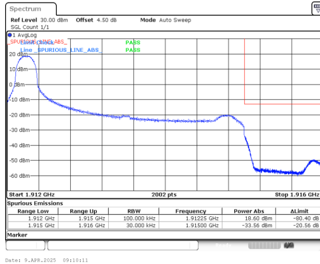
Band25_3MHz_16QAM_26675_1RB#0
