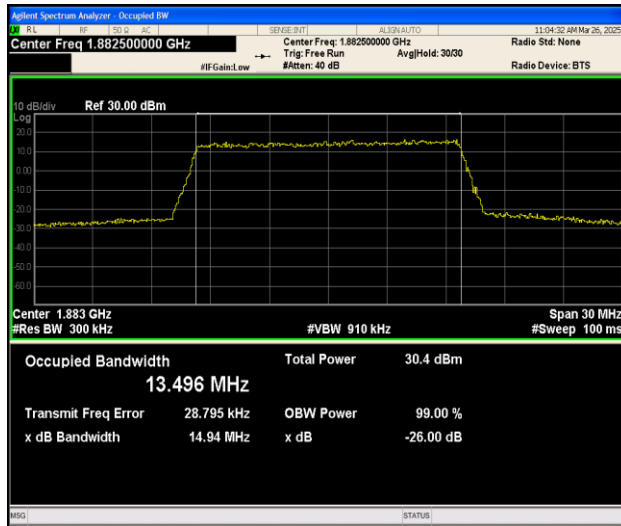
Band25-15MHz-16QAM-26365-75RB#0-PASS
