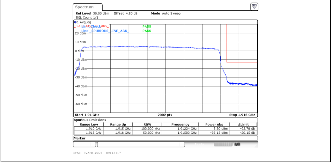
Band25_5MHz_16QAM_26665_25RB#0
