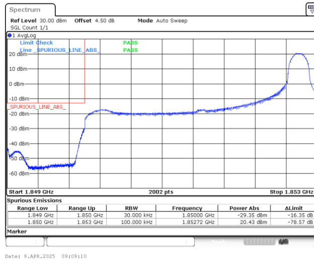
Band25_3MHz_QPSK_26055_1RB#14
