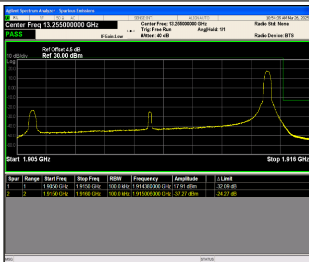
Band25_10MHz_16QAM_26640_1RB#49
