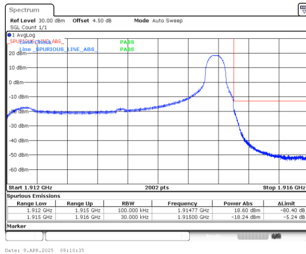
Band25_3MHz_16QAM_26675_1RB#14
