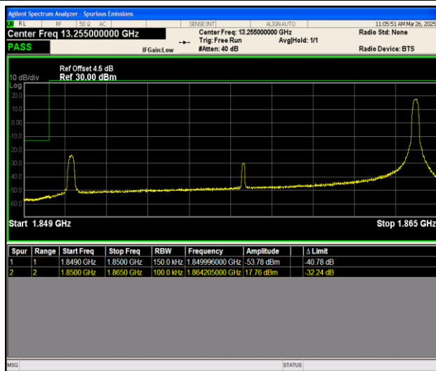
Band25_15MHz_16QAM_26115_1RB#74
