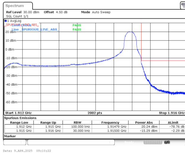
Band25_3MHz_QPSK_26675_1RB#14
