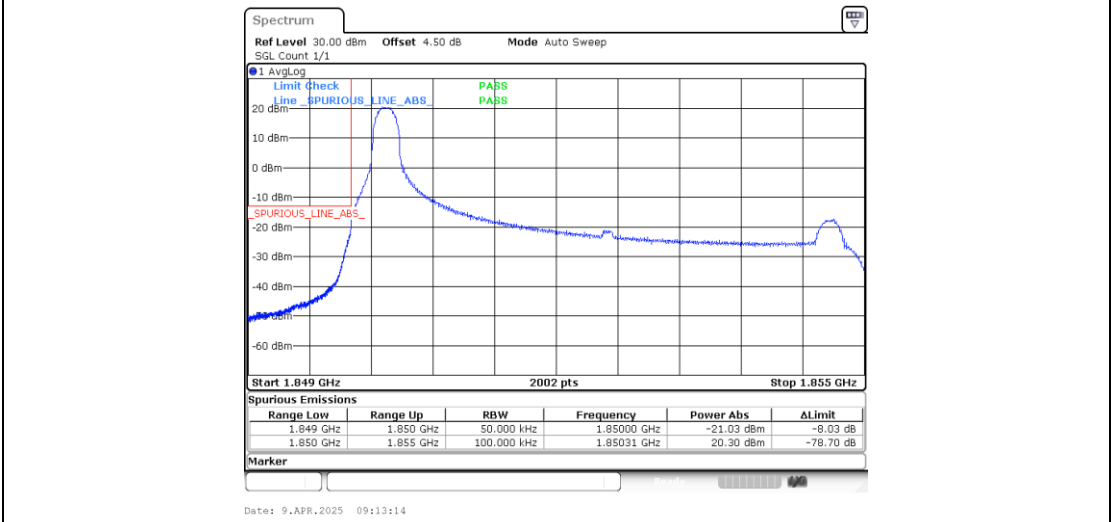
Band25_5MHz_QPSK_26065_1RB#0
