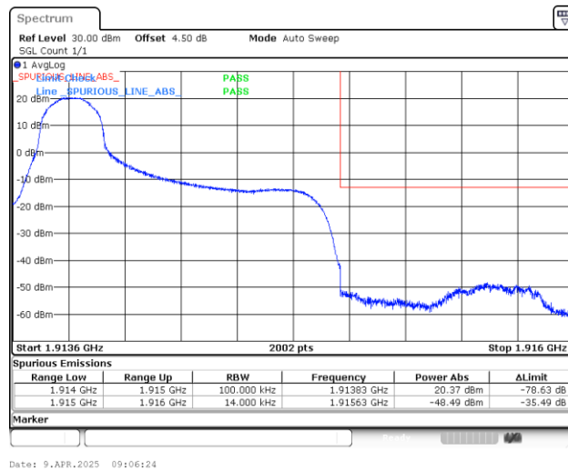
Band25_1.4MHz_QPSK_26683_1RB#0
