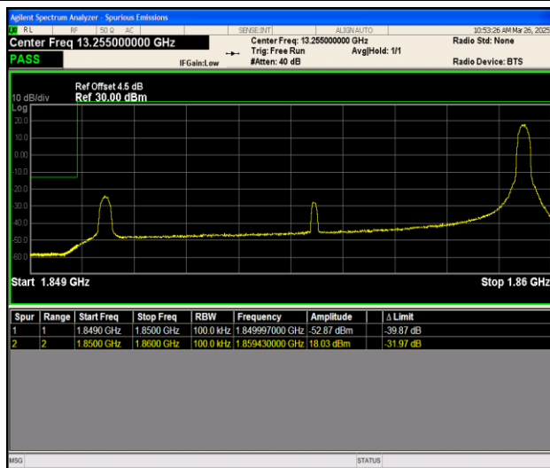
Band25_10MHz_16QAM_26090_1RB#49
