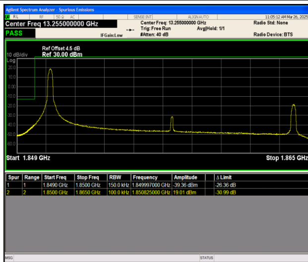
Band25_15MHz_QPSK_26115_1RB#0
