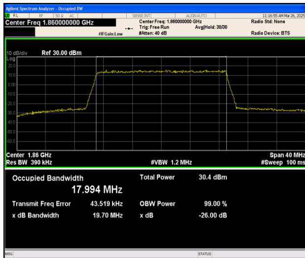
Band25-20MHz-16QAM-26140-100RB#0-PASS
