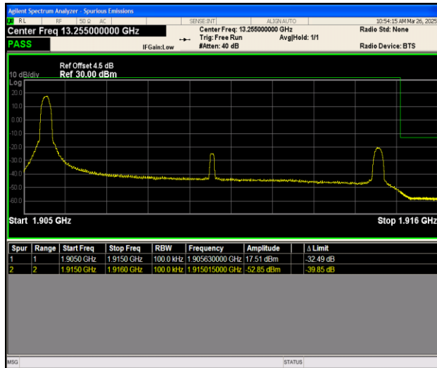
Band25_10MHz_16QAM_26640_1RB#0
