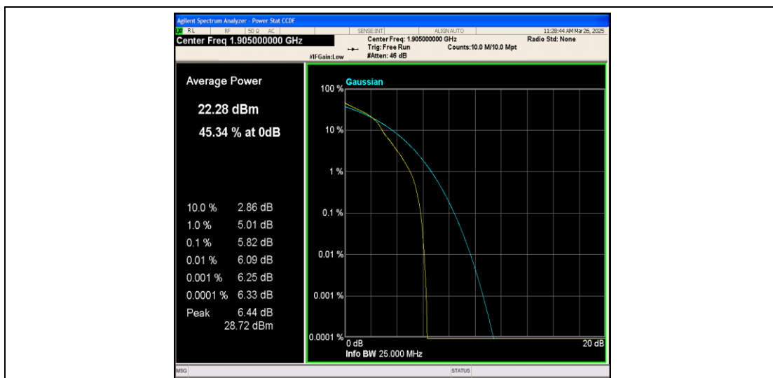
Band25-20MHz-16QAM-26590-1RB#0-PASS
