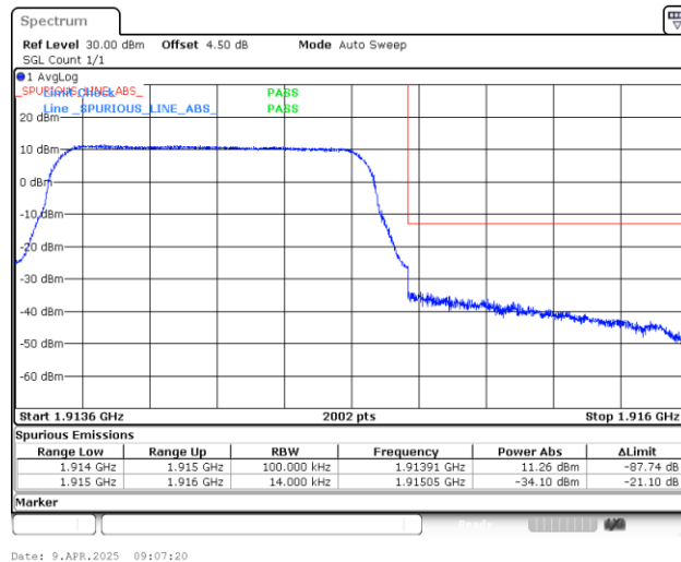
Band25_1.4MHz_16QAM_26683_6RB#0
