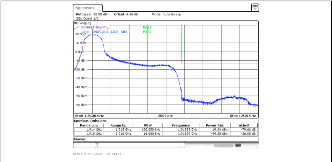
Band25_1.4MHz_16QAM_26683_1RB#0
