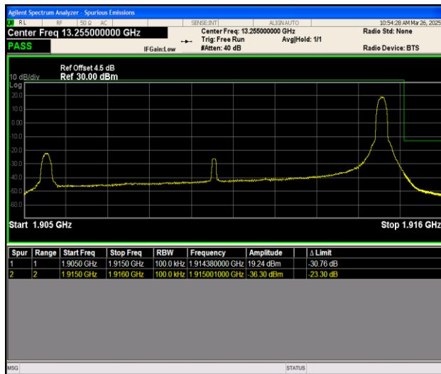
Band25_10MHz_QPSK_26640_1RB#49
