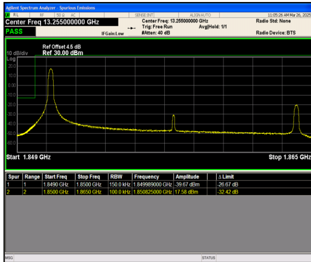
Band25_15MHz_16QAM_26115_1RB#0
