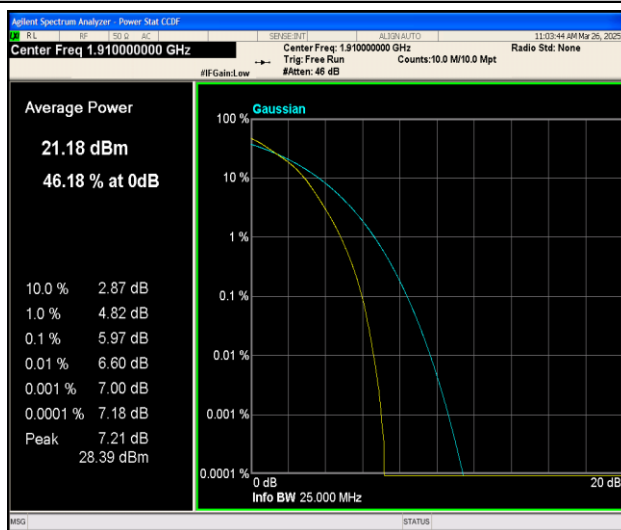
Band25-10MHz-16QAM-26640-50RB#0-PASS
