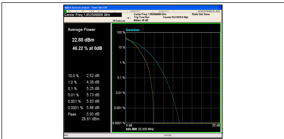
Band25-5MHz-QPSK-26065-1RB#0-PASS
