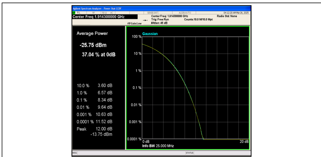
Band25-1.4MHz-16QAM-26683-1RB#0-PASS
