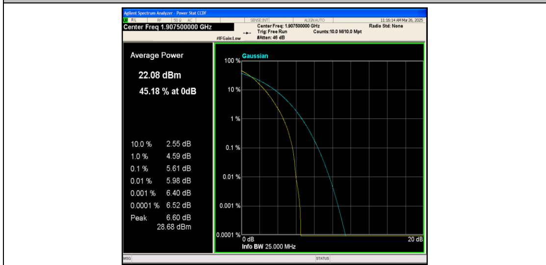
Band25-15MHz-QPSK-26615-75RB#0-PASS
