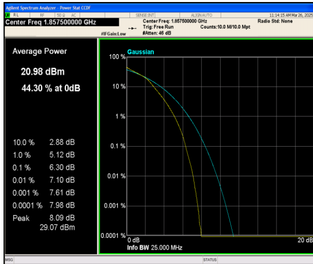
Band25-15MHz-16QAM-26115-75RB#0-PASS
