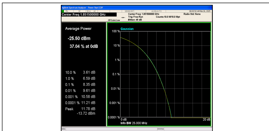
Band25-3MHz-16QAM-26055-15RB#0-PASS
