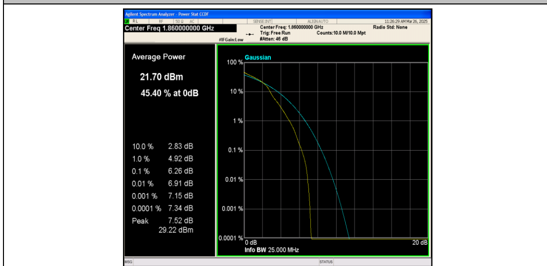
Band25-20MHz-16QAM-26140-1RB#0-PASS
