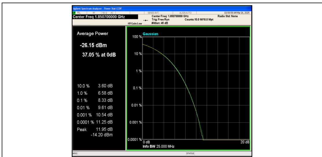
Band25-1.4MHz-16QAM-26047-6RB#0-PASS
