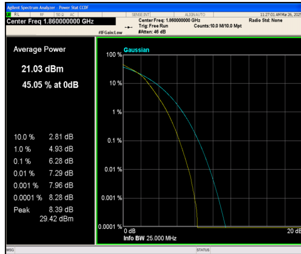
Band25-20MHz-16QAM-26140-100RB#0-PASS
