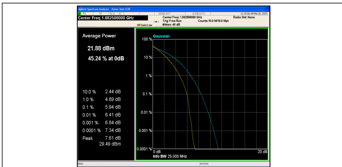
Band25-15MHz-QPSK-26365-75RB#0-PASS
