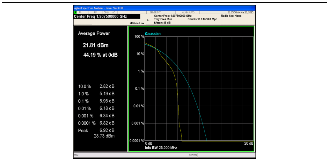
Band25-15MHz-16QAM-26615-1RB#0-PASS
