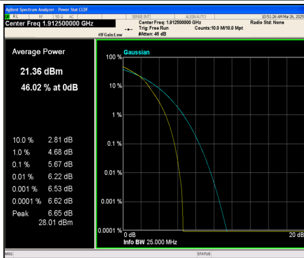
Band25-5MHz-16QAM-26665-25RB#0-PASS
