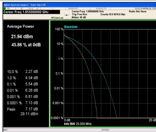
Band25-10MHz-QPSK-26090-50RB#0-PASS
