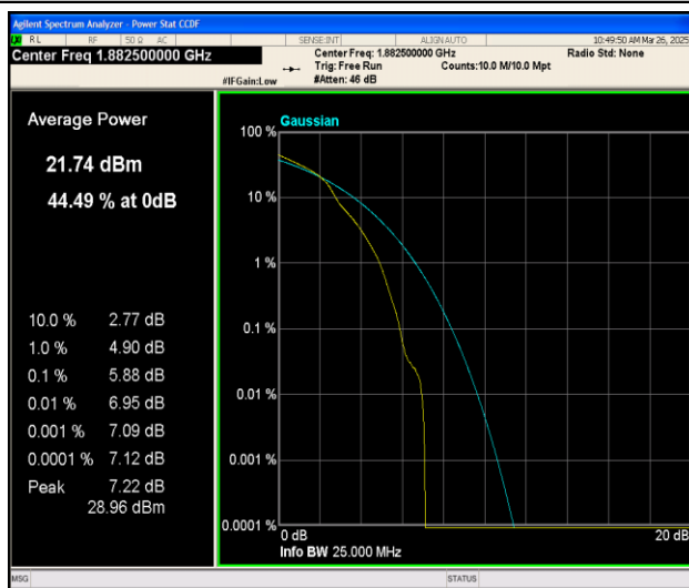
Band25-5MHz-16QAM-26365-1RB#0-PASS
