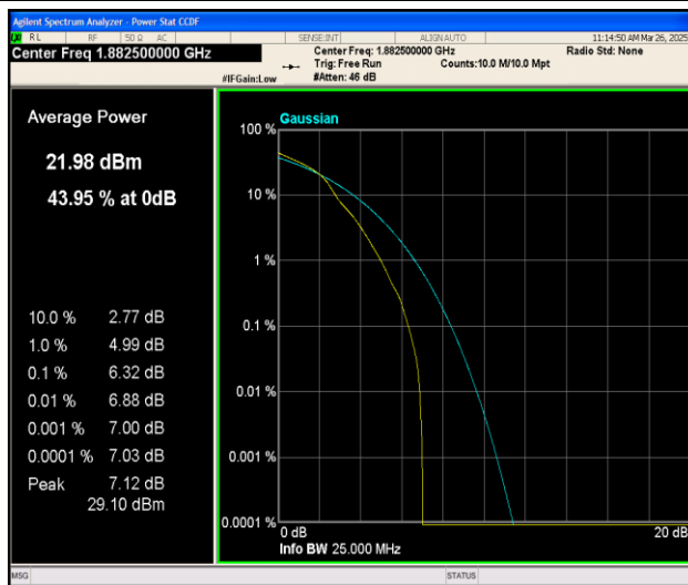
Band25-15MHz-16QAM-26365-1RB#0-PASS
