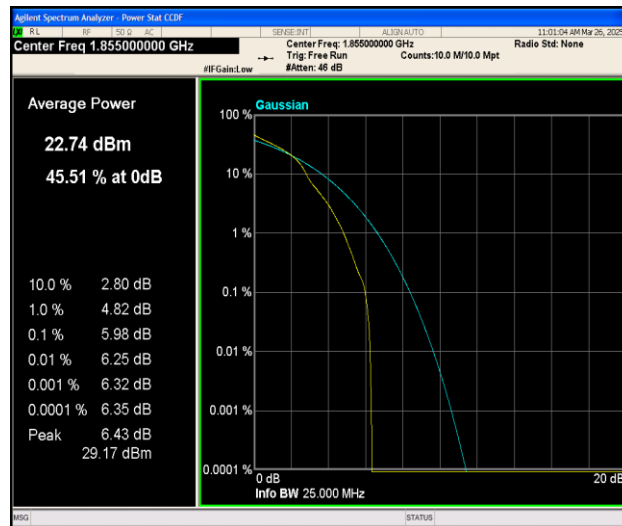
Band25-10MHz-16QAM-26090-1RB#0-PASS
