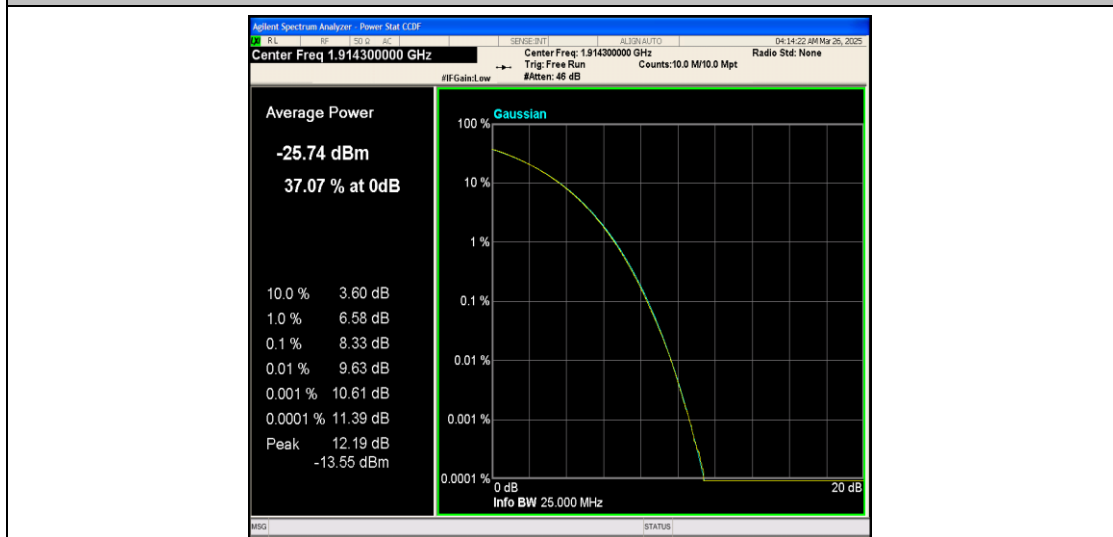
Band25-1.4MHz-QPSK-26683-6RB#0-PASS
