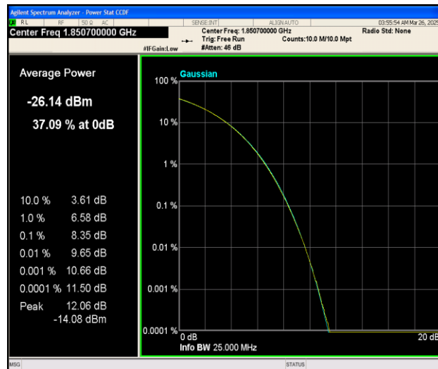
Band25-1.4MHz-16QAM-26047-1RB#0-PASS
