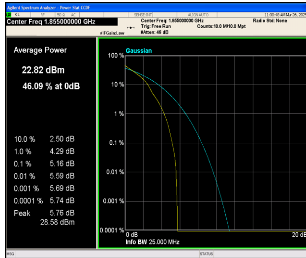
Band25-10MHz-QPSK-26090-1RB#0-PASS
