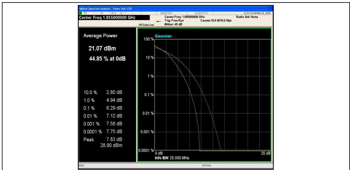
Band25-10MHz-16QAM-26090-50RB#0-PASS
