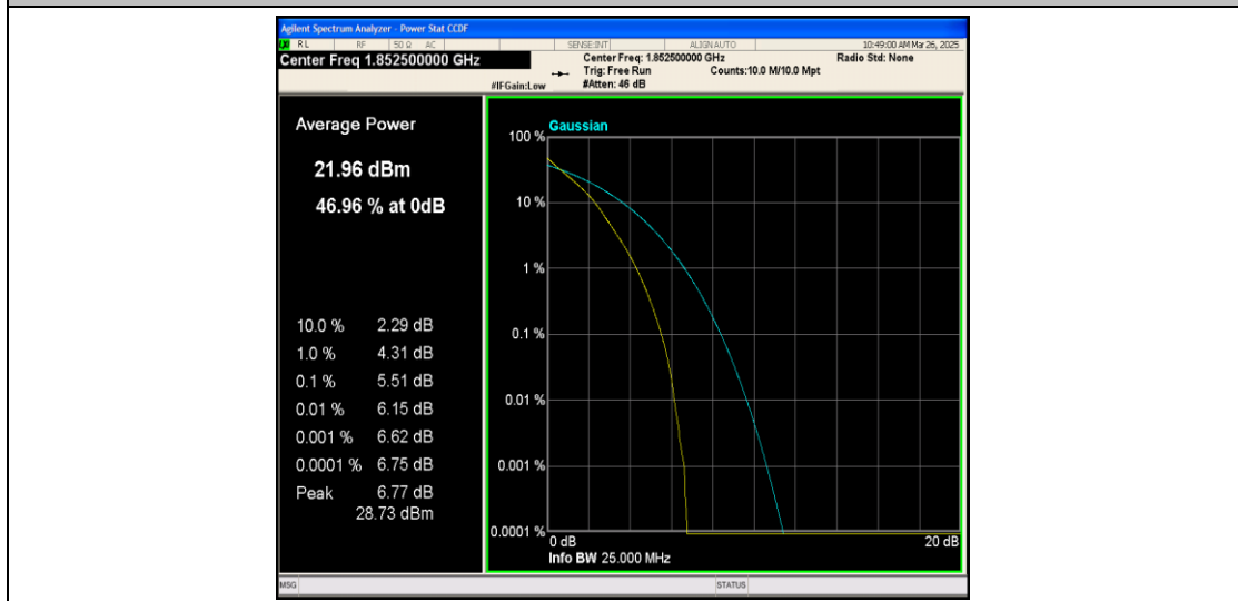
Band25-5MHz-QPSK-26065-25RB#0-PASS
