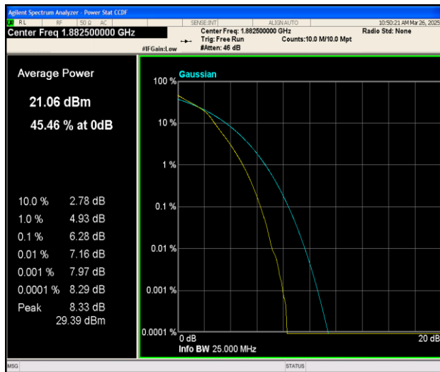
Band25-5MHz-16QAM-26365-25RB#0-PASS
