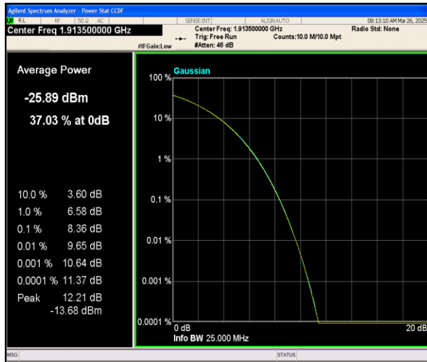
Band25-3MHz-16QAM-26675-1RB#0-PASS
