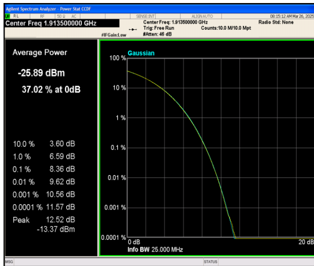
Band25-3MHz-QPSK-26675-15RB#0-PASS
