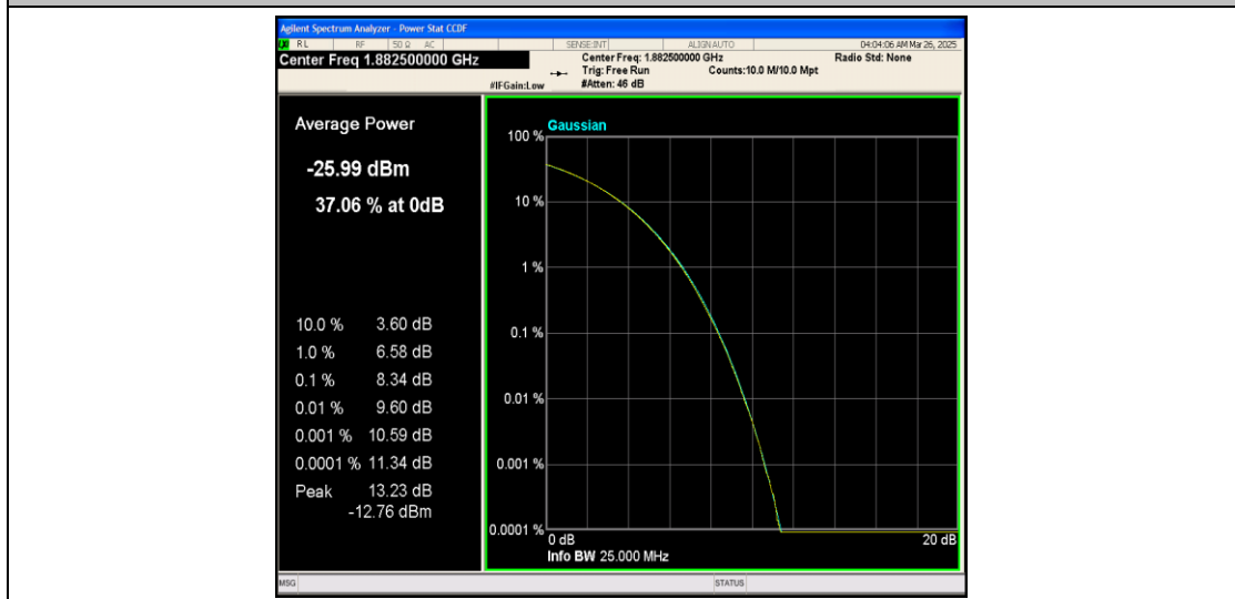
Band25-1.4MHz-16QAM-26365-1RB#0-PASS
