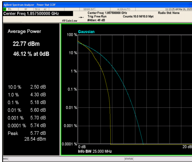
Band25-15MHz-QPSK-26115-1RB#0-PASS
