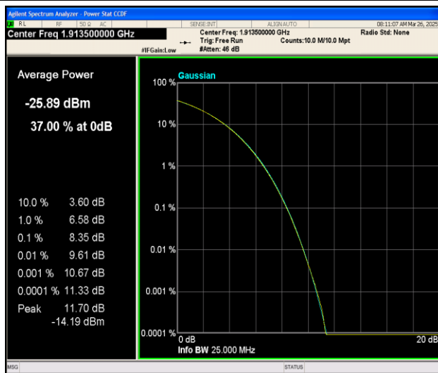
Band25-3MHz-QPSK-26675-1RB#0-PASS
