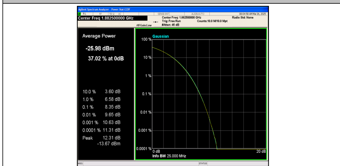
Band25-3MHz-16QAM-26365-1RB#0-PASS
