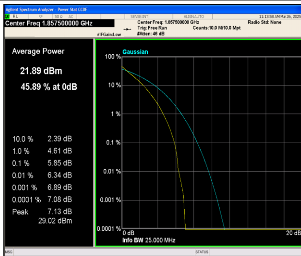
Band25-15MHz-QPSK-26115-75RB#0-PASS
