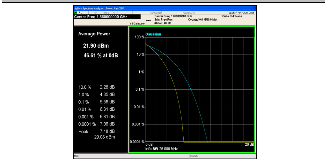
Band25-20MHz-QPSK-26140-100RB#0-PASS
