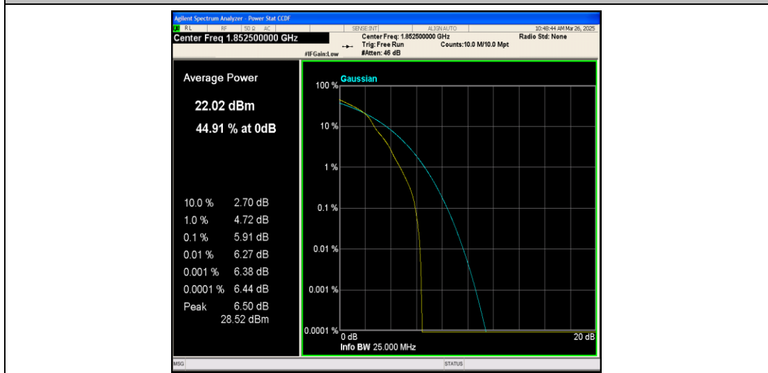
Band25-5MHz-16QAM-26065-1RB#0-PASS
