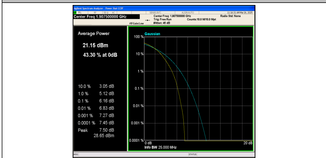
Band25-15MHz-16QAM-26615-75RB#0-PASS
