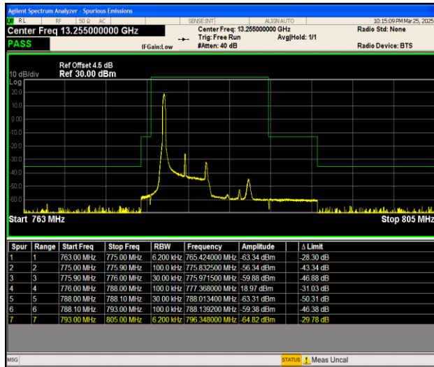
Band13_5MHz_16QAM_23205_1RB#0
