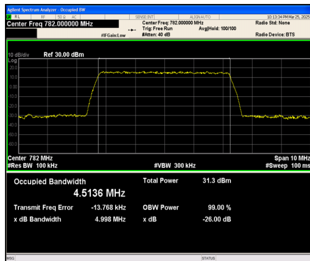
Band13-5MHz-QPSK-23230-25RB#0-PASS
