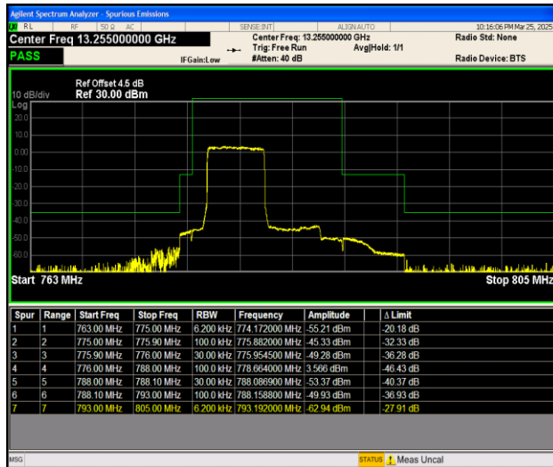
Band13_5MHz_QPSK_23205_25RB#0
