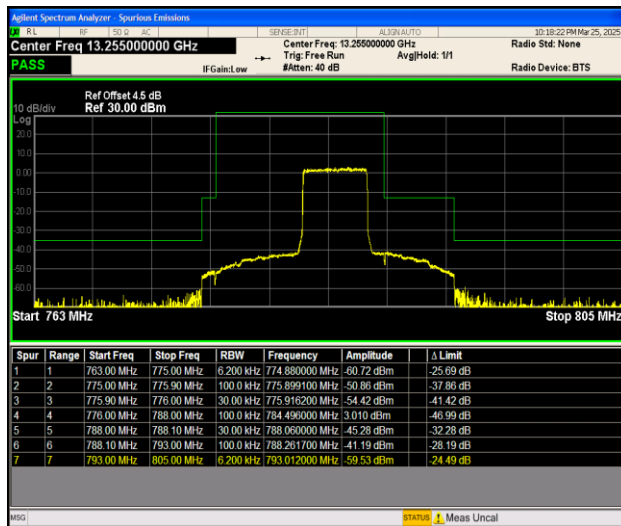
Band13_5MHz_16QAM_23255_25RB#0
