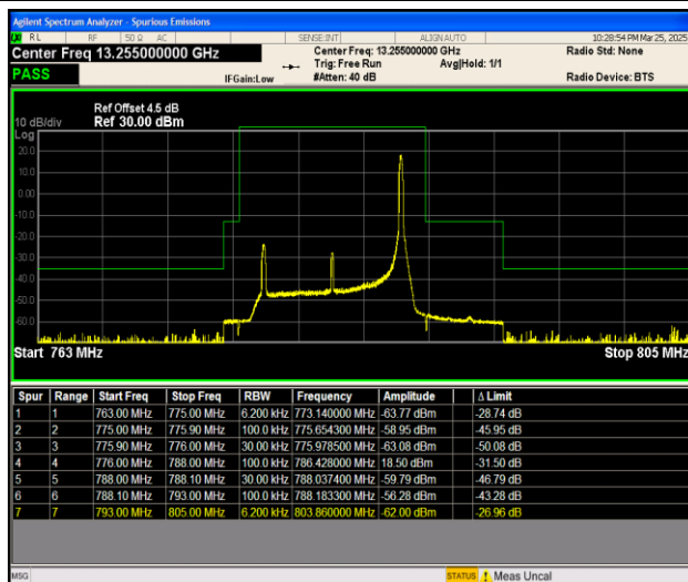
Band13_10MHz_16QAM_23230_1RB#49
