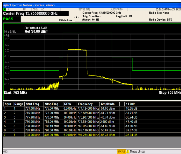
Band13_5MHz_16QAM_23205_25RB#0
