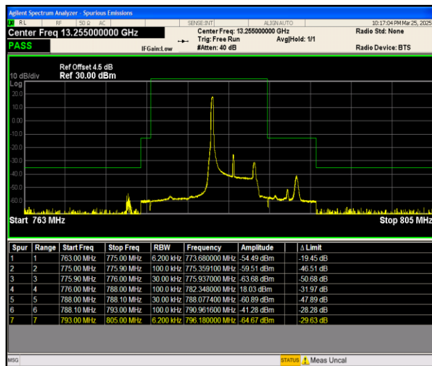
Band13_5MHz_16QAM_23255_1RB#0
