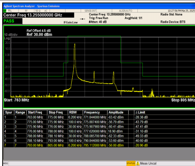
Band13_10MHz_QPSK_23230_1RB#0
