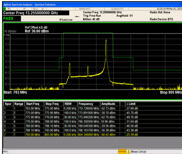
Band13_10MHz_QPSK_23230_1RB#49
