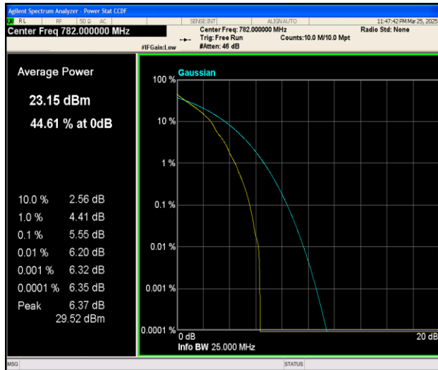
Band13-10MHz-QPSK-23230-1RB#0-PASS
