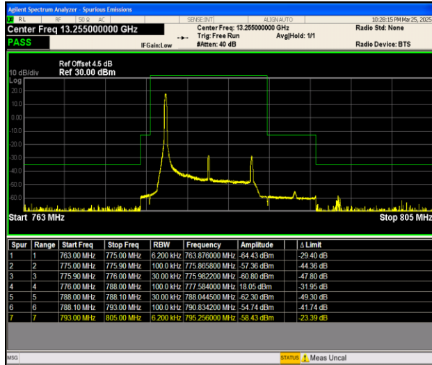
Band13_10MHz_16QAM_23230_1RB#0
