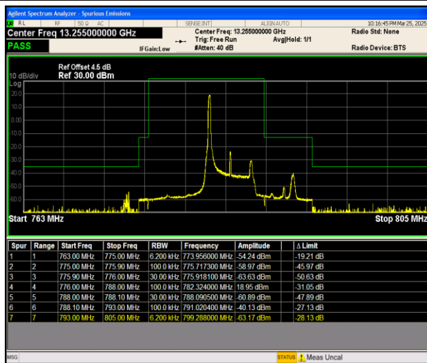
Band13_5MHz_QPSK_23255_1RB#0
