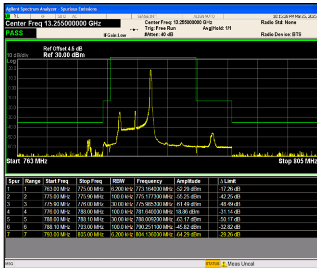
Band13_5MHz_QPSK_23205_1RB#24
