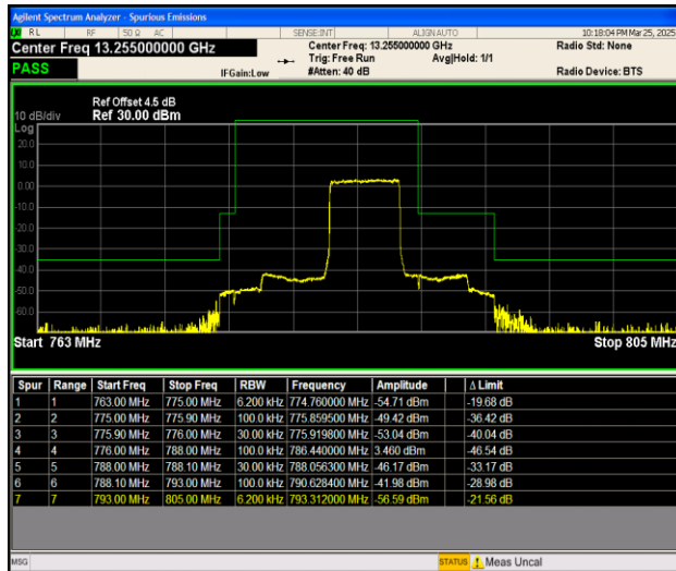
Band13_5MHz_QPSK_23255_25RB#0
