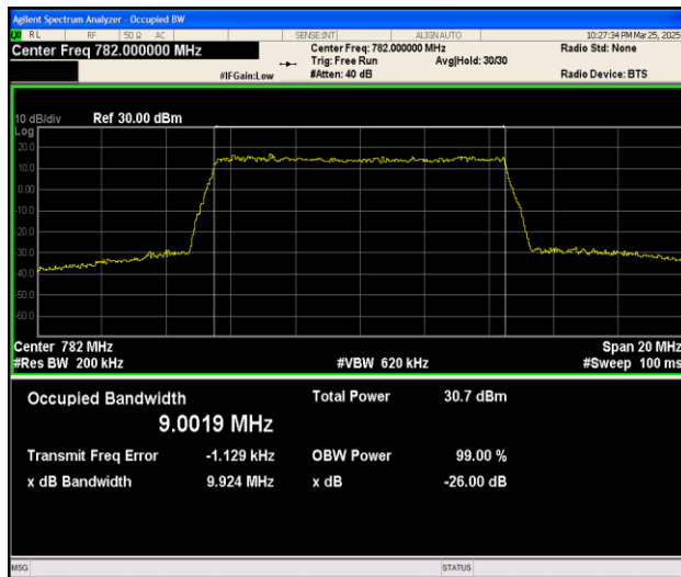
Band13-10MHz-16QAM-23230-50RB#0-PASS
