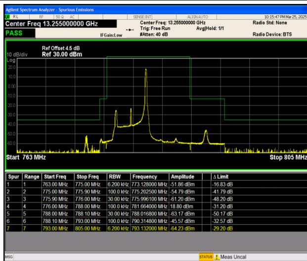
Band13_5MHz_16QAM_23205_1RB#24
