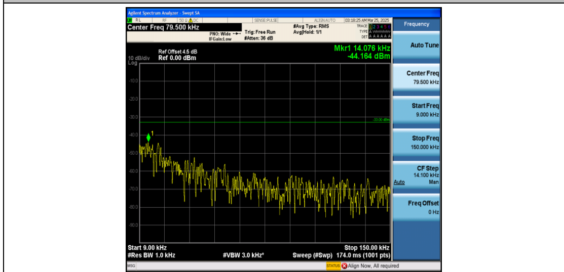
Band12_3MHz_QPSK_23165_1RB#0_0.009~0.15_0.009~0.15
