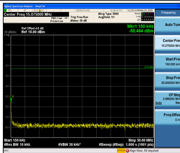
Band12_1.4MHz_16QAM_23173_1RB#0_0.15~30_0.15~30
