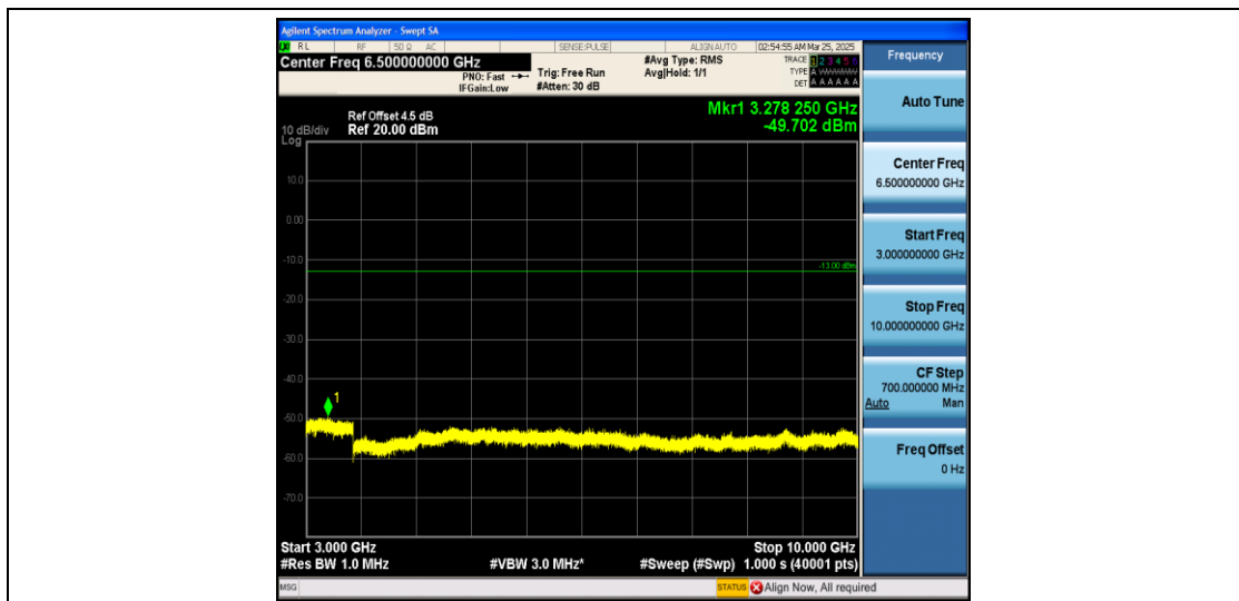
Band12_3MHz_16QAM_23025_1RB#0_3000~10000_3000~10000
