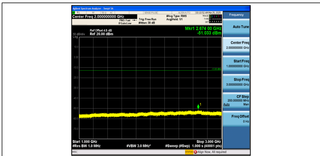
Band12_3MHz_16QAM_23095_1RB#0_1000~3000_1000~3000
