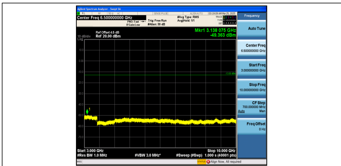
Band12_3MHz_QPSK_23165_1RB#0_3000~10000_3000~10000
