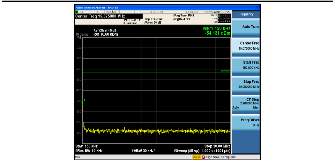
Band12_3MHz_QPSK_23095_1RB#0_0.15~30_0.15~30
