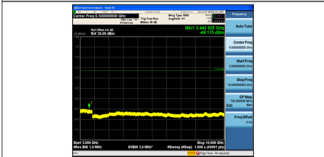
Band12_3MHz_16QAM_23095_1RB#0_3000~10000_3000~10000
