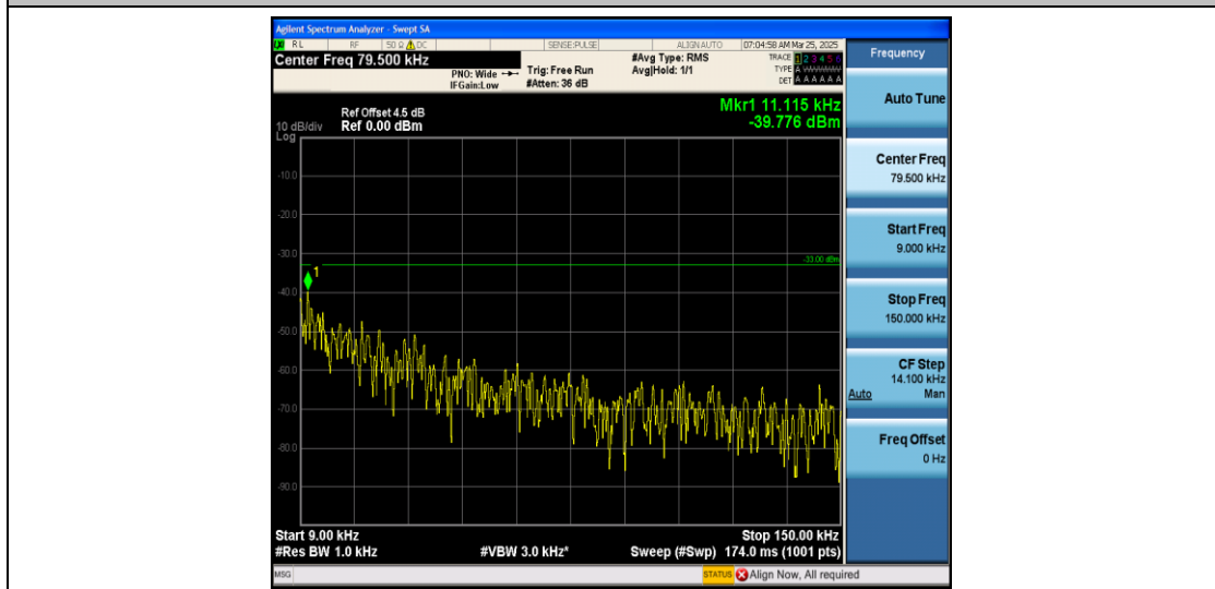
Band12_5MHz_QPSK_23095_1RB#0_0.009~0.15_0.009~0.15
