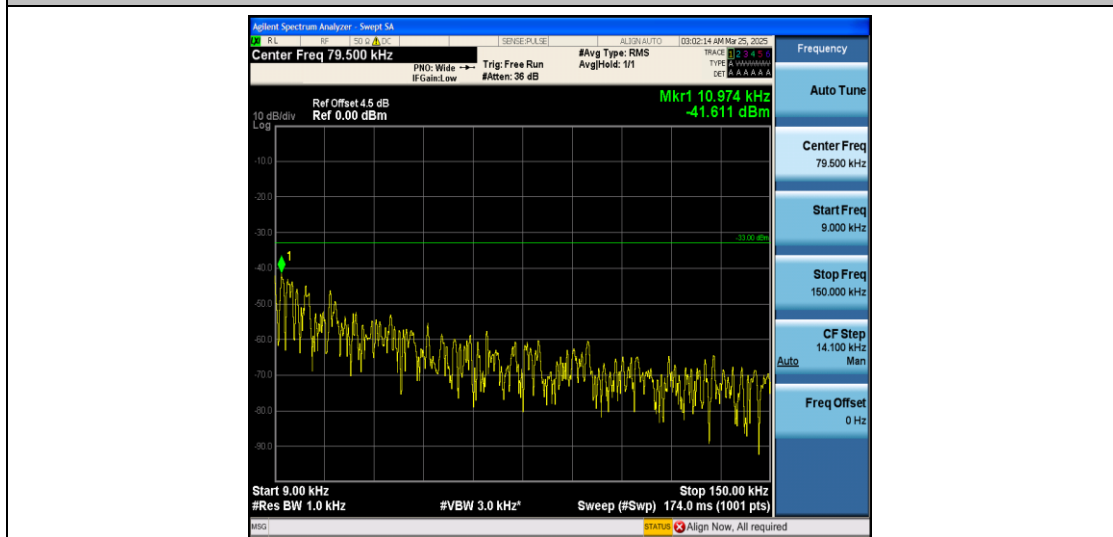
Band12_3MHz_QPSK_23095_1RB#0_0.009~0.15_0.009~0.15
