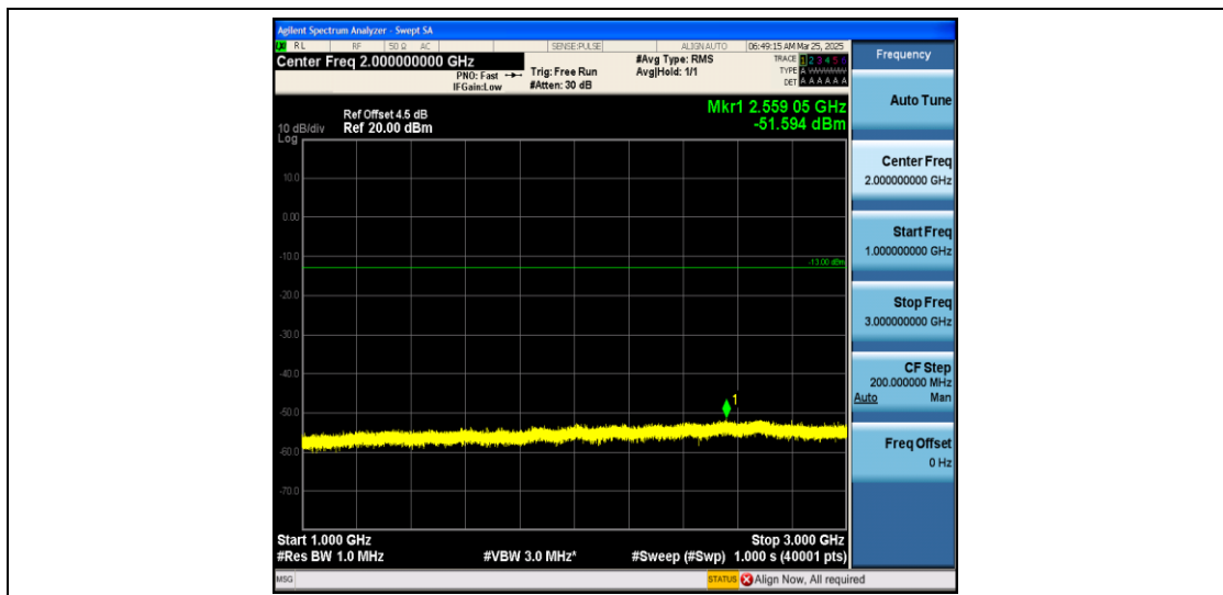
Band12_5MHz_QPSK_23035_1RB#0_1000~3000_1000~3000
