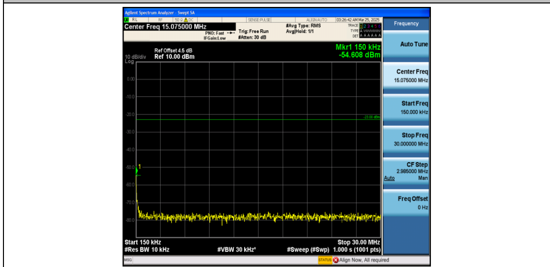
Band12_3MHz_16QAM_23165_1RB#0_0.15~30_0.15~30
