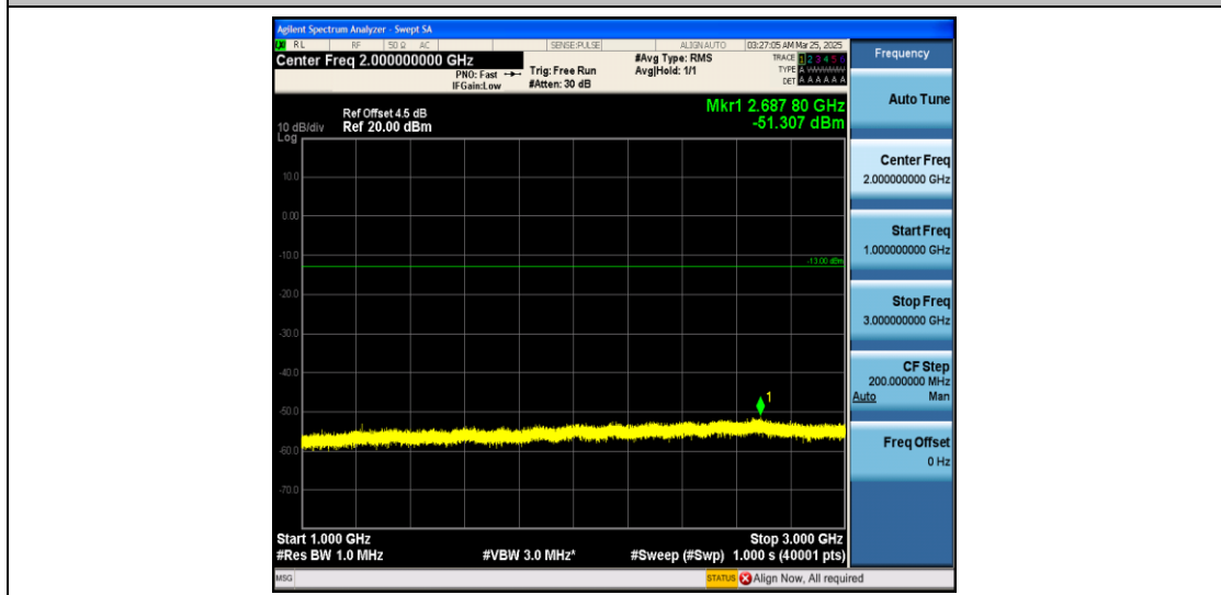
Band12_3MHz_16QAM_23165_1RB#0_1000~3000_1000~3000
