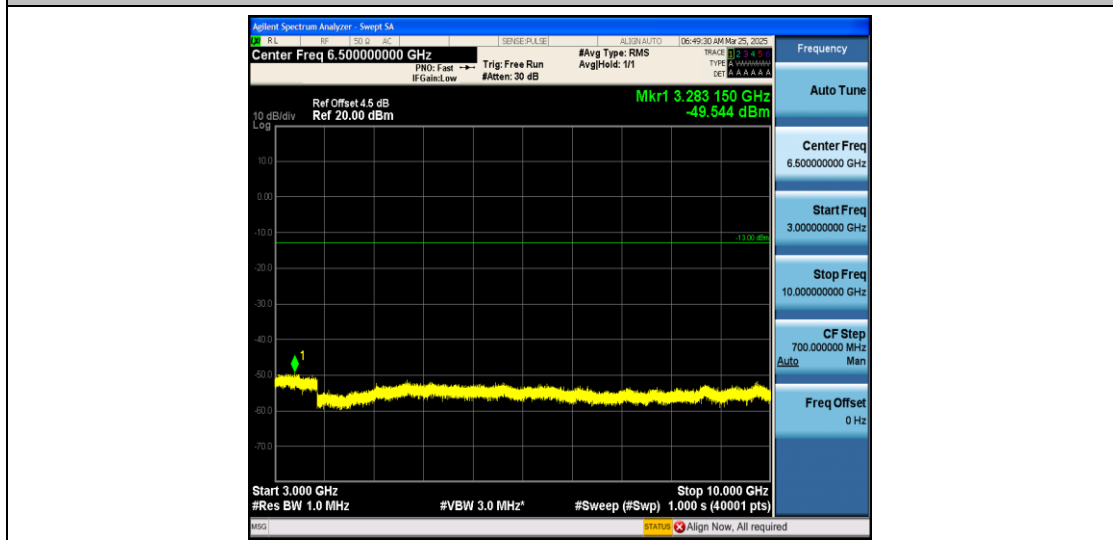
Band12_5MHz_QPSK_23035_1RB#0_3000~10000_3000~10000
