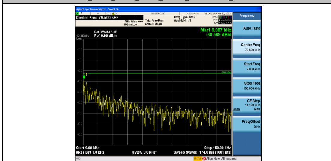
Band12_3MHz_16QAM_23025_1RB#0_0.009~0.15_0.009~0.15
