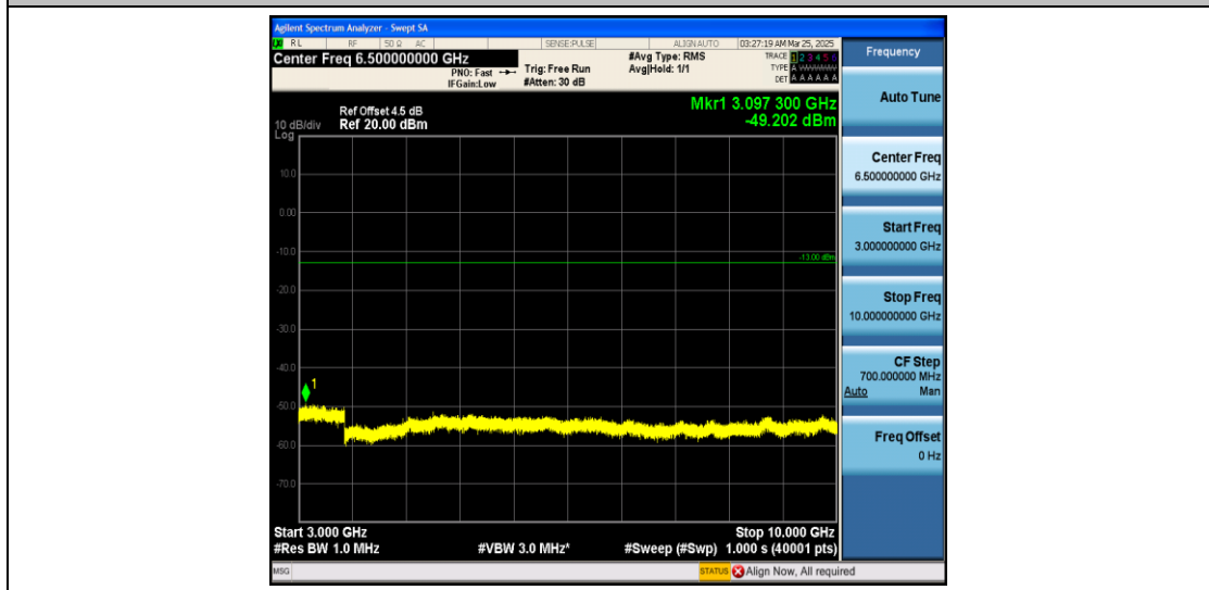
Band12_3MHz_16QAM_23165_1RB#0_3000~10000_3000~10000
