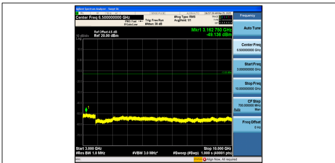
Band12_5MHz_16QAM_23035_1RB#0_3000~10000_3000~10000
