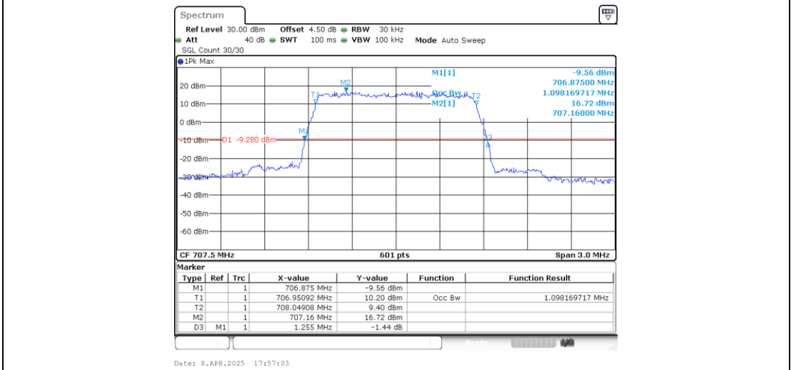
Band12-1.4MHz-QPSK-23095-6RB#0-PASS
