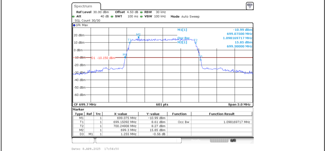
Band12-1.4MHz-16QAM-23017-6RB#0-PASS
