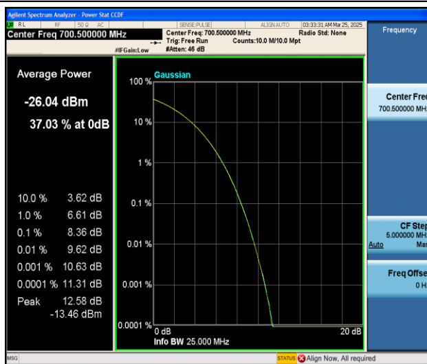
Band12-3MHz-QPSK-23025-15RB#0-PASS
