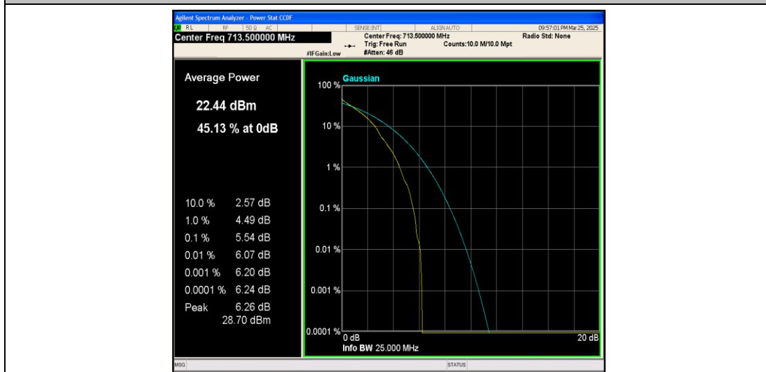
Band12-5MHz-QPSK-23155-1RB#0-PASS
