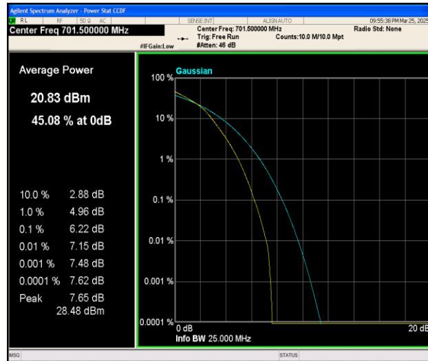
Band12-5MHz-16QAM-23035-25RB#0-PASS
