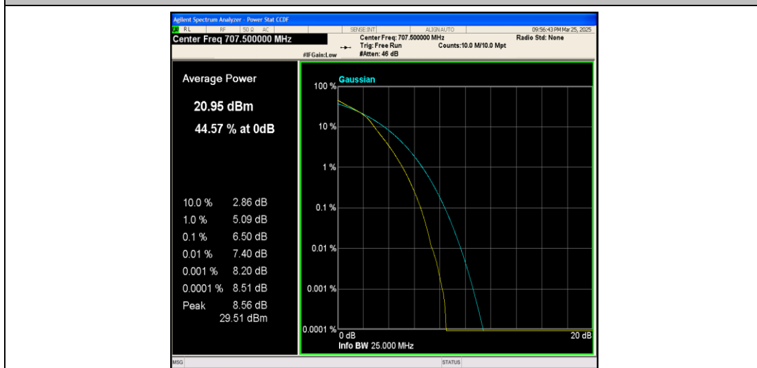
Band12-5MHz-16QAM-23095-25RB#0-PASS
