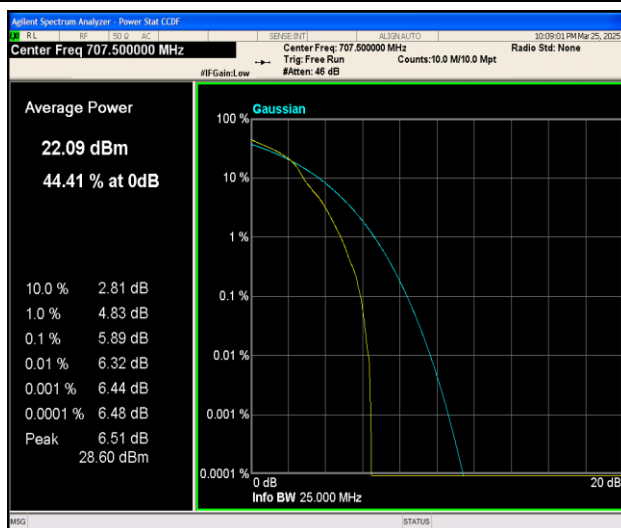
Band12-10MHz-16QAM-23095-1RB#0-PASS
