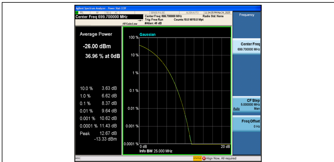
Band12-1.4MHz-16QAM-23017-6RB#0-PASS
