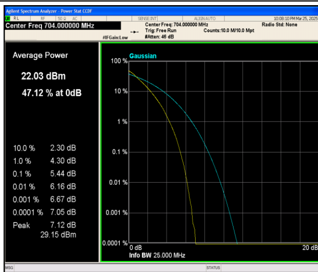
Band12-10MHz-QPSK-23060-50RB#0-PASS
