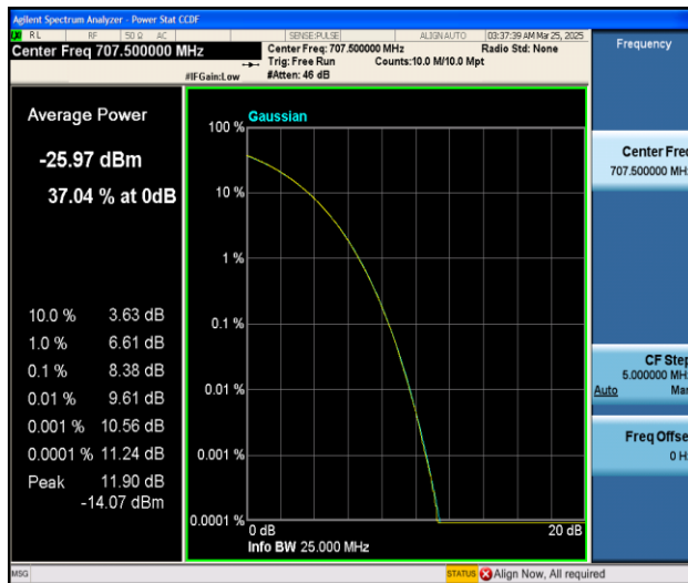
Band12-3MHz-QPSK-23095-1RB#0-PASS
