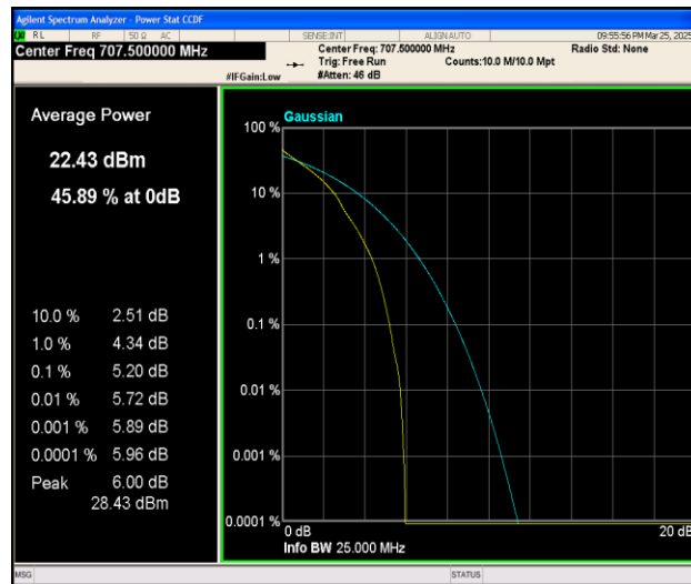
Band12-5MHz-QPSK-23095-1RB#0-PASS
