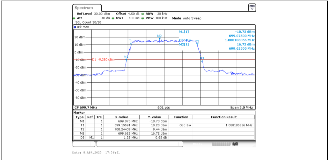
Band12-1.4MHz-QPSK-23017-6RB#0-PASS
