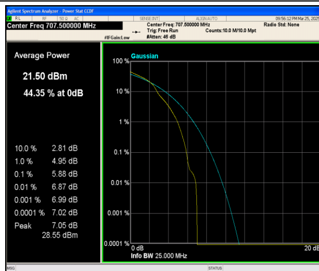
Band12-5MHz-16QAM-23095-1RB#0-PASS
