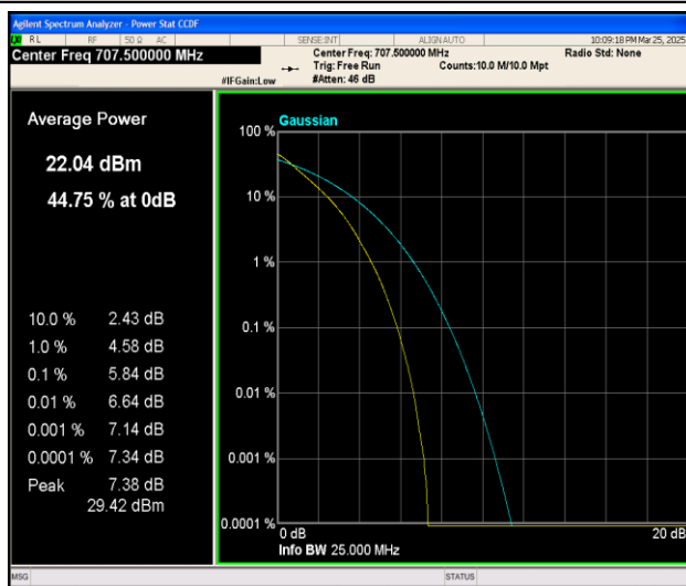
Band12-10MHz-QPSK-23095-50RB#0-PASS
