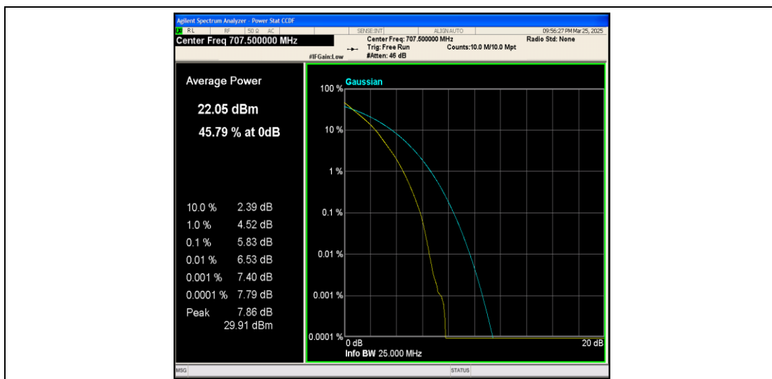
Band12-5MHz-QPSK-23095-25RB#0-PASS
