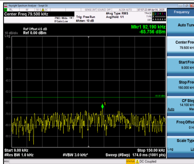
Band7_10MHz_QPSK_21400_1RB#0_0.009~0.15_0.009~0.15
