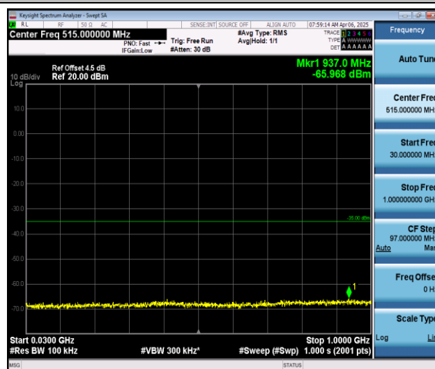
Band7_15MHz_QPSK_20825_1RB#0_30~1000_30~1000
