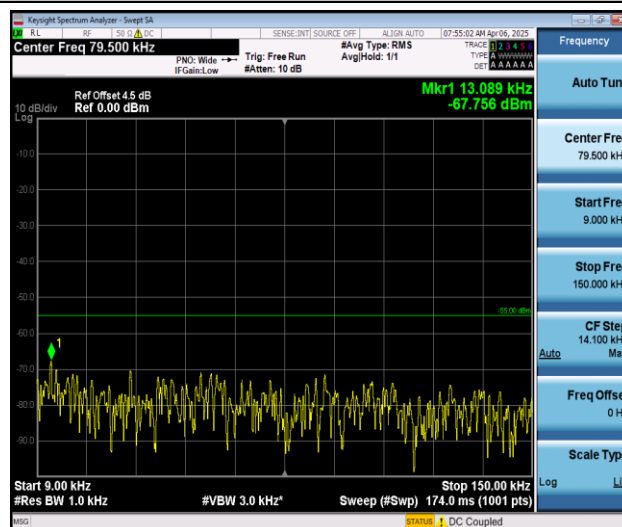
Band7_10MHz_16QAM_20800_1RB#0_0.009~0.15_0.009~0.15
