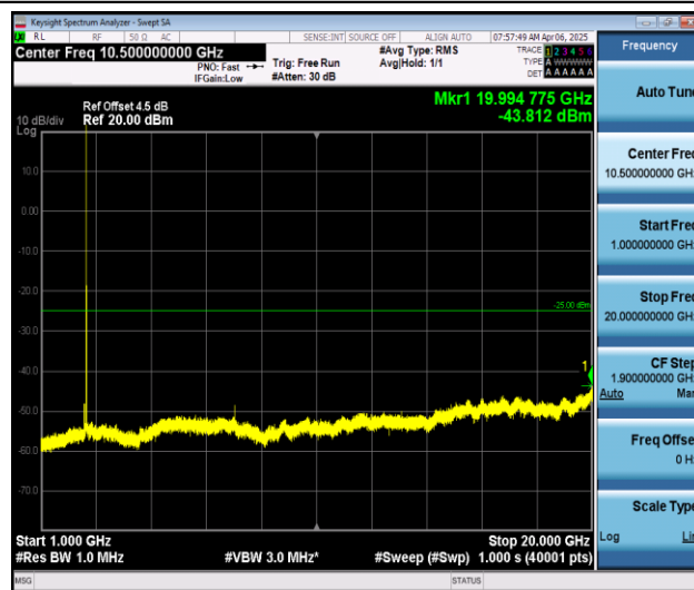
Band7_10MHz_QPSK_21400_1RB#0_1000~20000_1000~20000
