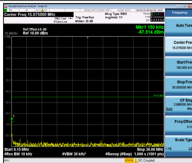
Band7_15MHz_QPSK_21100_1RB#0_0.15~30_0.15~30
