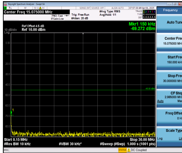
Band7_10MHz_QPSK_21400_1RB#0_0.15~30_0.15~30
