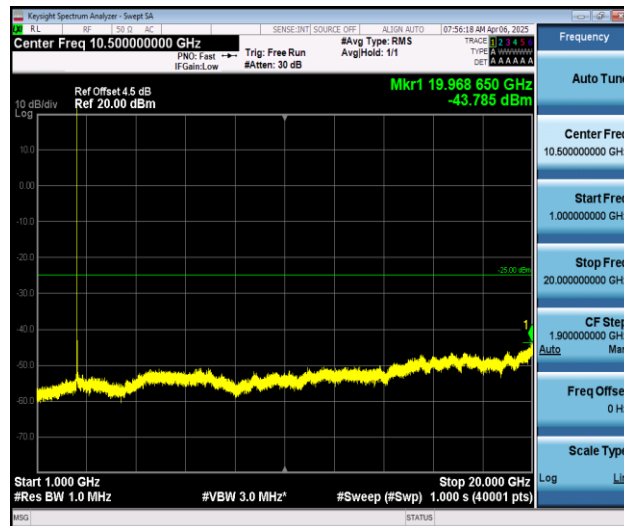
Band7_10MHz_QPSK_21100_1RB#0_1000~20000_1000~20000
