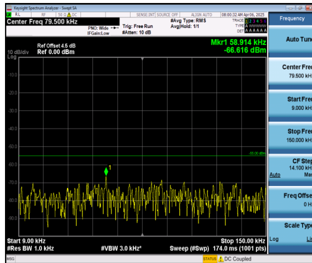
Band7_15MHz_QPSK_21100_1RB#0_0.009~0.15_0.009~0.15
