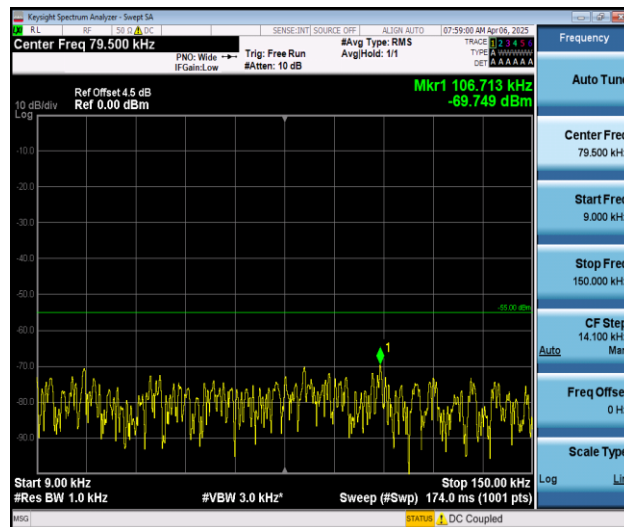
Band7_15MHz_QPSK_20825_1RB#0_0.009~0.15_0.009~0.15
