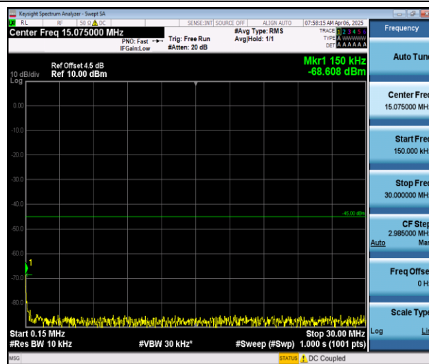
Band7_10MHz_16QAM_21400_1RB#0_0.15~30_0.15~30
