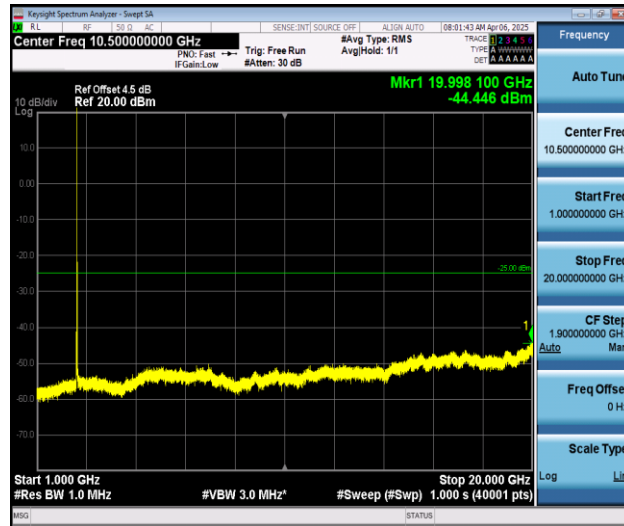
Band7_15MHz_16QAM_21100_1RB#0_1000~20000_1000~20000
