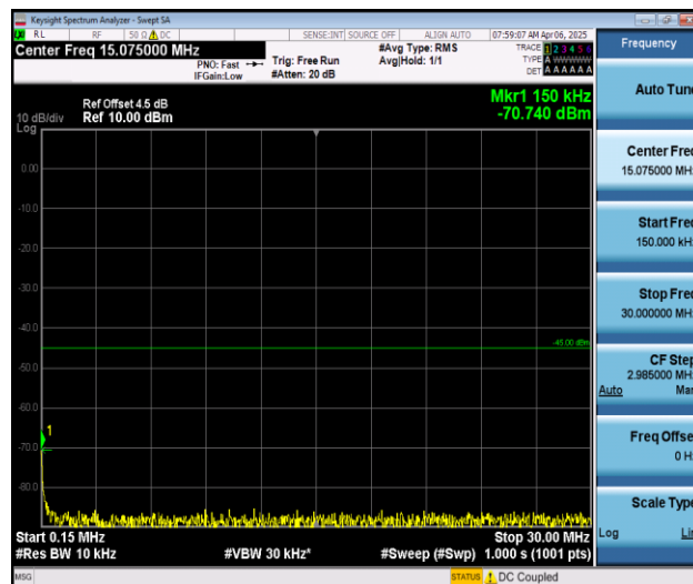
Band7_15MHz_QPSK_20825_1RB#0_0.15~30_0.15~30
