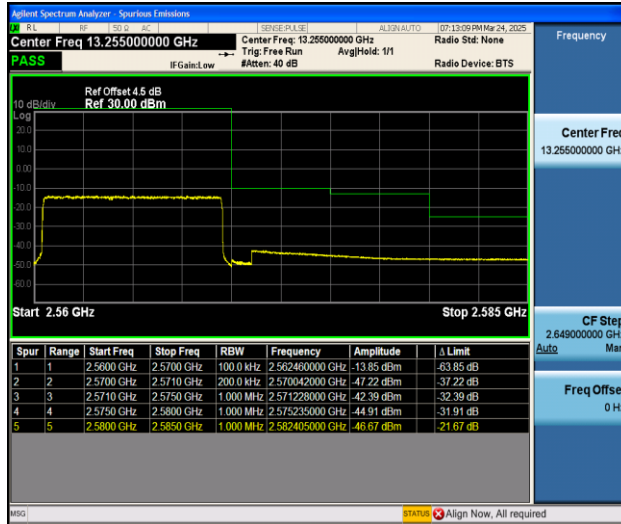
Band7_10MHz_16QAM_21400_50RB#0
