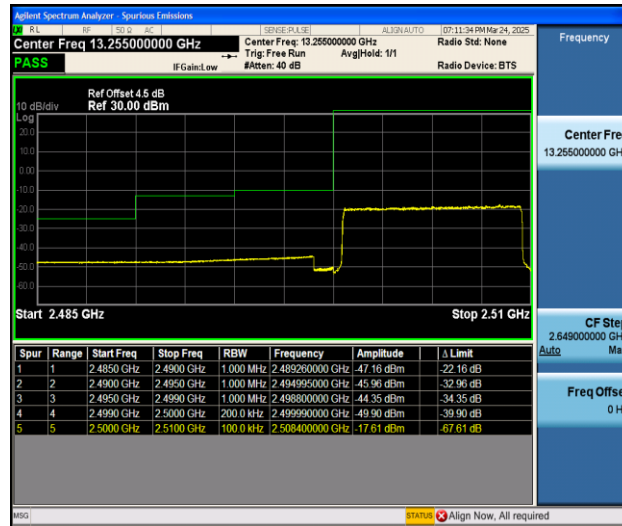
Band7_10MHz_16QAM_20800_50RB#0
