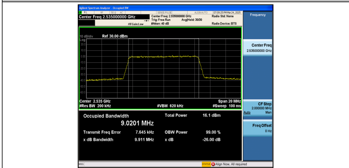
Band7-10MHz-QPSK-21100-50RB#0-PASS
