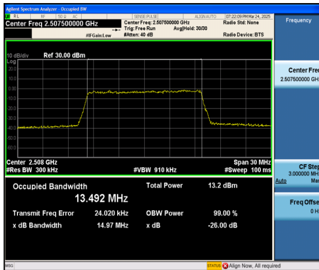
Band7-15MHz-16QAM-20825-75RB#0-PASS
