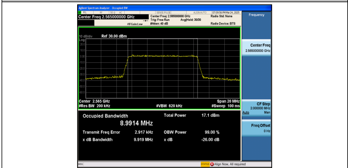
Band7-10MHz-16QAM-21400-50RB#0-PASS
