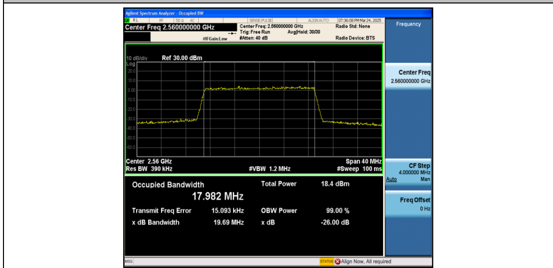
Band7-20MHz-QPSK-21350-100RB#0-PASS
