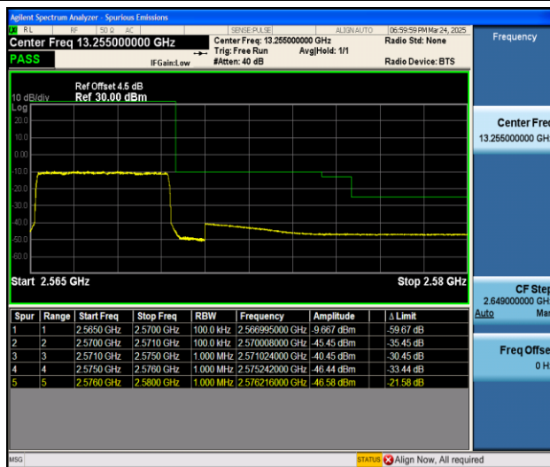
Band7_5MHz_QPSK_21425_25RB#0
