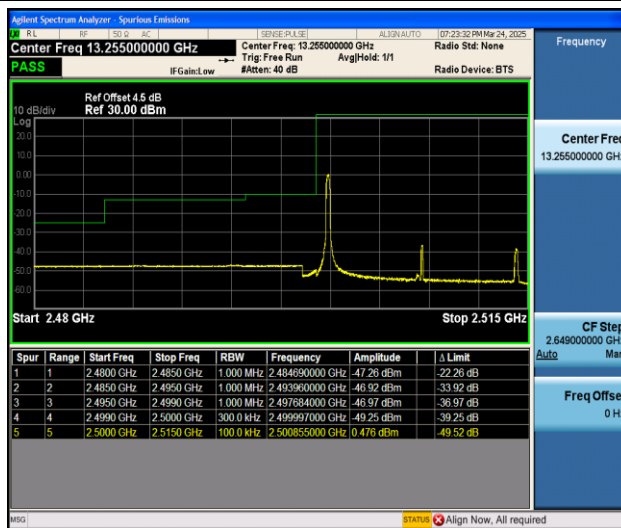
Band7_15MHz_16QAM_20825_1RB#0
