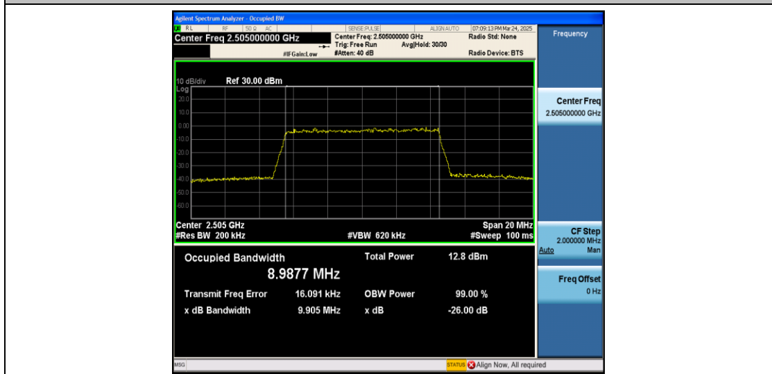
Band7-10MHz-16QAM-20800-50RB#0-PASS
