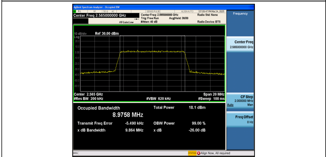
Band7-10MHz-QPSK-21400-50RB#0-PASS
