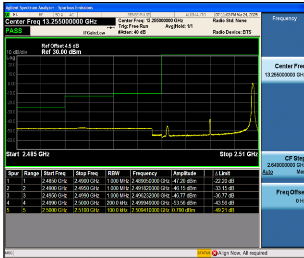
Band7_10MHz_16QAM_20800_1RB#49
