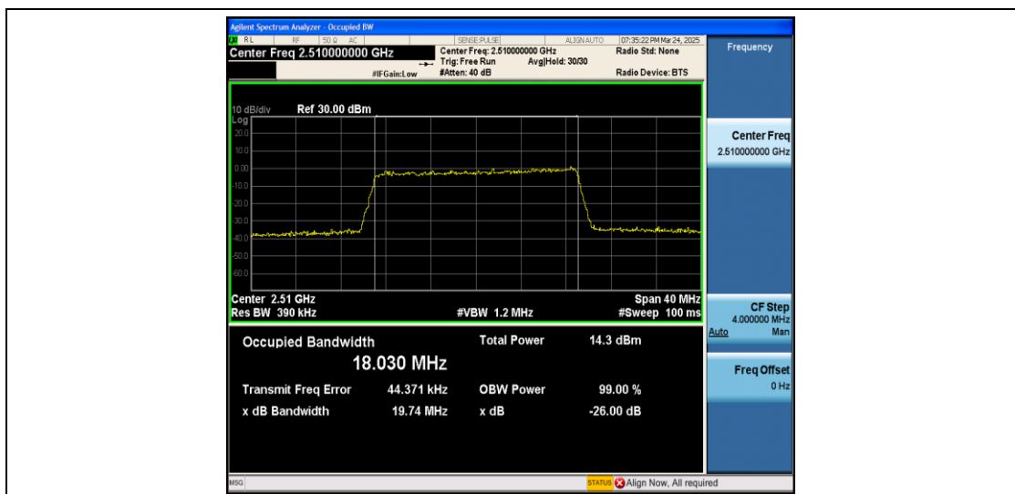
Band7-20MHz-QPSK-20850-100RB#0-PASS
