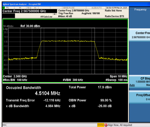
Band7-5MHz-QPSK-21425-25RB#0-PASS
