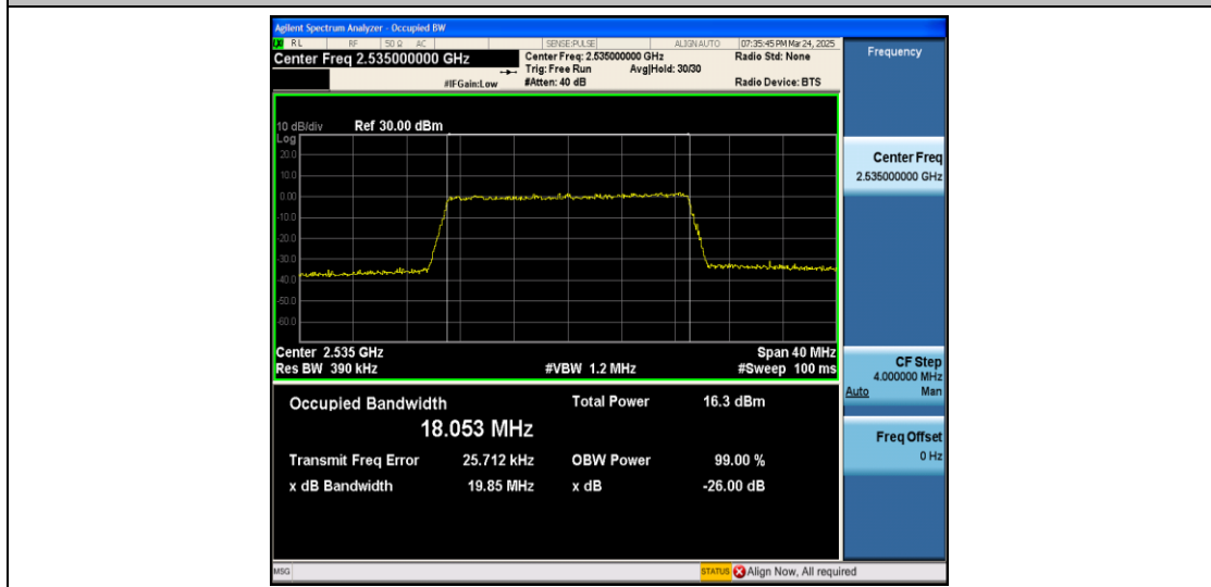
Band7-20MHz-QPSK-21100-100RB#0-PASS
