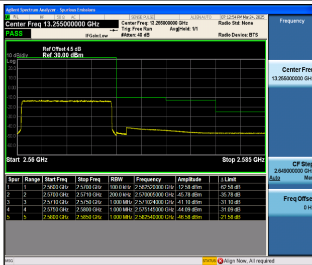
Band7_10MHz_QPSK_21400_50RB#0
