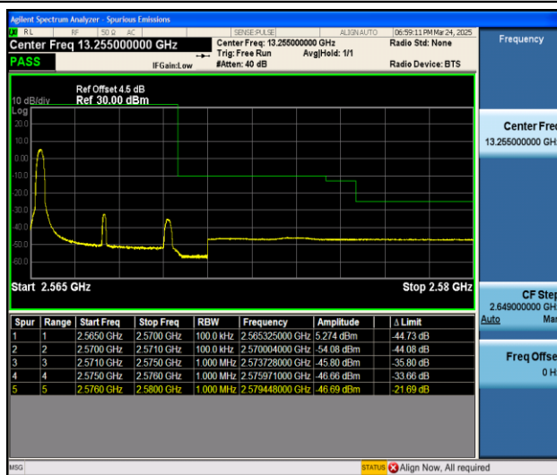
Band7_5MHz_16QAM_21425_1RB#0
