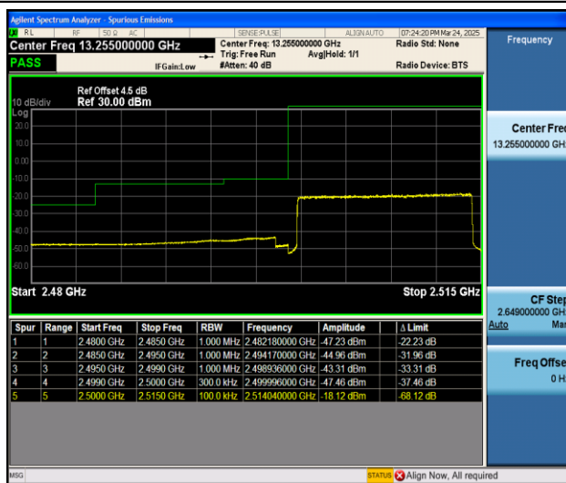
Band7_15MHz_QPSK_20825_75RB#0
