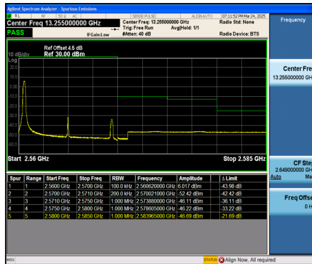
Band7_10MHz_QPSK_21400_1RB#0
