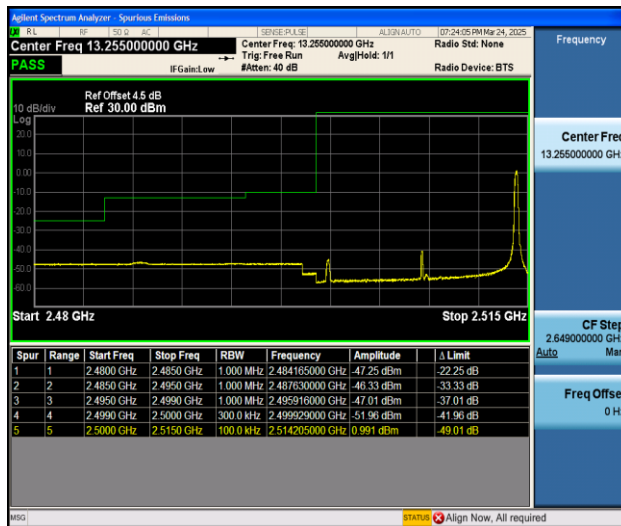
Band7_15MHz_16QAM_20825_1RB#74
