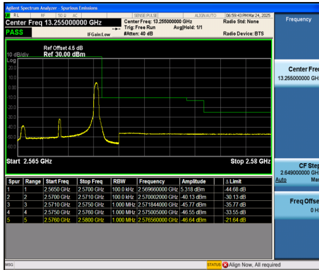
Band7_5MHz_16QAM_21425_1RB#24
