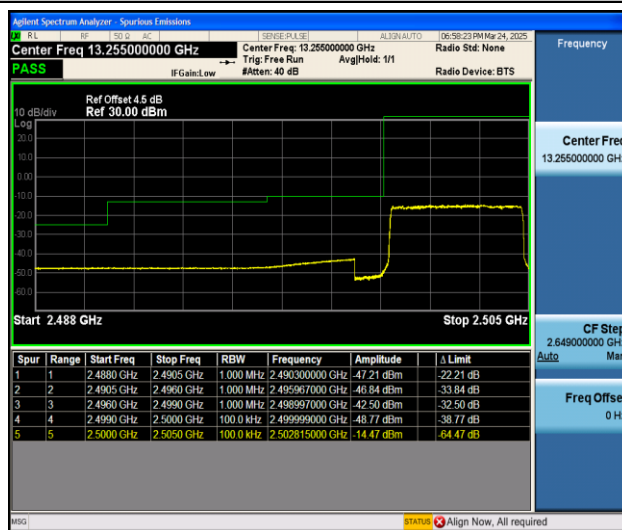
Band7_5MHz_QPSK_20775_25RB#0
