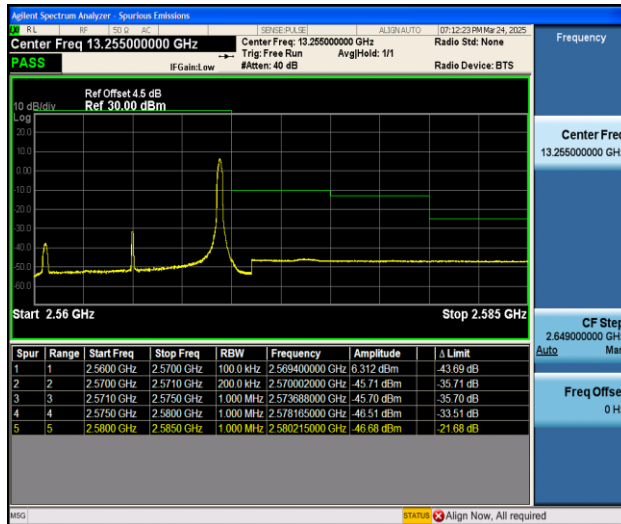
Band7_10MHz_QPSK_21400_1RB#49
