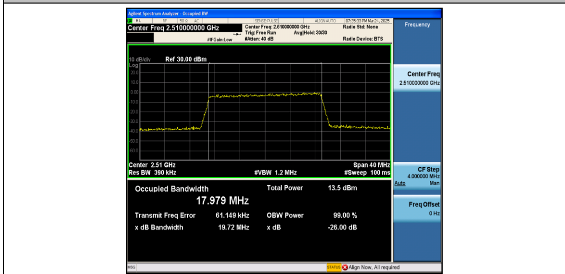
Band7-20MHz-16QAM-20850-100RB#0-PASS
