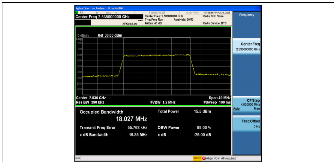
Band7-20MHz-16QAM-21100-100RB#0-PASS
