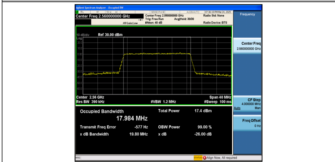
Band7-20MHz-16QAM-21350-100RB#0-PASS
