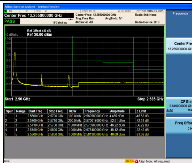
Band7_10MHz_16QAM_21400_1RB#0
