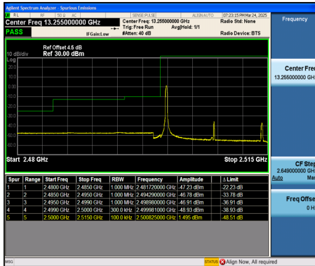
Band7_15MHz_QPSK_20825_1RB#0
