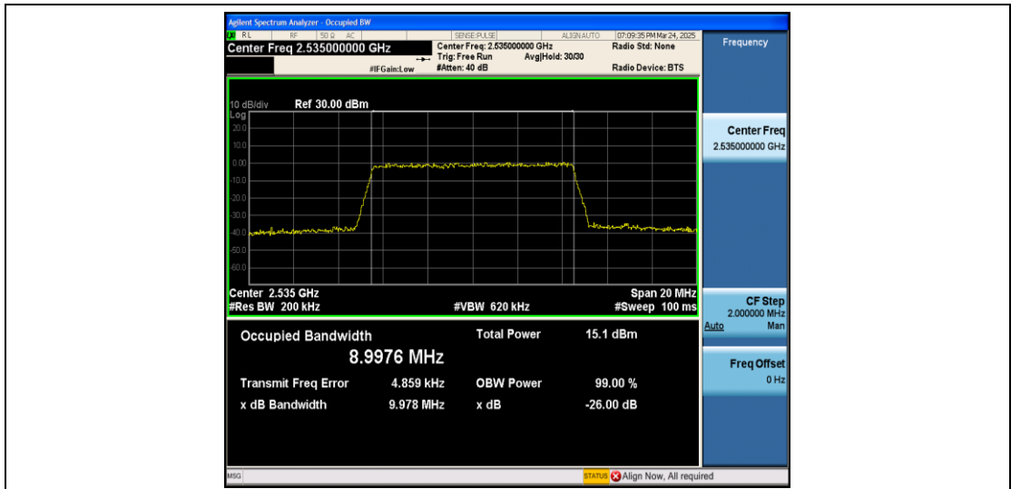
Band7-10MHz-16QAM-21100-50RB#0-PASS
