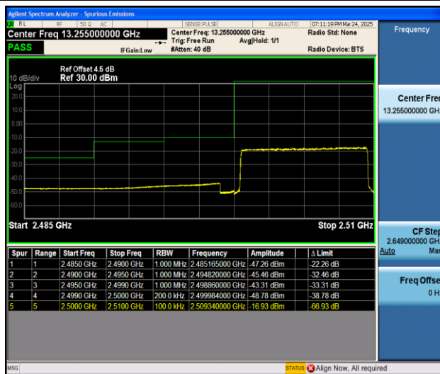
Band7_10MHz_QPSK_20800_50RB#0
