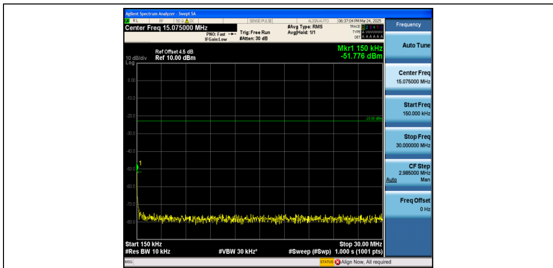
Band5_5MHz_QPSK_20625_1RB#0_0.15~30_0.15~30
