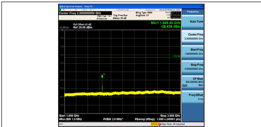
Band5_10MHz_QPSK_20450_1RB#0_1000~3000_1000~3000
