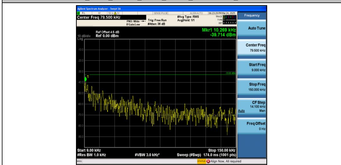
Band5_3MHz_QPSK_20635_1RB#0_0.009~0.15_0.009~0.15
