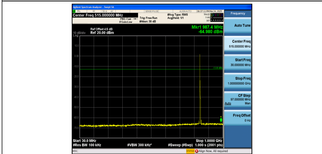
Band5_5MHz_QPSK_20625_1RB#0_30~1000_30~1000
