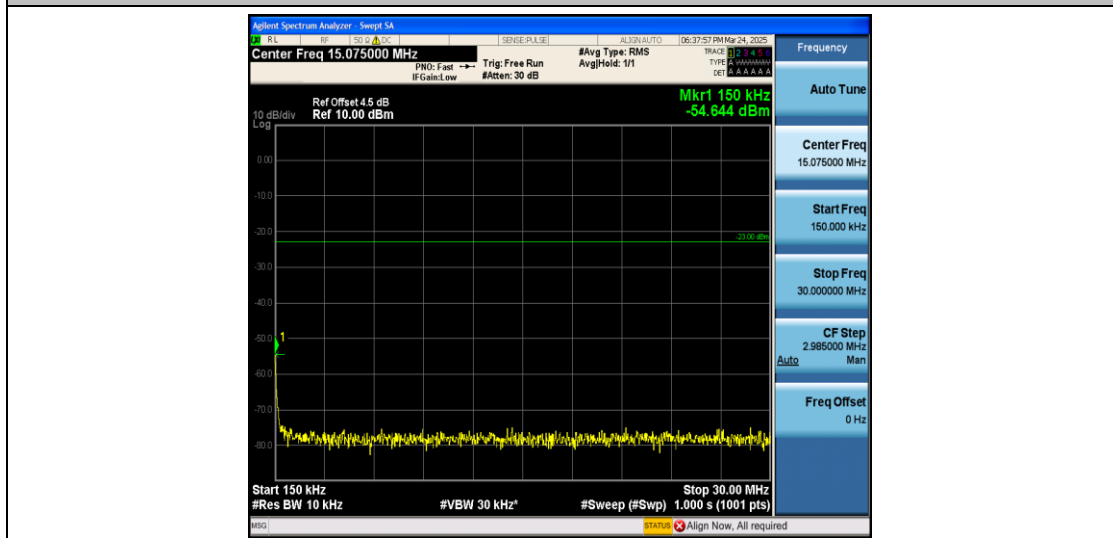
Band5_5MHz_16QAM_20625_1RB#0_0.15~30_0.15~30
