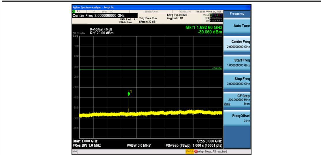
Band5_3MHz_QPSK_20635_1RB#0_1000~3000_1000~3000
