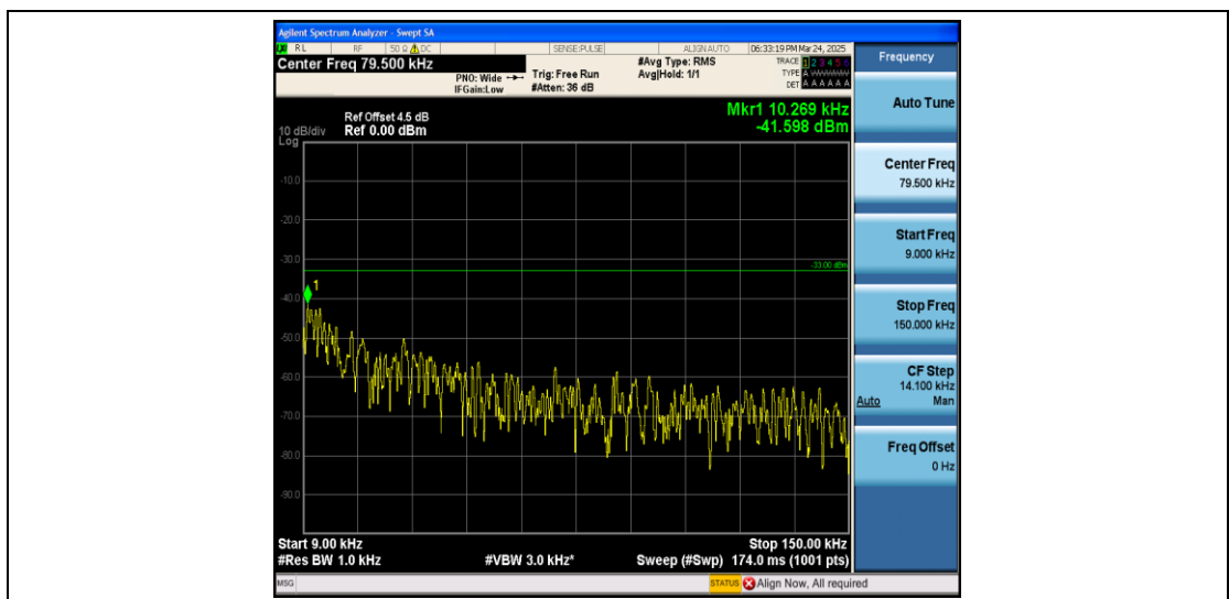
Band5_5MHz_QPSK_20425_1RB#0_0.009~0.15_0.009~0.15
