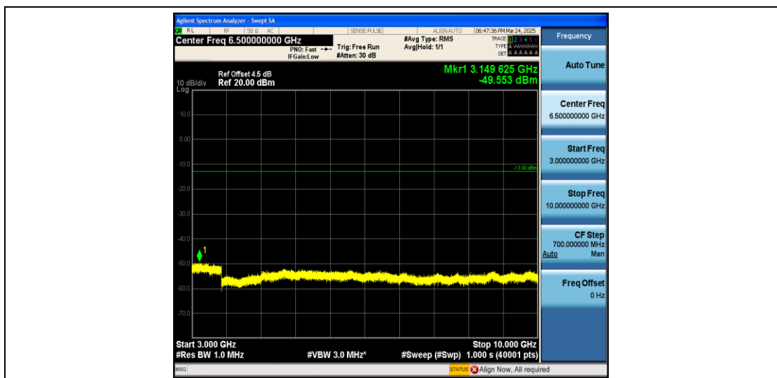
Band5_10MHz_16QAM_20450_1RB#0_3000~10000_3000~10000
