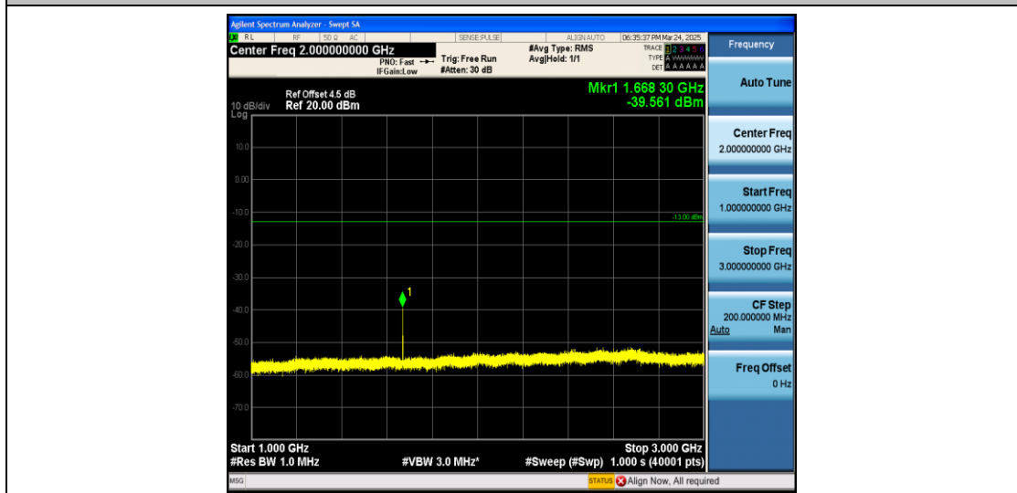
Band5_5MHz_QPSK_20525_1RB#0_1000~3000_1000~3000
