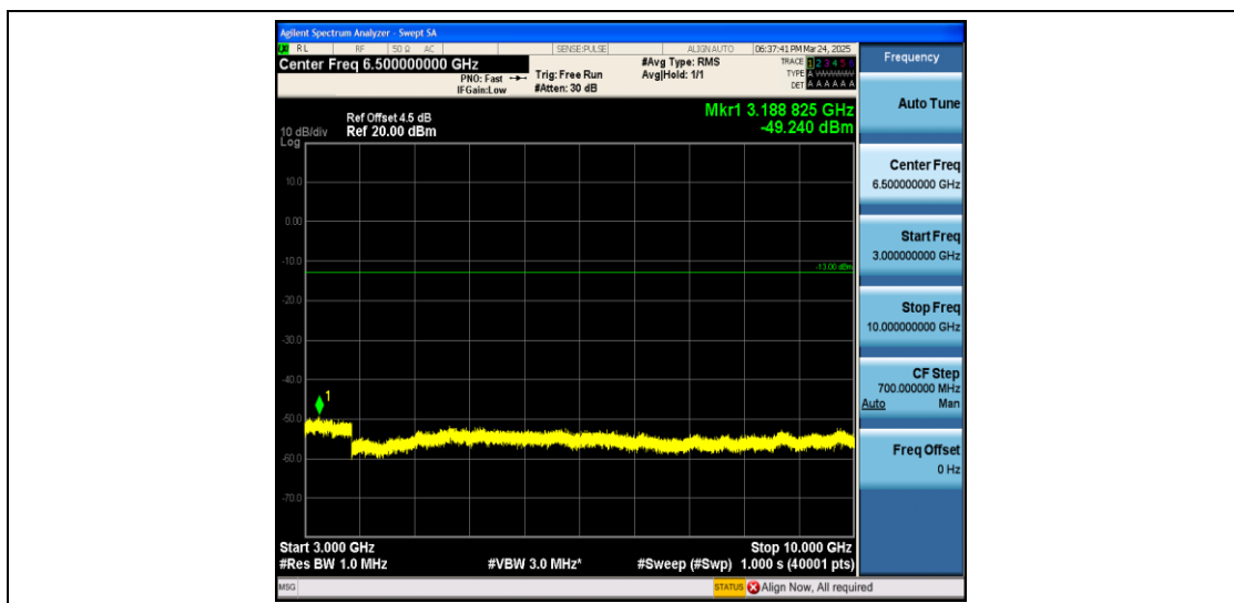
Band5_5MHz_QPSK_20625_1RB#0_3000~10000_3000~10000
