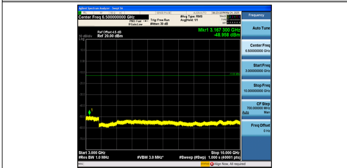
Band5_3MHz_16QAM_20525_1RB#0_3000~10000_3000~10000
