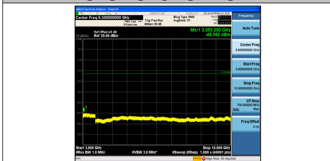
Band5_5MHz_16QAM_20525_1RB#0_3000~10000_3000~10000
