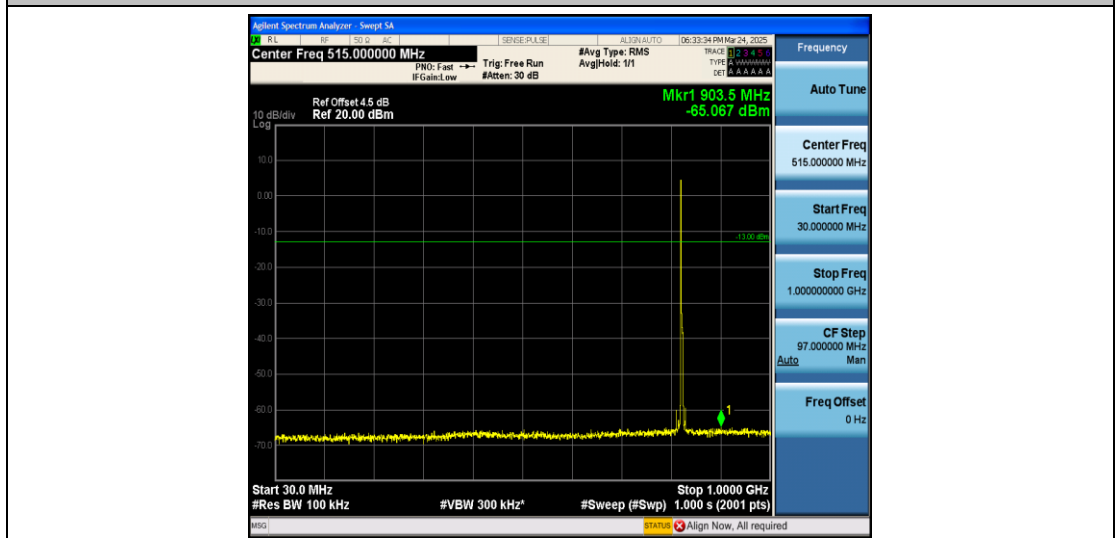
Band5_5MHz_QPSK_20425_1RB#0_30~1000_30~1000
