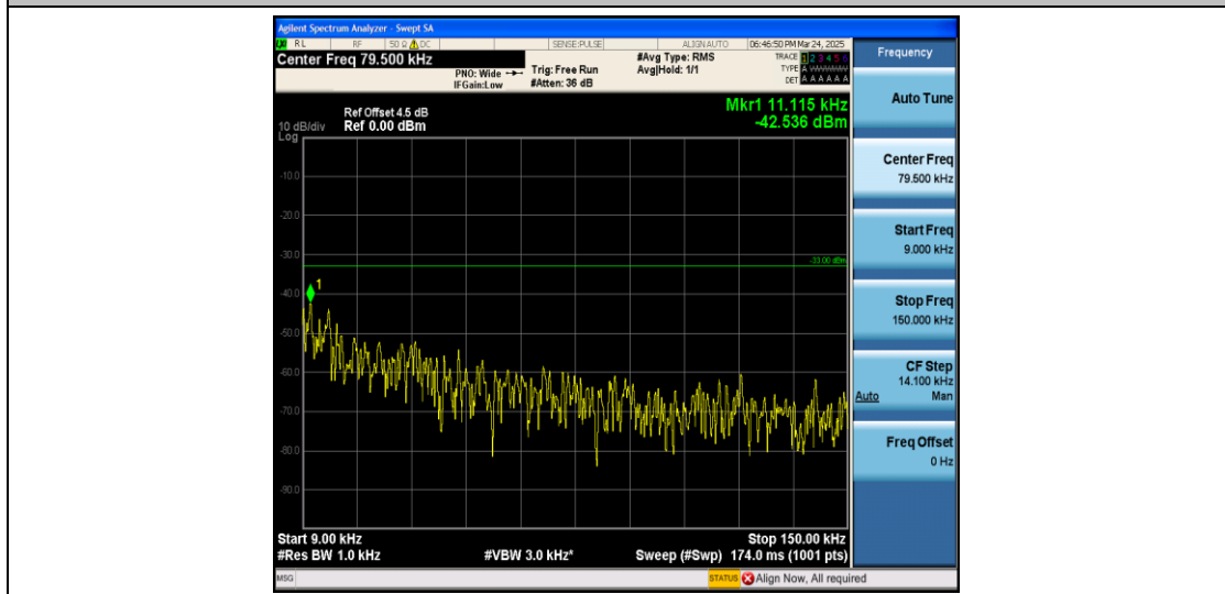
Band5_10MHz_16QAM_20450_1RB#0_0.009~0.15_0.009~0.15
