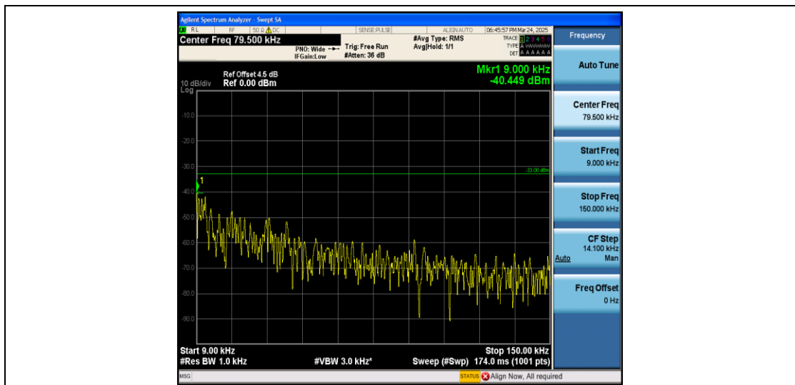
Band5_10MHz_QPSK_20450_1RB#0_0.009~0.15_0.009~0.15
