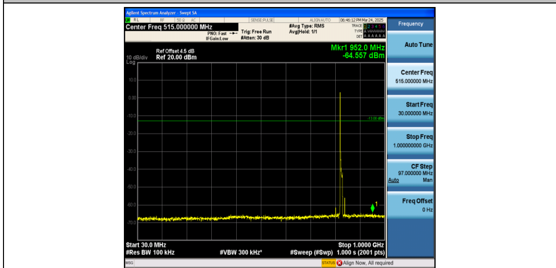
Band5_10MHz_QPSK_20450_1RB#0_30~1000_30~1000
