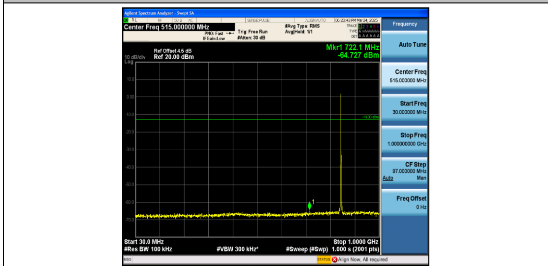
Band5_3MHz_QPSK_20635_1RB#0_30~1000_30~1000
