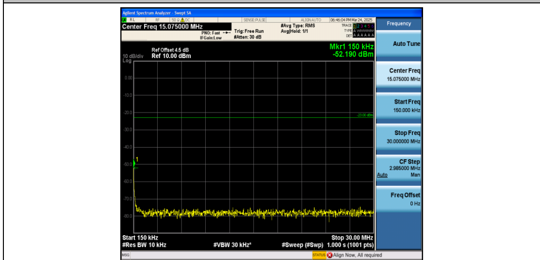
Band5_10MHz_QPSK_20450_1RB#0_0.15~30_0.15~30
