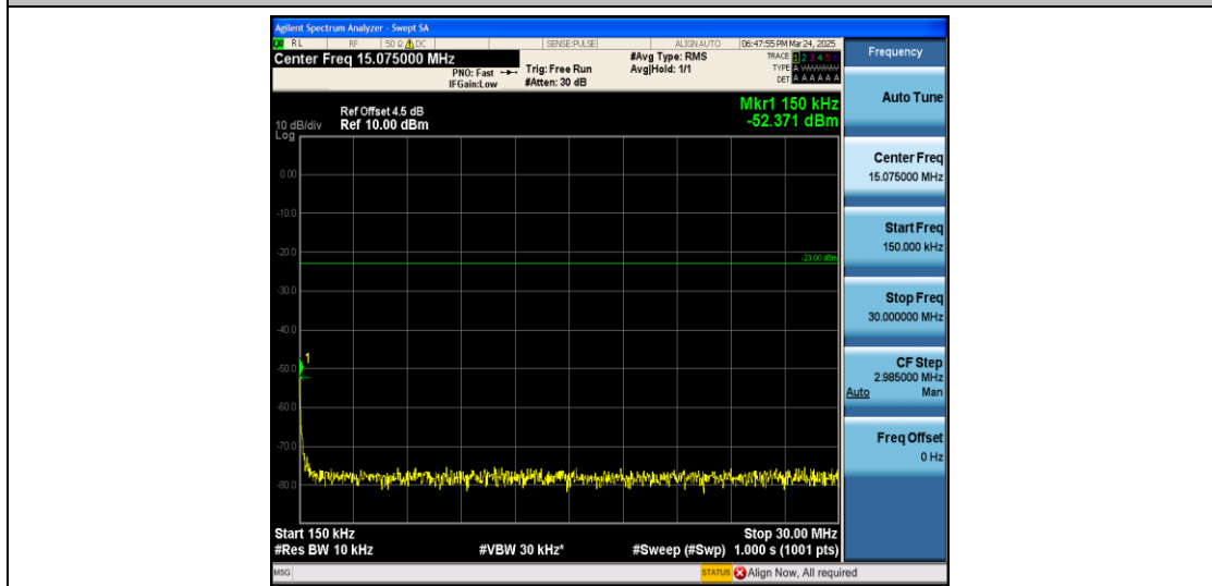
Band5_10MHz_QPSK_20525_1RB#0_0.15~30_0.15~30
