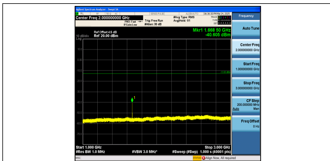
Band5_5MHz_16QAM_20525_1RB#0_1000~3000_1000~3000
