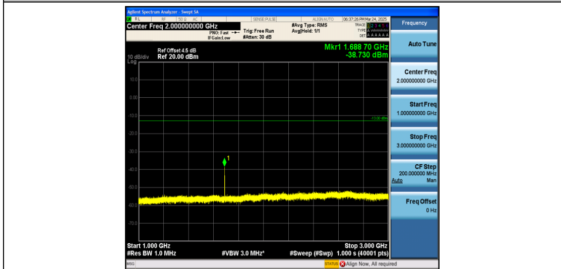
Band5_5MHz_QPSK_20625_1RB#0_1000~3000_1000~3000
