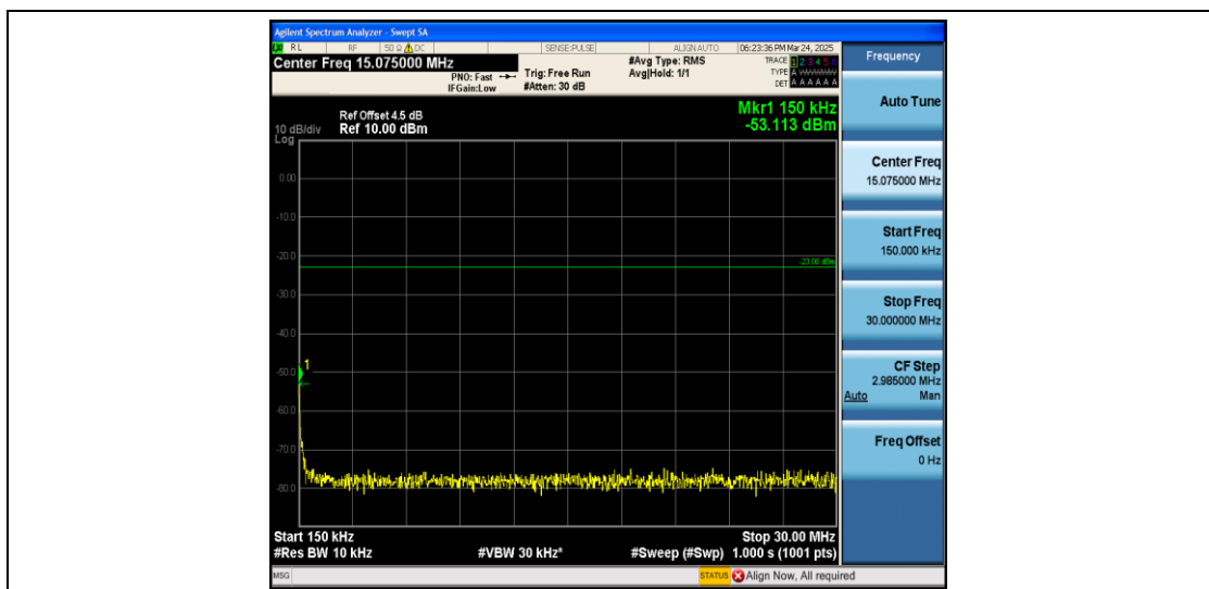
Band5_3MHz_QPSK_20635_1RB#0_0.15~30_0.15~30
