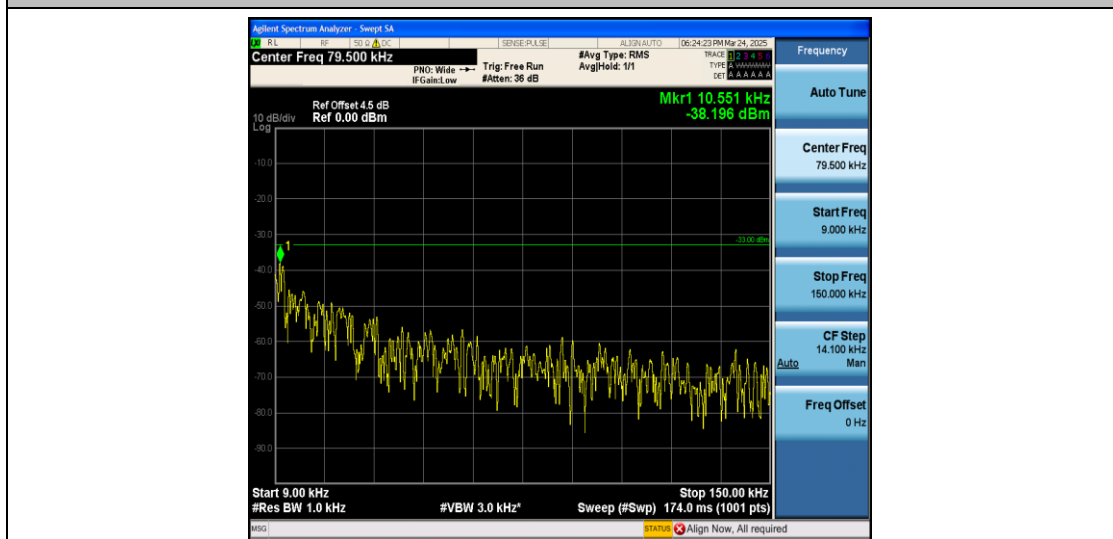
Band5_3MHz_16QAM_20635_1RB#0_0.009~0.15_0.009~0.15
