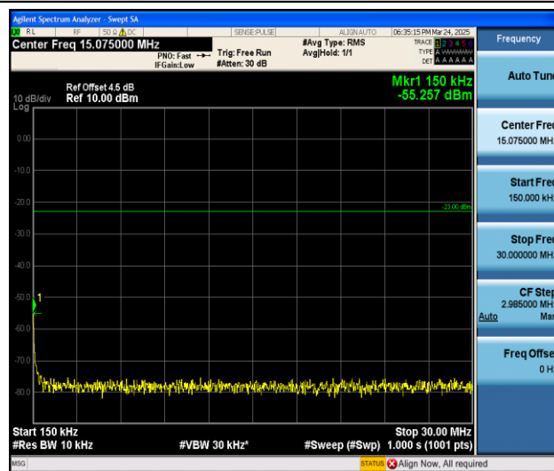
Band5_5MHz_QPSK_20525_1RB#0_0.15~30_0.15~30
