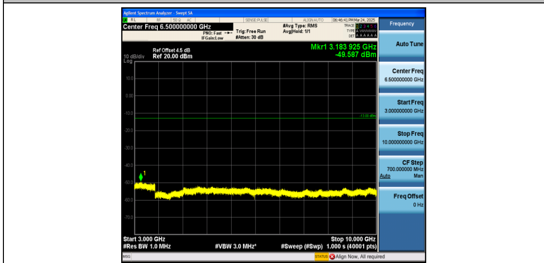
Band5_10MHz_QPSK_20450_1RB#0_3000~10000_3000~10000
