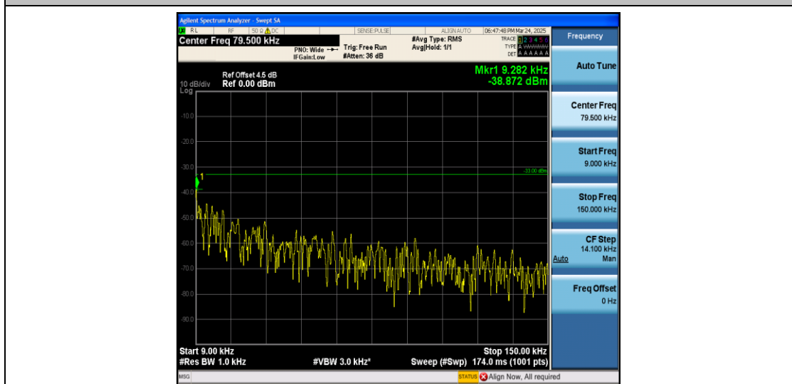
Band5_10MHz_QPSK_20525_1RB#0_0.009~0.15_0.009~0.15
