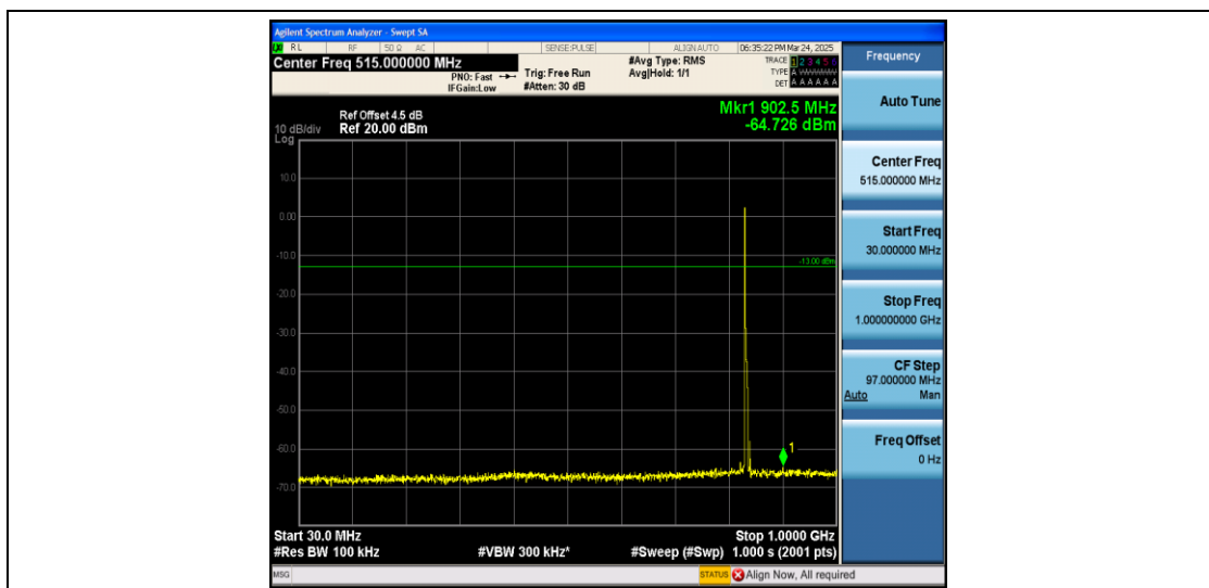
Band5_5MHz_QPSK_20525_1RB#0_30~1000_30~1000
