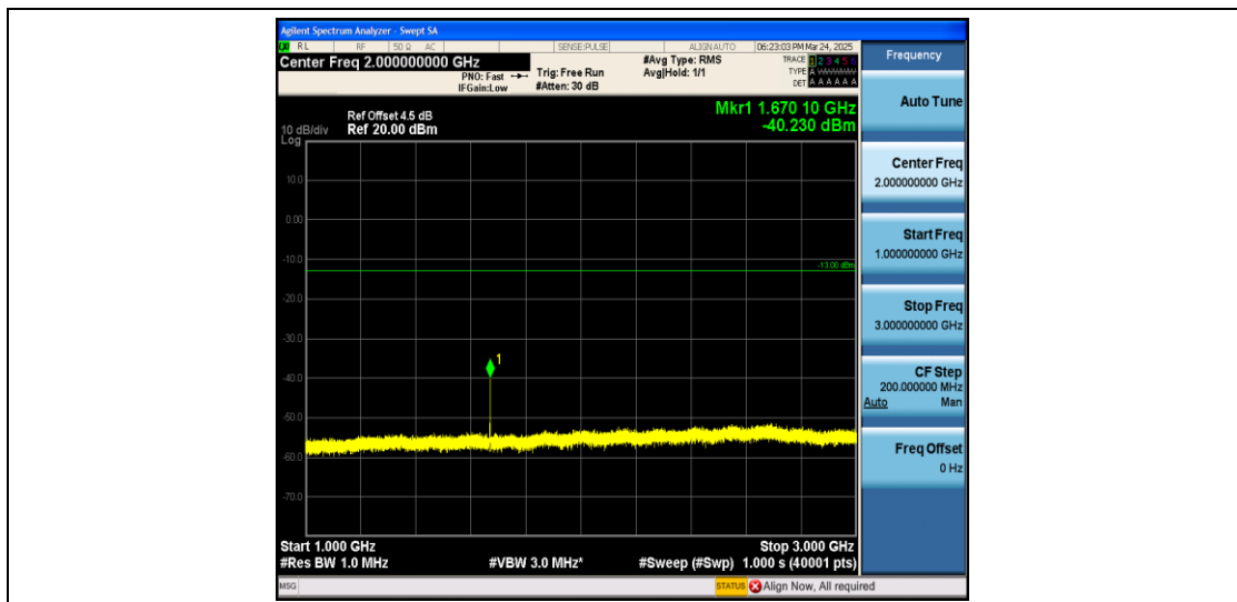
Band5_3MHz_16QAM_20525_1RB#0_1000~3000_1000~3000
