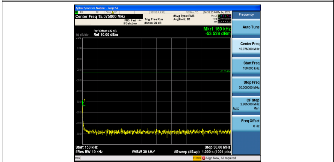
Band5_5MHz_QPSK_20425_1RB#0_0.15~30_0.15~30
