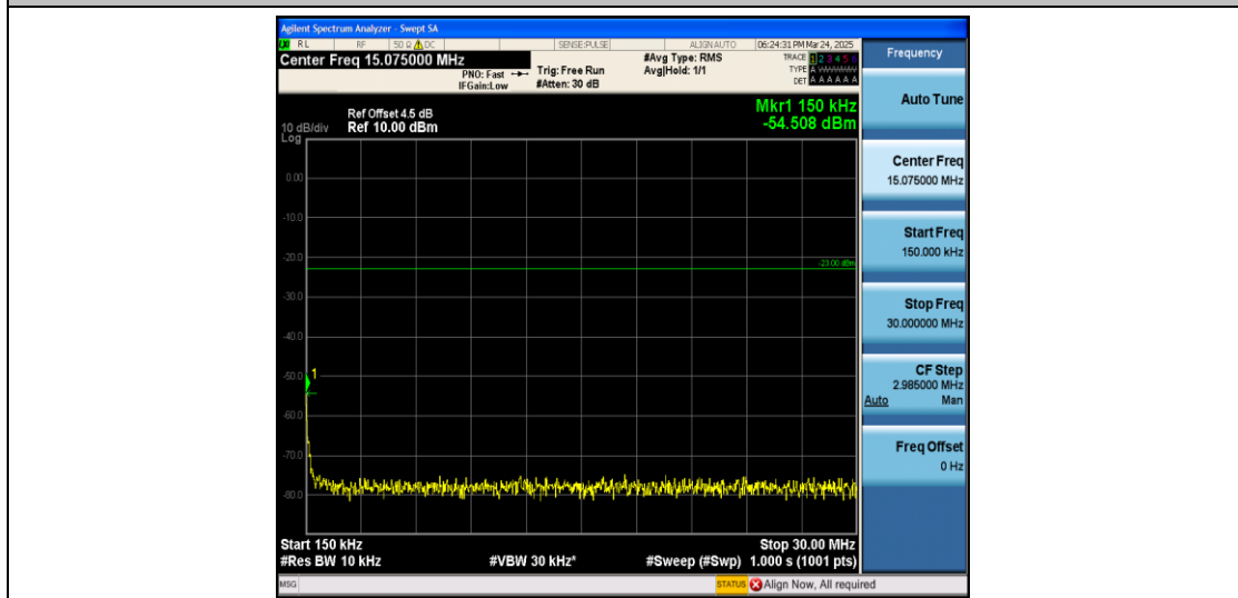
Band5_3MHz_16QAM_20635_1RB#0_0.15~30_0.15~30
