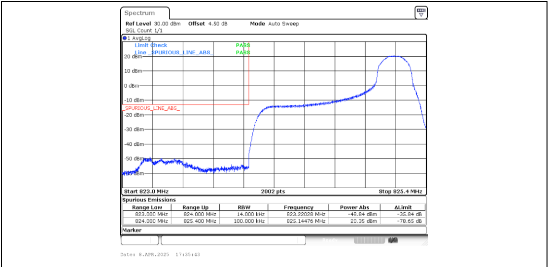
Band5_1.4MHz_QPSK_20407_1RB#5
