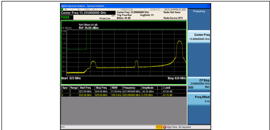
Band5_5MHz_QPSK_20425_1RB#24
