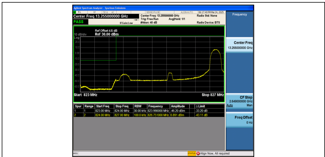
Band5_3MHz_QPSK_20415_1RB#14
