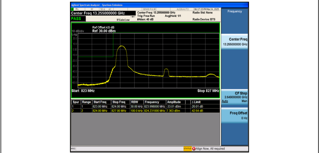
Band5_3MHz_QPSK_20415_1RB#0
