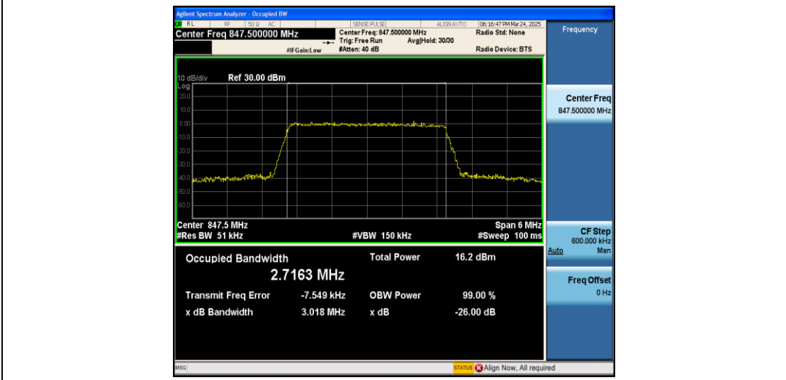
Band5-3MHz-QPSK-20635-15RB#0-PASS
