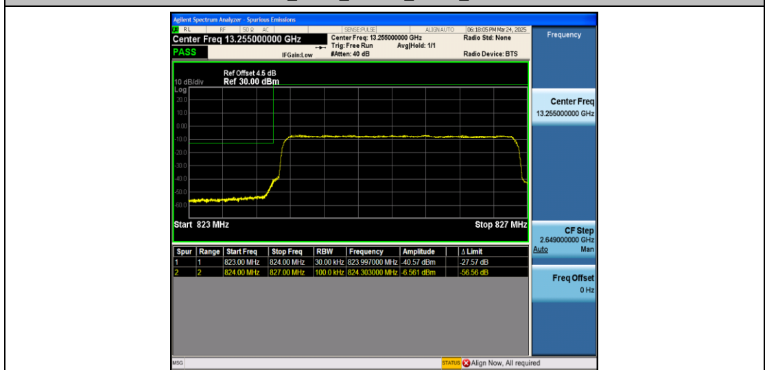
Band5_3MHz_QPSK_20415_15RB#0
