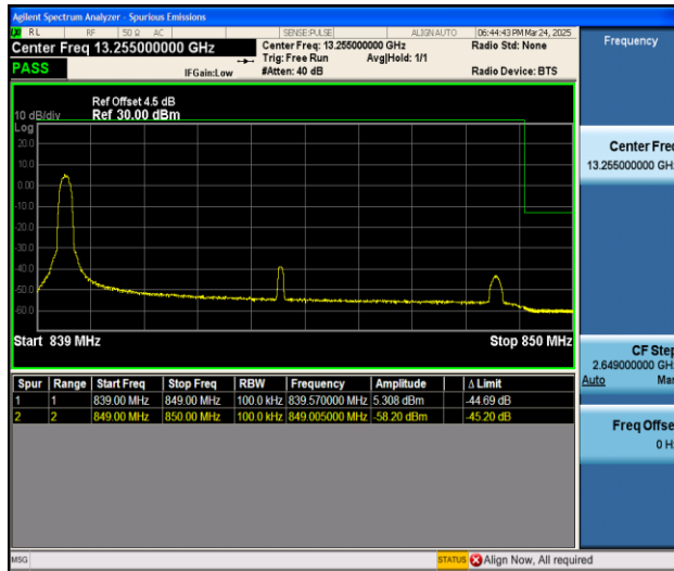
Band5_10MHz_QPSK_20600_1RB#0
