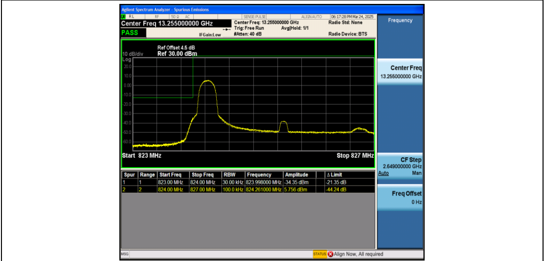
Band5_3MHz_16QAM_20415_1RB#0
