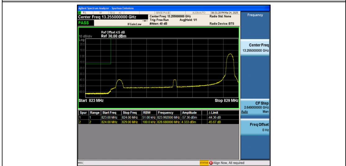
Band5_5MHz_16QAM_20425_1RB#24
