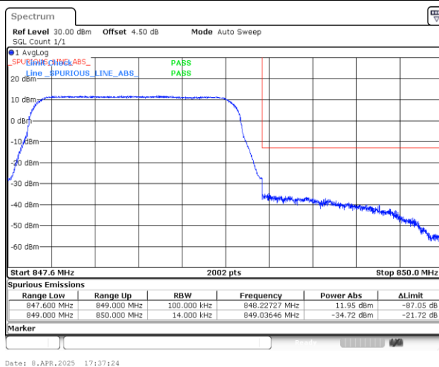
Band5_1.4MHz_QPSK_20643_6RB#0
