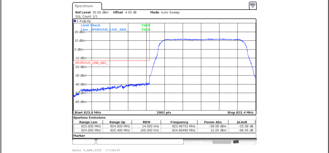
Band5_1.4MHz_QPSK_20407_6RB#0
