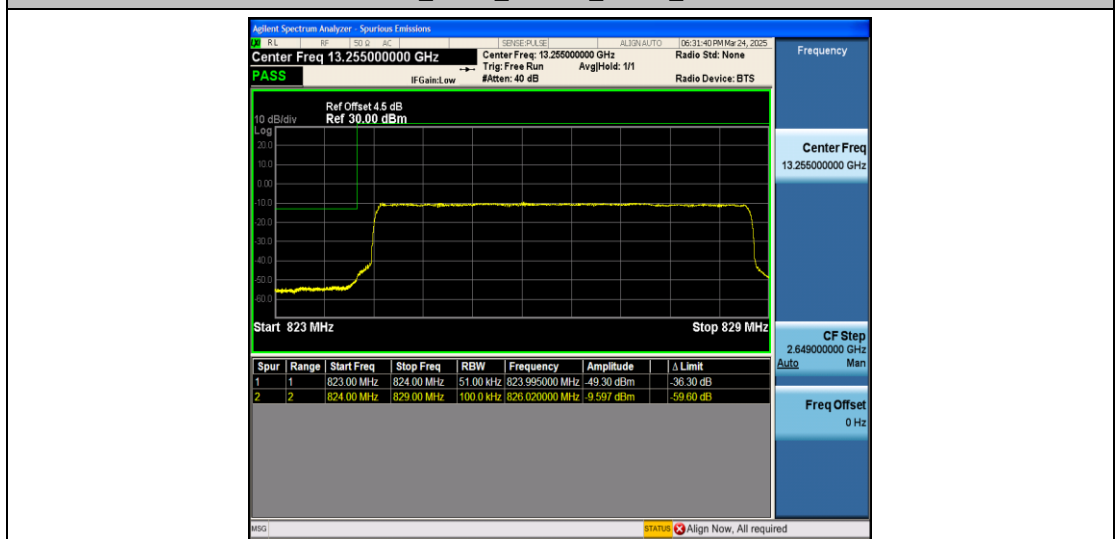
Band5_5MHz_QPSK_20425_25RB#0
