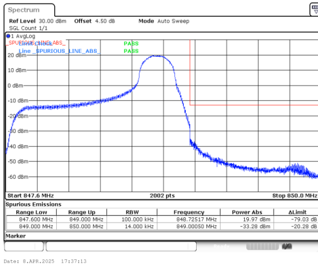
Band5_1.4MHz_16QAM_20643_1RB#5
