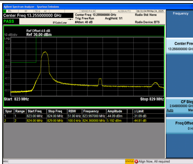
Band5_5MHz_16QAM_20425_1RB#0
