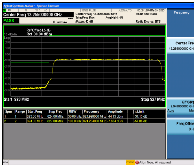
Band5_3MHz_16QAM_20415_15RB#0
