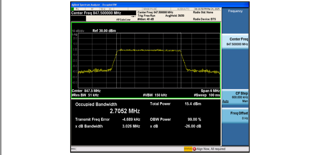
Band5-3MHz-16QAM-20635-15RB#0-PASS
