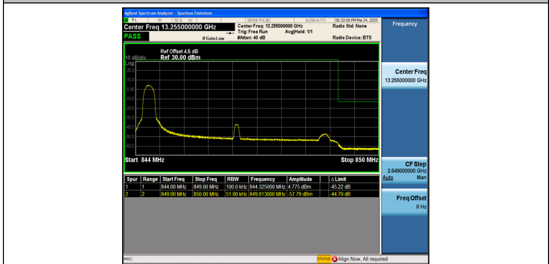
Band5_5MHz_QPSK_20625_1RB#0
