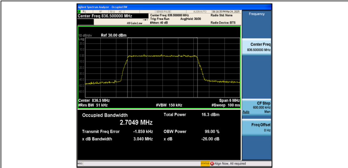
Band5-3MHz-16QAM-20525-15RB#0-PASS
