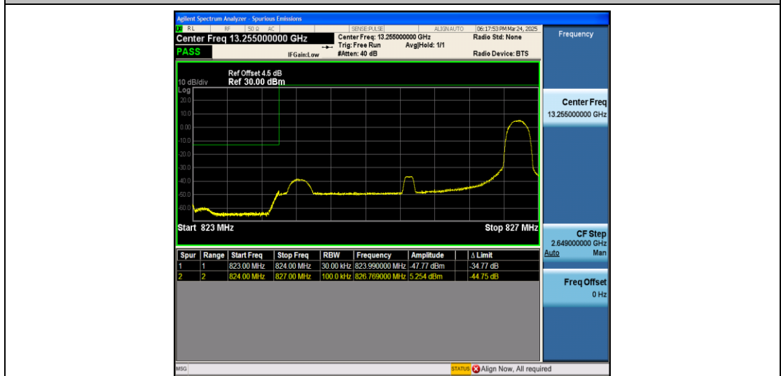
Band5_3MHz_16QAM_20415_1RB#14
