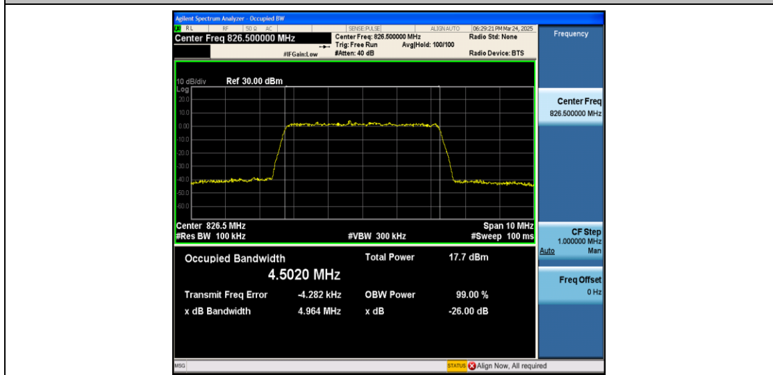
Band5-5MHz-16QAM-20425-25RB#0-PASS
