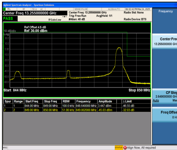
Band5_5MHz_16QAM_20625_1RB#24
