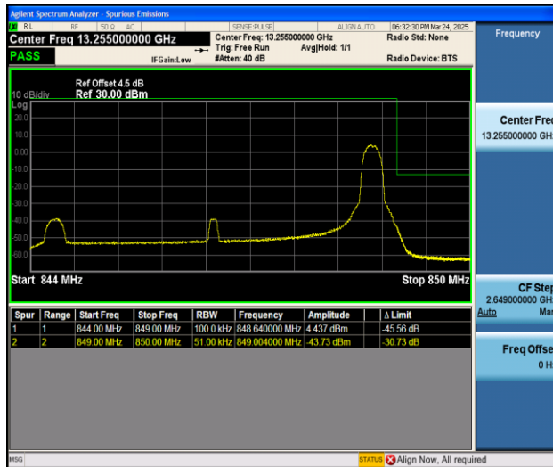
Band5_5MHz_QPSK_20625_1RB#24
