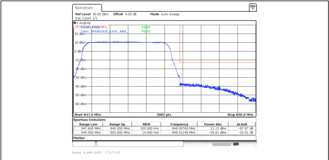
Band5_1.4MHz_16QAM_20643_6RB#0
