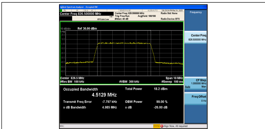
Band5-5MHz-QPSK-20425-25RB#0-PASS
