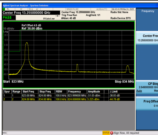
Band5_10MHz_16QAM_20450_1RB#0
