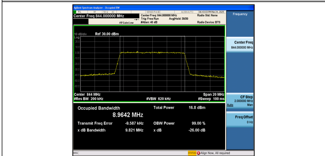
Band5-10MHz-QPSK-20600-50RB#0-PASS
