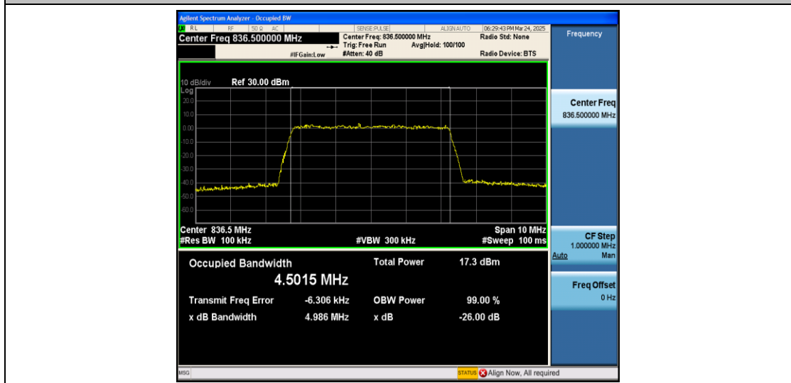
Band5-5MHz-QPSK-20525-25RB#0-PASS
