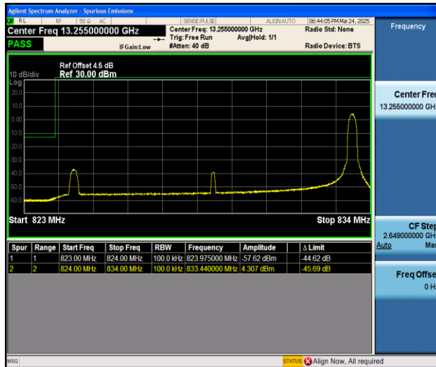
Band5_10MHz_16QAM_20450_1RB#49
