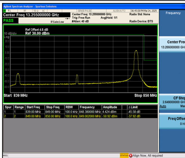
Band5_10MHz_QPSK_20600_1RB#49
