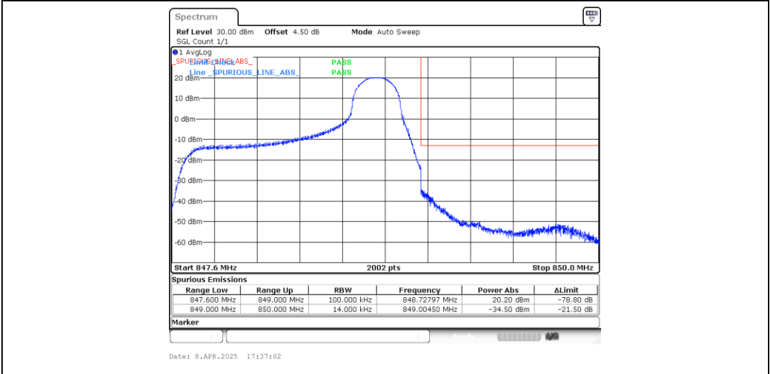
Band5_1.4MHz_QPSK_20643_1RB#5
