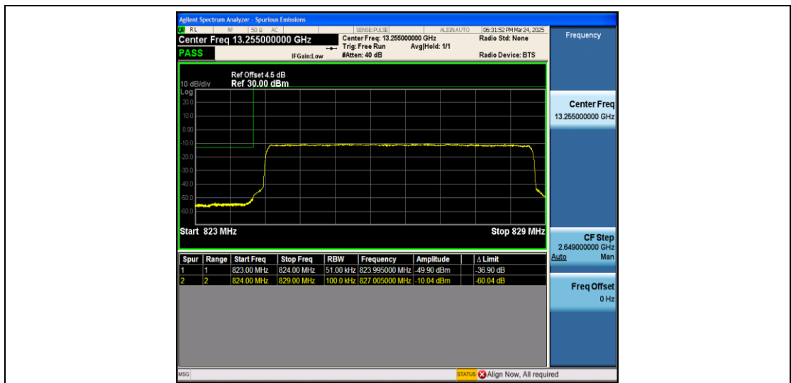
Band5_5MHz_16QAM_20425_25RB#0
