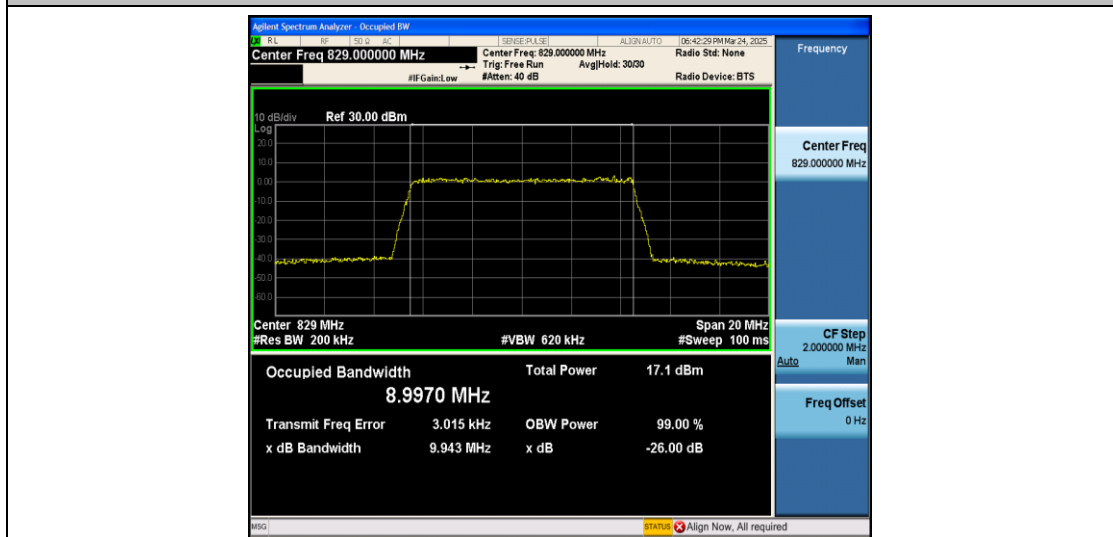
Band5-10MHz-16QAM-20450-50RB#0-PASS
