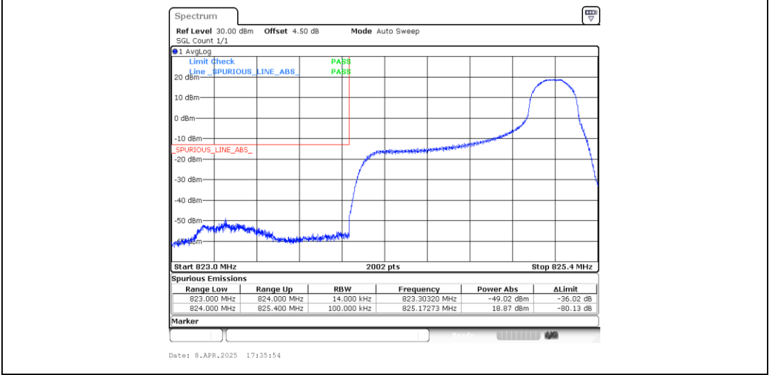
Band5_1.4MHz_16QAM_20407_1RB#5
