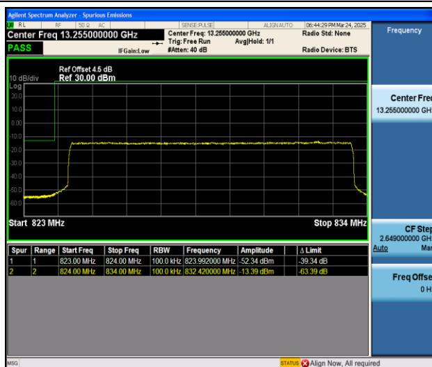
Band5_10MHz_16QAM_20450_50RB#0
