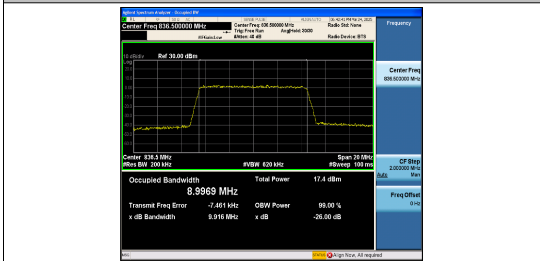
Band5-10MHz-QPSK-20525-50RB#0-PASS
