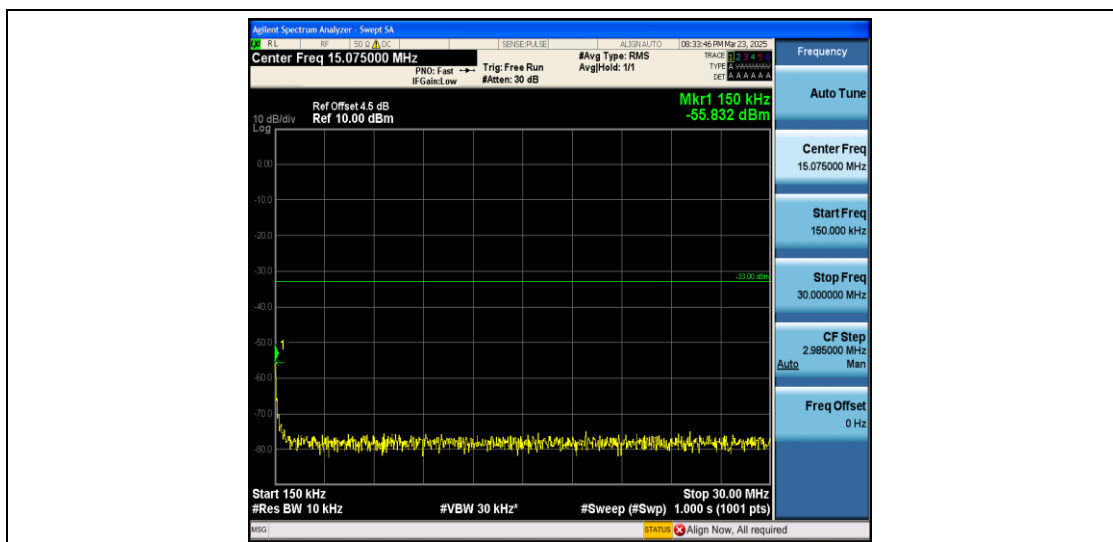
Band4_10MHz_QPSK_20175_1RB#0_0.15~30_0.15~30
