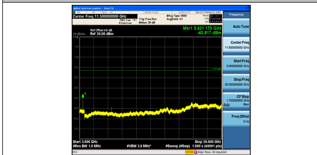
Band4_10MHz_16QAM_20000_1RB#0_3000~20000_3000~20000
