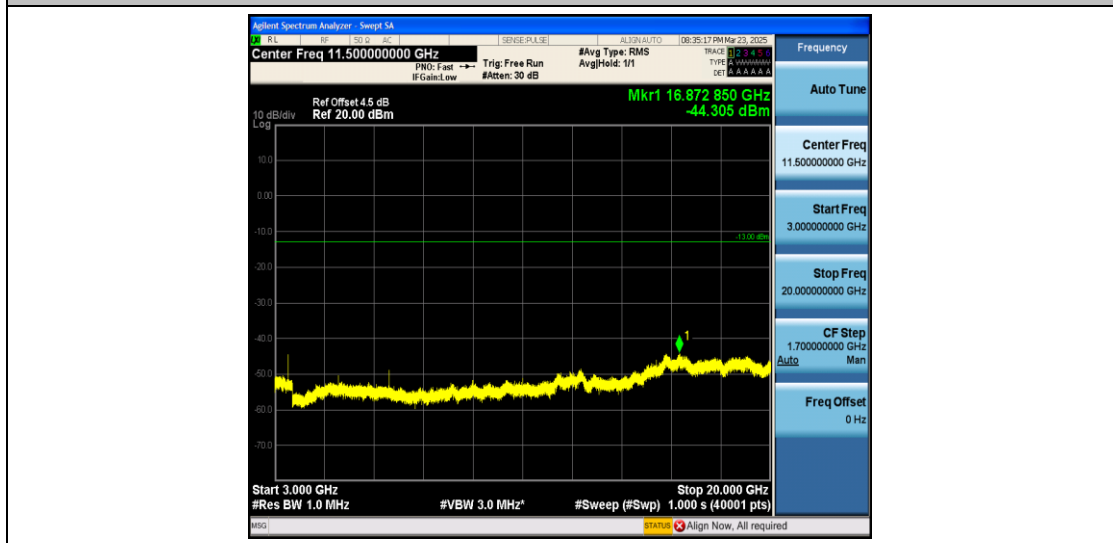
Band4_10MHz_16QAM_20175_1RB#0_3000~20000_3000~20000
