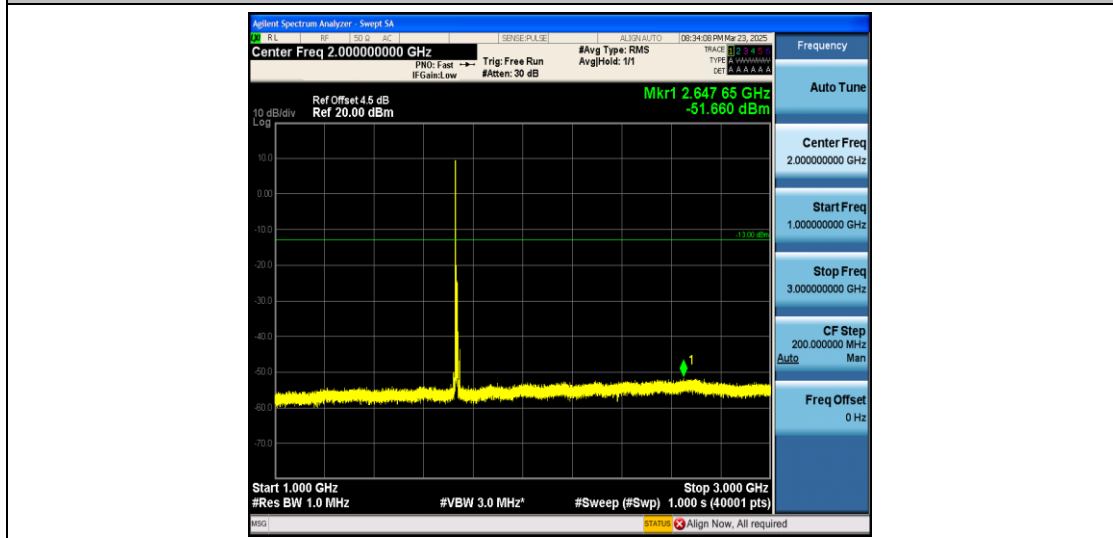
Band4_10MHz_QPSK_20175_1RB#0_1000~3000_1000~3000
