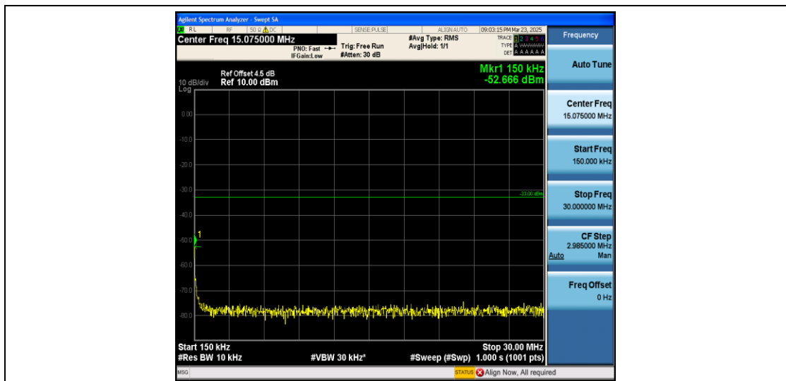
Band4_15MHz_QPSK_20175_1RB#0_0.15~30_0.15~30
