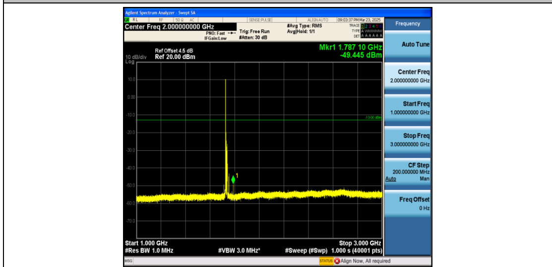
Band4_15MHz_QPSK_20175_1RB#0_1000~3000_1000~3000
