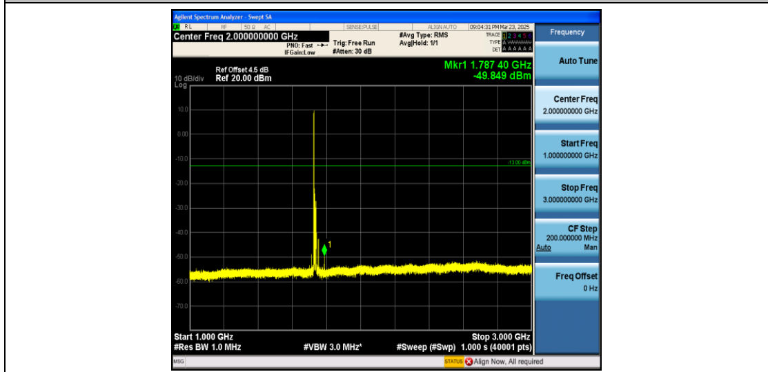
Band4_15MHz_16QAM_20175_1RB#0_1000~3000_1000~3000
