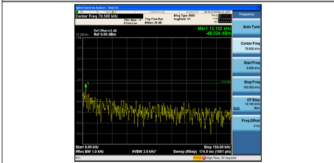
Band4_10MHz_16QAM_20350_1RB#0_0.009~0.15_0.009~0.15
