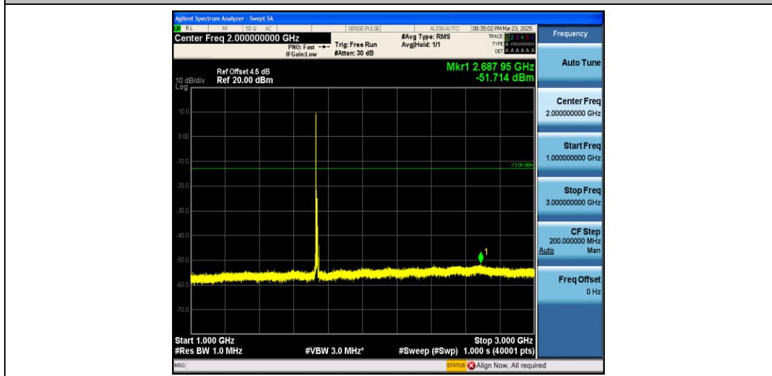
Band4_10MHz_16QAM_20175_1RB#0_1000~3000_1000~3000
