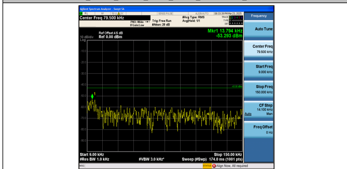
Band4_10MHz_QPSK_20175_1RB#0_0.009~0.15_0.009~0.15
