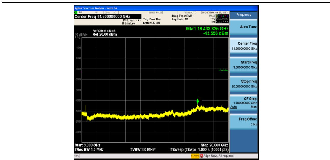
Band4_5MHz_16QAM_20375_1RB#0_3000~20000_3000~20000
