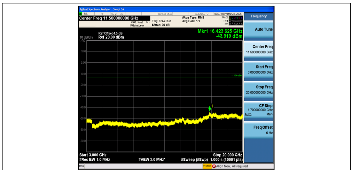
Band4_10MHz_16QAM_20350_1RB#0_3000~20000_3000~20000
