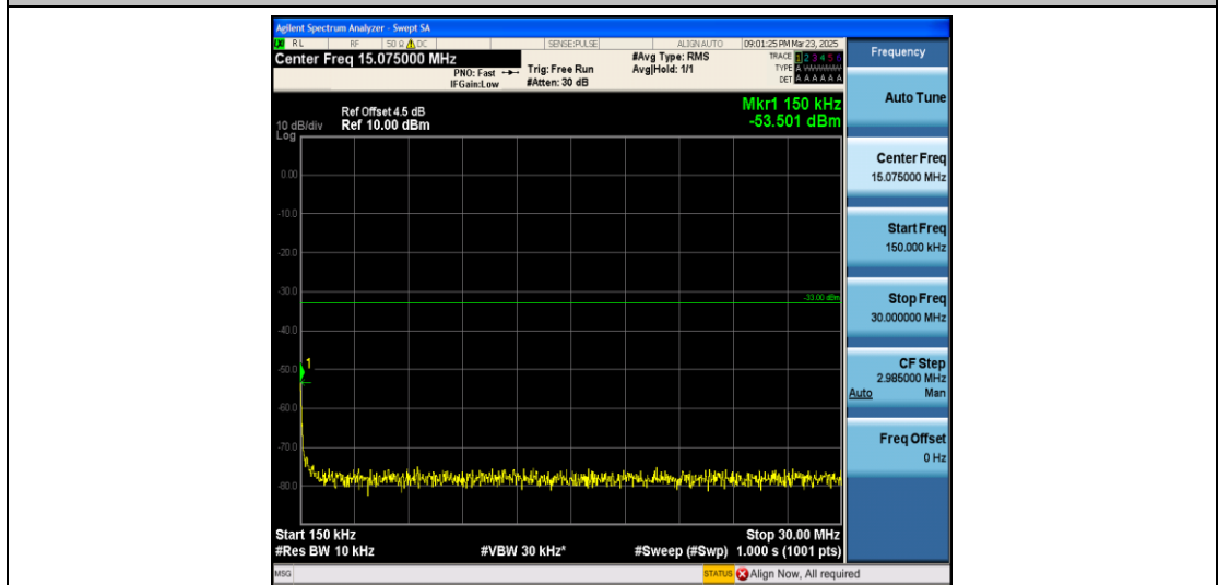
Band4_15MHz_QPSK_20025_1RB#0_0.15~30_0.15~30
