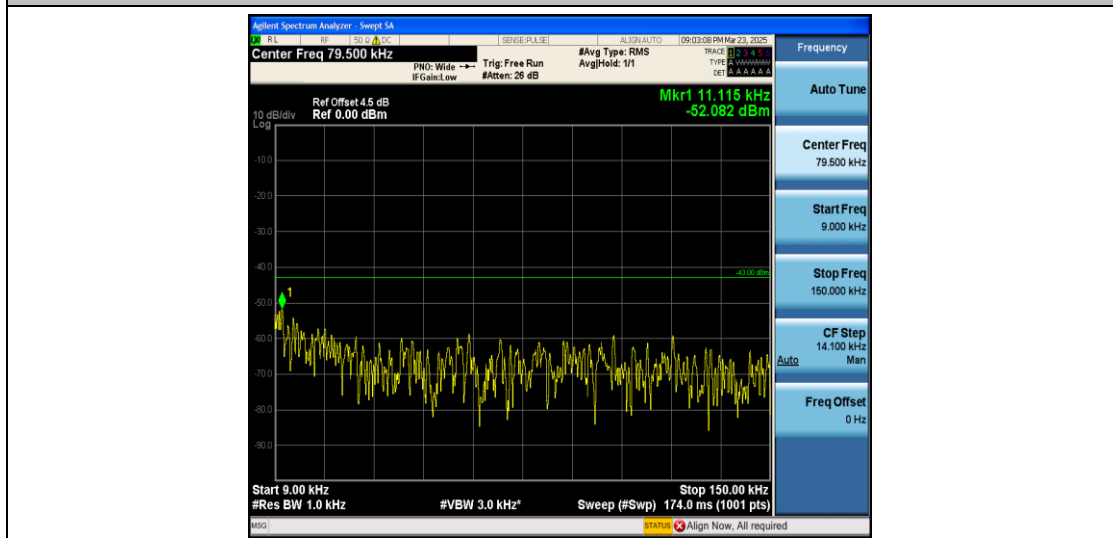
Band4_15MHz_QPSK_20175_1RB#0_0.009~0.15_0.009~0.15
