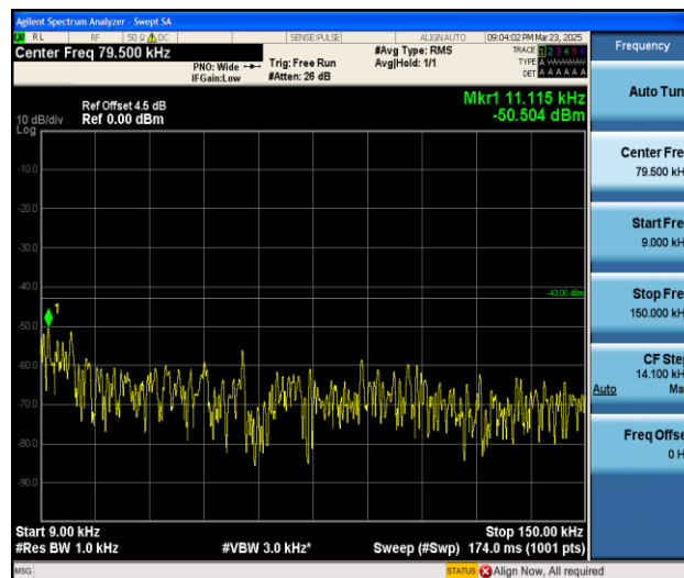
Band4_15MHz_16QAM_20175_1RB#0_0.009~0.15_0.009~0.15
