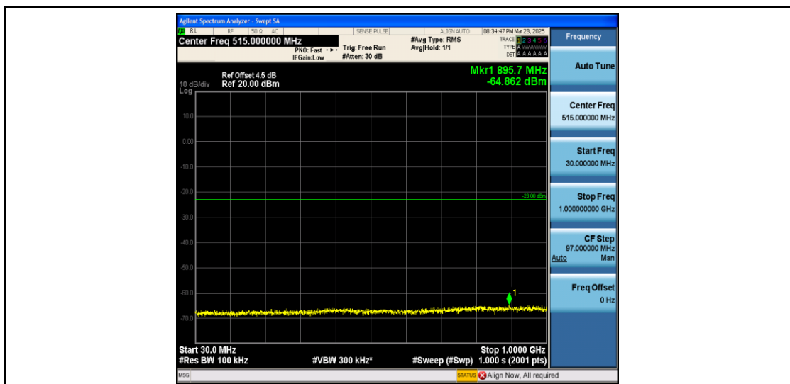
Band4_10MHz_16QAM_20175_1RB#0_30~1000_30~1000
