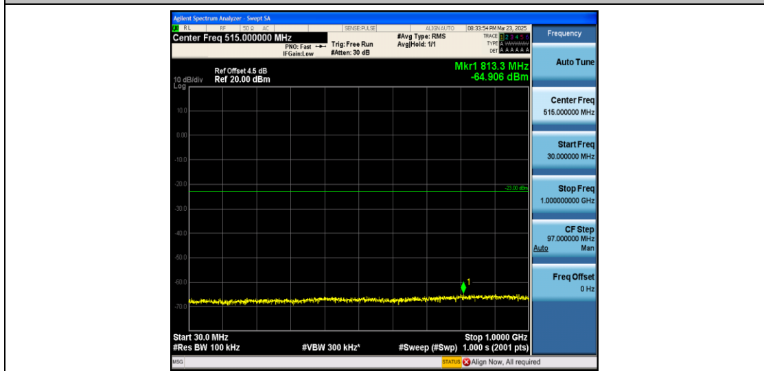
Band4_10MHz_QPSK_20175_1RB#0_30~1000_30~1000
