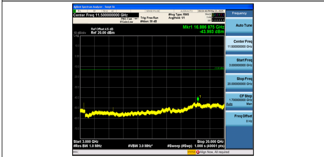
Band4_15MHz_16QAM_20175_1RB#0_3000~20000_3000~20000
