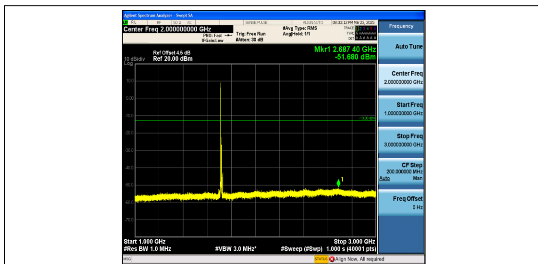
Band4_10MHz_16QAM_20000_1RB#0_1000~3000_1000~3000
