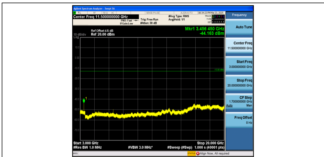
Band4_10MHz_QPSK_20175_1RB#0_3000~20000_3000~20000
