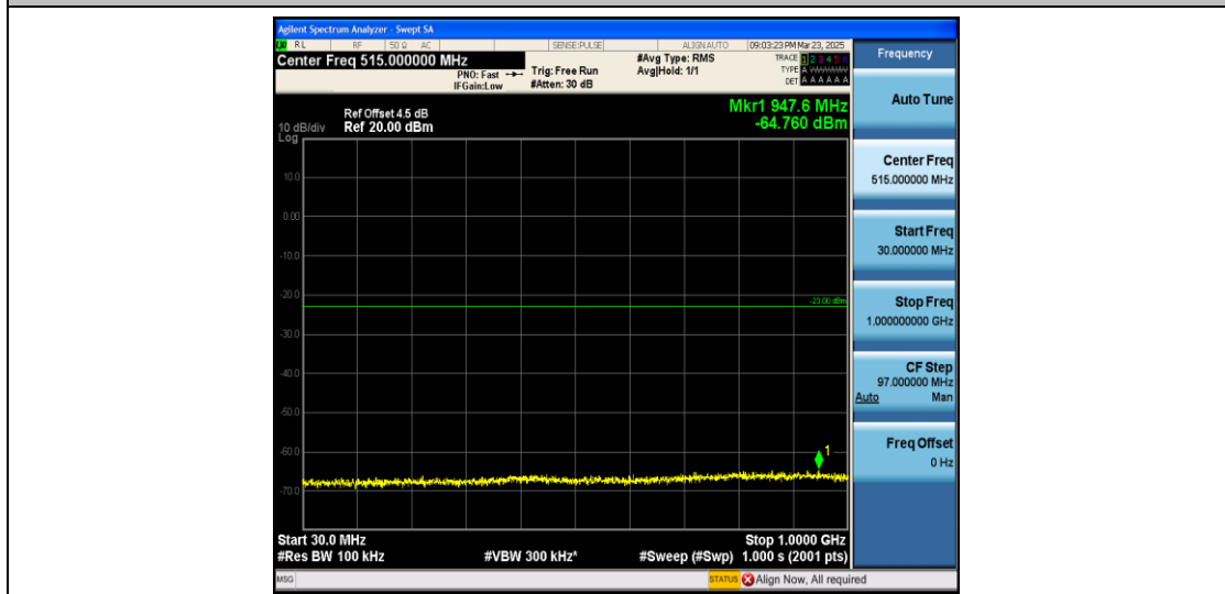
Band4_15MHz_QPSK_20175_1RB#0_30~1000_30~1000
