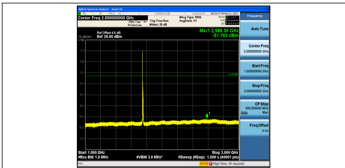
Band4_10MHz_QPSK_20350_1RB#0_1000~3000_1000~3000
