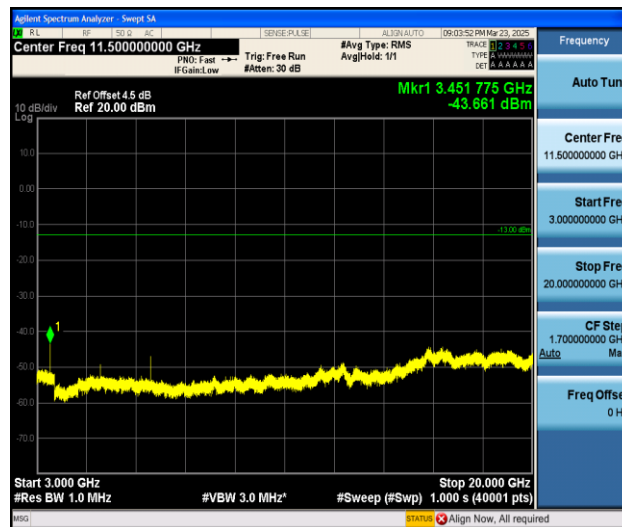
Band4_15MHz_QPSK_20175_1RB#0_3000~20000_3000~20000
