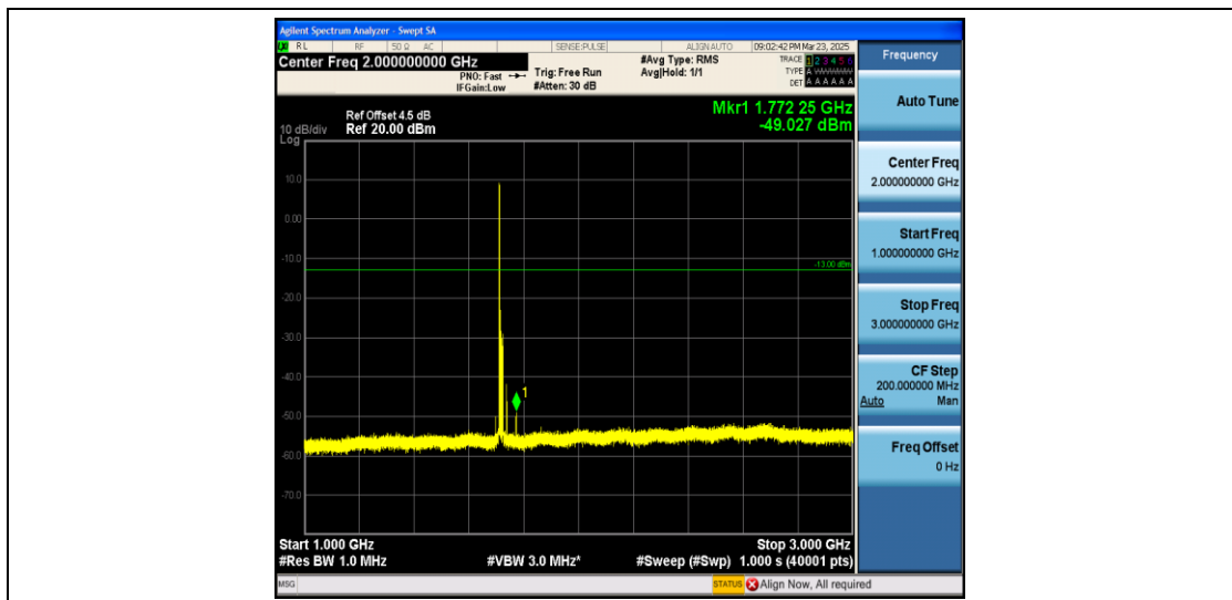
Band4_15MHz_16QAM_20025_1RB#0_1000~3000_1000~3000
