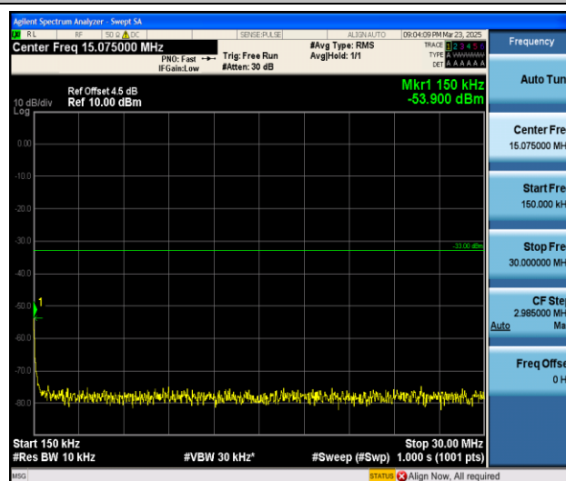
Band4_15MHz_16QAM_20175_1RB#0_0.15~30_0.15~30
