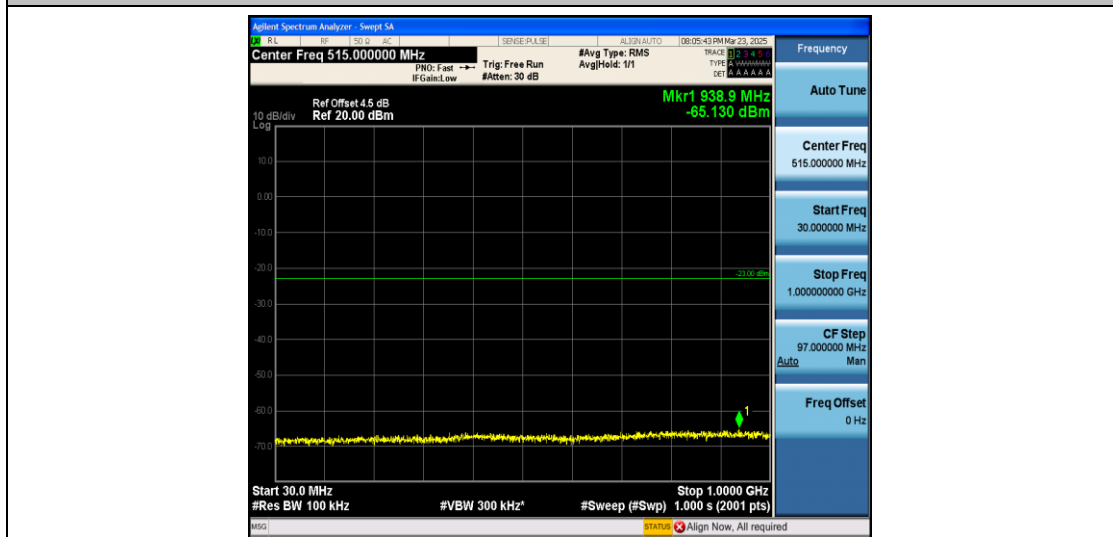
Band4_5MHz_QPSK_20175_1RB#0_30~1000_30~1000
