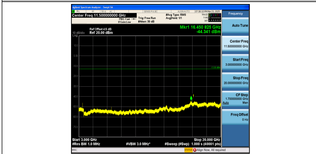
Band4_3MHz_16QAM_20175_1RB#0_3000~20000_3000~20000
