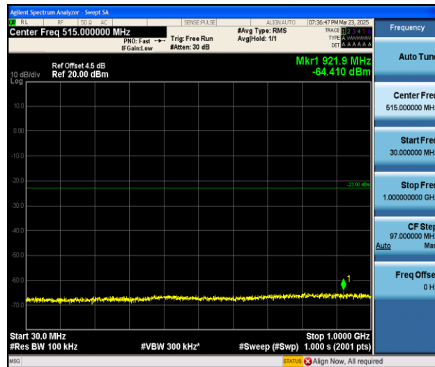
Band4_3MHz_QPSK_20175_1RB#0_30~1000_30~1000
