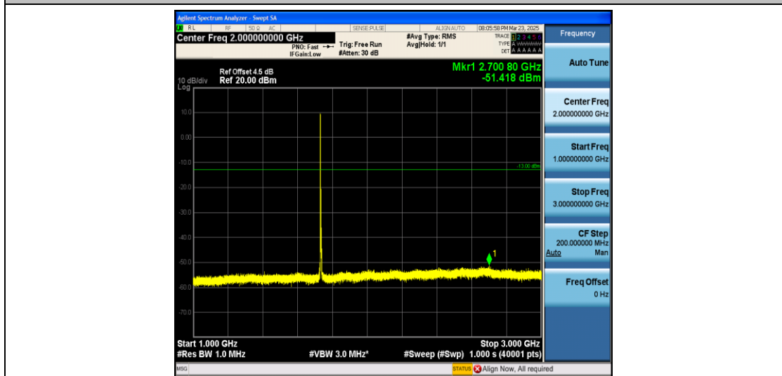
Band4_5MHz_QPSK_20175_1RB#0_1000~3000_1000~3000
