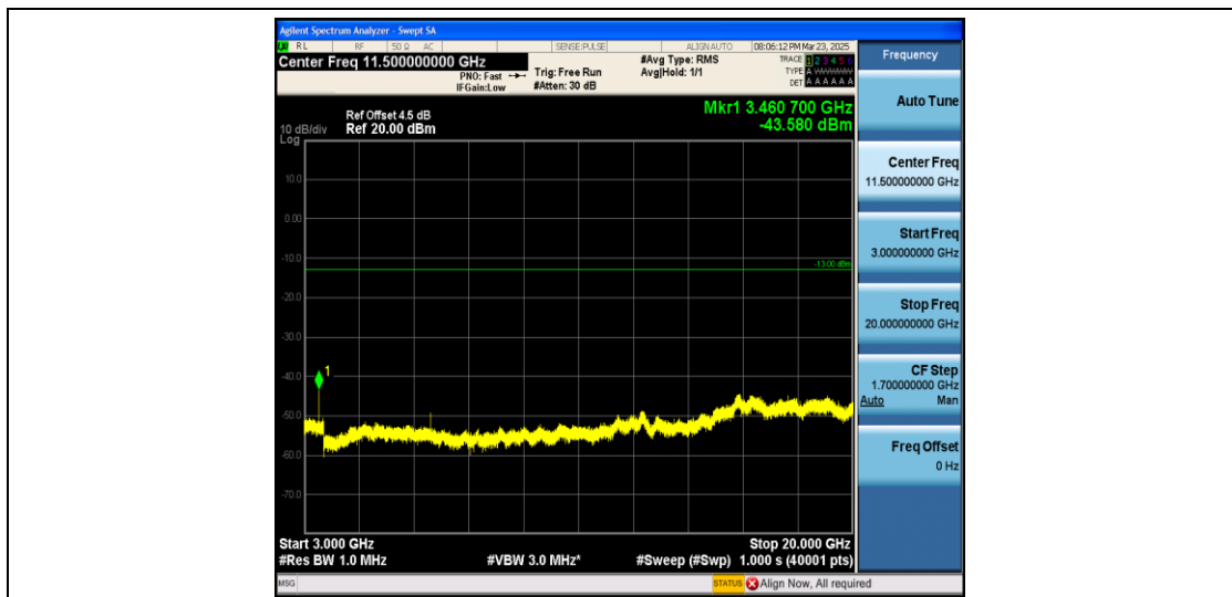
Band4_5MHz_QPSK_20175_1RB#0_3000~20000_3000~20000
