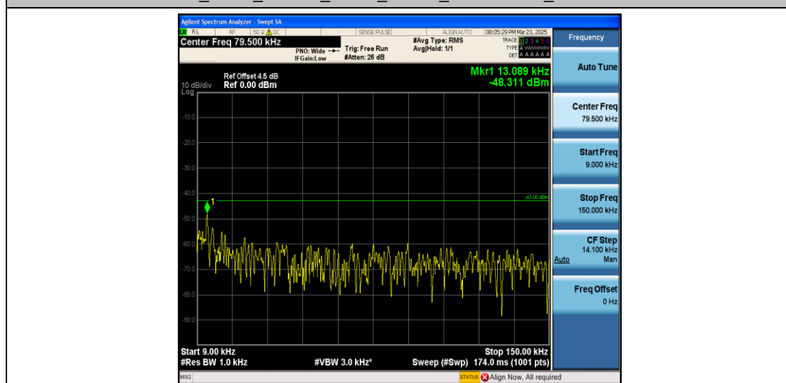
Band4_5MHz_QPSK_20175_1RB#0_0.009~0.15_0.009~0.15
