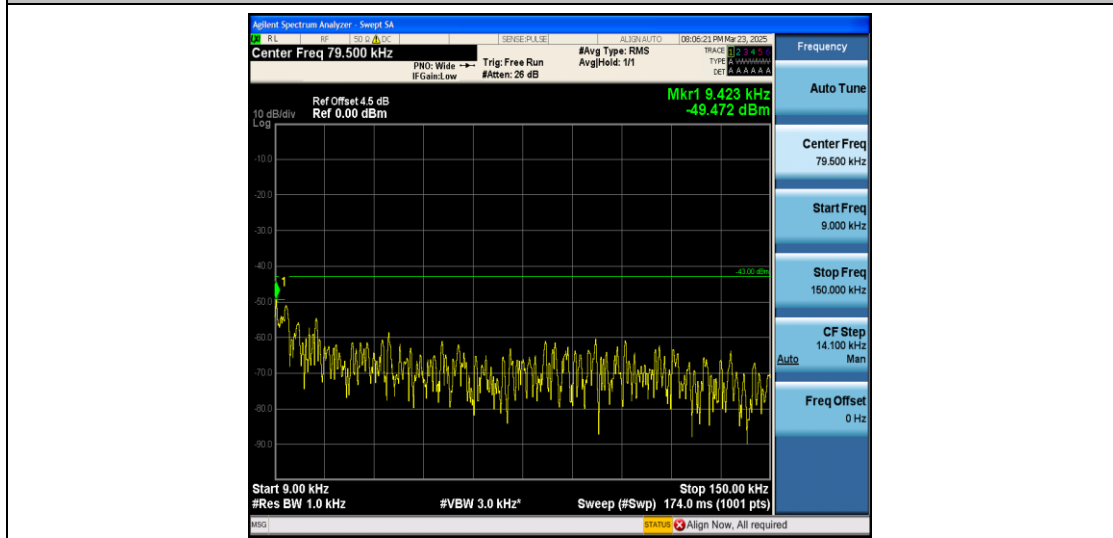
Band4_5MHz_16QAM_20175_1RB#0_0.009~0.15_0.009~0.15
