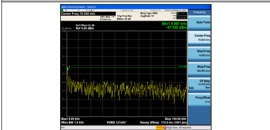
Band4_5MHz_QPSK_19975_1RB#0_0.009~0.15_0.009~0.15
