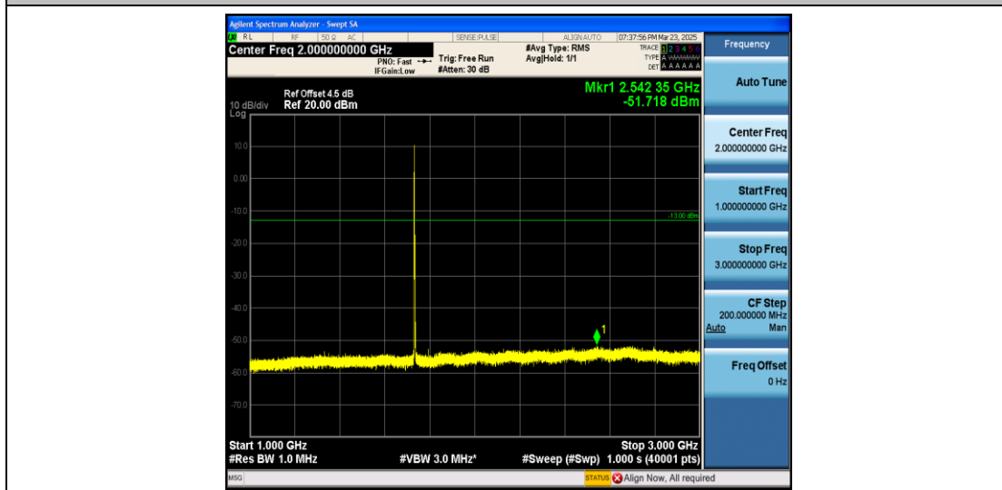
Band4_3MHz_16QAM_20175_1RB#0_1000~3000_1000~3000
