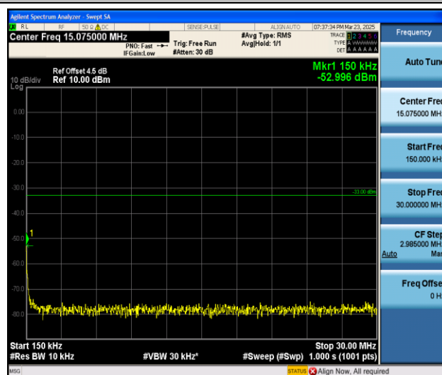
Band4_3MHz_16QAM_20175_1RB#0_0.15~30_0.15~30
