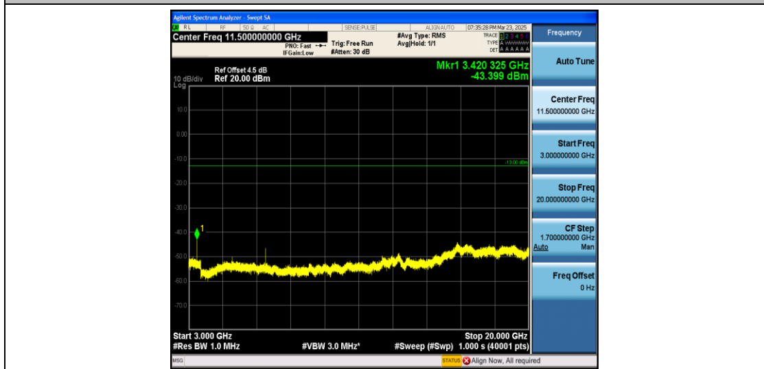
Band4_3MHz_QPSK_19965_1RB#0_3000~20000_3000~20000
