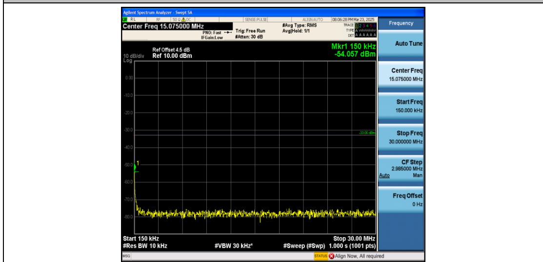
Band4_5MHz_16QAM_20175_1RB#0_0.15~30_0.15~30
