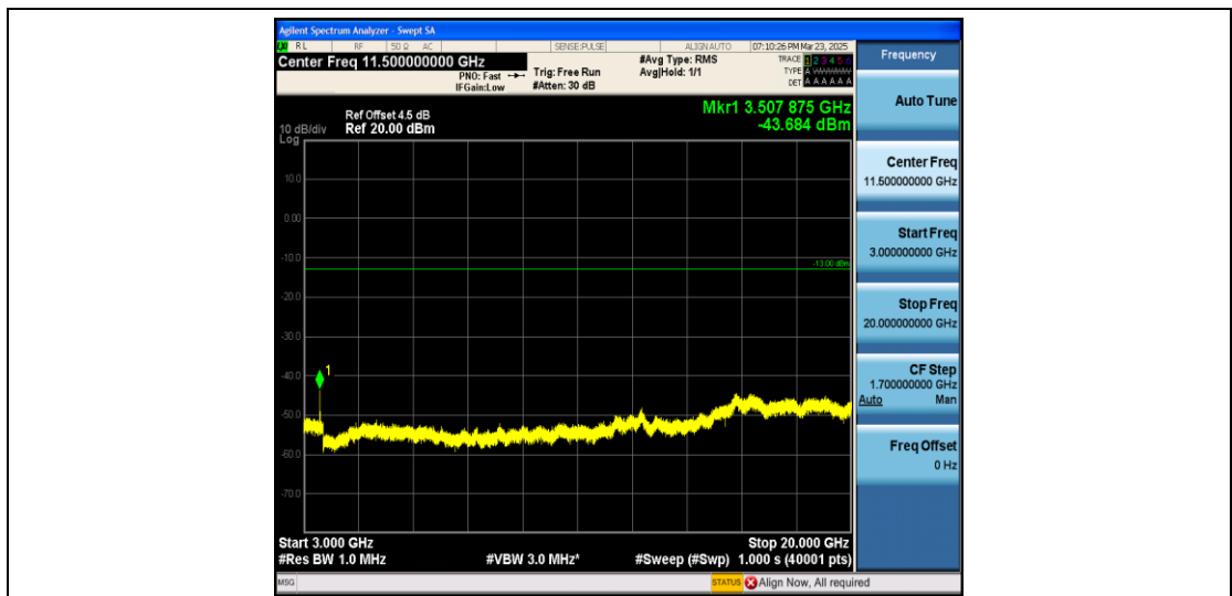
Band4_1.4MHz_16QAM_20393_1RB#0_3000~20000_3000~20000
