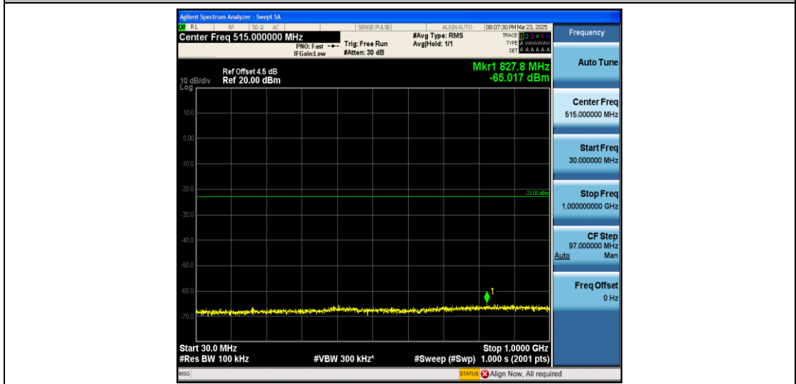
Band4_5MHz_QPSK_20375_1RB#0_30~1000_30~1000
