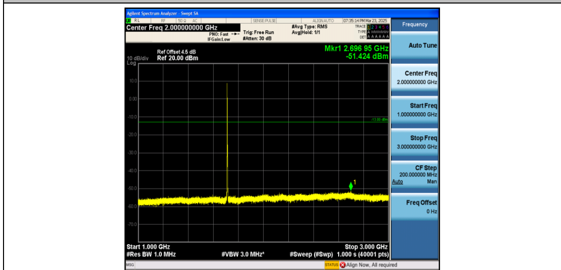
Band4_3MHz_QPSK_19965_1RB#0_1000~3000_1000~3000
