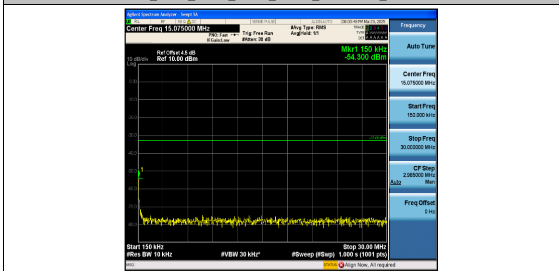
Band4_5MHz_QPSK_19975_1RB#0_0.15~30_0.15~30
