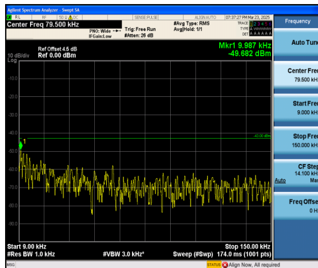
Band4_3MHz_16QAM_20175_1RB#0_0.009~0.15_0.009~0.15
