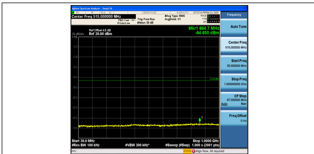
Band4_3MHz_16QAM_20175_1RB#0_30~1000_30~1000
