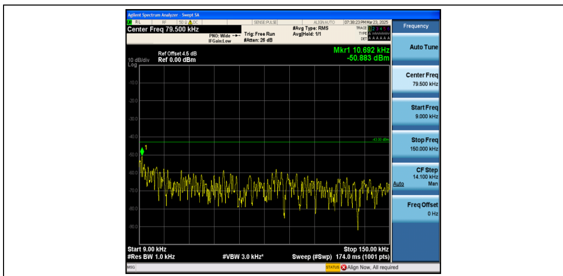
Band4_3MHz_QPSK_20385_1RB#0_0.009~0.15_0.009~0.15
