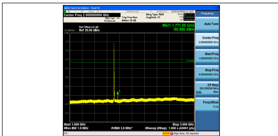
Band4_5MHz_16QAM_19975_1RB#0_1000~3000_1000~3000
