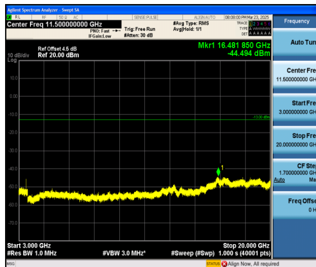
Band4_5MHz_QPSK_20375_1RB#0_3000~20000_3000~20000
