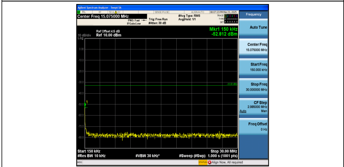
Band4_5MHz_QPSK_20375_1RB#0_0.15~30_0.15~30
