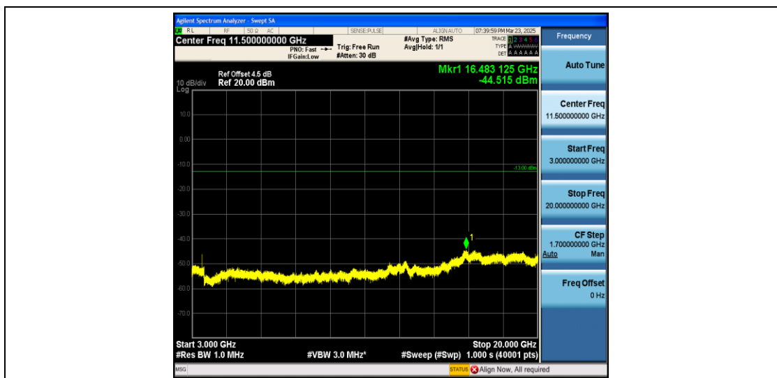
Band4_3MHz_16QAM_20385_1RB#0_3000~20000_3000~20000
