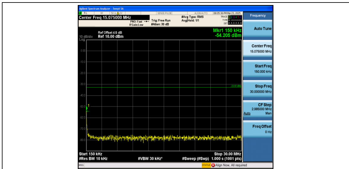
Band4_5MHz_QPSK_20175_1RB#0_0.15~30_0.15~30
