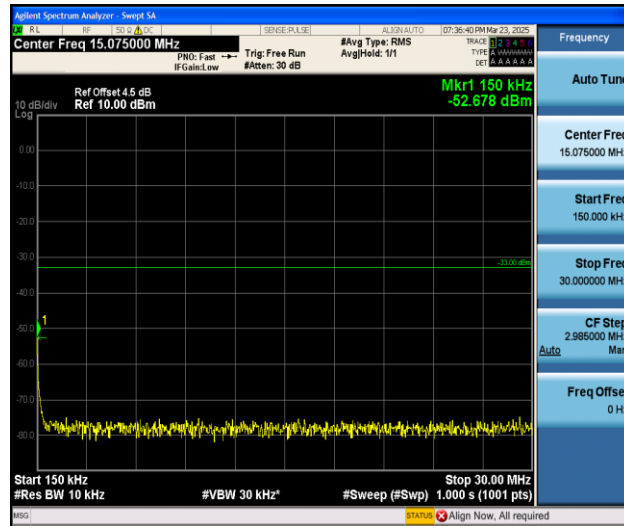
Band4_3MHz_QPSK_20175_1RB#0_0.15~30_0.15~30
