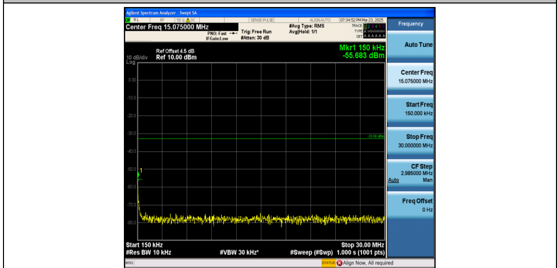
Band4_3MHz_QPSK_19965_1RB#0_0.15~30_0.15~30
