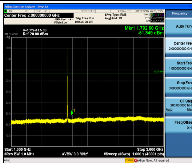
Band4_3MHz_QPSK_20175_1RB#0_1000~3000_1000~3000
