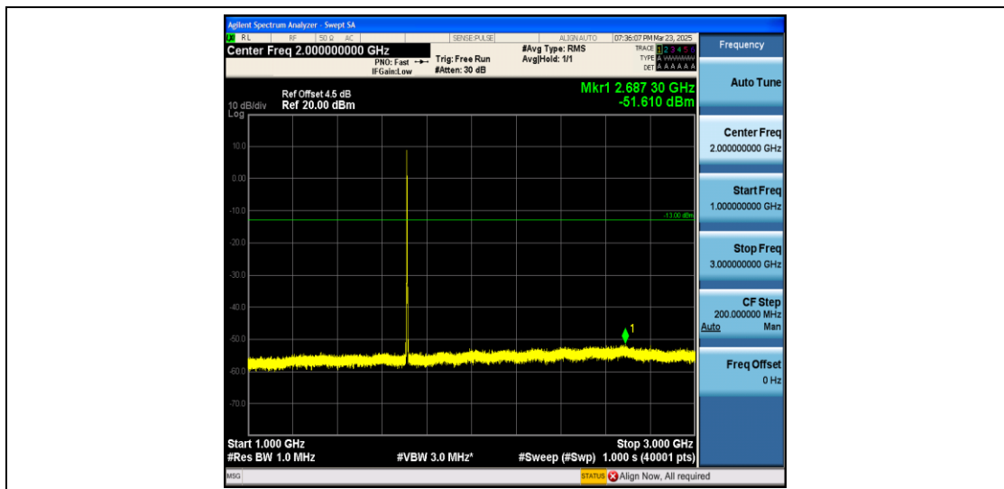
Band4_3MHz_16QAM_19965_1RB#0_1000~3000_1000~3000
