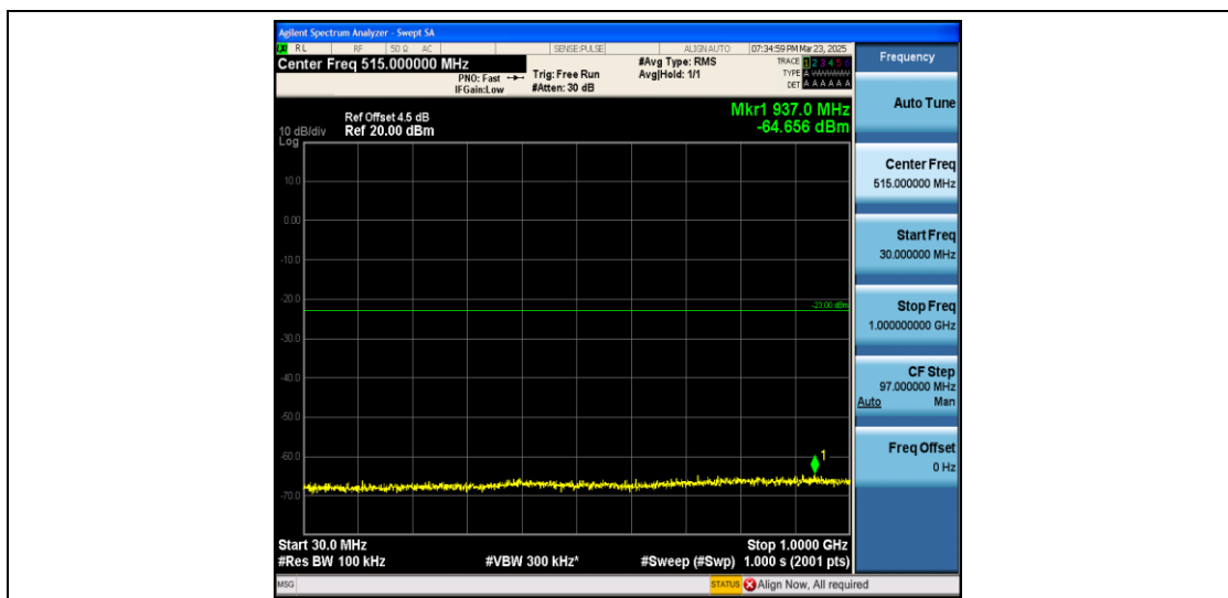
Band4_3MHz_QPSK_19965_1RB#0_30~1000_30~1000
