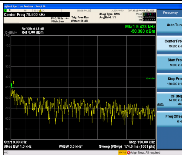
Band4_3MHz_16QAM_20385_1RB#0_0.009~0.15_0.009~0.15
