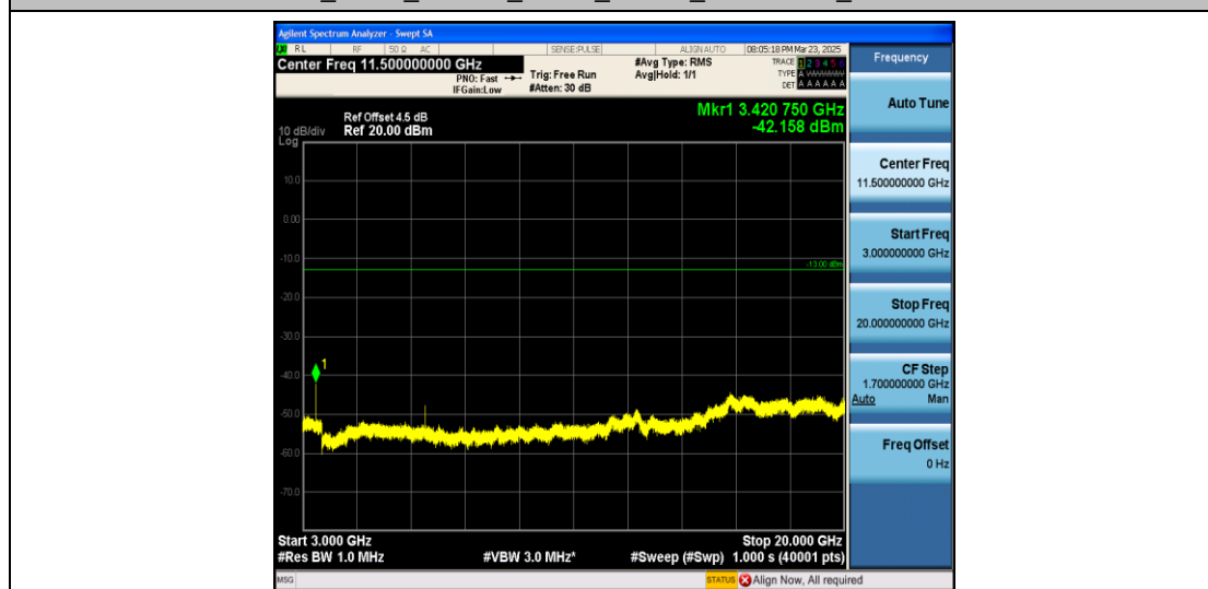
Band4_5MHz_16QAM_19975_1RB#0_3000~20000_3000~20000
