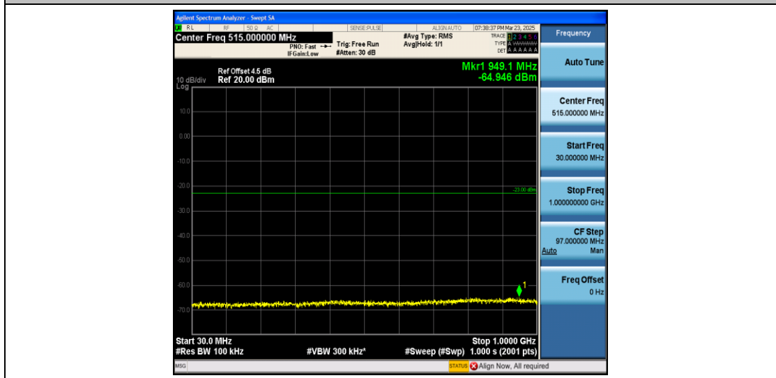
Band4_3MHz_QPSK_20385_1RB#0_30~1000_30~1000
