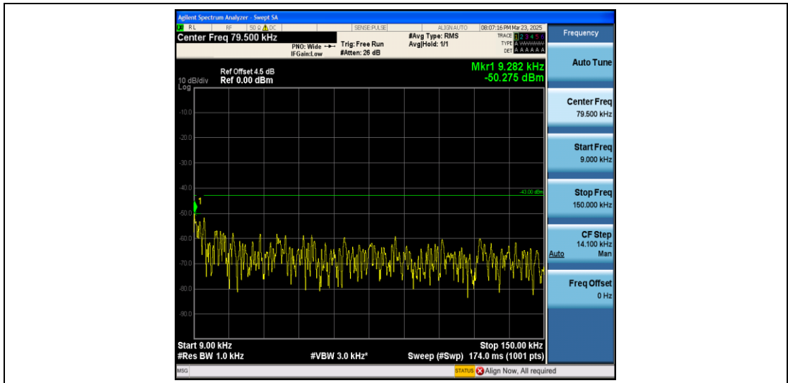
Band4_5MHz_QPSK_20375_1RB#0_0.009~0.15_0.009~0.15
