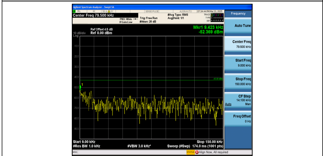
Band4_3MHz_QPSK_19965_1RB#0_0.009~0.15_0.009~0.15
