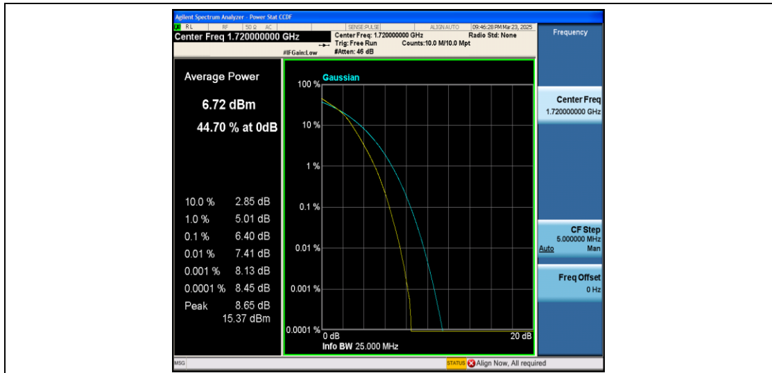
Band4-20MHz-16QAM-20050-100RB#0-PASS
