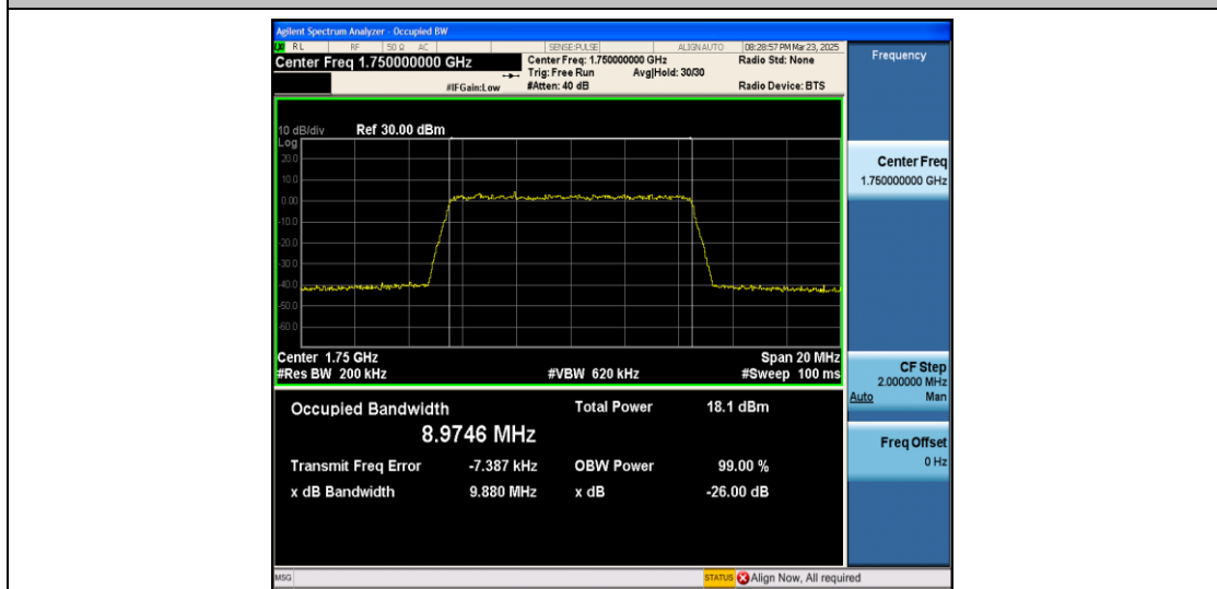
Band4-10MHz-QPSK-20350-50RB#0-PASS
