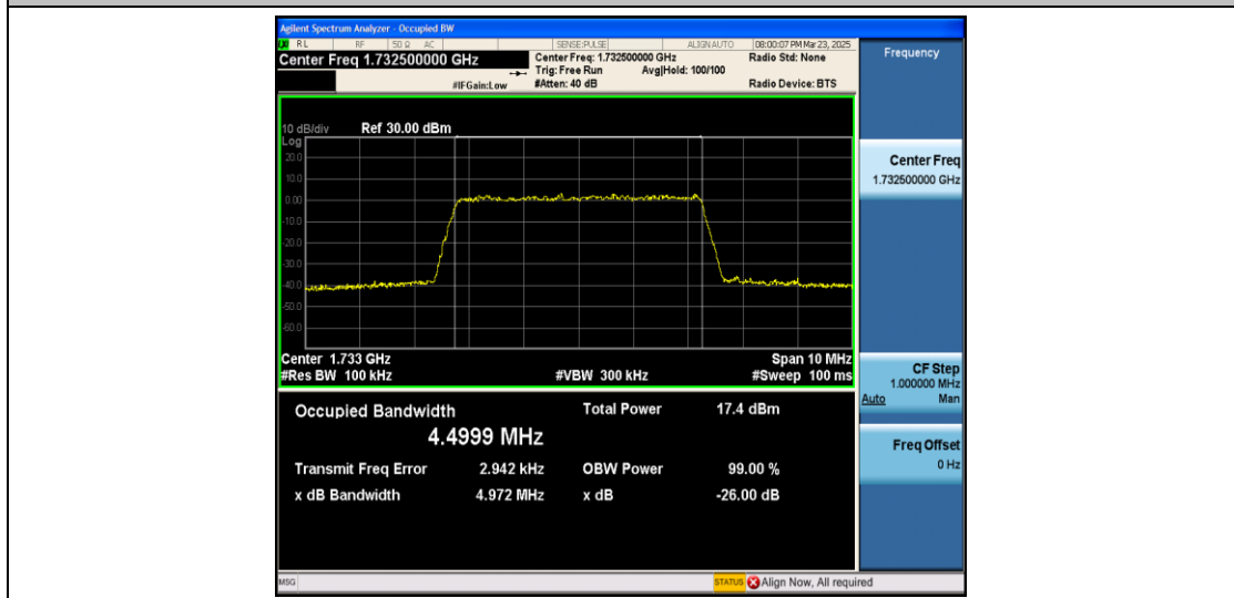
Band4-5MHz-QPSK-20175-25RB#0-PASS
