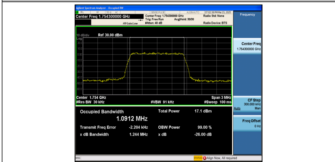
Band4-1.4MHz-QPSK-20393-6RB#0-PASS
