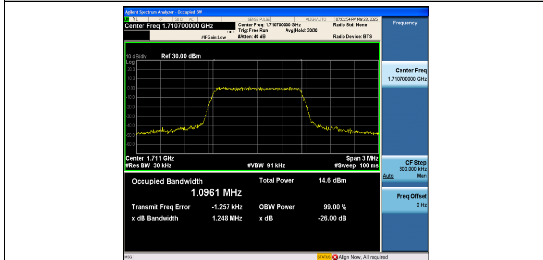
Band4-1.4MHz-16QAM-19957-6RB#0-PASS
