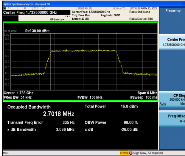
Band4-3MHz-16QAM-20175-15RB#0-PASS
