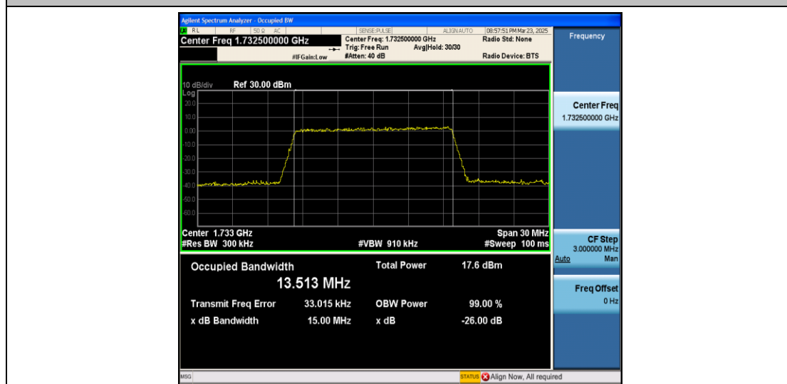
Band4-15MHz-QPSK-20175-75RB#0-PASS
