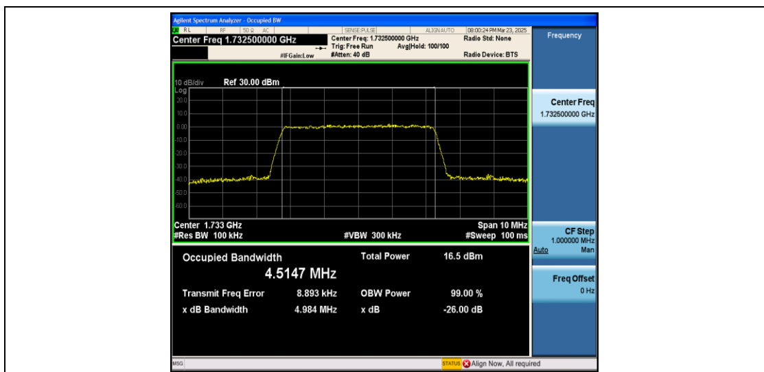
Band4-5MHz-16QAM-20175-25RB#0-PASS
