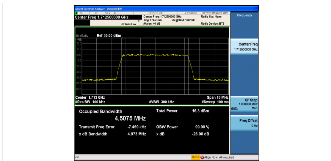
Band4-5MHz-QPSK-19975-25RB#0-PASS
