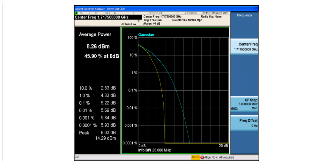
Band4-15MHz-QPSK-20025-1RB#0-PASS
