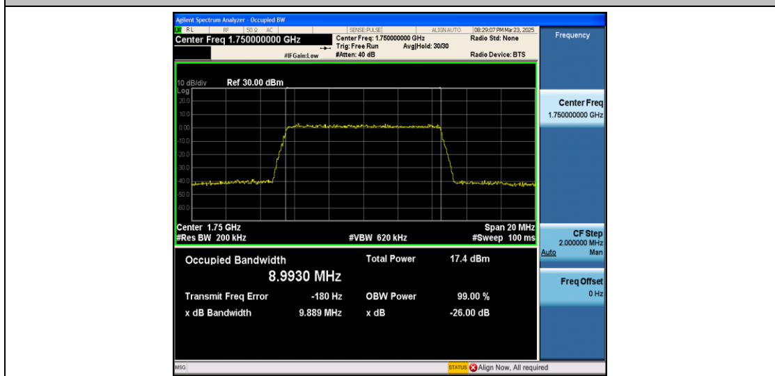
Band4-10MHz-16QAM-20350-50RB#0-PASS
