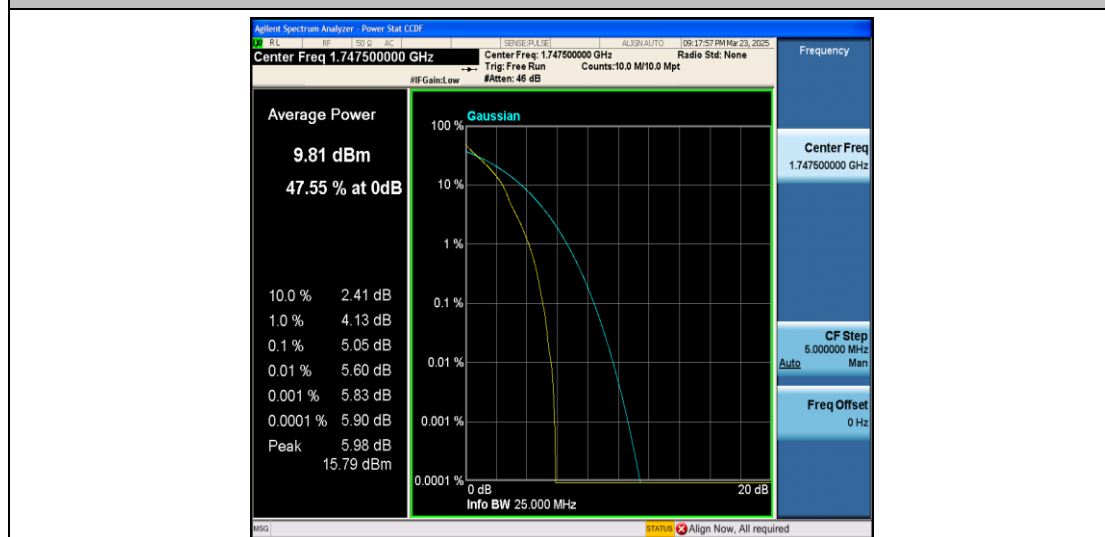
Band4-15MHz-QPSK-20325-1RB#0-PASS
