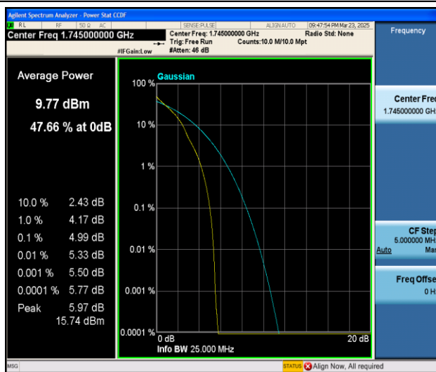
Band4-20MHz-QPSK-20300-1RB#0-PASS
