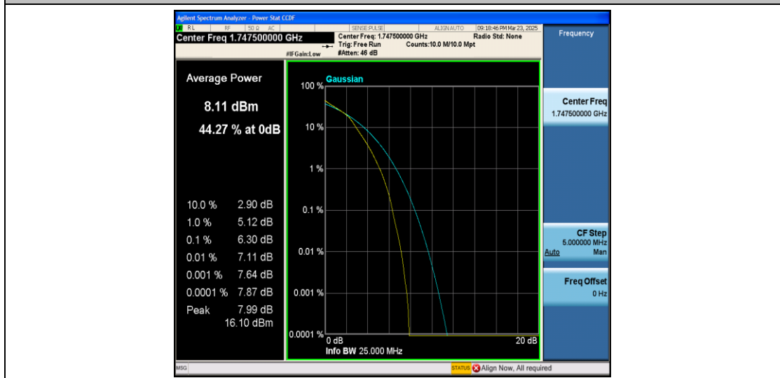
Band4-15MHz-16QAM-20325-75RB#0-PASS
