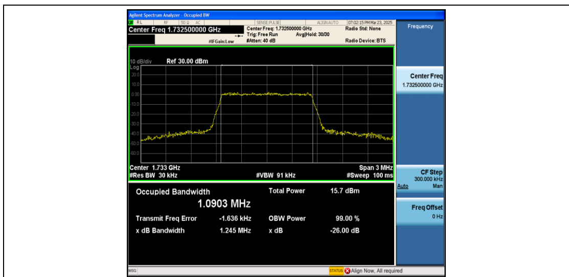
Band4-1.4MHz-16QAM-20175-6RB#0-PASS
