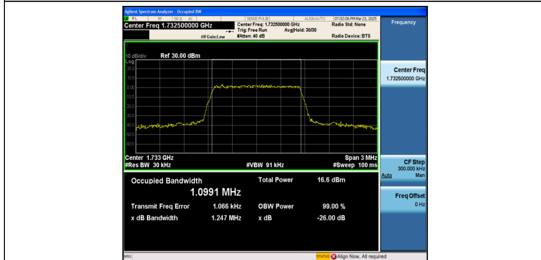
Band4-1.4MHz-QPSK-20175-6RB#0-PASS
