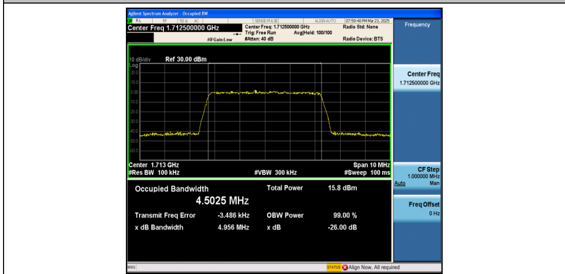
Band4-5MHz-16QAM-19975-25RB#0-PASS
