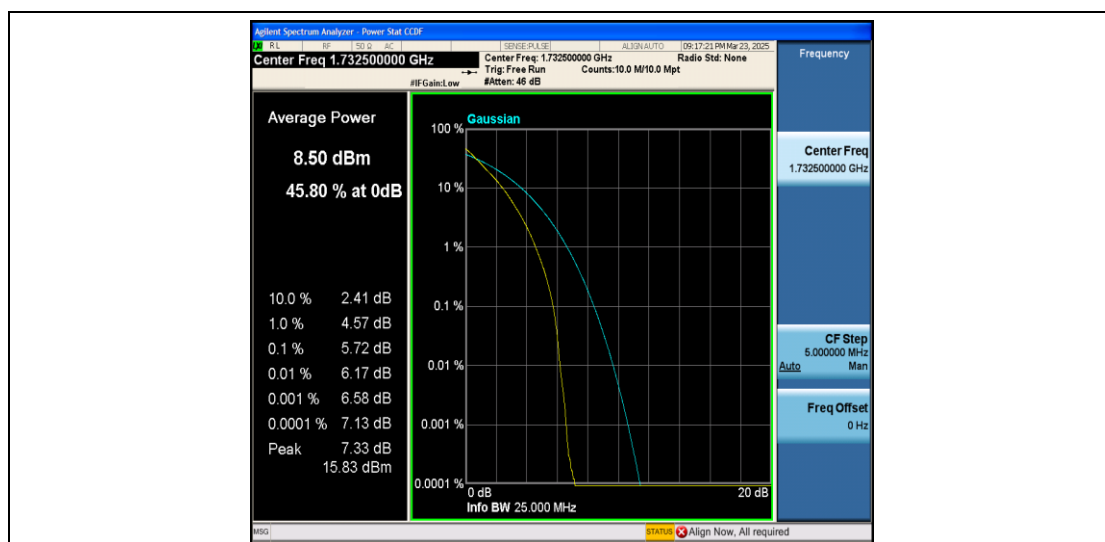
Band4-15MHz-QPSK-20175-75RB#0-PASS
