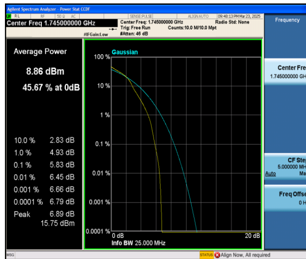
Band4-20MHz-16QAM-20300-1RB#0-PASS
