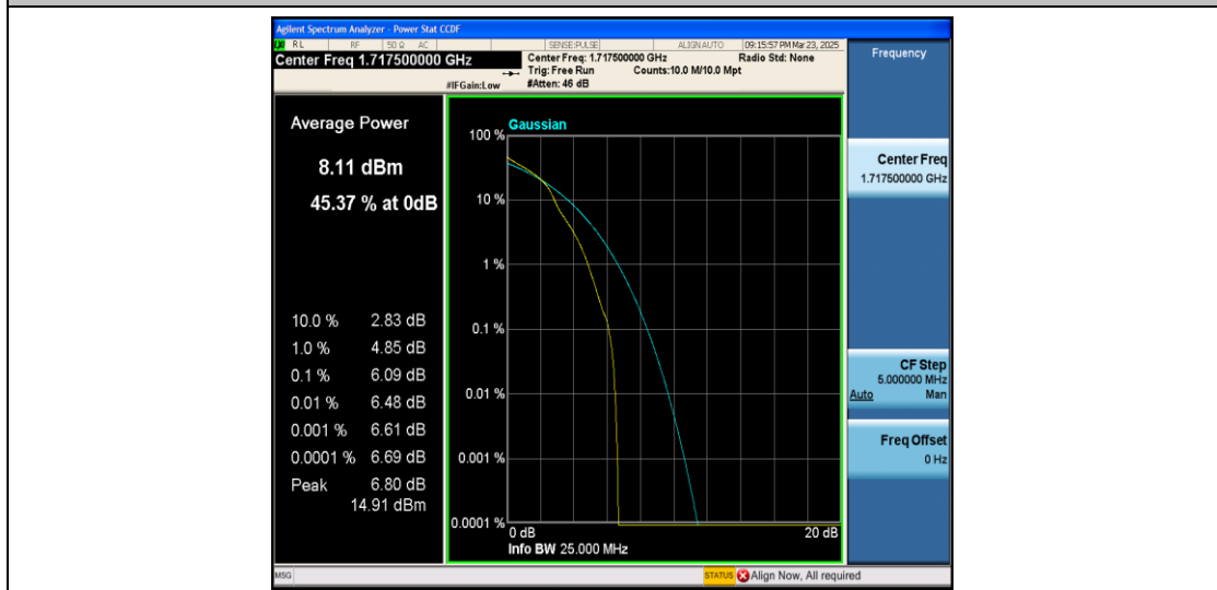
Band4-15MHz-16QAM-20025-1RB#0-PASS
