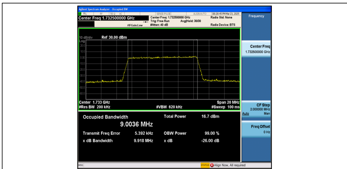
Band4-10MHz-16QAM-20175-50RB#0-PASS
