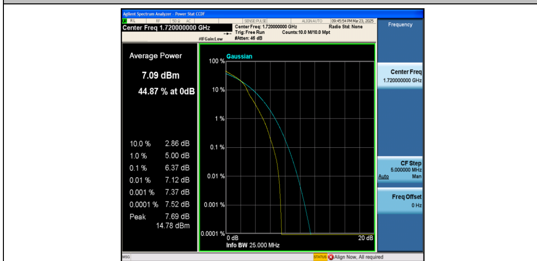
Band4-20MHz-16QAM-20050-1RB#0-PASS
