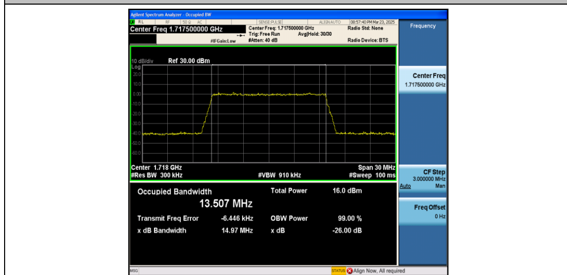
Band4-15MHz-16QAM-20025-75RB#0-PASS
