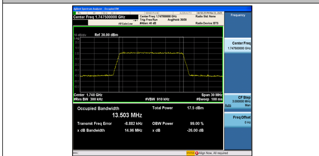
Band4-15MHz-16QAM-20325-75RB#0-PASS
