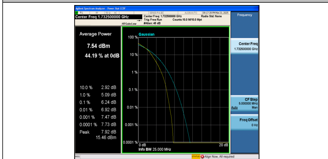
Band4-15MHz-16QAM-20175-75RB#0-PASS
