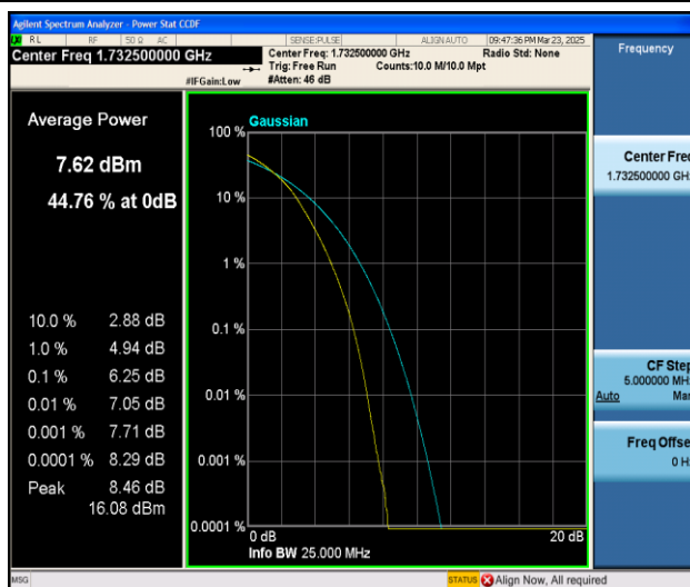
Band4-20MHz-16QAM-20175-100RB#0-PASS
