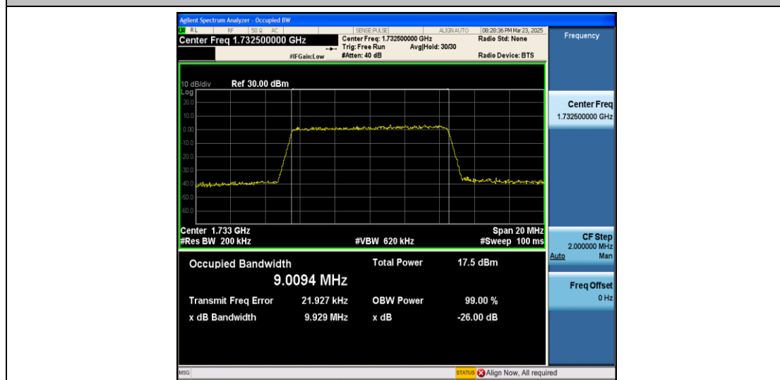
Band4-10MHz-QPSK-20175-50RB#0-PASS
