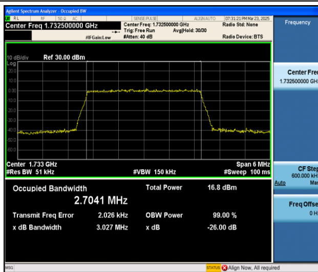
Band4-3MHz-QPSK-20175-15RB#0-PASS
