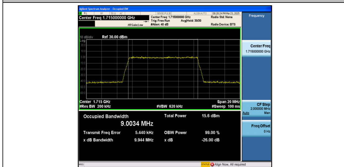
Band4-10MHz-16QAM-20000-50RB#0-PASS
