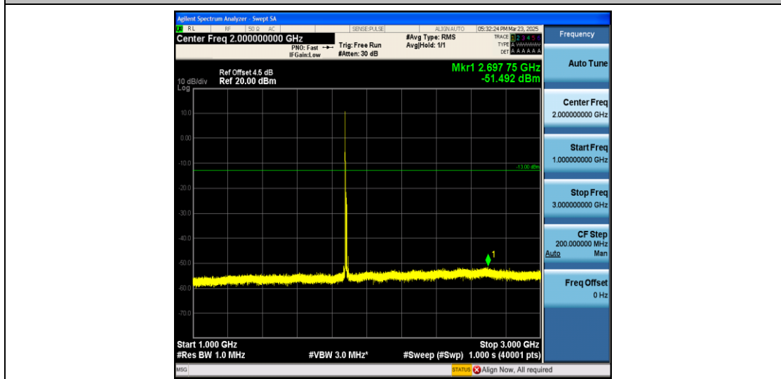
Band2_10MHz_16QAM_18900_1RB#0_1000~3000_1000~3000
