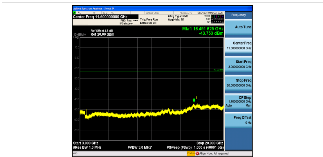
Band2_5MHz_16QAM_19175_1RB#0_3000~20000_3000~20000
