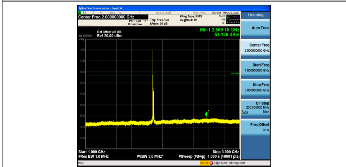
Band2_15MHz_16QAM_18900_1RB#0_1000~3000_1000~3000
