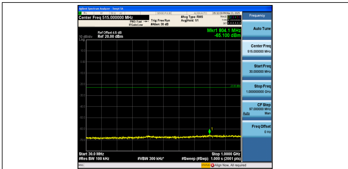
Band2_10MHz_16QAM_18900_1RB#0_30~1000_30~1000
