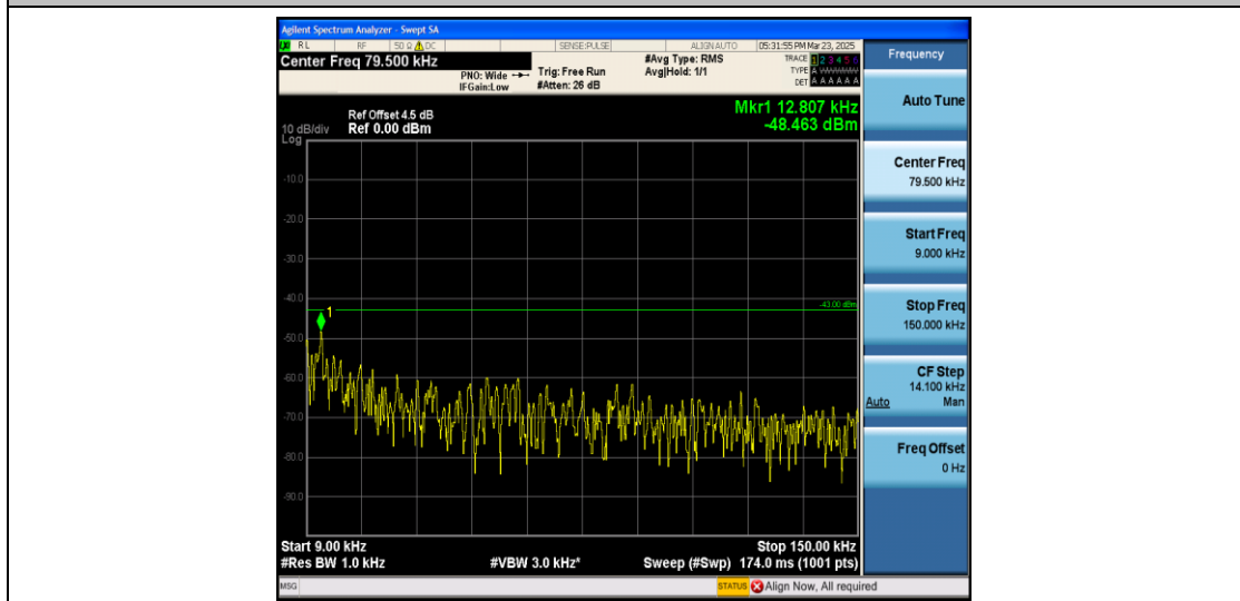
Band2_10MHz_16QAM_18900_1RB#0_0.009~0.15_0.009~0.15
