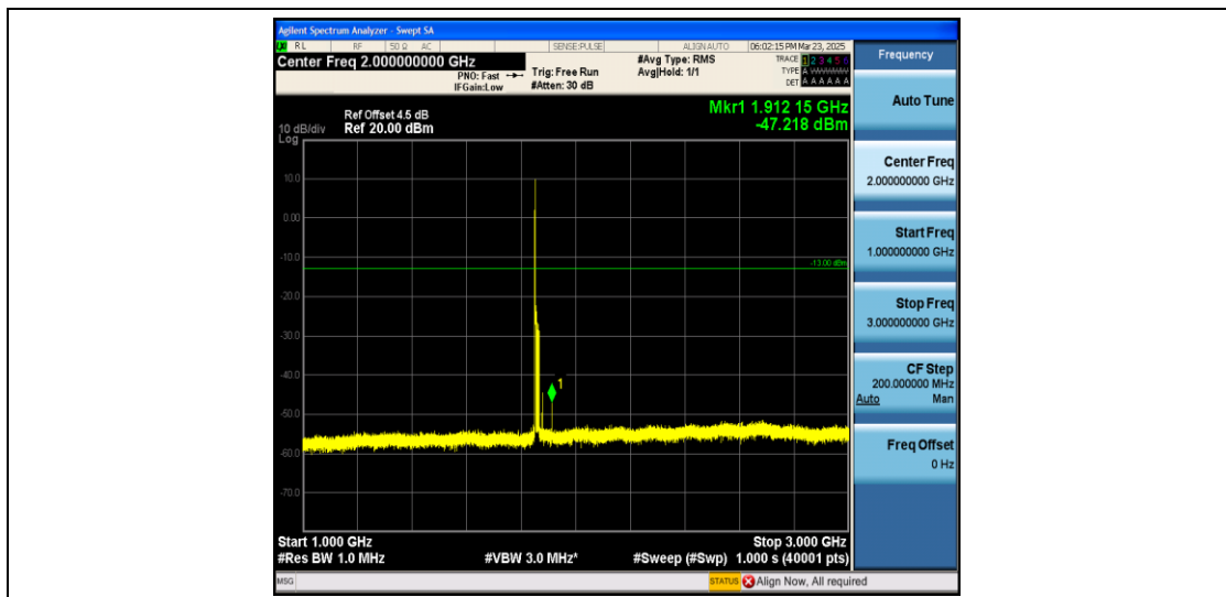
Band2_15MHz_16QAM_18675_1RB#0_1000~3000_1000~3000
