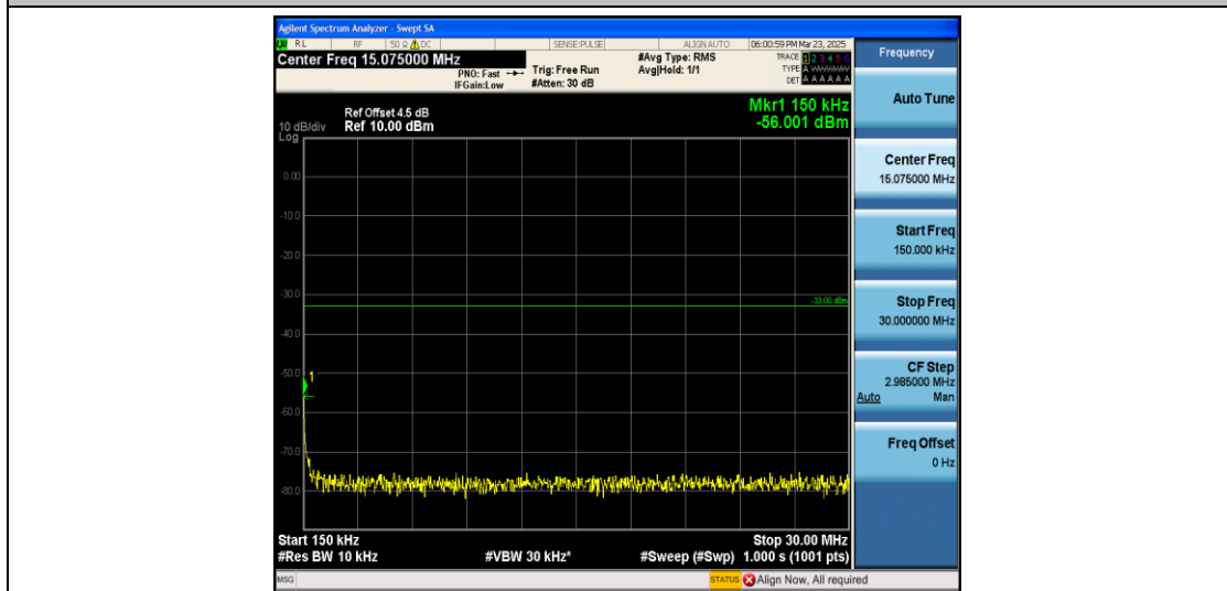
Band2_15MHz_QPSK_18675_1RB#0_0.15~30_0.15~30
