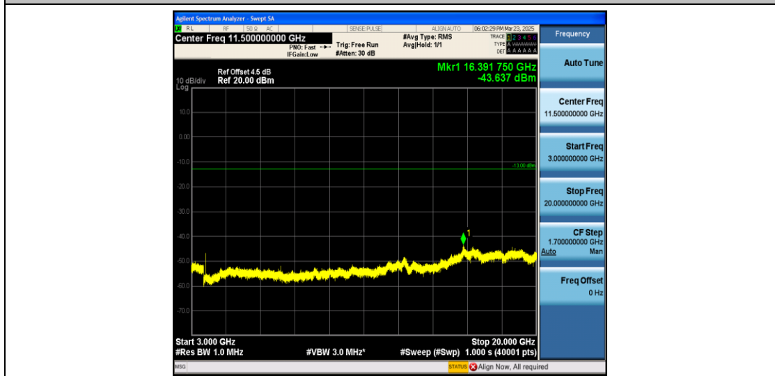
Band2_15MHz_16QAM_18675_1RB#0_3000~20000_3000~20000
