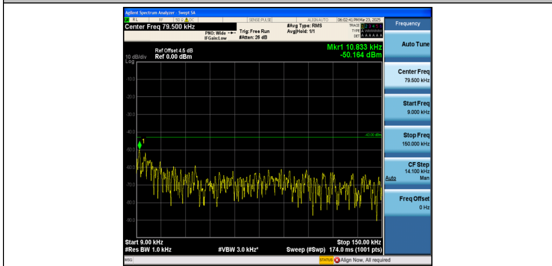
Band2_15MHz_QPSK_18900_1RB#0_0.009~0.15_0.009~0.15
