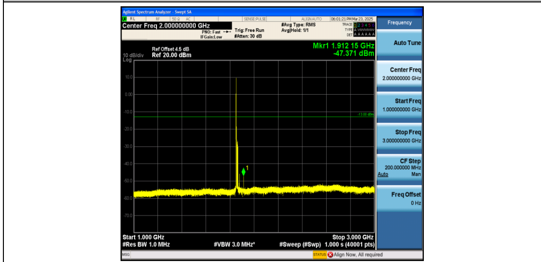
Band2_15MHz_QPSK_18675_1RB#0_1000~3000_1000~3000
