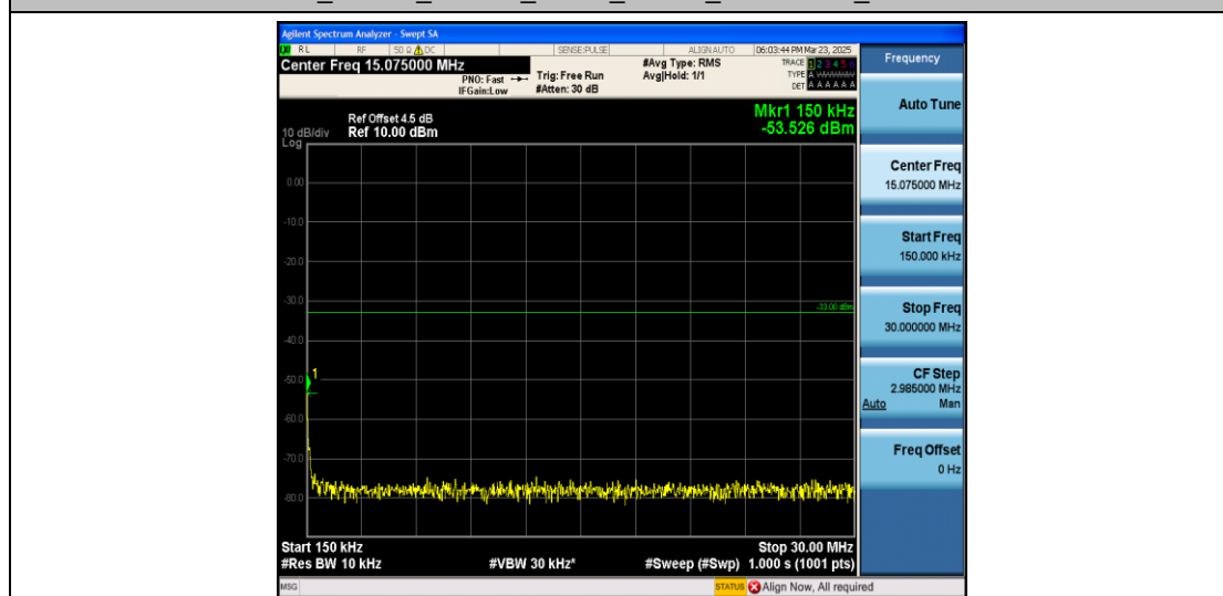
Band2_15MHz_16QAM_18900_1RB#0_0.15~30_0.15~30
