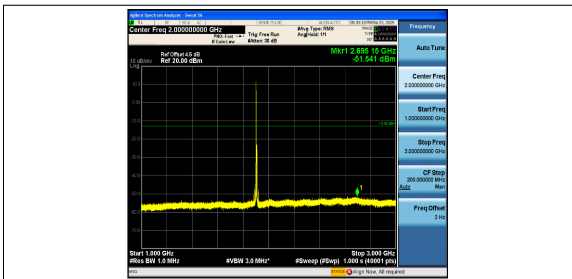
Band2_10MHz_QPSK_19150_1RB#0_1000~3000_1000~3000
