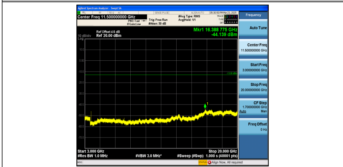
Band2_10MHz_16QAM_18650_1RB#0_3000~20000_3000~20000
