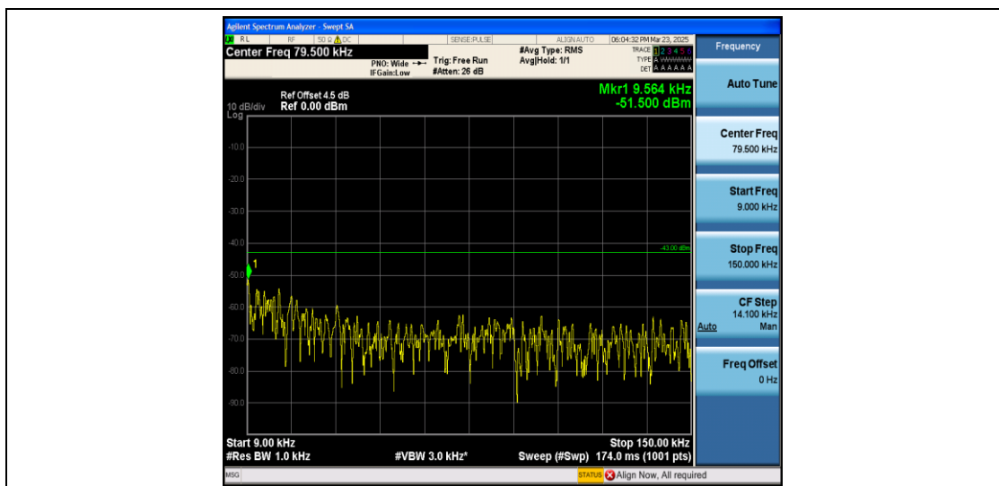
Band2_15MHz_QPSK_19125_1RB#0_0.009~0.15_0.009~0.15
