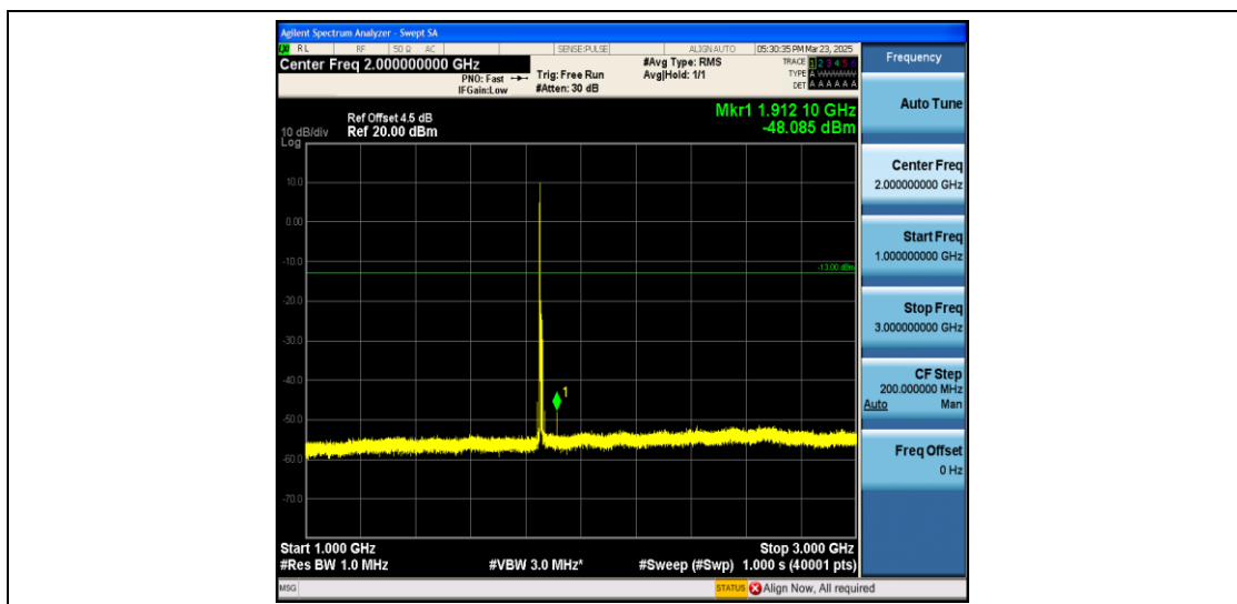
Band2_10MHz_16QAM_18650_1RB#0_1000~3000_1000~3000
