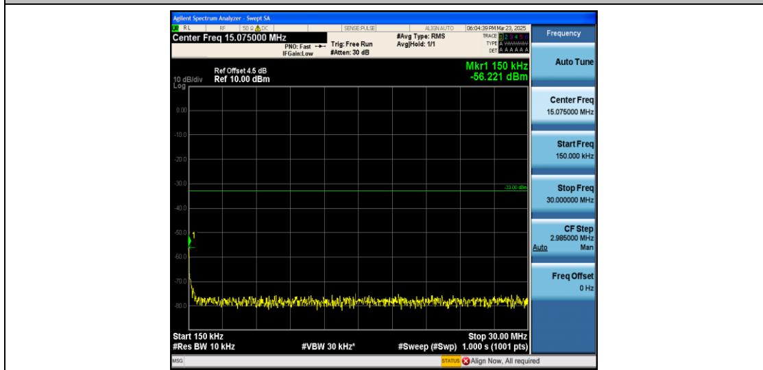
Band2_15MHz_QPSK_19125_1RB#0_0.15~30_0.15~30
