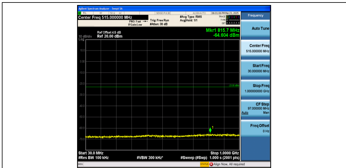
Band2_15MHz_QPSK_18675_1RB#0_30~1000_30~1000
