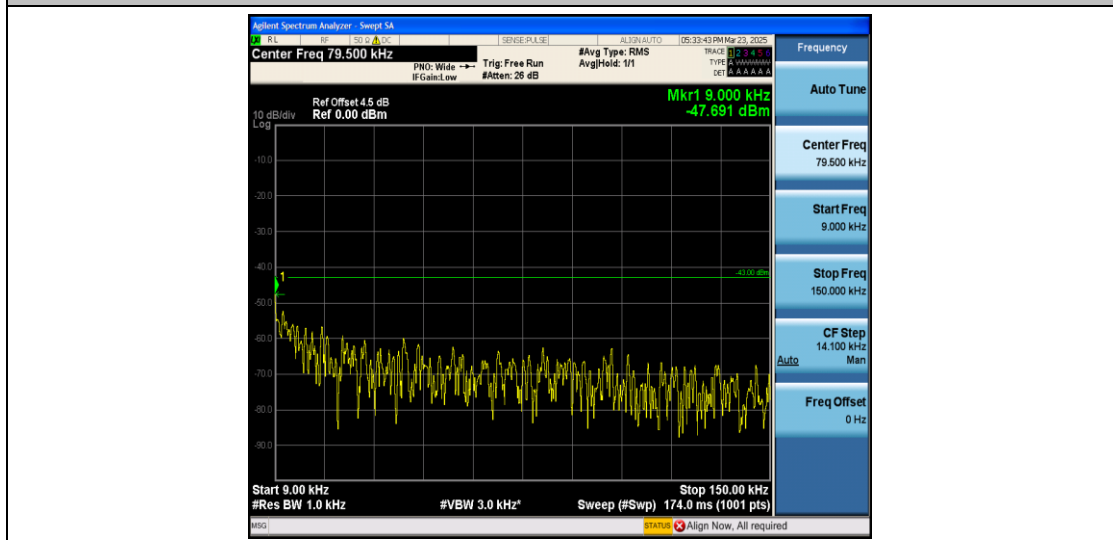
Band2_10MHz_16QAM_19150_1RB#0_0.009~0.15_0.009~0.15
