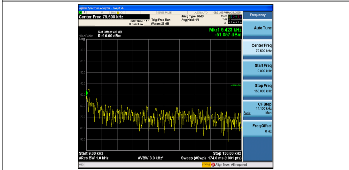
Band2_10MHz_QPSK_18900_1RB#0_0.009~0.15_0.009~0.15
