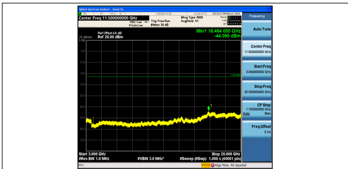
Band2_10MHz_16QAM_19150_1RB#0_3000~20000_3000~20000
