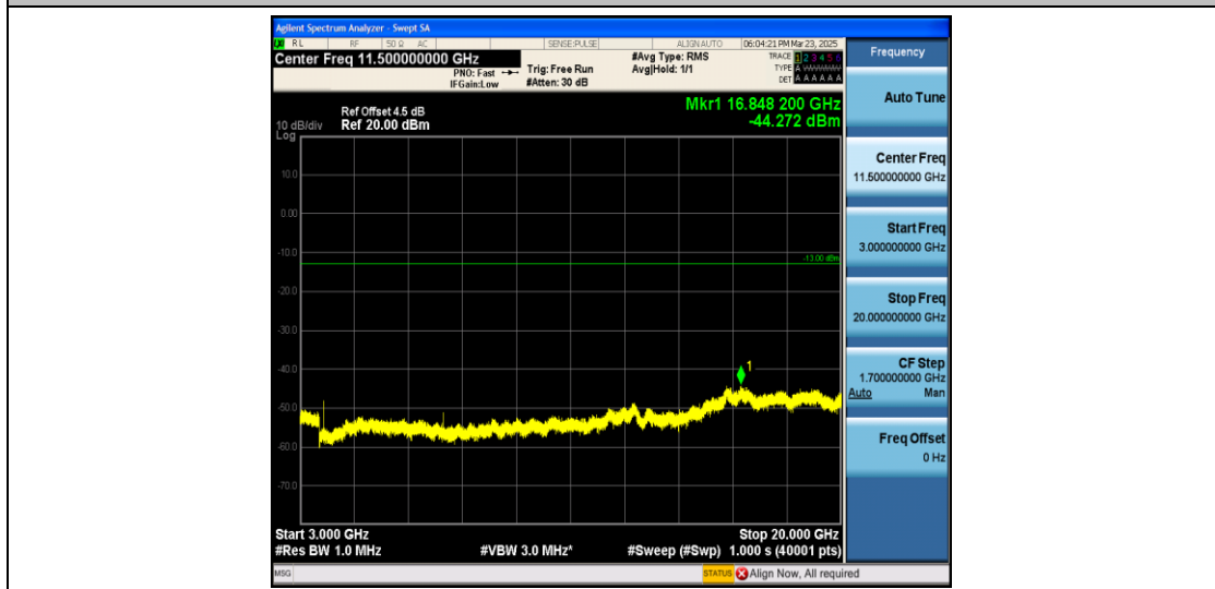
Band2_15MHz_16QAM_18900_1RB#0_3000~20000_3000~20000
