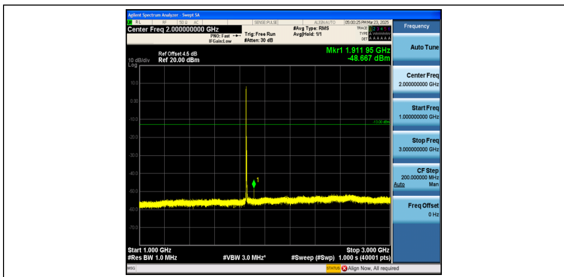
Band2_5MHz_16QAM_18625_1RB#0_1000~3000_1000~3000
