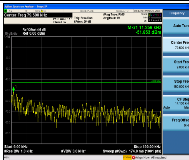
Band2_3MHz_16QAM_19185_1RB#0_0.009~0.15_0.009~0.15
