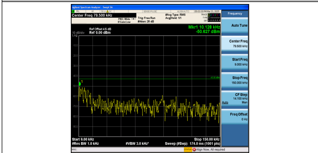
Band2_5MHz_16QAM_19175_1RB#0_0.009~0.15_0.009~0.15
