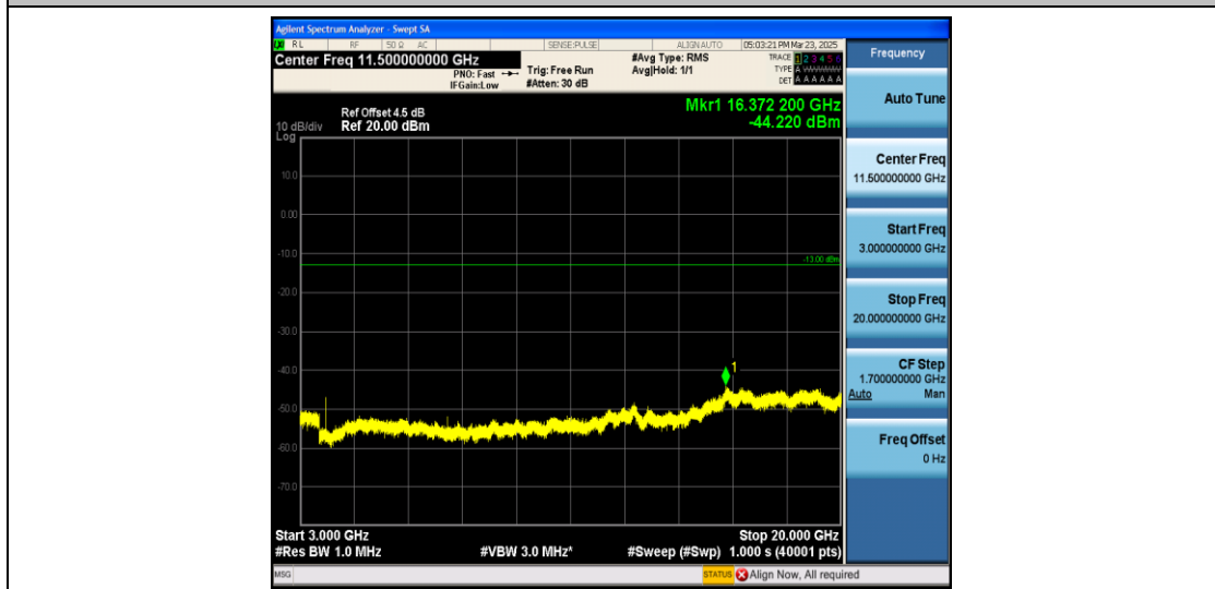
Band2_5MHz_QPSK_19175_1RB#0_3000~20000_3000~20000
