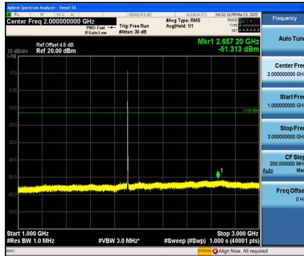
Band2_3MHz_QPSK_19185_1RB#0_1000~3000_1000~3000
