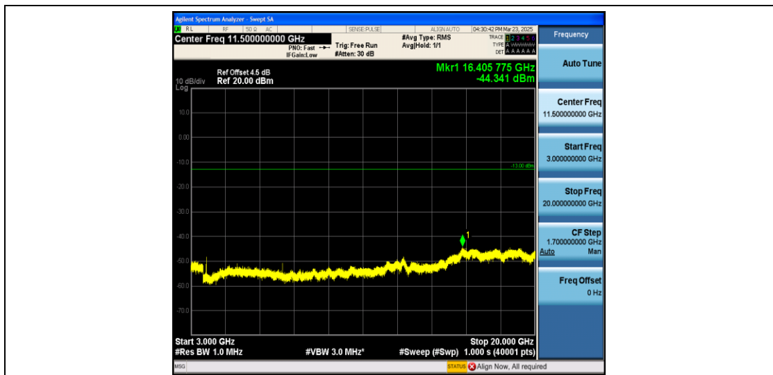
Band2_3MHz_QPSK_18900_1RB#0_3000~20000_3000~20000
