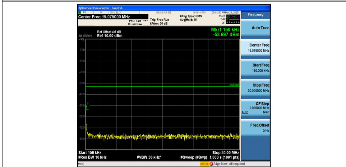
Band2_5MHz_16QAM_18900_1RB#0_0.15~30_0.15~30
