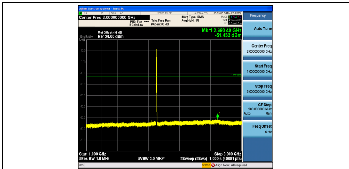
Band2_5MHz_QPSK_19175_1RB#0_1000~3000_1000~3000
