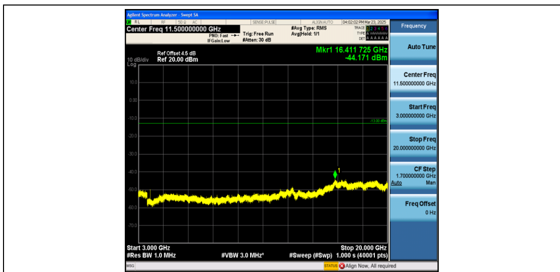
Band2_1.4MHz_16QAM_19193_1RB#0_3000~20000_3000~20000
