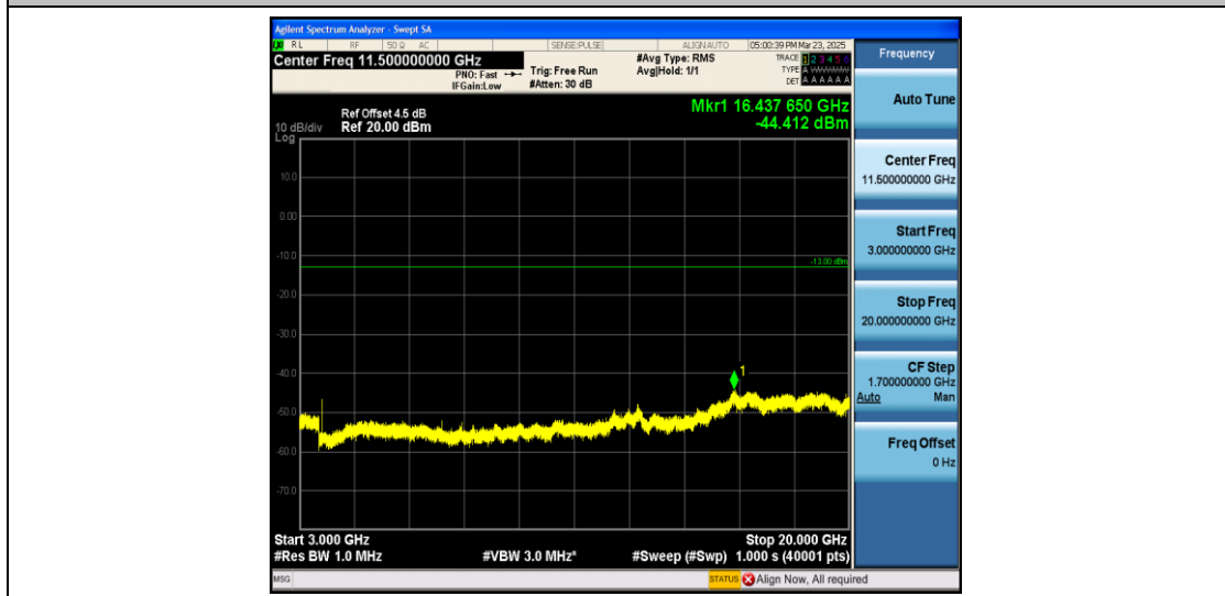
Band2_5MHz_16QAM_18625_1RB#0_3000~20000_3000~20000
