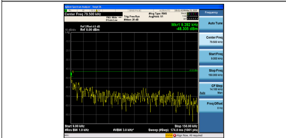
Band2_5MHz_16QAM_18900_1RB#0_0.009~0.15_0.009~0.15
