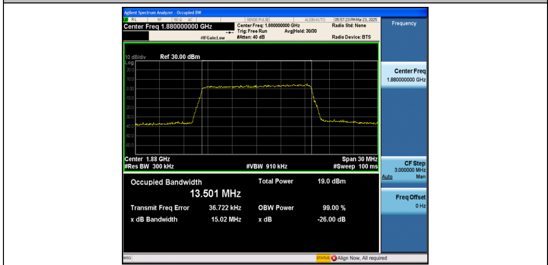
Band2-15MHz-QPSK-18900-75RB#0-PASS
