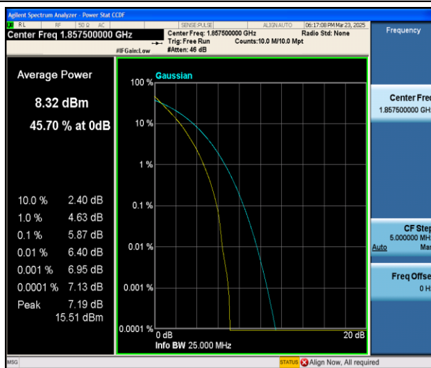
Band2-15MHz-QPSK-18675-75RB#0-PASS
