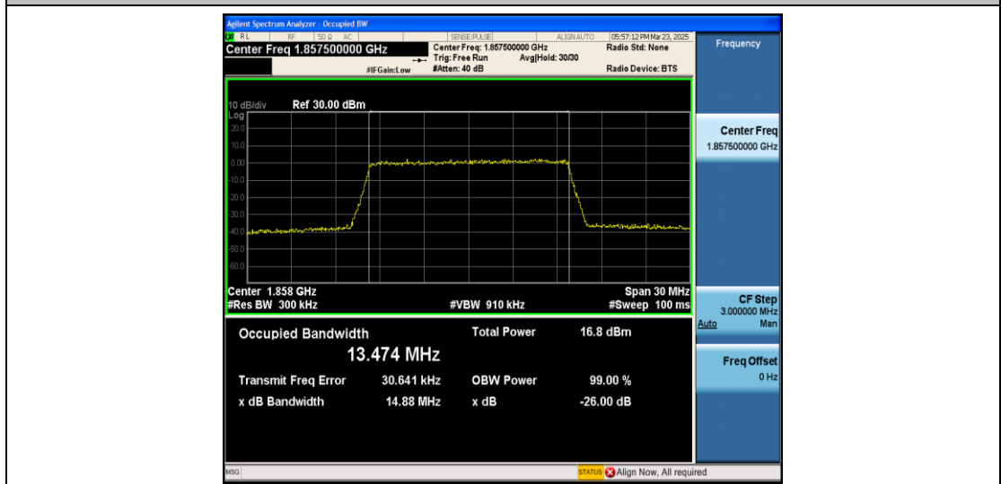
Band2-15MHz-16QAM-18675-75RB#0-PASS
