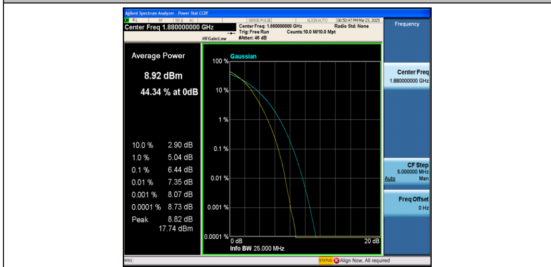
Band2-20MHz-16QAM-18900-100RB#0-PASS
