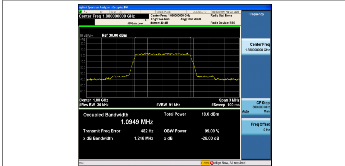
Band2-1.4MHz-QPSK-18900-6RB#0-PASS
