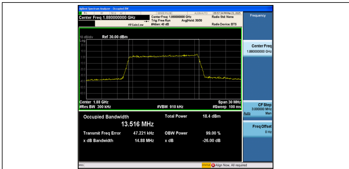
Band2-15MHz-16QAM-18900-75RB#0-PASS
