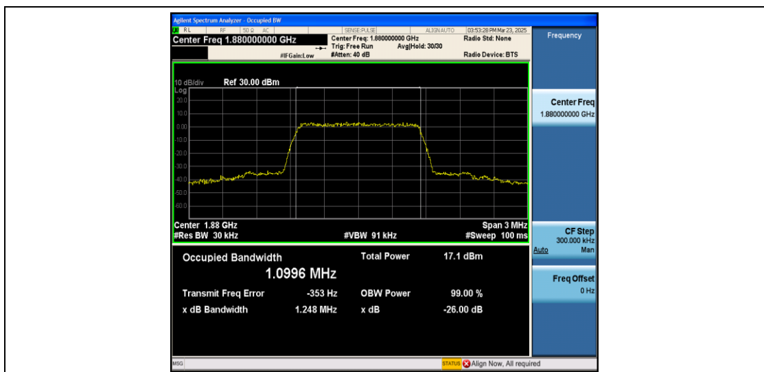
Band2-1.4MHz-16QAM-18900-6RB#0-PASS
