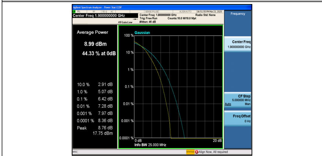
Band2-20MHz-16QAM-19100-100RB#0-PASS
