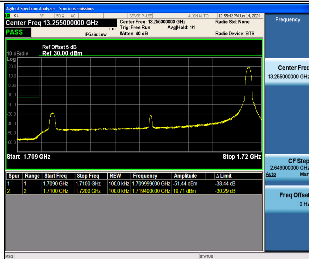
Band66_10MHz_QPSK_132022_1RB#49
