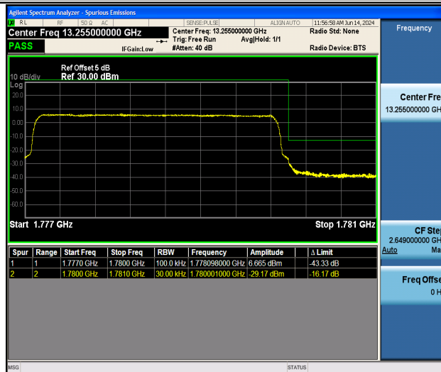
Band66_3MHz_QPSK_132657_15RB#0
