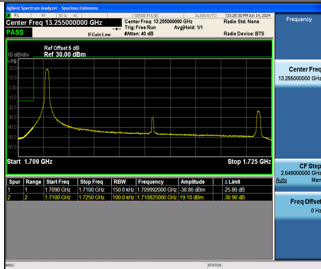
Band66_15MHz_QPSK_132047_1RB#0
