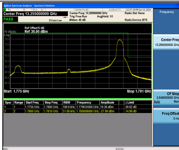
Band66_5MHz_QPSK_132647_1RB#24
