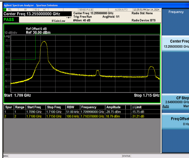
Band66_5MHz_16QAM_131997_1RB#0
