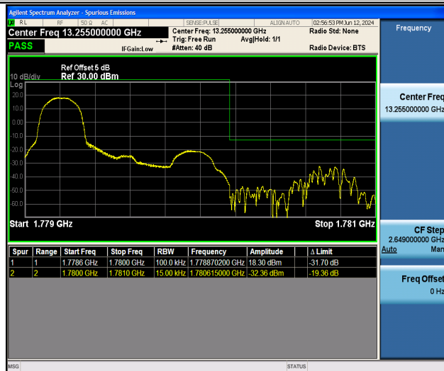
Band66_1.4MHz_16QAM_132665_1RB#0
