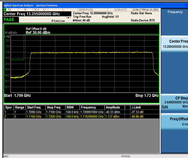
Band66_10MHz_16QAM_132022_50RB#0
