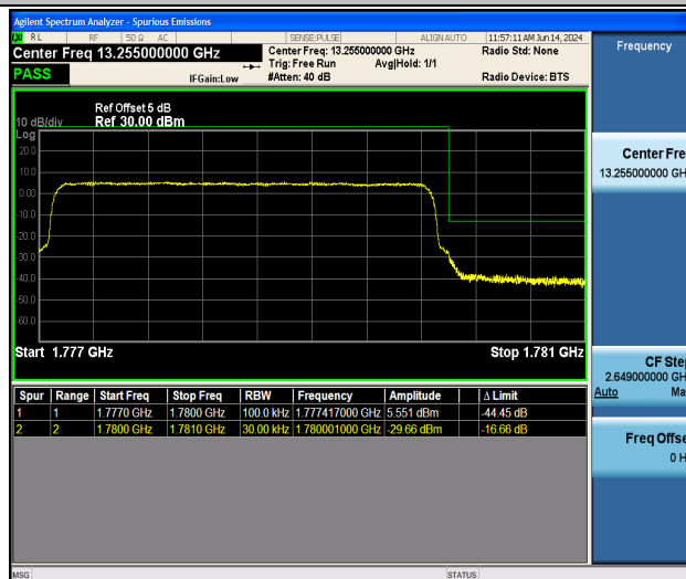
Band66_3MHz_16QAM_132657_15RB#0
