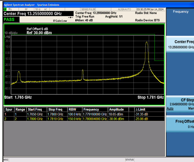
Band66_15MHz_16QAM_132597_1RB#74
