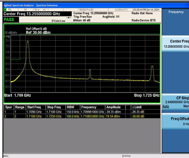
Band66_15MHz_16QAM_132047_1RB#0
