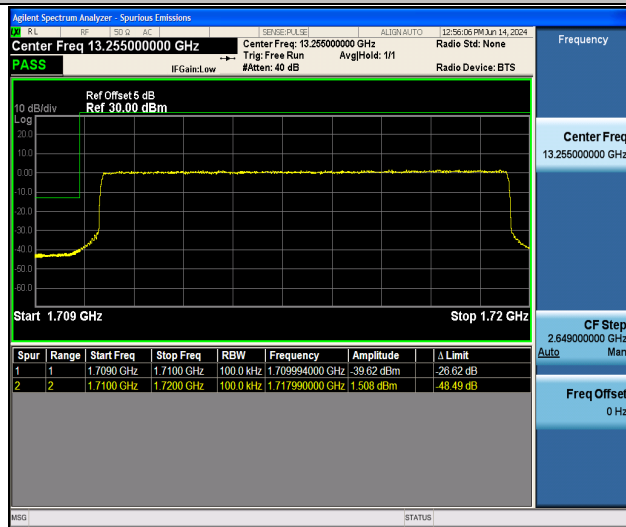
Band66_10MHz_QPSK_132022_50RB#0
