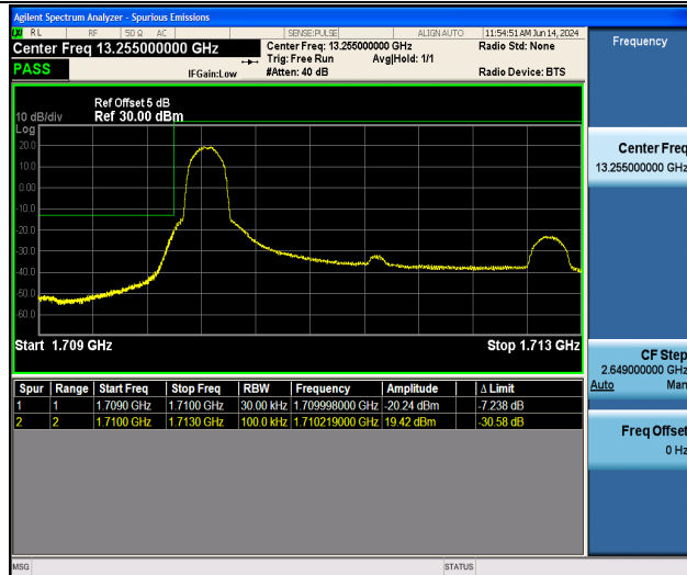
Band66_3MHz_QPSK_131987_1RB#0
