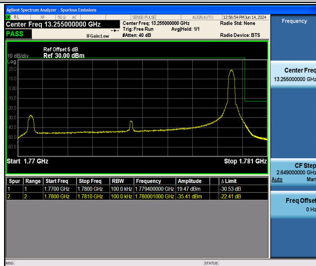
Band66_10MHz_QPSK_132622_1RB#49
