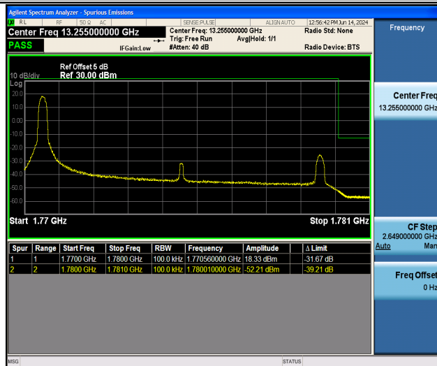
Band66_10MHz_16QAM_132622_1RB#0
