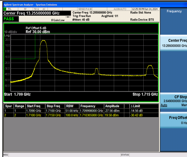
Band66_5MHz_QPSK_131997_1RB#0
