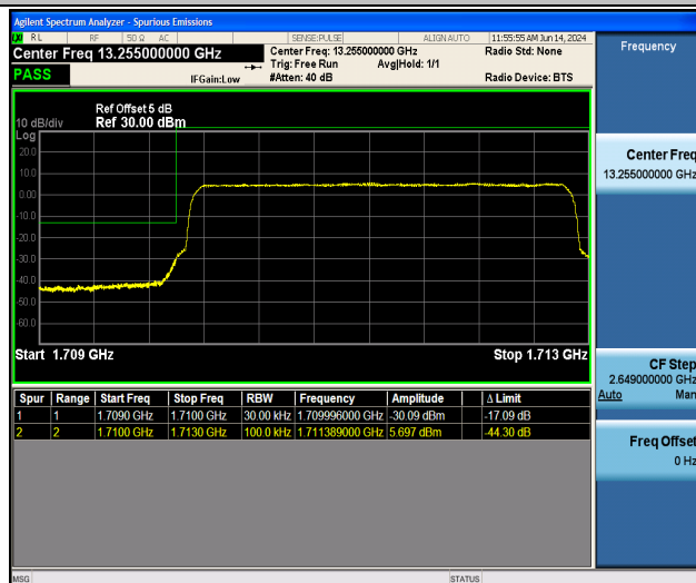
Band66_3MHz_16QAM_131987_15RB#0
