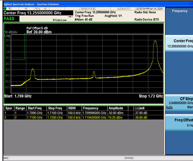
Band66_10MHz_16QAM_132022_1RB#49
