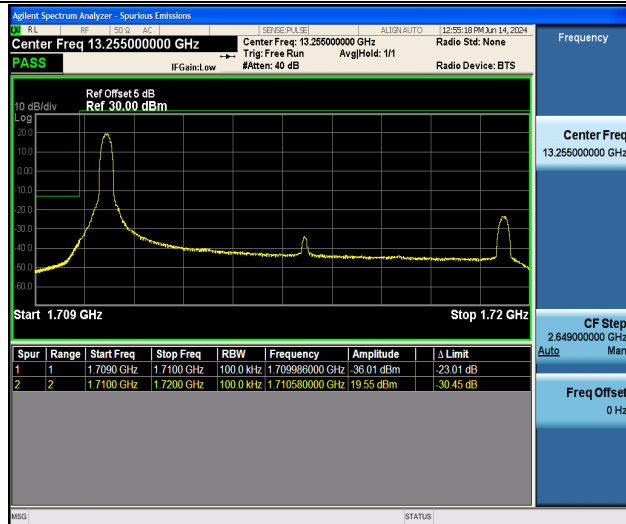
Band66_10MHz_QPSK_132022_1RB#0
