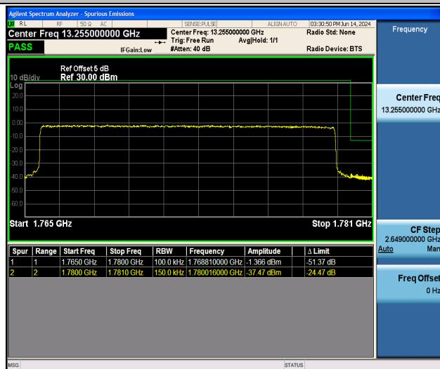
Band66_15MHz_16QAM_132597_75RB#0
