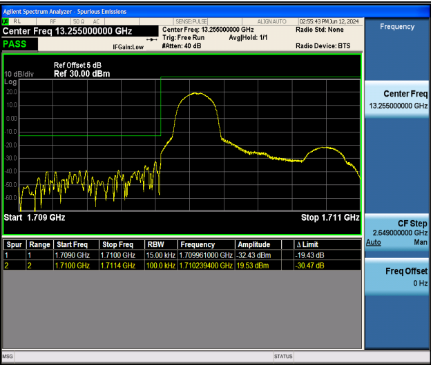
Band66_1.4MHz_QPSK_131979_1RB#0
