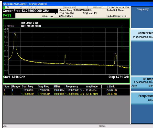
Band66_15MHz_QPSK_132597_1RB#0
