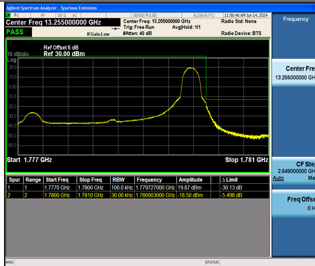
Band66_3MHz_16QAM_132657_1RB#14
