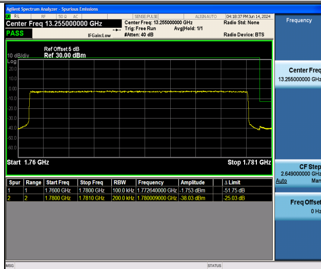
Band66_20MHz_QPSK_132572_100RB#0
