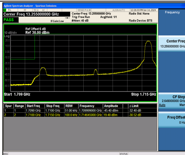
Band66_5MHz_QPSK_131997_1RB#24
