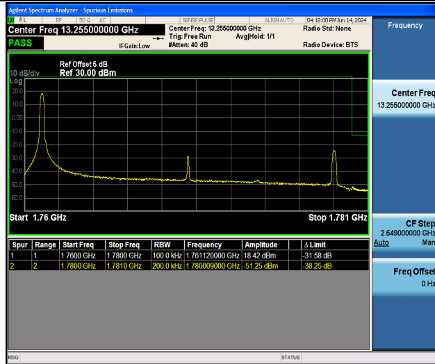
Band66_20MHz_16QAM_132572_1RB#0
