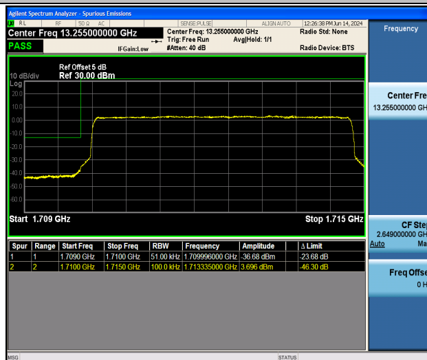
Band66_5MHz_16QAM_131997_25RB#0
