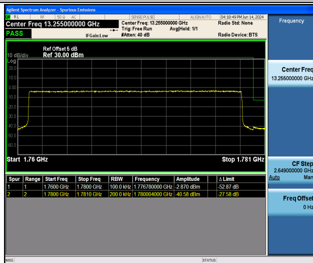
Band66_20MHz_16QAM_132572_100RB#0
