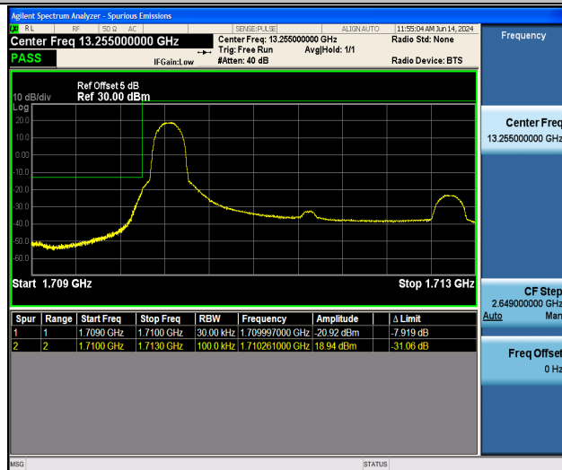
Band66_3MHz_16QAM_131987_1RB#0
