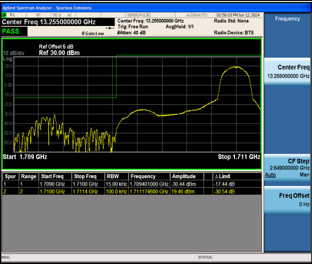
Band66_1.4MHz_QPSK_131979_1RB#5
