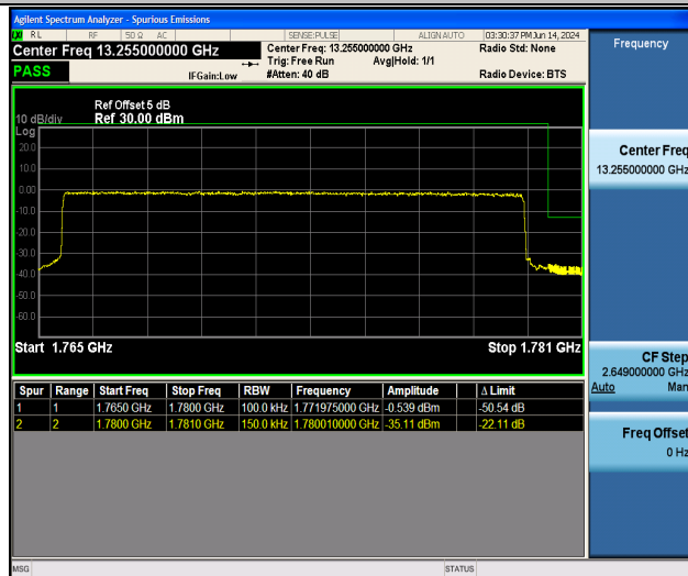
Band66_15MHz_QPSK_132597_75RB#0
