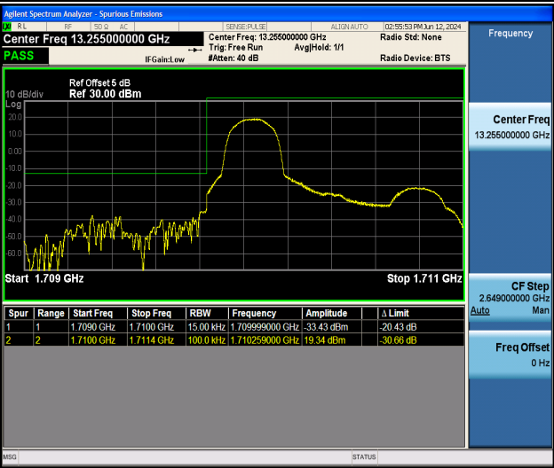
Band66_1.4MHz_16QAM_131979_1RB#0
