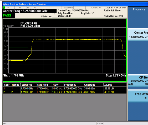
Band66_5MHz_QPSK_131997_25RB#0
