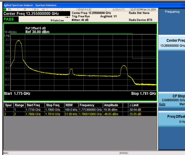
Band66_5MHz_16QAM_132647_1RB#0
