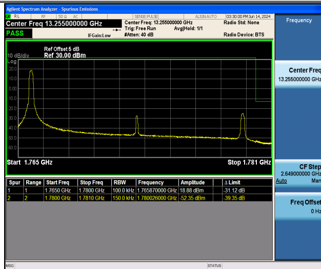
Band66_15MHz_16QAM_132597_1RB#0
