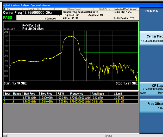
Band66_1.4MHz_QPSK_132665_1RB#5
