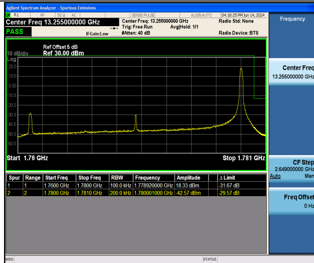
Band66_20MHz_16QAM_132572_1RB#99
