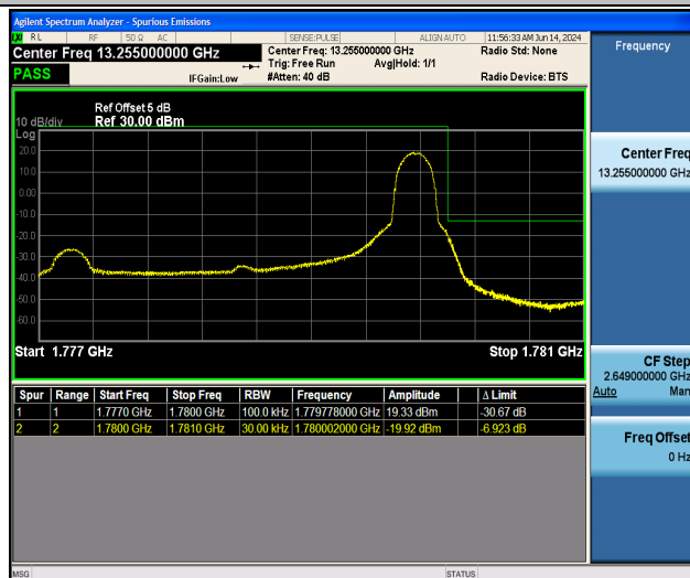
Band66_3MHz_QPSK_132657_1RB#14
