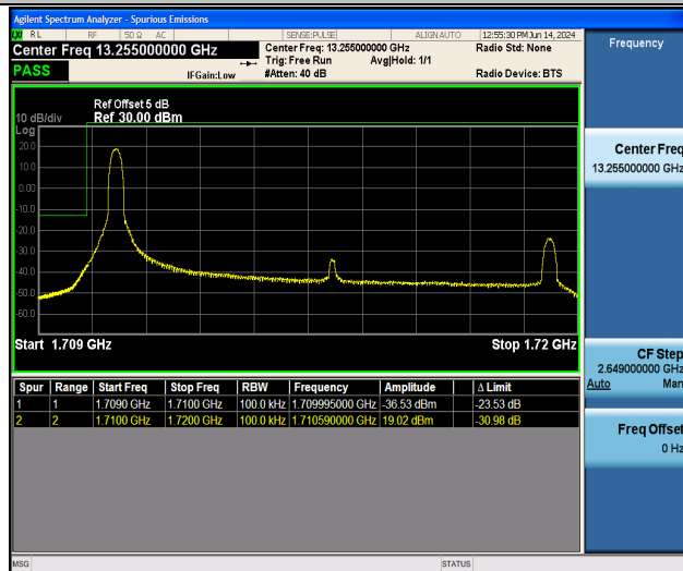
Band66_10MHz_16QAM_132022_1RB#0
