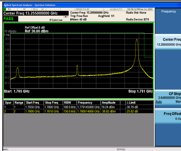
Band66_15MHz_QPSK_132597_1RB#74
