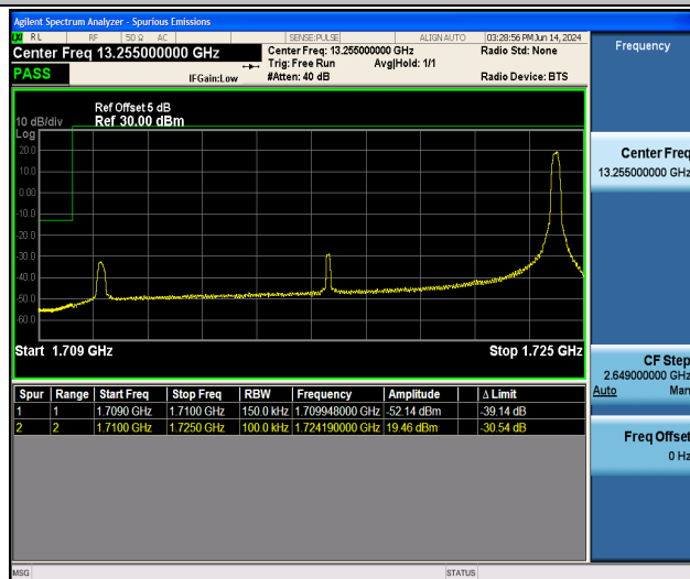
Band66_15MHz_QPSK_132047_1RB#74
