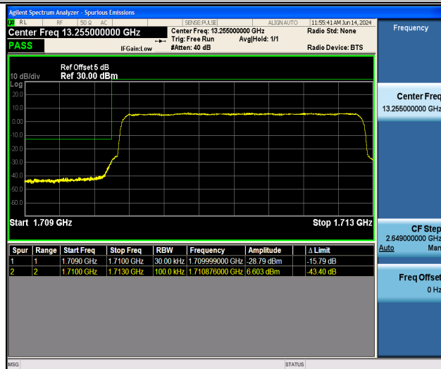
Band66_3MHz_QPSK_131987_15RB#0
