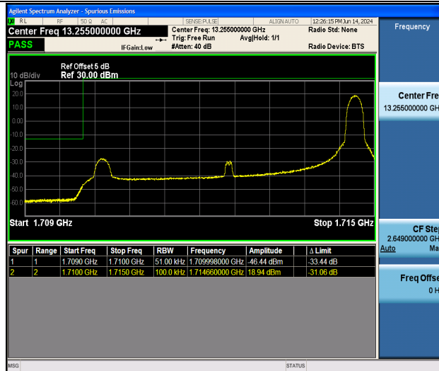
Band66_5MHz_16QAM_131997_1RB#24
