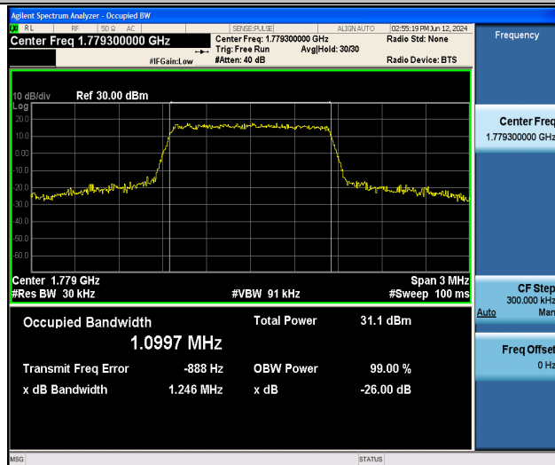
Band66-1.4MHz-QPSK-132665-6RB#0-PASS
