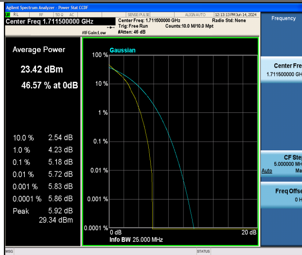
Band66-3MHz-QPSK-131987-1RB#0-PASS
