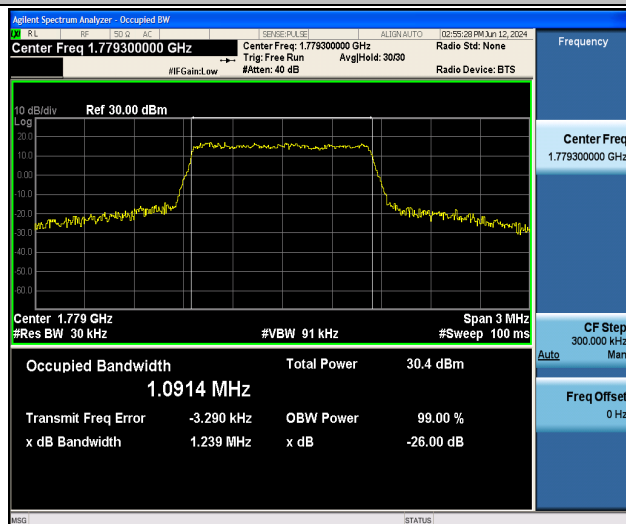
Band66-1.4MHz-16QAM-132665-6RB#0-PASS
