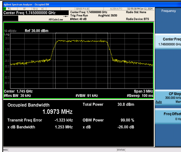
Band66-1.4MHz-16QAM-132322-6RB#0-PASS
