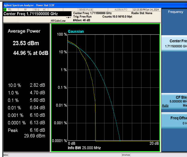
Band66-3MHz-16QAM-131987-1RB#0-PASS
