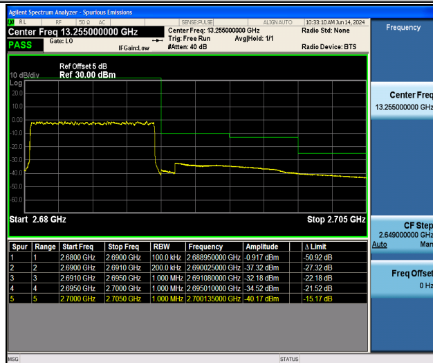
Band41_10MHz_16QAM_41540_50RB#0
