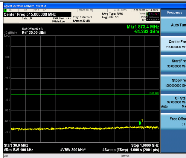
Band41_10MHz_16QAM_40620_1RB#0_30~1000_30~1000
