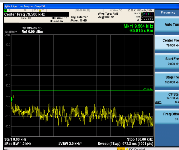
Band41_10MHz_16QAM_40620_1RB#0_0.009~0.15_0.009~0.15
