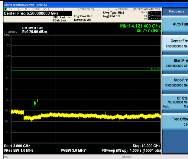
Band26_3MHz_16QAM_26805_1RB#0_3000~10000_3000~10000
