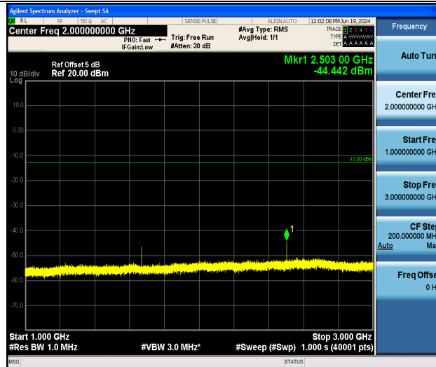
Band26_5MHz_16QAM_26915_1RB#0_1000~3000_1000~3000
