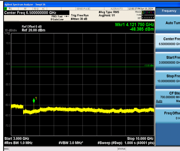
Band26_5MHz_16QAM_26815_1RB#0_3000~10000_3000~10000
