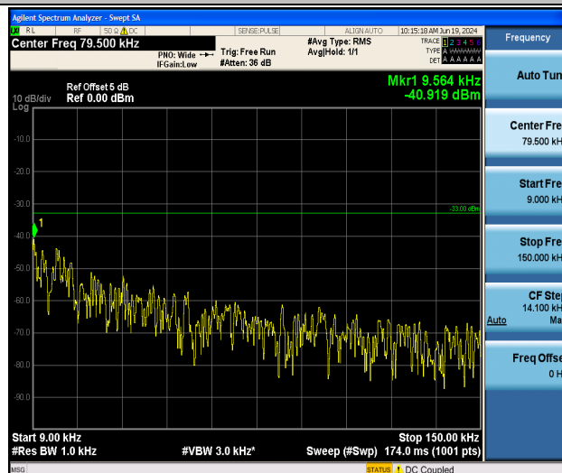
Band26_3MHz_QPSK_27025_1RB#0_0.009~0.15_0.009~0.15
