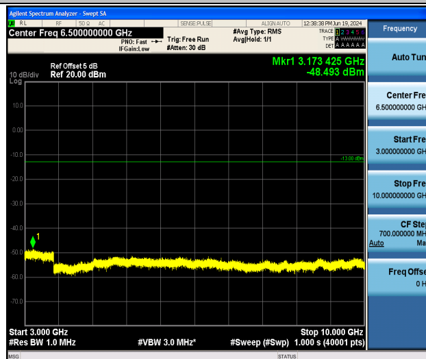
Band26_10MHz_16QAM_26990_1RB#0_3000~10000_3000~10000
