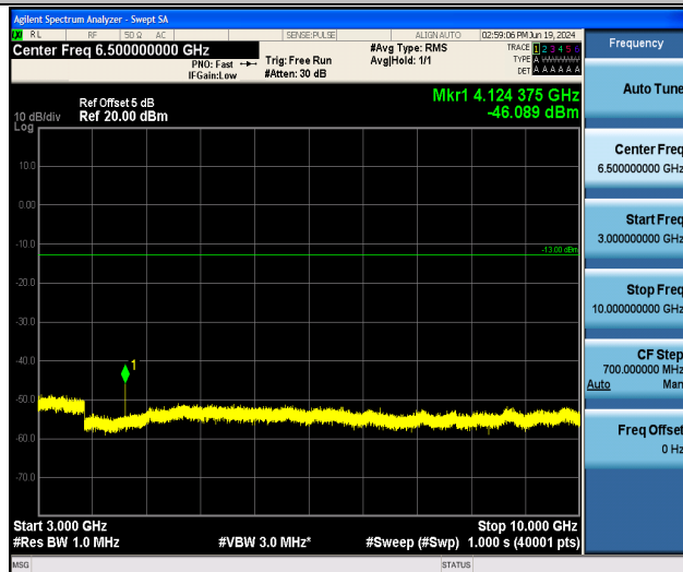
Band26_15MHz_QPSK_26865_1RB#0_3000~10000_3000~10000
