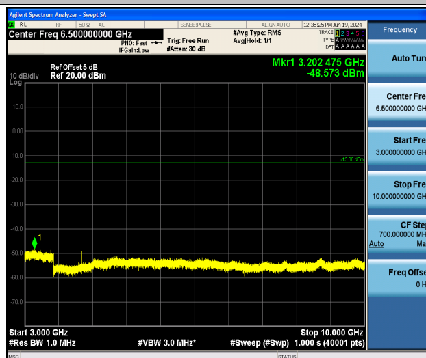
Band26_10MHz_QPSK_26915_1RB#0_3000~10000_3000~10000
