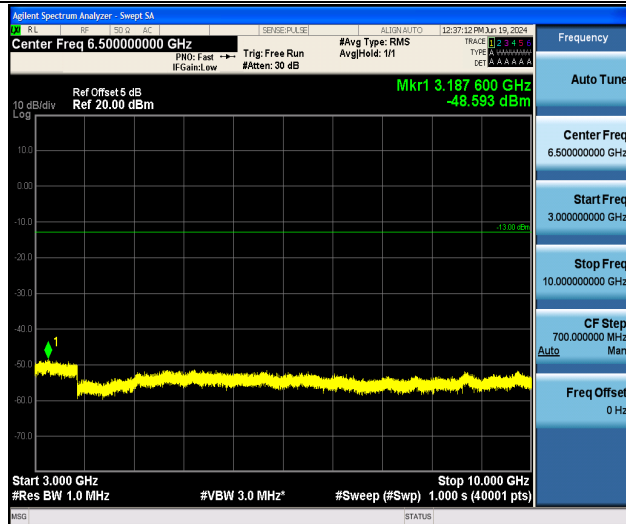
Band26_10MHz_QPSK_26990_1RB#0_3000~10000_3000~10000
