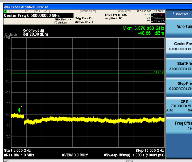
Band26_5MHz_16QAM_27015_1RB#0_3000~10000_3000~10000
