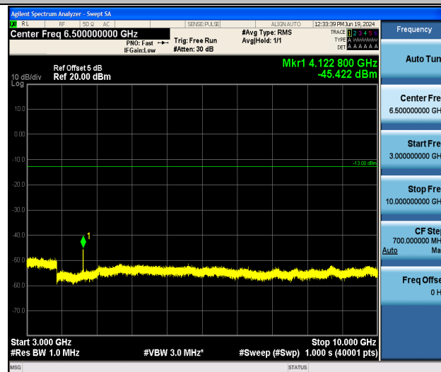
Band26_10MHz_QPSK_26840_1RB#0_3000~10000_3000~10000
