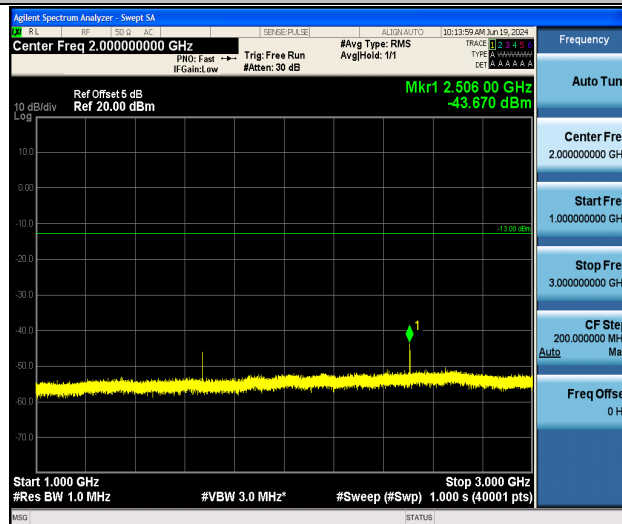
Band26_3MHz_QPSK_26915_1RB#0_1000~3000_1000~3000
