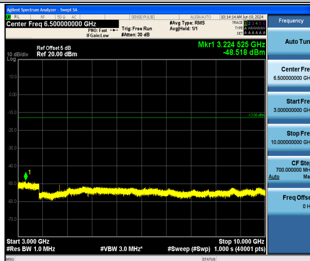
Band26_3MHz_QPSK_26915_1RB#0_3000~10000_3000~10000
