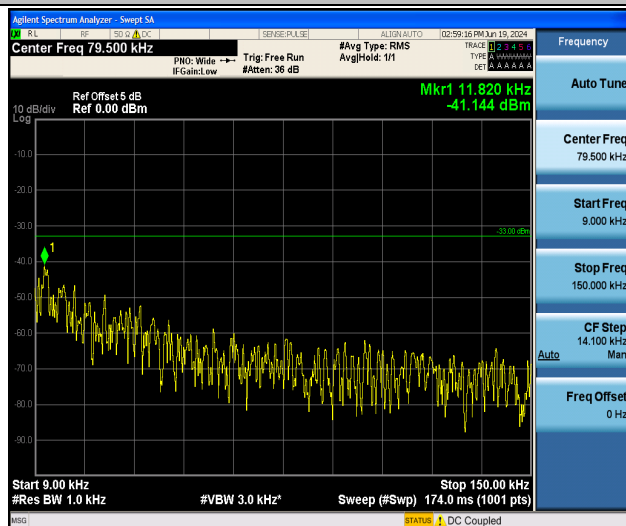
Band26_15MHz_16QAM_26865_1RB#0_0.009~0.15_0.009~0.15
