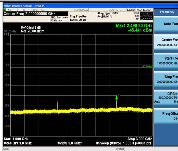
Band26_10MHz_QPSK_26915_1RB#0_1000~3000_1000~3000
