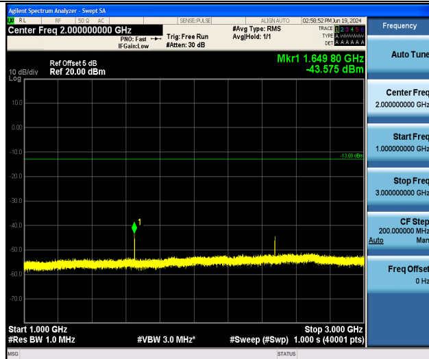
Band26_15MHz_QPSK_26865_1RB#0_1000~3000_1000~3000
