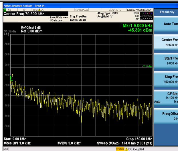
Band26_3MHz_16QAM_27025_1RB#0_0.009~0.15_0.009~0.15
