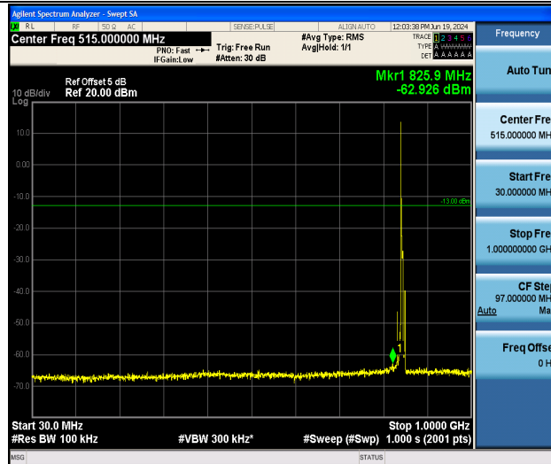
Band26_5MHz_16QAM_27015_1RB#0_30~1000_30~1000
