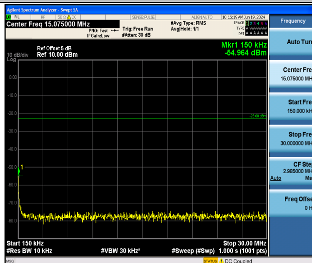
Band26_3MHz_16QAM_27025_1RB#0_0.15~30_0.15~30
