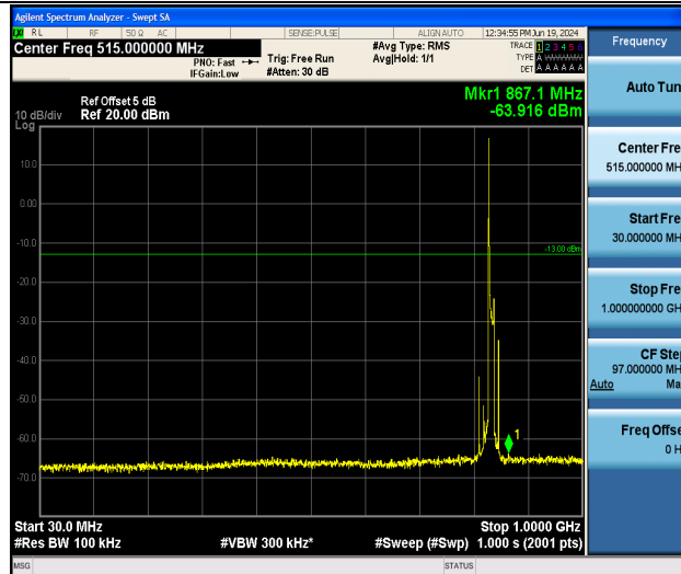
Band26_10MHz_QPSK_26915_1RB#0_30~1000_30~1000
