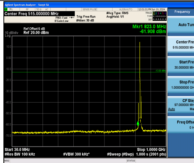
Band26_5MHz_QPSK_26915_1RB#0_30~1000_30~1000
