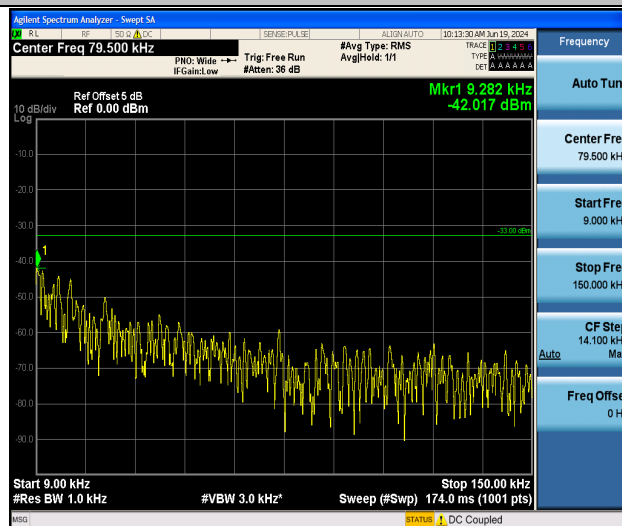
Band26_3MHz_QPSK_26915_1RB#0_0.009~0.15_0.009~0.15
