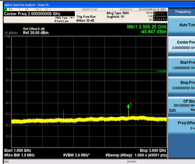
Band26_3MHz_16QAM_26915_1RB#0_1000~3000_1000~3000
