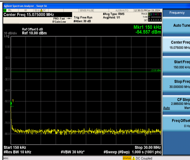
Band26_10MHz_16QAM_26990_1RB#0_0.15~30_0.15~30
