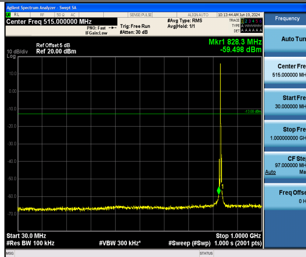
Band26_3MHz_QPSK_26915_1RB#0_30~1000_30~1000
