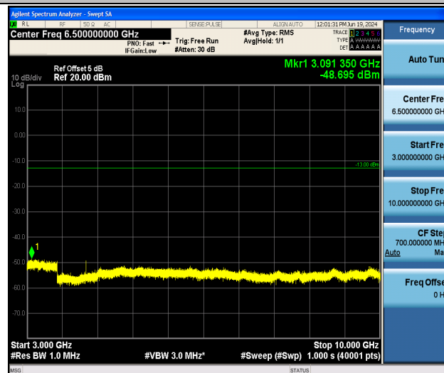
Band26_5MHz_QPSK_26915_1RB#0_3000~10000_3000~10000
