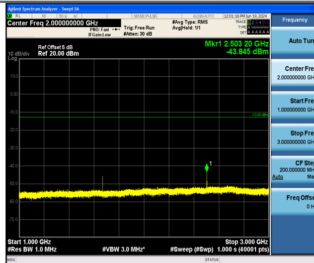
Band26_5MHz_QPSK_26915_1RB#0_1000~3000_1000~3000
