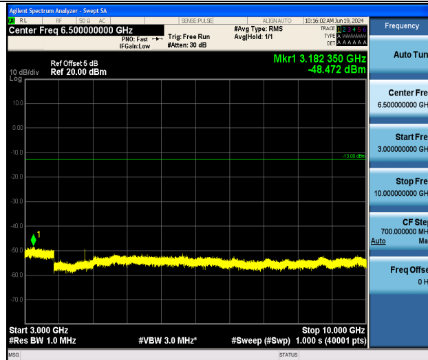
Band26_3MHz_QPSK_27025_1RB#0_3000~10000_3000~10000
