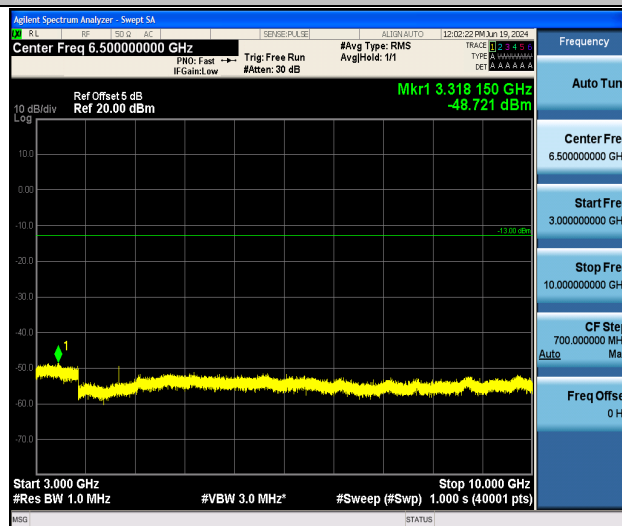
Band26_5MHz_16QAM_26915_1RB#0_3000~10000_3000~10000
