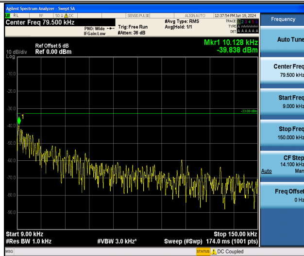
Band26_10MHz_16QAM_26990_1RB#0_0.009~0.15_0.009~0.15
