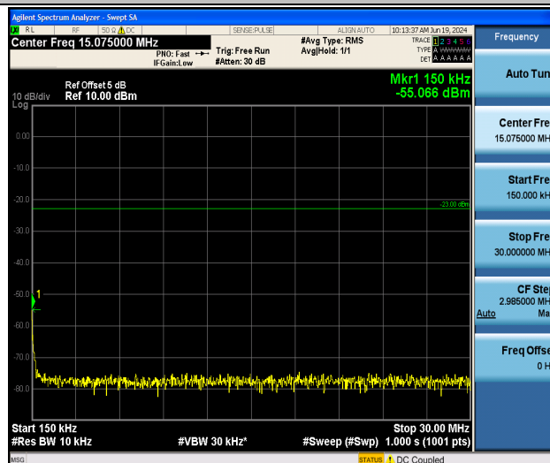
Band26_3MHz_QPSK_26915_1RB#0_0.15~30_0.15~30
