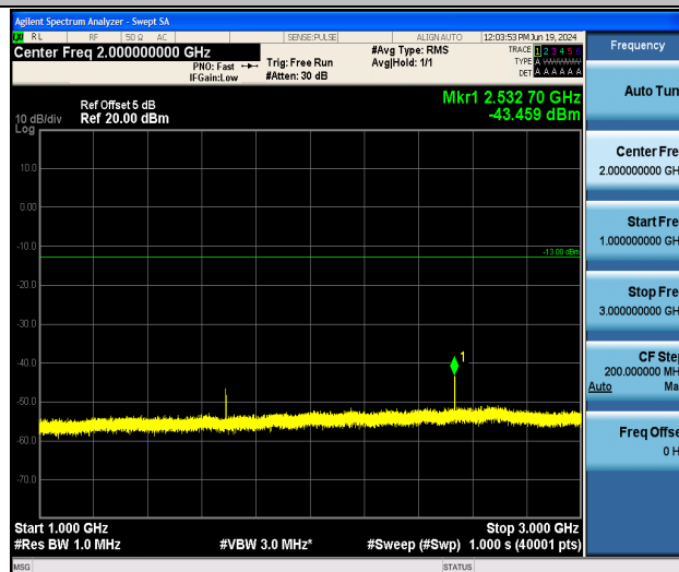
Band26_5MHz_16QAM_27015_1RB#0_1000~3000_1000~3000
