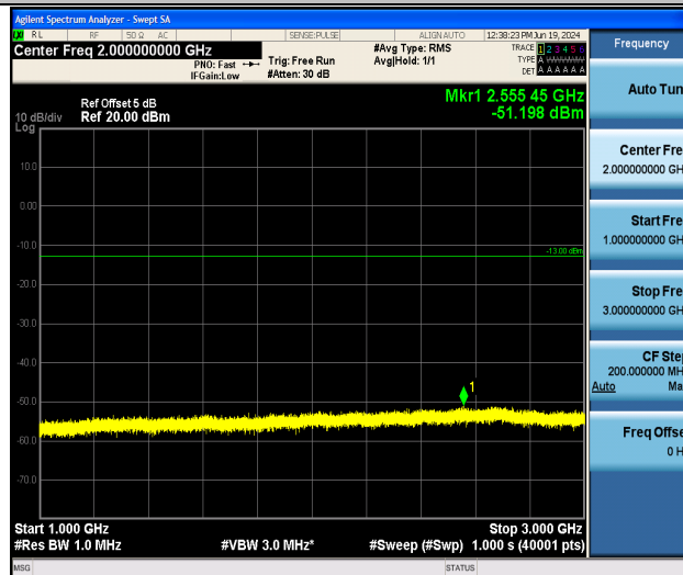
Band26_10MHz_16QAM_26990_1RB#0_1000~3000_1000~3000
