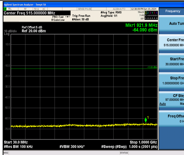
Band26_10MHz_16QAM_26990_1RB#0_30~1000_30~1000
