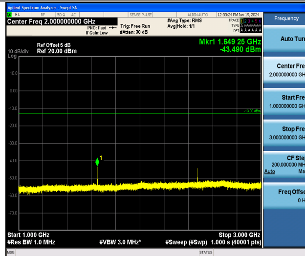
Band26_10MHz_QPSK_26840_1RB#0_1000~3000_1000~3000
