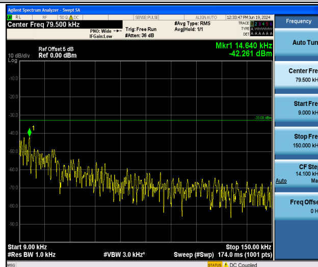
Band26_10MHz_16QAM_26840_1RB#0_0.009~0.15_0.009~0.15
