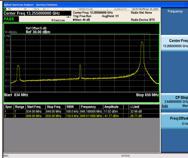
Band26_15MHz_16QAM_26965_1RB#74
