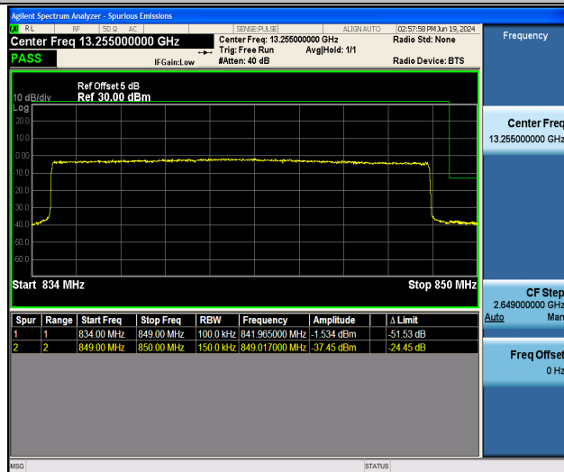
Band26_15MHz_QPSK_26965_75RB#0
