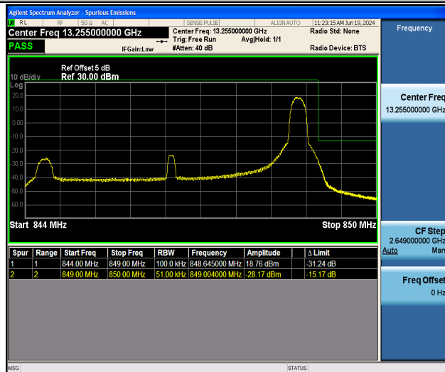
Band26_5MHz_QPSK_27015_1RB#24
