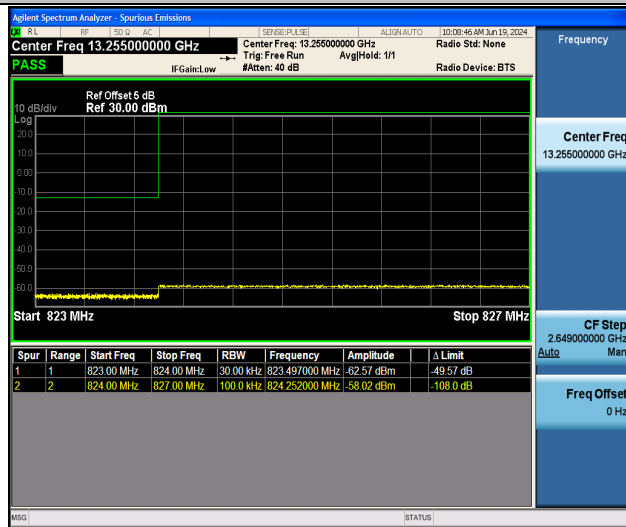
Band26_3MHz_16QAM_26805_1RB#0
