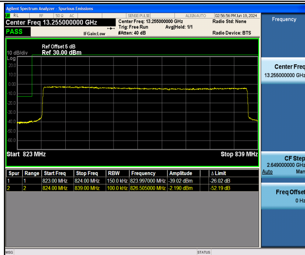
Band26_15MHz_16QAM_26865_75RB#0
