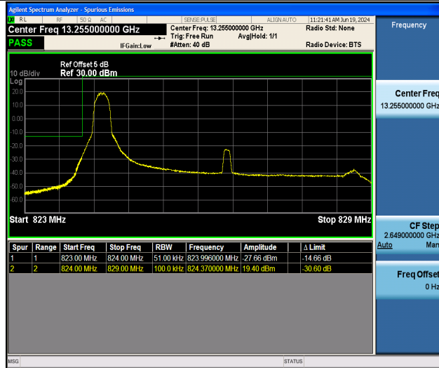
Band26_5MHz_QPSK_26815_1RB#0
