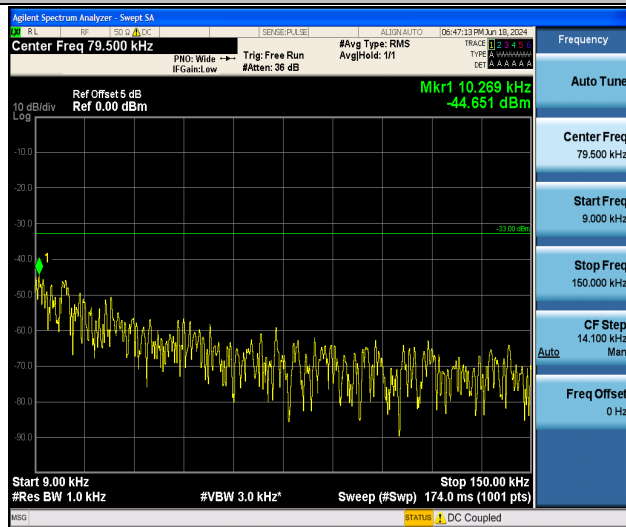
Band26_1.4MHz_16QAM_27033_1RB#0_0.009~0.15_0.009~0.15
