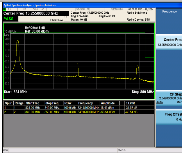
Band26_15MHz_16QAM_26965_1RB#0
