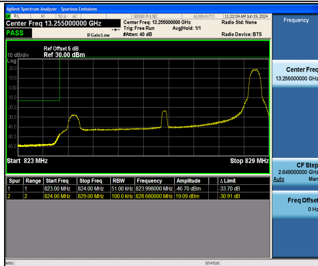
Band26_5MHz_QPSK_26815_1RB#24
