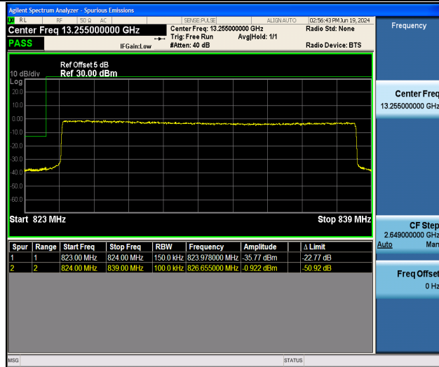
Band26_15MHz_QPSK_26865_75RB#0
