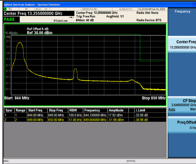
Band26_5MHz_16QAM_27015_1RB#0
