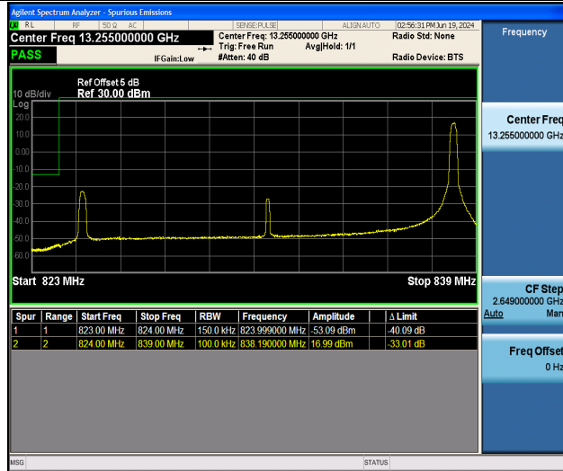
Band26_15MHz_16QAM_26865_1RB#74
