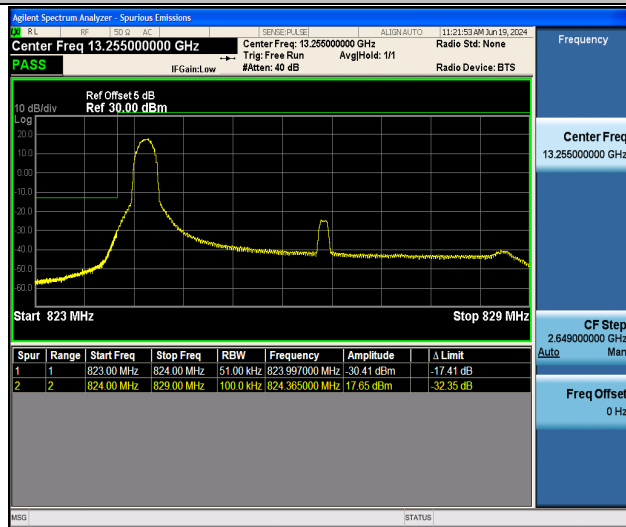
Band26_5MHz_16QAM_26815_1RB#0
