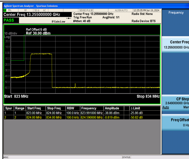
Band26_10MHz_16QAM_26840_50RB#0
