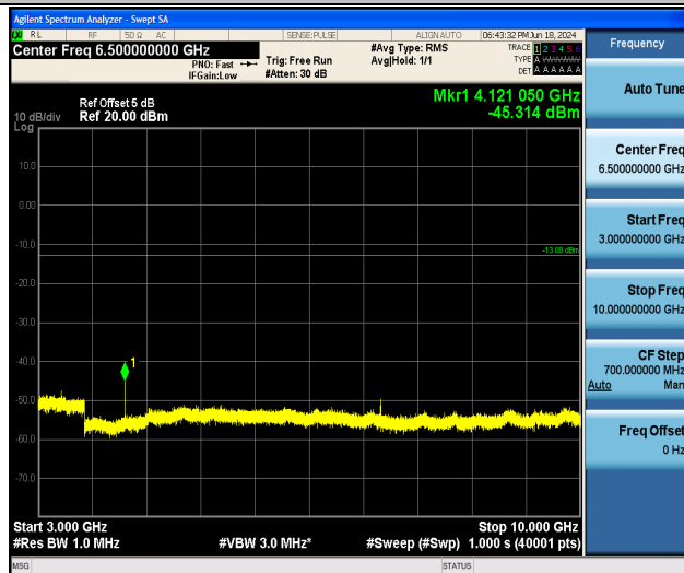
Band26_1.4MHz_QPSK_26797_1RB#0_3000~10000_3000~10000
