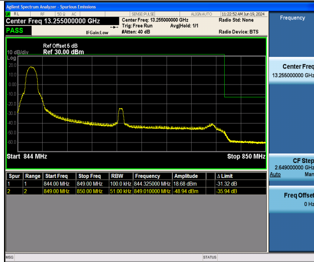
Band26_5MHz_QPSK_27015_1RB#0
