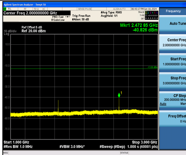
Band26_1.4MHz_QPSK_26797_1RB#0_1000~3000_1000~3000
