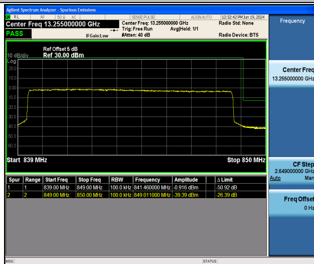
Band26_10MHz_16QAM_26990_50RB#0
