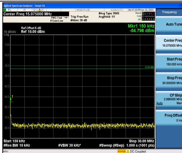
Band26_1.4MHz_16QAM_27033_1RB#0_0.15~30_0.15~30
