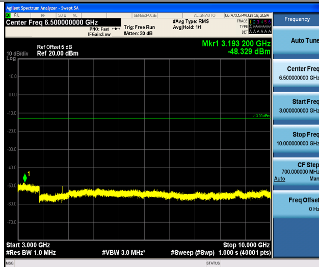
Band26_1.4MHz_QPSK_27033_1RB#0_3000~10000_3000~10000
