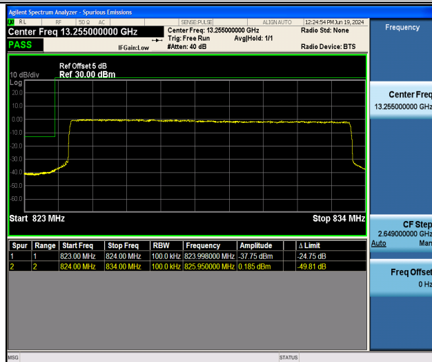
Band26_10MHz_QPSK_26840_50RB#0
