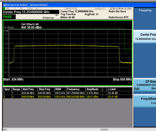
Band26_15MHz_16QAM_26965_75RB#0
