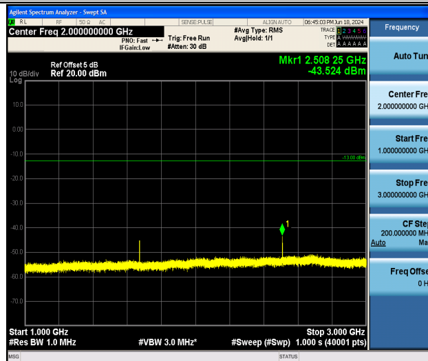
Band26_1.4MHz_QPSK_26915_1RB#0_1000~3000_1000~3000
