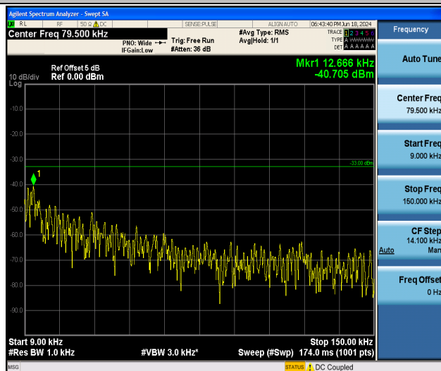
Band26_1.4MHz_16QAM_26797_1RB#0_0.009~0.15_0.009~0.15
