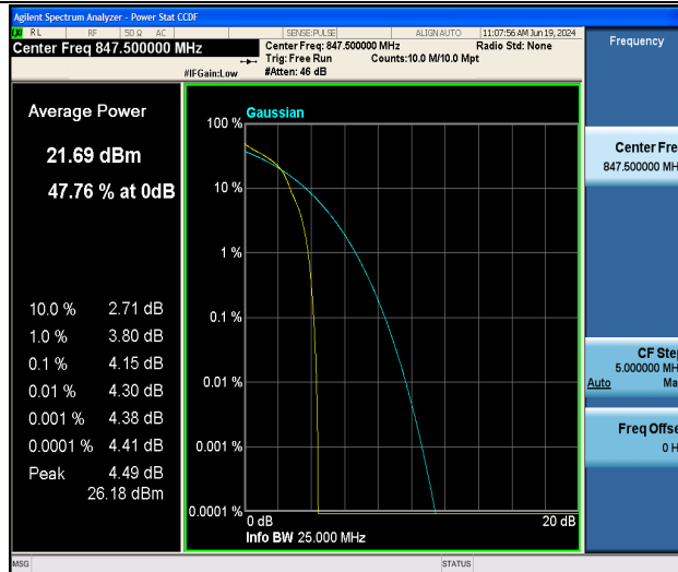
26(824-849)-3MHz-16QAM-27025-1RB#0-PASS
