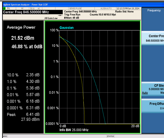
26(824-849)-5MHz-QPSK-27015-25RB#0-PASS
