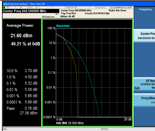
26(824-849)-5MHz-16QAM-27015-1RB#0-PASS
