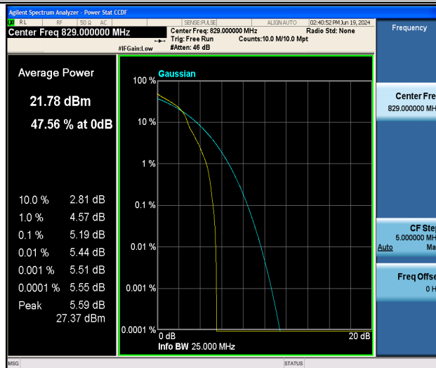
26(824-849)-10MHz-16QAM-26840-1RB#0-PASS
