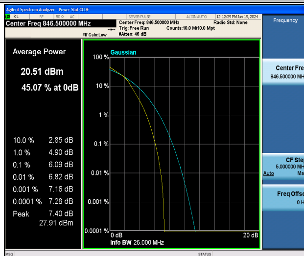
26(824-849)-5MHz-16QAM-27015-25RB#0-PASS
