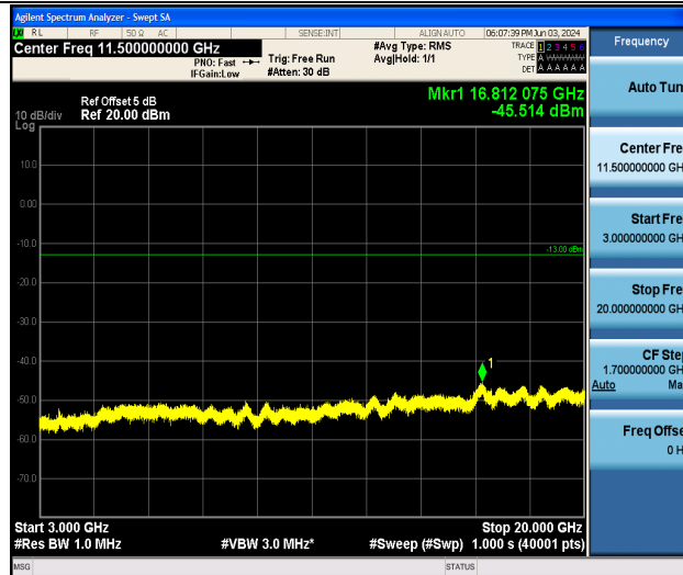
Band25_15MHz_16QAM_26115_1RB#0_3000~20000_3000~20000
