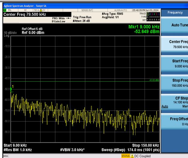
Band25_10MHz_16QAM_26640_1RB#0_0.009~0.15_0.009~0.15
