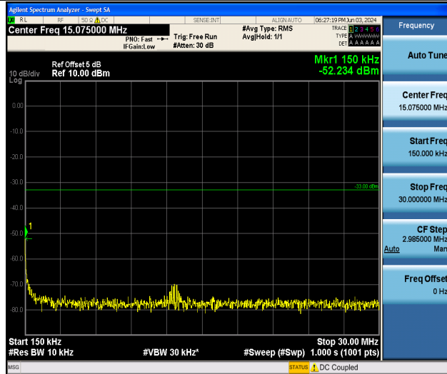
Band25_20MHz_16QAM_26140_1RB#0_0.15~30_0.15~30
