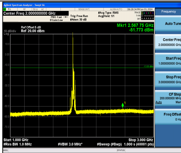
Band25_20MHz_QPSK_26365_1RB#0_1000~3000_1000~3000
