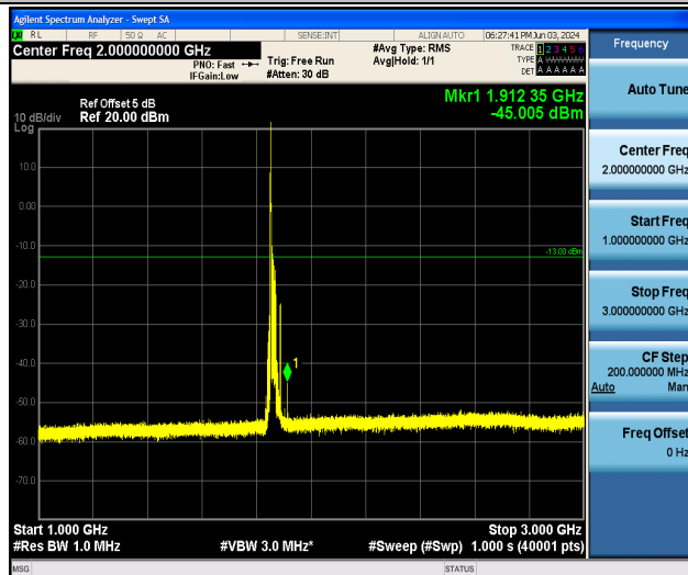
Band25_20MHz_16QAM_26140_1RB#0_1000~3000_1000~3000
