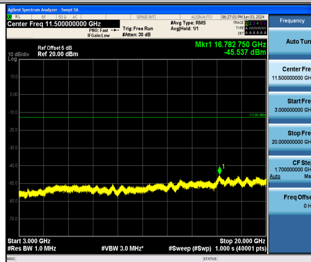
Band25_20MHz_QPSK_26140_1RB#0_3000~20000_3000~20000
