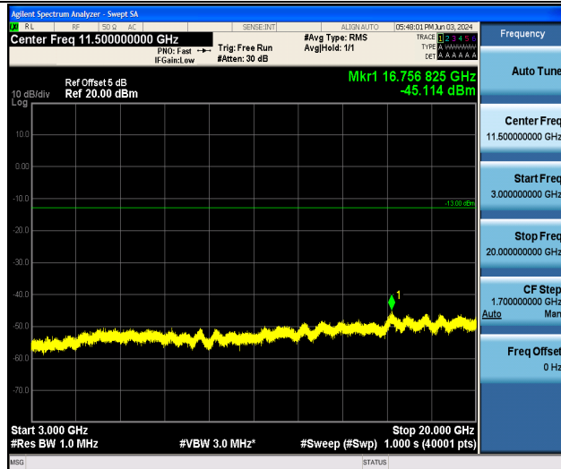
Band25_10MHz_QPSK_26640_1RB#0_3000~20000_3000~20000
