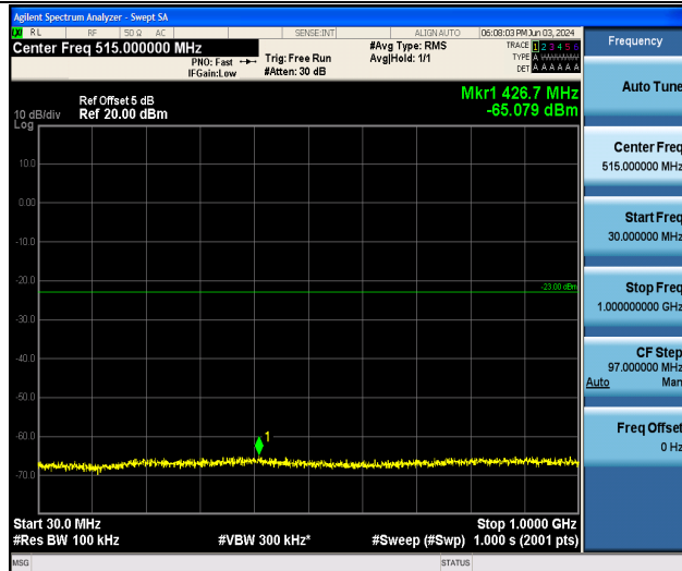
Band25_15MHz_QPSK_26365_1RB#0_30~1000_30~1000
