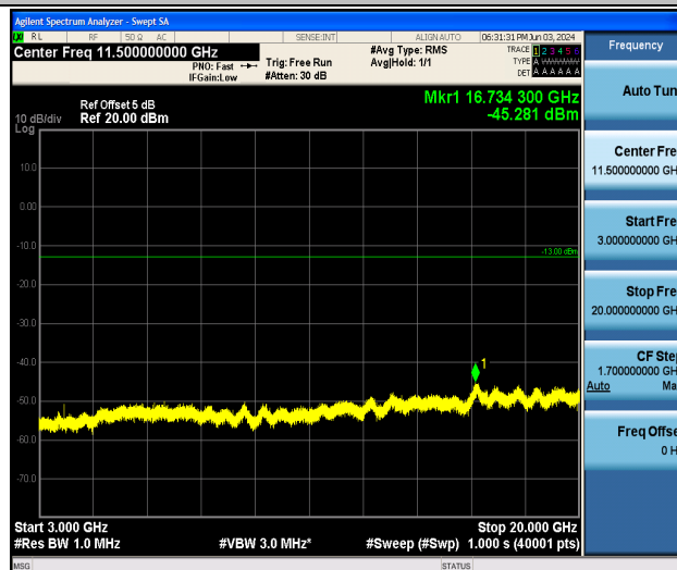
Band25_20MHz_16QAM_26590_1RB#0_3000~20000_3000~20000
