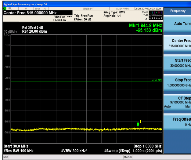
Band25_20MHz_QPSK_26365_1RB#0_30~1000_30~1000
