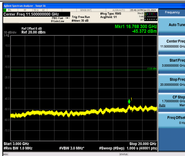
Band25_10MHz_QPSK_26365_1RB#0_3000~20000_3000~20000
