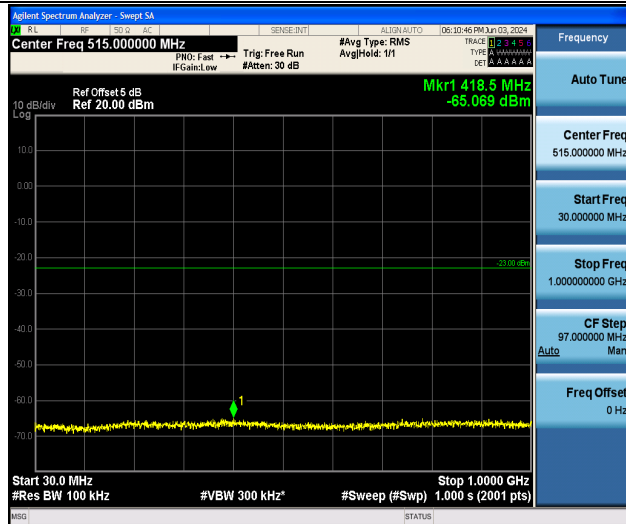
Band25_15MHz_16QAM_26615_1RB#0_30~1000_30~1000
