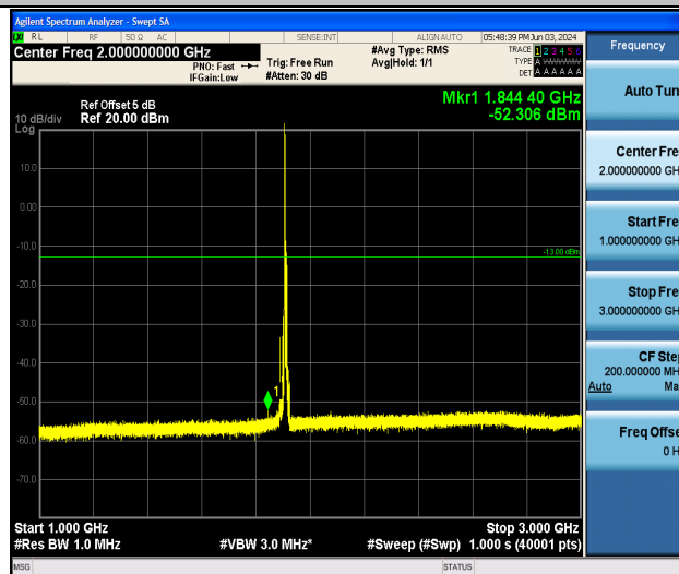
Band25_10MHz_16QAM_26640_1RB#0_1000~3000_1000~3000
