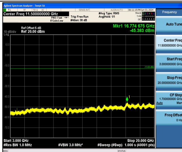
Band25_15MHz_16QAM_26615_1RB#0_3000~20000_3000~20000
