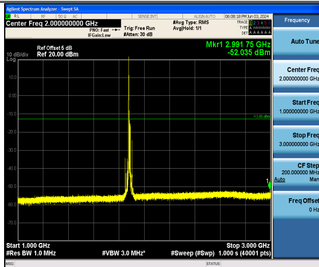
Band25_15MHz_QPSK_26365_1RB#0_1000~3000_1000~3000
