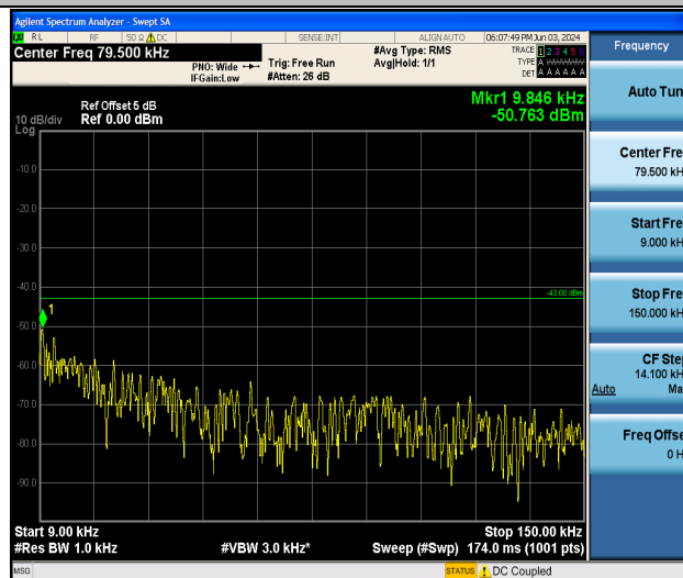
Band25_15MHz_QPSK_26365_1RB#0_0.009~0.15_0.009~0.15
