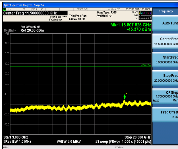
Band25_20MHz_QPSK_26365_1RB#0_3000~20000_3000~20000
