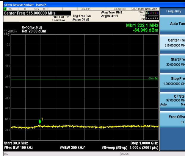
Band25_20MHz_16QAM_26590_1RB#0_30~1000_30~1000
