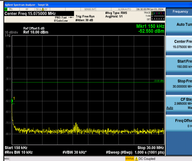
Band25_20MHz_QPSK_26590_1RB#0_0.15~30_0.15~30
