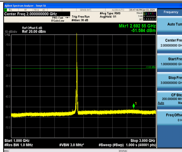
Band25_10MHz_QPSK_26640_1RB#0_1000~3000_1000~3000
