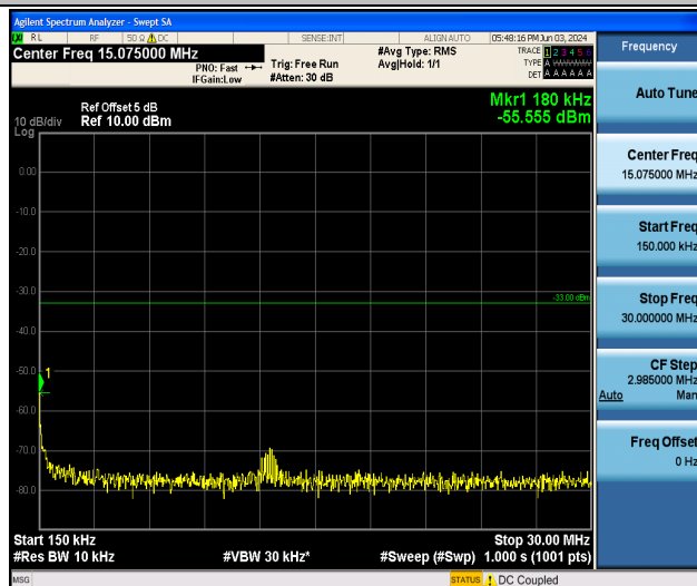
Band25_10MHz_16QAM_26640_1RB#0_0.15~30_0.15~30
