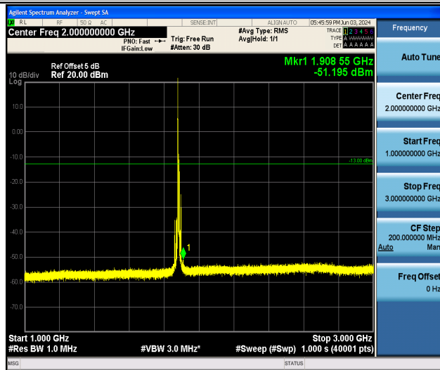
Band25_10MHz_QPSK_26365_1RB#0_1000~3000_1000~3000
