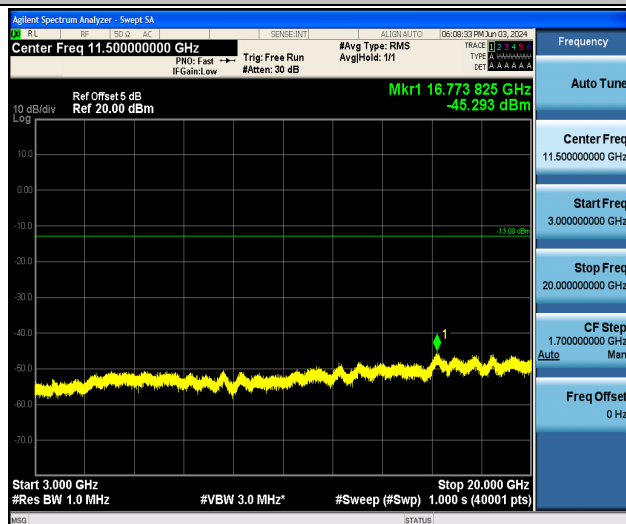
Band25_15MHz_QPSK_26365_1RB#0_3000~20000_3000~20000
