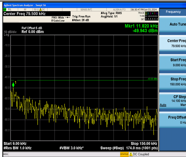
Band25_20MHz_16QAM_26590_1RB#0_0.009~0.15_0.009~0.15
