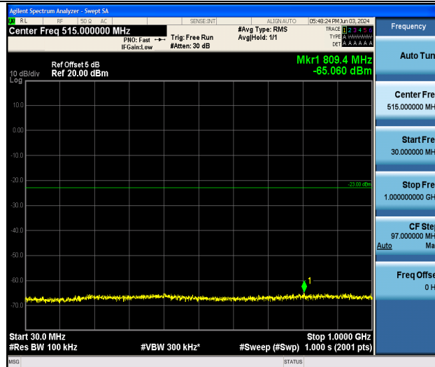
Band25_10MHz_16QAM_26640_1RB#0_30~1000_30~1000
