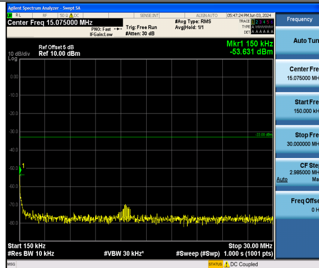
Band25_10MHz_QPSK_26640_1RB#0_0.15~30_0.15~30
