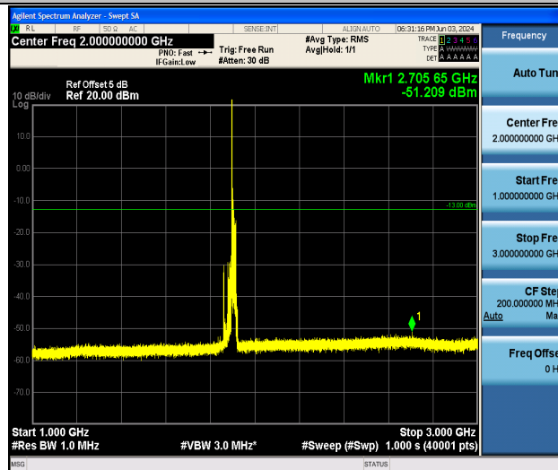
Band25_20MHz_16QAM_26590_1RB#0_1000~3000_1000~3000
