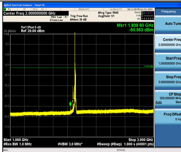
Band25_15MHz_16QAM_26615_1RB#0_1000~3000_1000~3000
