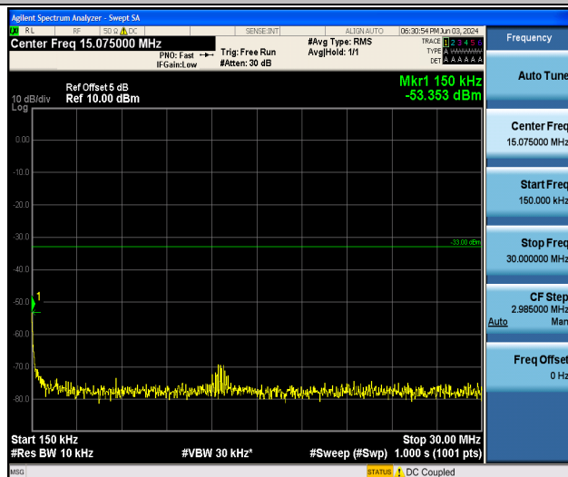
Band25_20MHz_16QAM_26590_1RB#0_0.15~30_0.15~30
