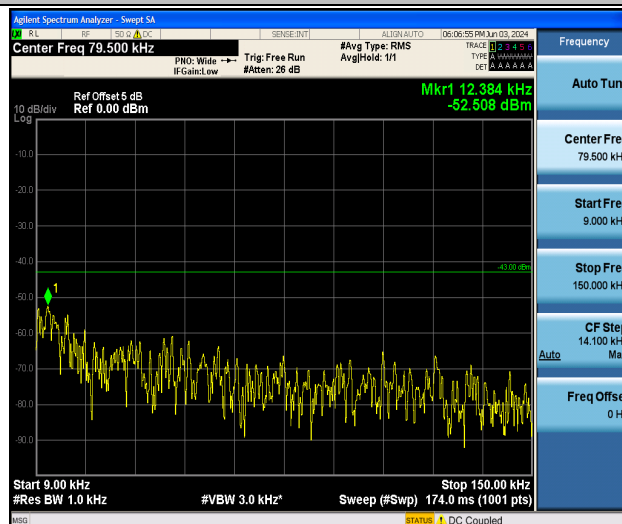
Band25_15MHz_16QAM_26115_1RB#0_0.009~0.15_0.009~0.15
