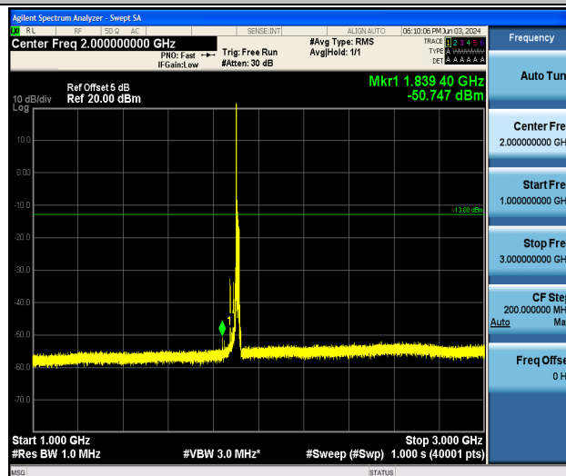
Band25_15MHz_QPSK_26615_1RB#0_1000~3000_1000~3000
