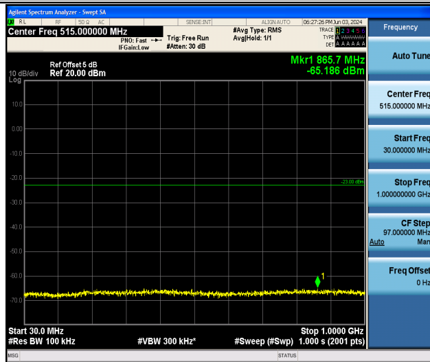
Band25_20MHz_16QAM_26140_1RB#0_30~1000_30~1000
