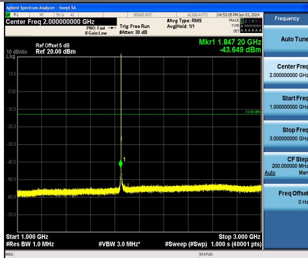
Band25_1.4MHz_QPSK_26047_1RB#0_1000~3000_1000~3000
