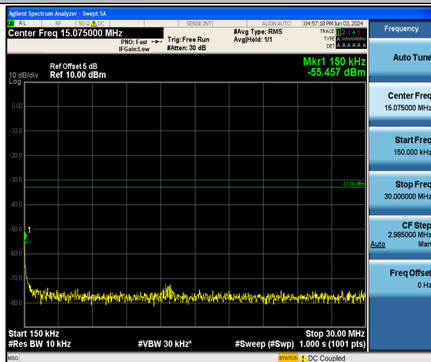
Band25_1.4MHz_16QAM_26683_1RB#0_0.15~30_0.15~30
