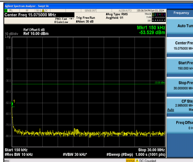
Band25_3MHz_QPSK_26365_1RB#0_0.15~30_0.15~30
