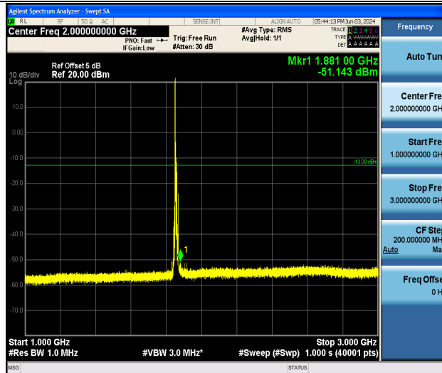
Band25_10MHz_QPSK_26090_1RB#0_1000~3000_1000~3000
