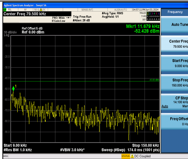
Band25_1.4MHz_16QAM_26683_1RB#0_0.009~0.15_0.009~0.15
