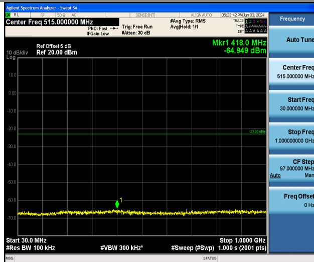
Band25_5MHz_QPSK_26365_1RB#0_30~1000_30~1000
