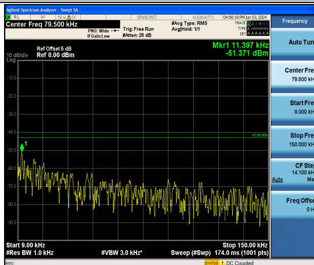
Band25_1.4MHz_QPSK_26683_1RB#0_0.009~0.15_0.009~0.15
