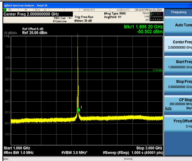
Band25_5MHz_QPSK_26365_1RB#0_1000~3000_1000~3000
