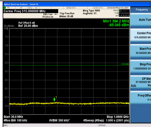
Band25_1.4MHz_16QAM_26047_1RB#0_30~1000_30~1000
