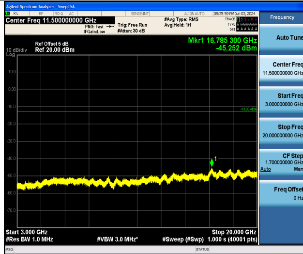
Band25_5MHz_QPSK_26665_1RB#0_3000~20000_3000~20000
