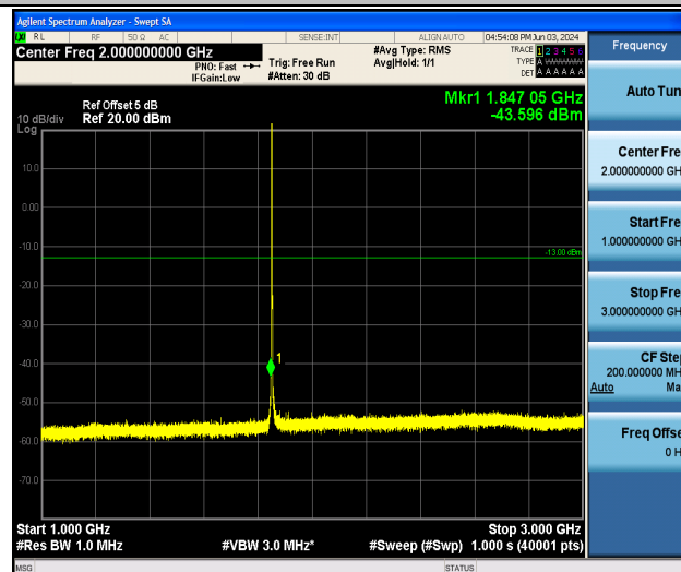
Band25_1.4MHz_16QAM_26047_1RB#0_1000~3000_1000~3000
