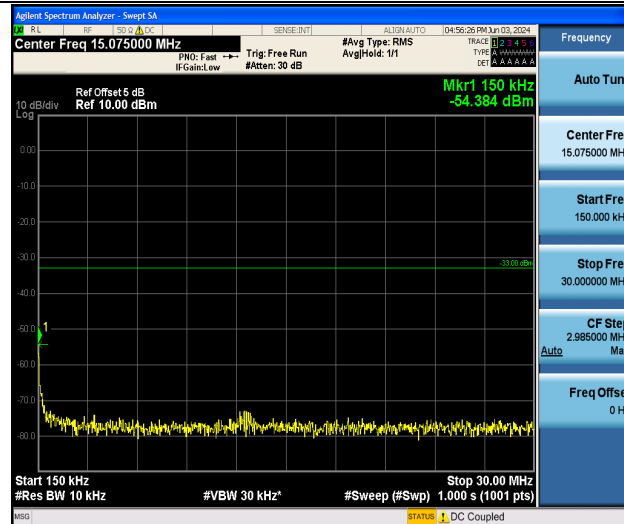
Band25_1.4MHz_QPSK_26683_1RB#0_0.15~30_0.15~30
