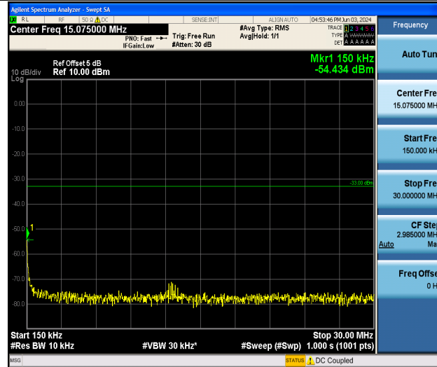
Band25_1.4MHz_16QAM_26047_1RB#0_0.15~30_0.15~30
