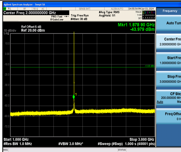
Band25_1.4MHz_16QAM_26365_1RB#0_1000~3000_1000~3000
