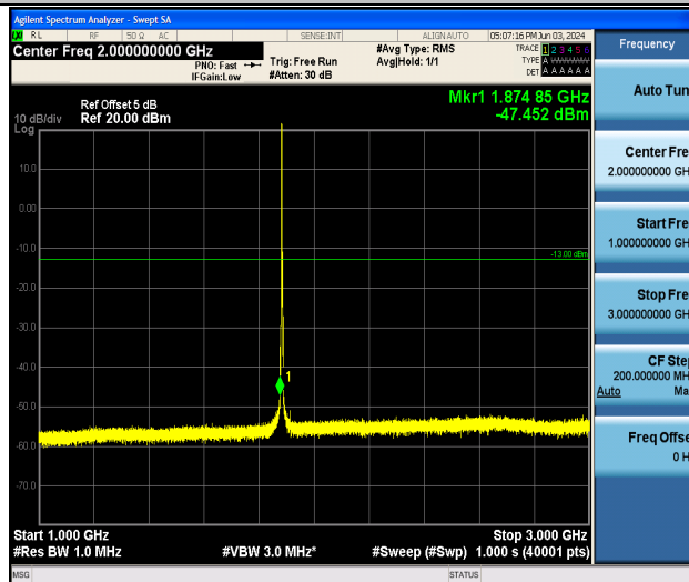
Band25_3MHz_QPSK_26365_1RB#0_1000~3000_1000~3000
