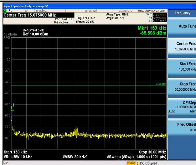
Band25_5MHz_QPSK_26365_1RB#0_0.15~30_0.15~30
