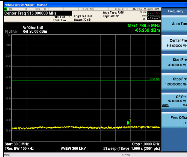
Band25_5MHz_16QAM_26665_1RB#0_30~1000_30~1000
