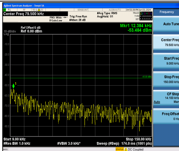
Band25_1.4MHz_16QAM_26047_1RB#0_0.009~0.15_0.009~0.15
