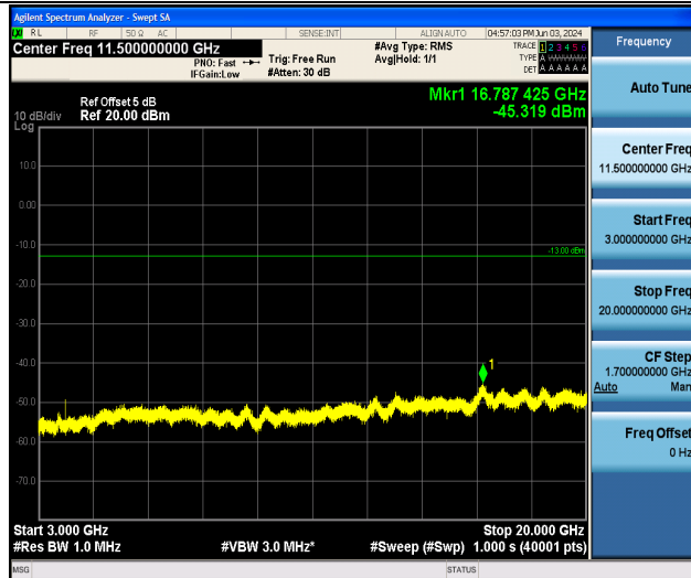
Band25_1.4MHz_QPSK_26683_1RB#0_3000~20000_3000~20000
