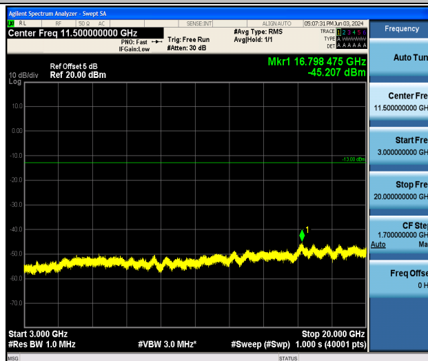
Band25_3MHz_QPSK_26365_1RB#0_3000~20000_3000~20000
