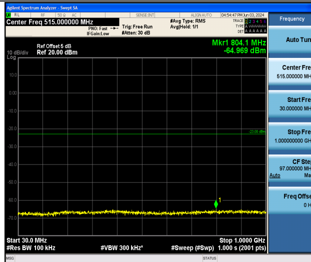
Band25_1.4MHz_QPSK_26365_1RB#0_30~1000_30~1000
