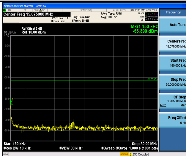
Band25_5MHz_16QAM_26665_1RB#0_0.15~30_0.15~30
