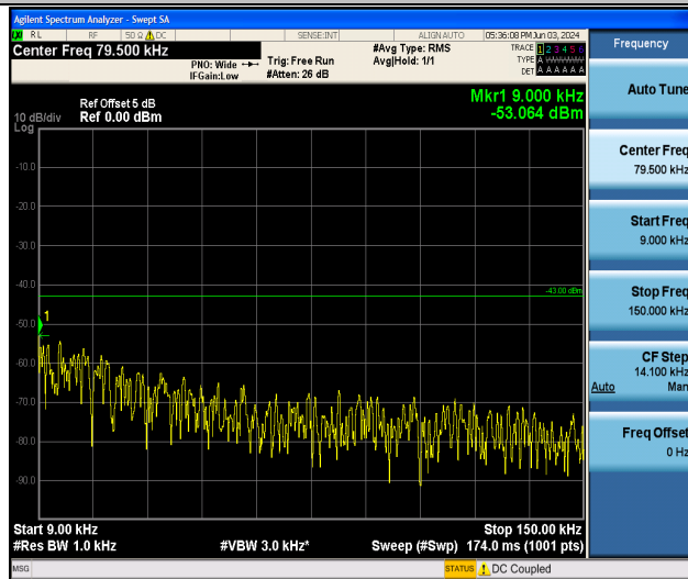
Band25_5MHz_16QAM_26665_1RB#0_0.009~0.15_0.009~0.15
