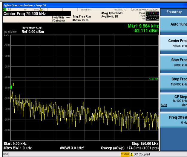
Band25_5MHz_QPSK_26365_1RB#0_0.009~0.15_0.009~0.15
