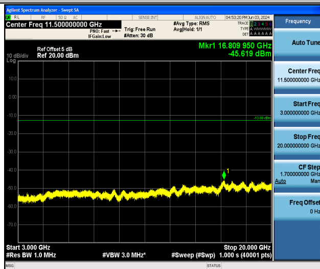
Band25_1.4MHz_QPSK_26047_1RB#0_3000~20000_3000~20000
