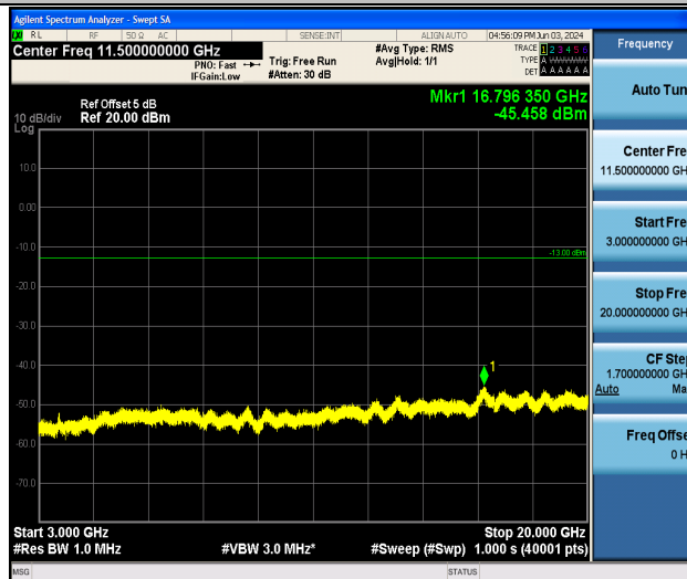
Band25_1.4MHz_16QAM_26365_1RB#0_3000~20000_3000~20000
