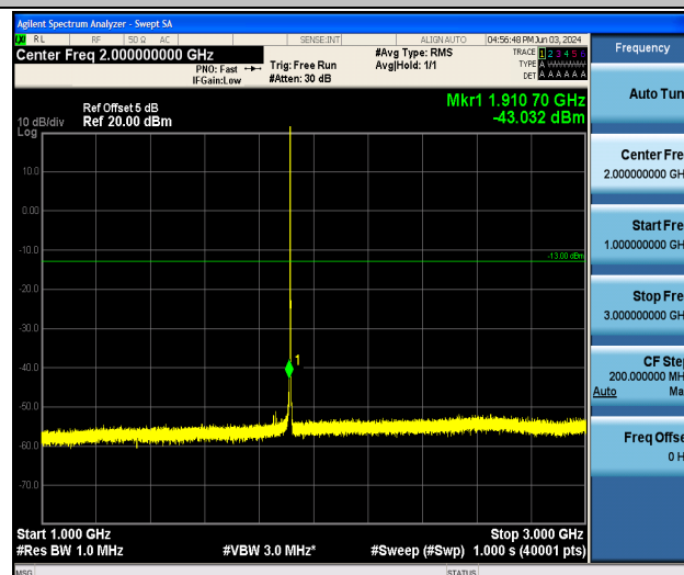
Band25_1.4MHz_QPSK_26683_1RB#0_1000~3000_1000~3000
