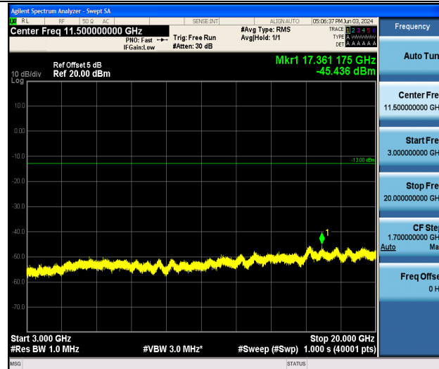
Band25_3MHz_16QAM_26055_1RB#0_3000~20000_3000~20000
