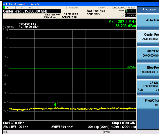
Band25_3MHz_QPSK_26365_1RB#0_30~1000_30~1000
