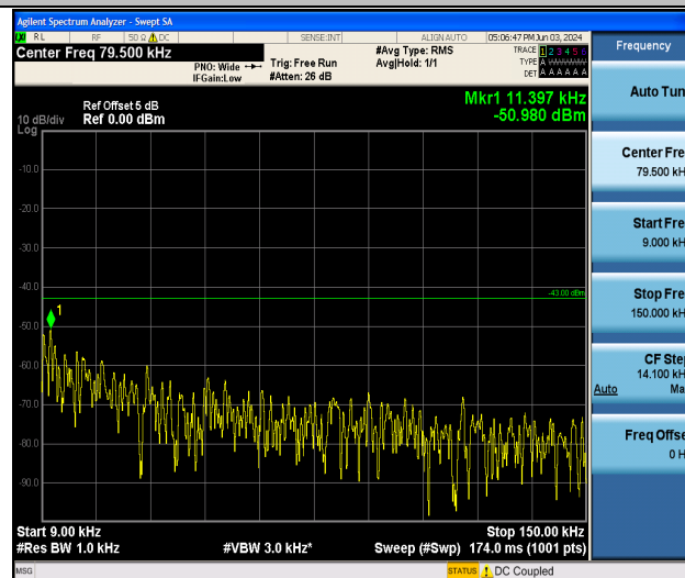
Band25_3MHz_QPSK_26365_1RB#0_0.009~0.15_0.009~0.15
