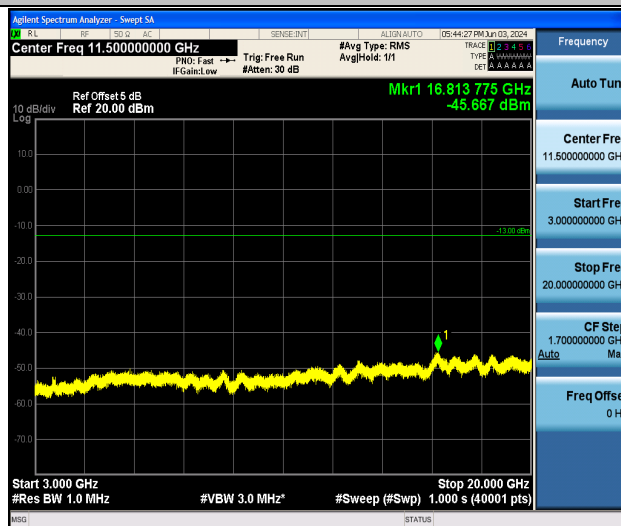
Band25_10MHz_QPSK_26090_1RB#0_3000~20000_3000~20000
