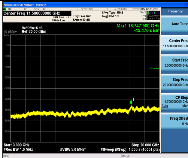
Band25_5MHz_16QAM_26065_1RB#0_3000~20000_3000~20000
