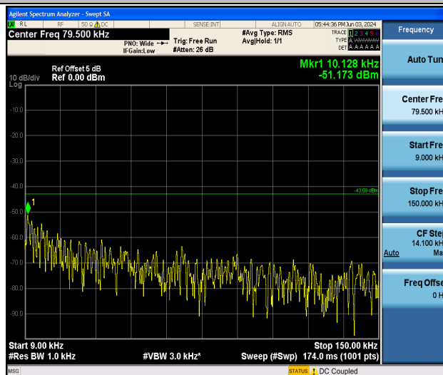
Band25_10MHz_16QAM_26090_1RB#0_0.009~0.15_0.009~0.15
