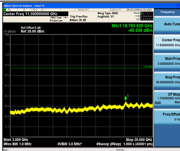
Band25_5MHz_QPSK_26365_1RB#0_3000~20000_3000~20000
